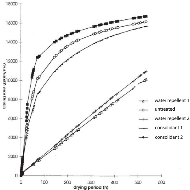
FIG. 4.3 Drying curve of a material: untreated, treated with water repellent treatments and treated with consolidant treatments (adapted from Hees et al., 1998)
