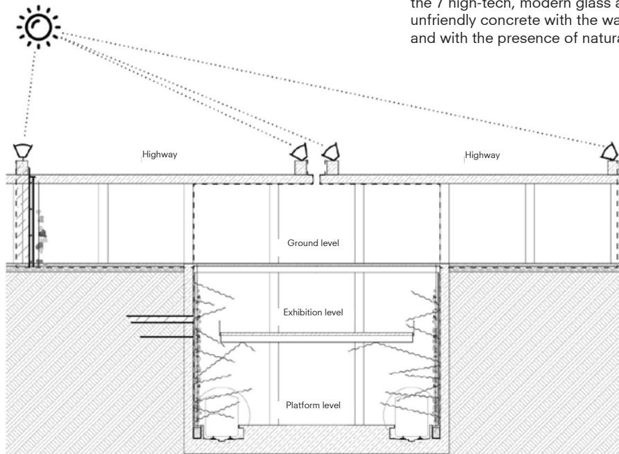
Solar Lighting System (Parans) Short Section
