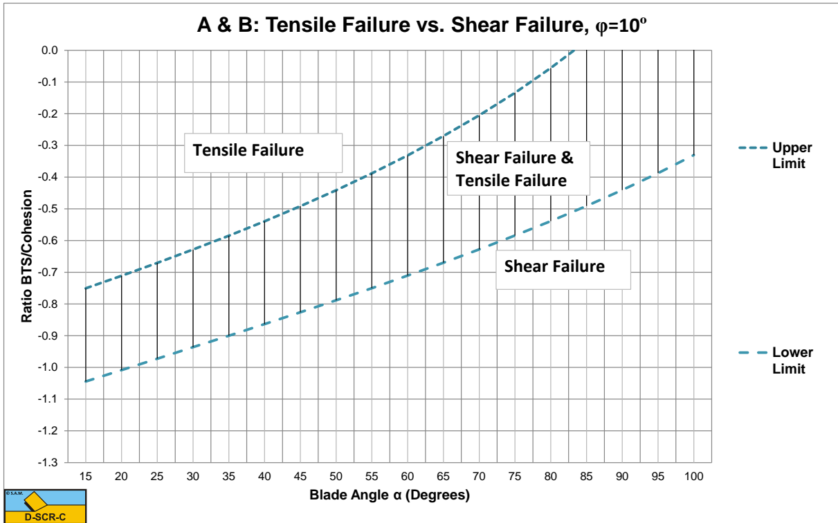
Figure W-15: The tensile/shear failure range based on BTS/Cohesion for \phi=10^\circ .
