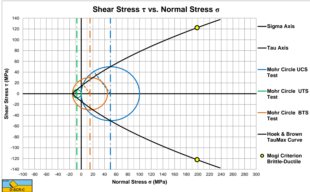
Figure 8-11: Construction Hoek & Brown failure criterion Mohr circles.
