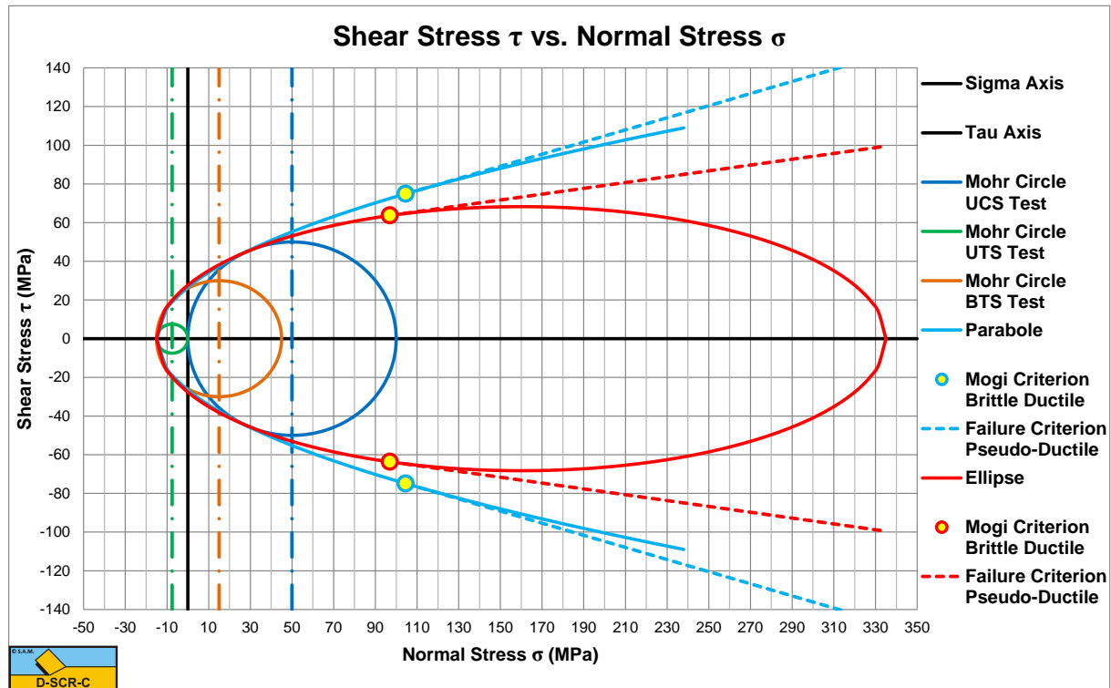
Figure 8-14: The Parabolic and Ellipsoid failure envelopes, with a=1.75 \cdot UCS .
