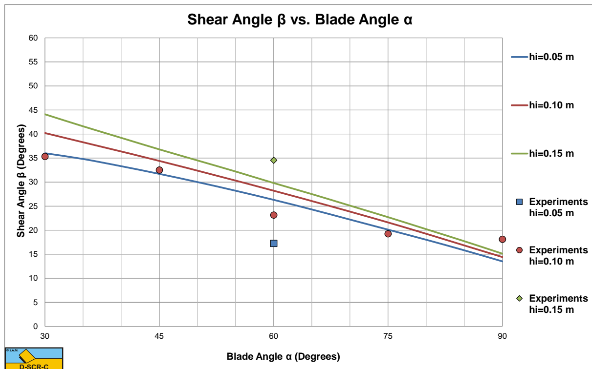
Figure 5-19: The shear angle versus the blade angle.
