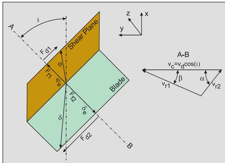
Figure 3-18: Force directions.
