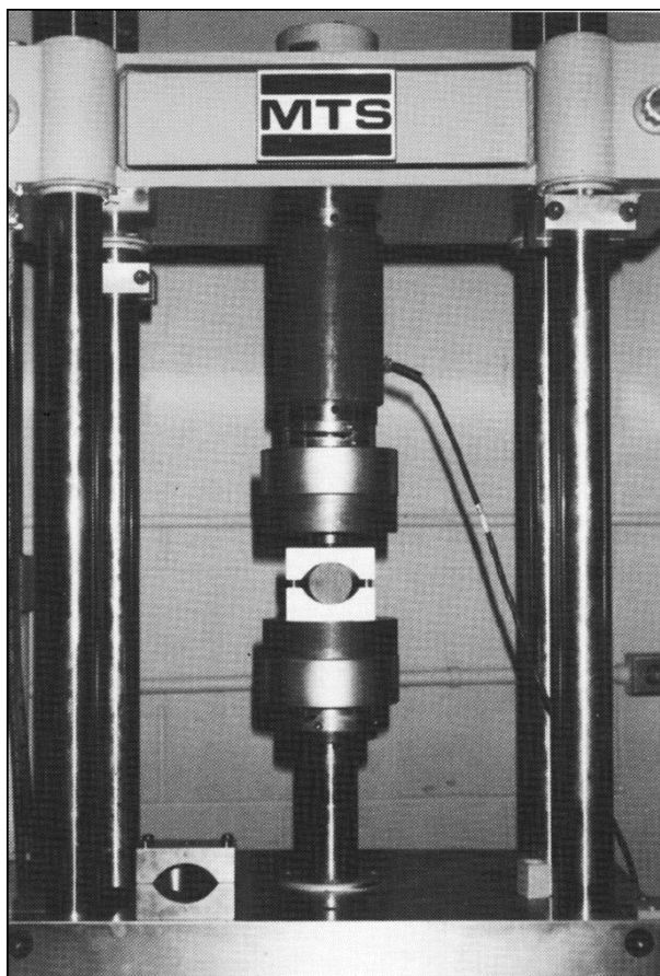
Figure 2-41: Brazilian splitting tension test.
