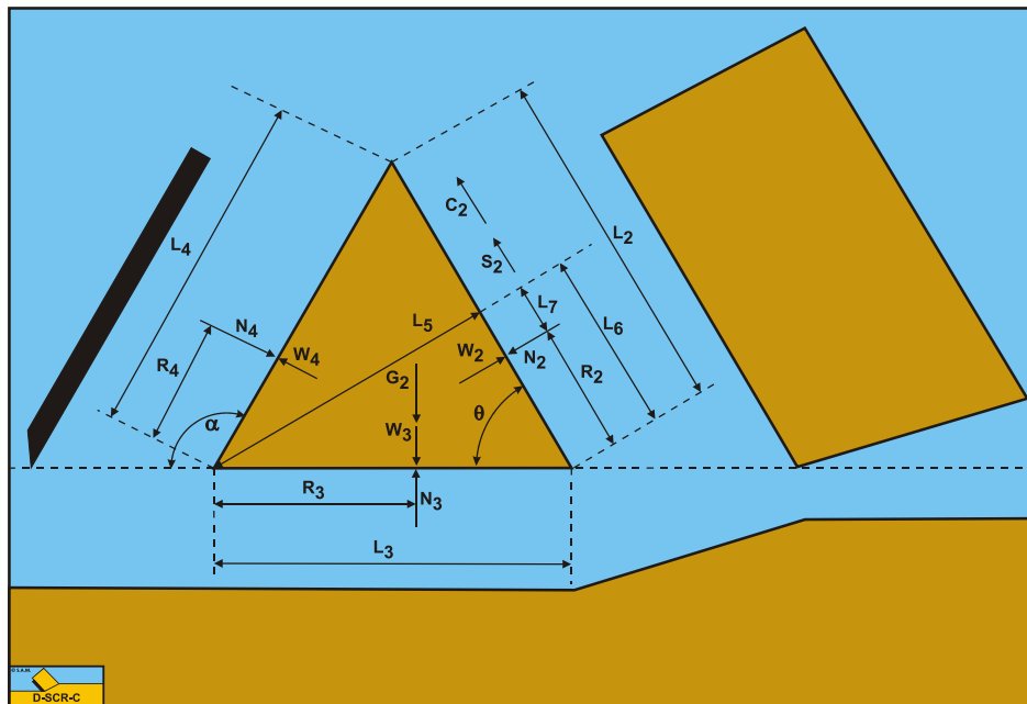
Figure 10-5: The moments on the wedge.
