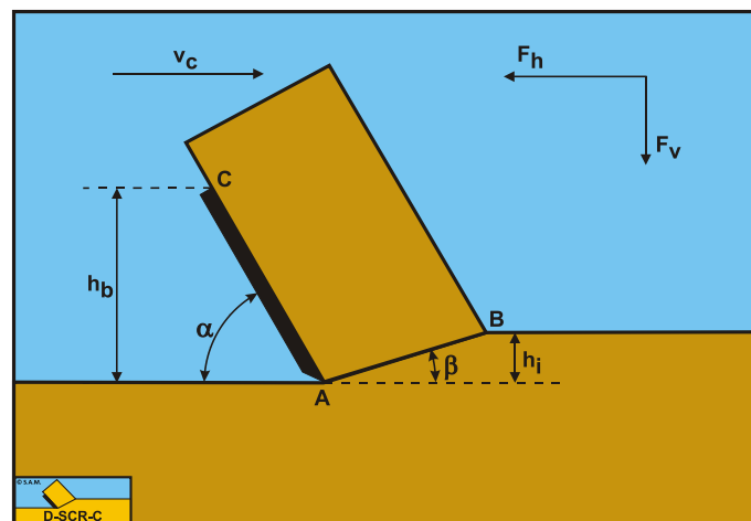
Figure 6-1: The cutting process definitions.
