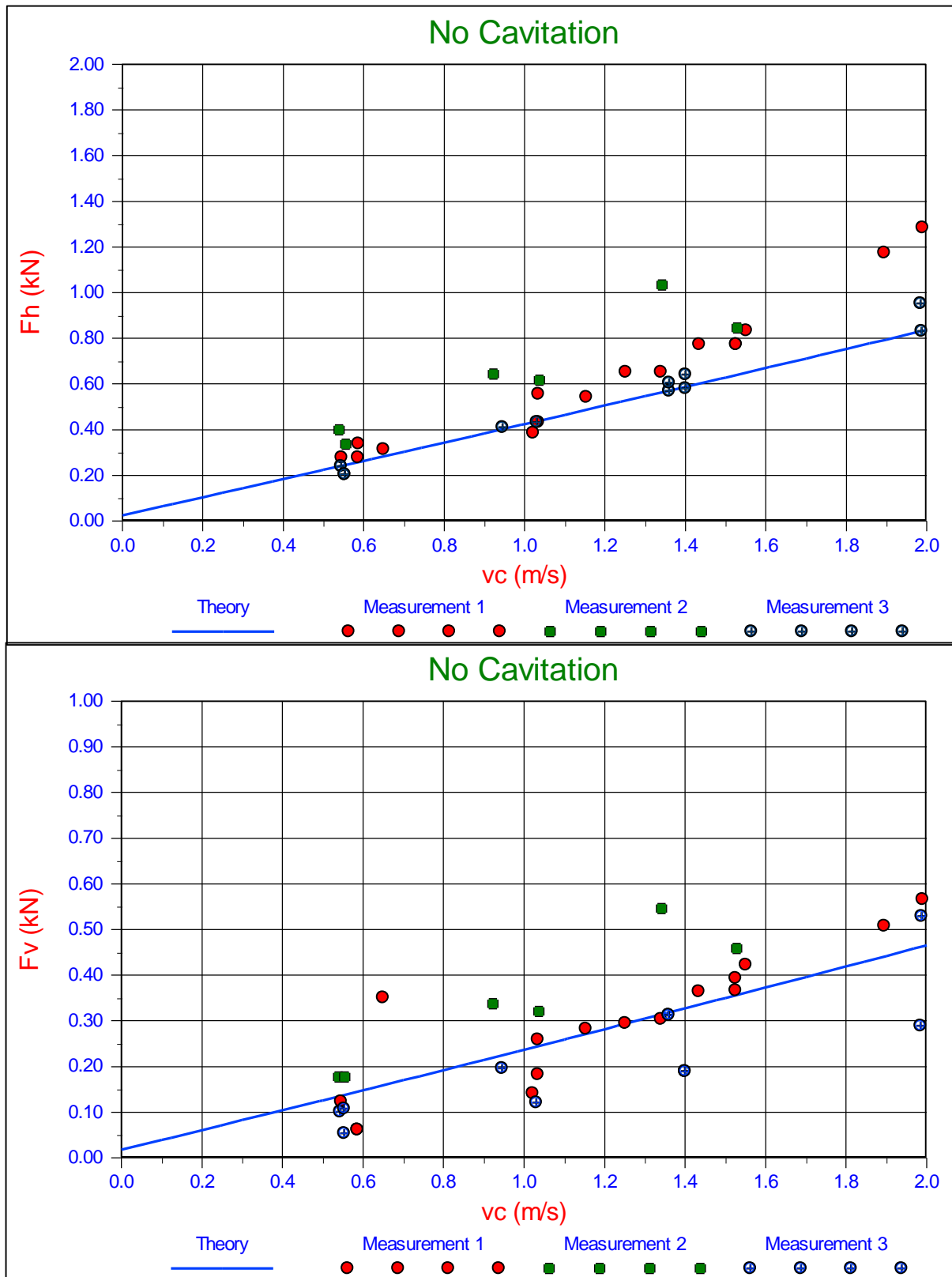
Figure M-20: \alpha=30^\circ , h_i=33 mm, h_b=100 mm.
