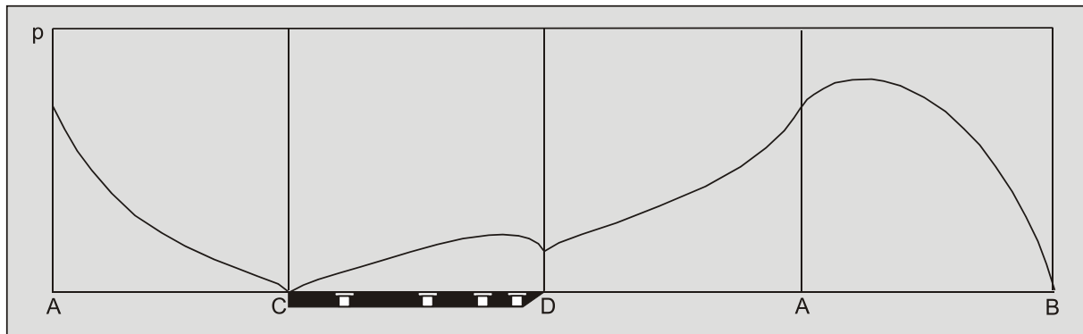
Figure S-12: Pore pressure distribution on the shear plane A-B, the bottom of the wedge A-D, the blade D-C and the front of the wedge A-C.
