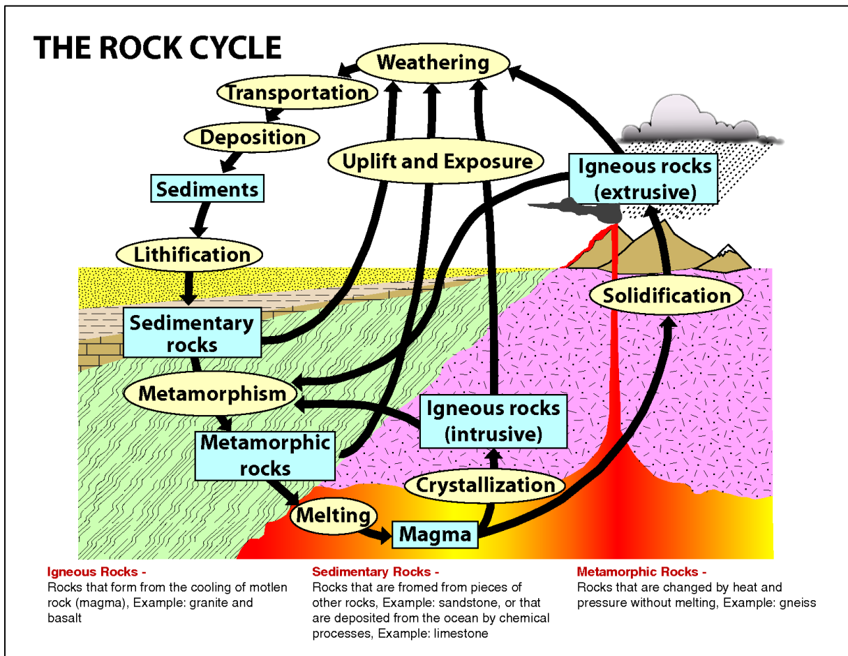
Figure 2-17: The rock formation cycle (galleryhip.com).
