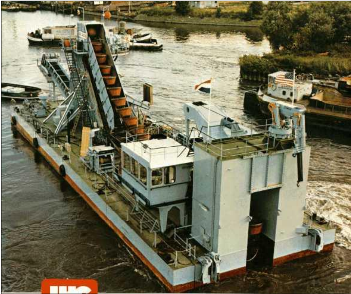
Figure Y-4: A bucket ladder dredge (IHC).
