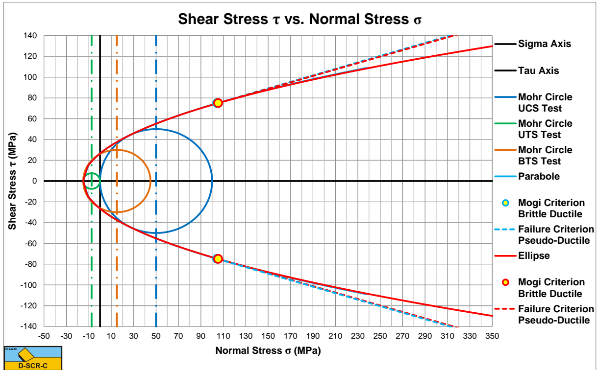
Figure 8-15 The Parabolic and Ellipsoid failure envelopes, with a=100 \cdot \text{UCS} .
