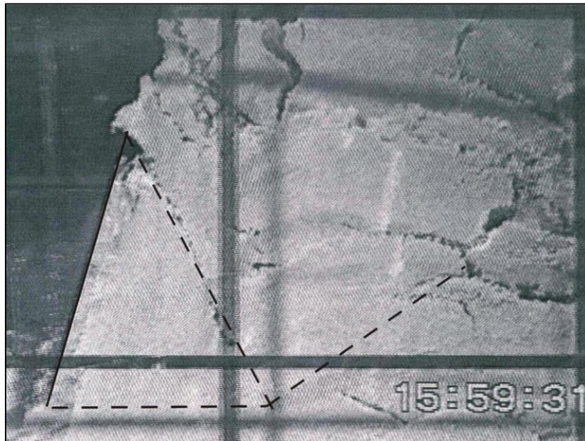
Figure 12-1: Failure pattern with rake angle of 120^\circ .
