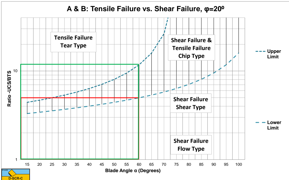
Figure W-10: The tensile/shear failure range based on UCS/BTS for \phi=20^\circ .
