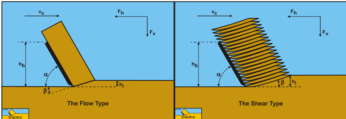
Figure 3-3: The Flow Type
