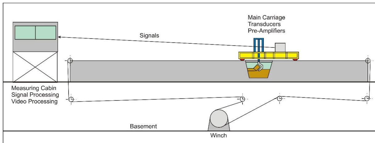
Figure 6-36: Side view of the old laboratory.
