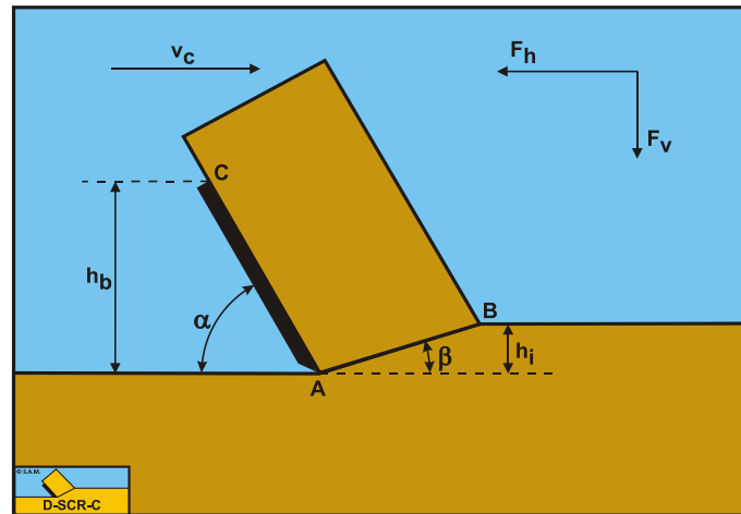
Figure 5-3: The cutting process, definitions.
