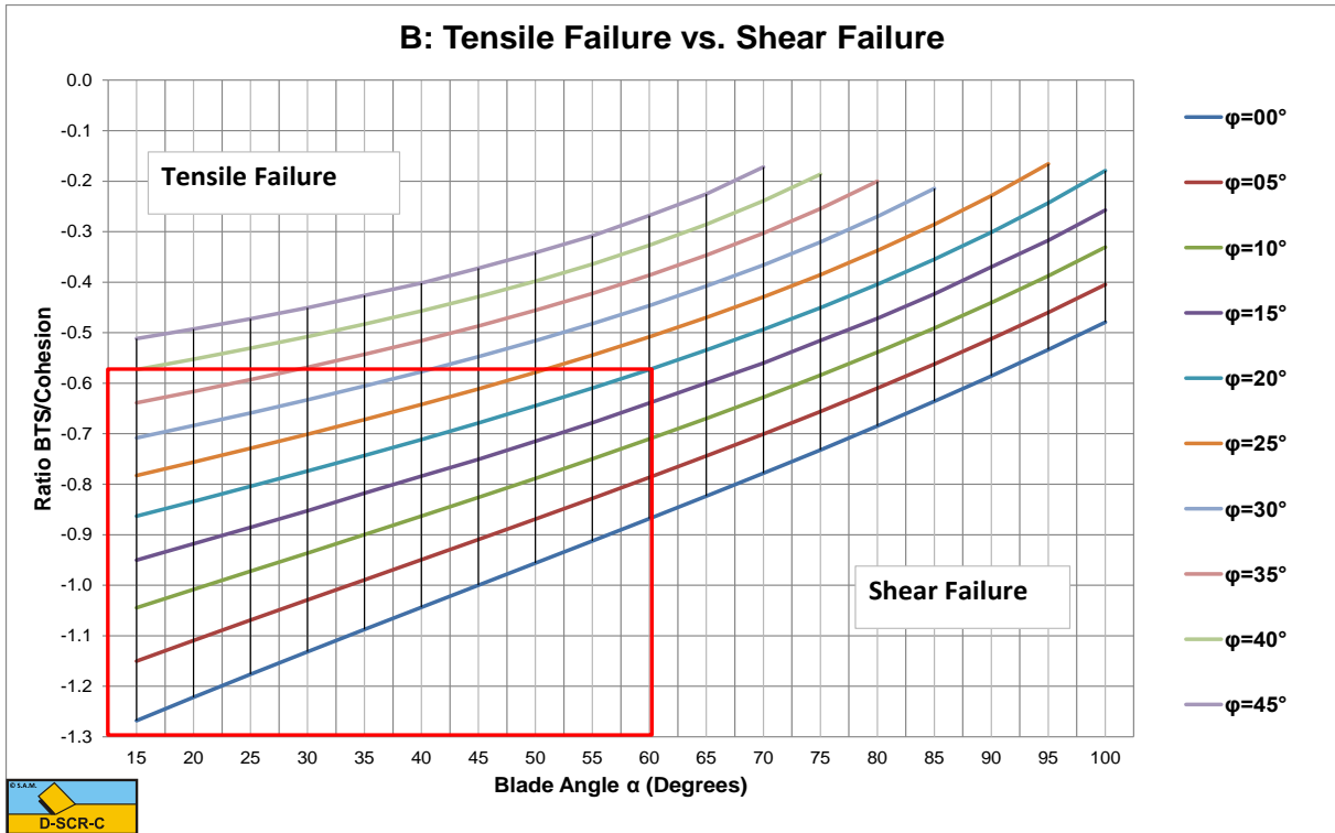
Figure 8-47: Below the lines (equation (8-125)) the cutting process is brittle (shear failure); above the lines it is brittle (tensile failure).
