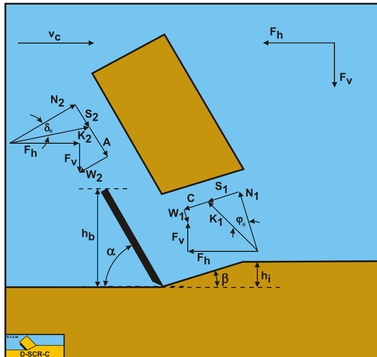
Figure 3-14: The forces on the layer cut.
