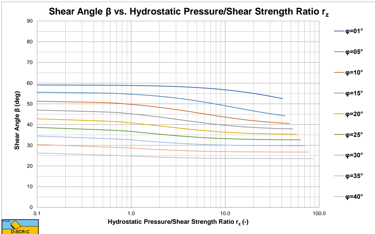
Figure 9-18: The shear angle \beta for a 60 degree blade
