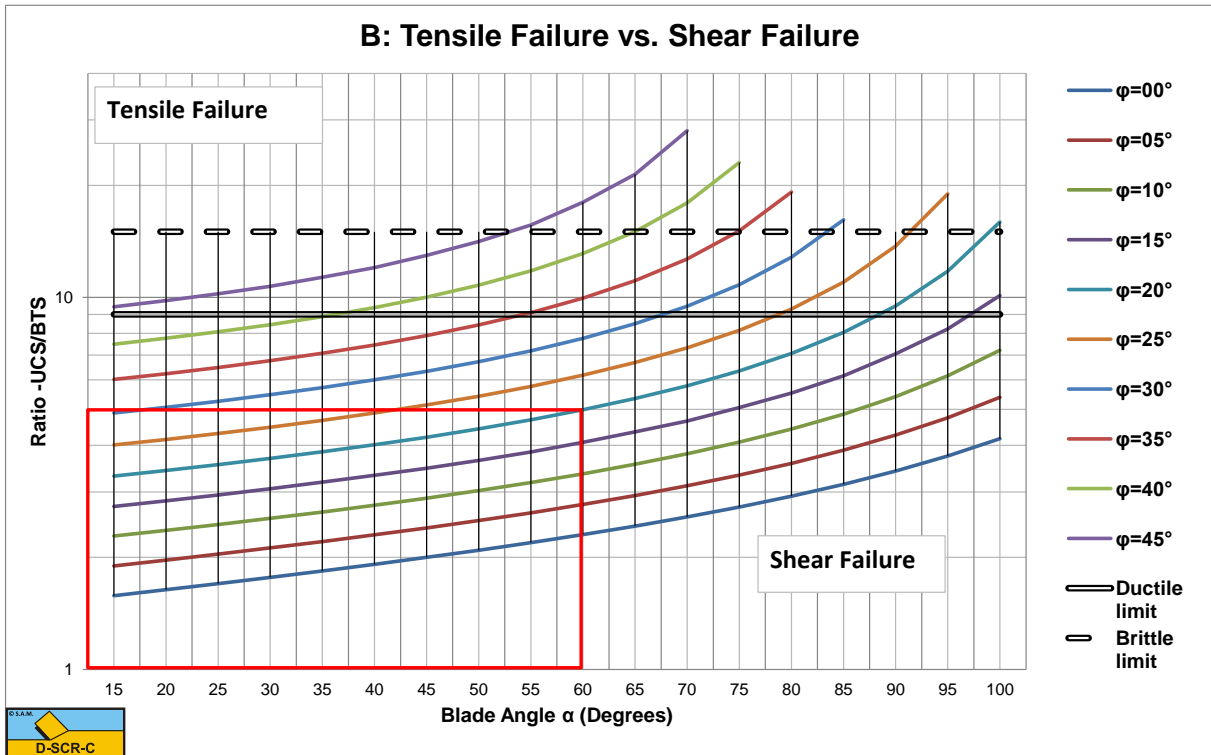
Figure W-8: The tensile/shear failure criterion based on UCS/BTS.
