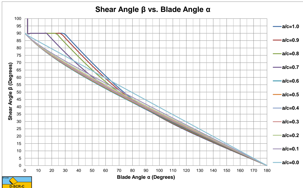
Figure 7-35: The shear angle \beta for the Curling Type.
