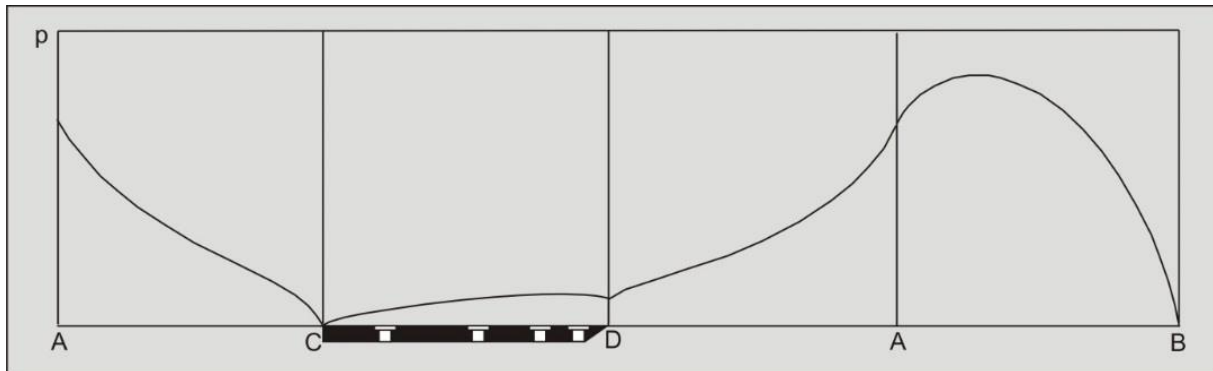
Figure 12-10: Pore pressure distribution on the shear plane A-B, the bottom of the wedge A-D, the blade D-C and the front of the wedge A-C.
