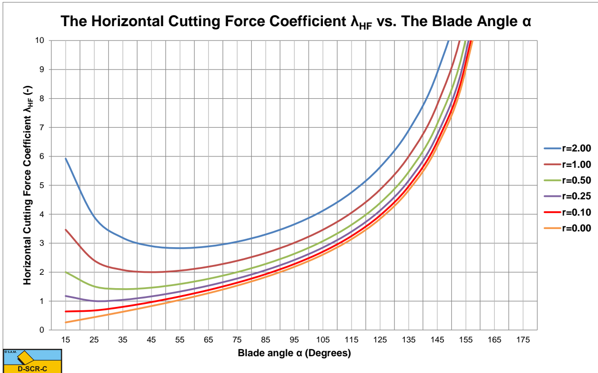
Figure 7-23: The horizontal cutting force coefficient \lambda_{HF} as a function of the blade angle and the ac ratio r .
