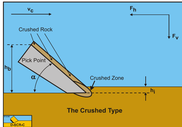
Figure 9-6: The Crushed Type cutting mechanism.
