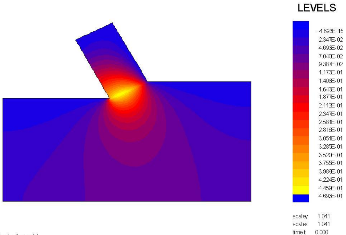
Figure S-4: The equipotential lines in color.
