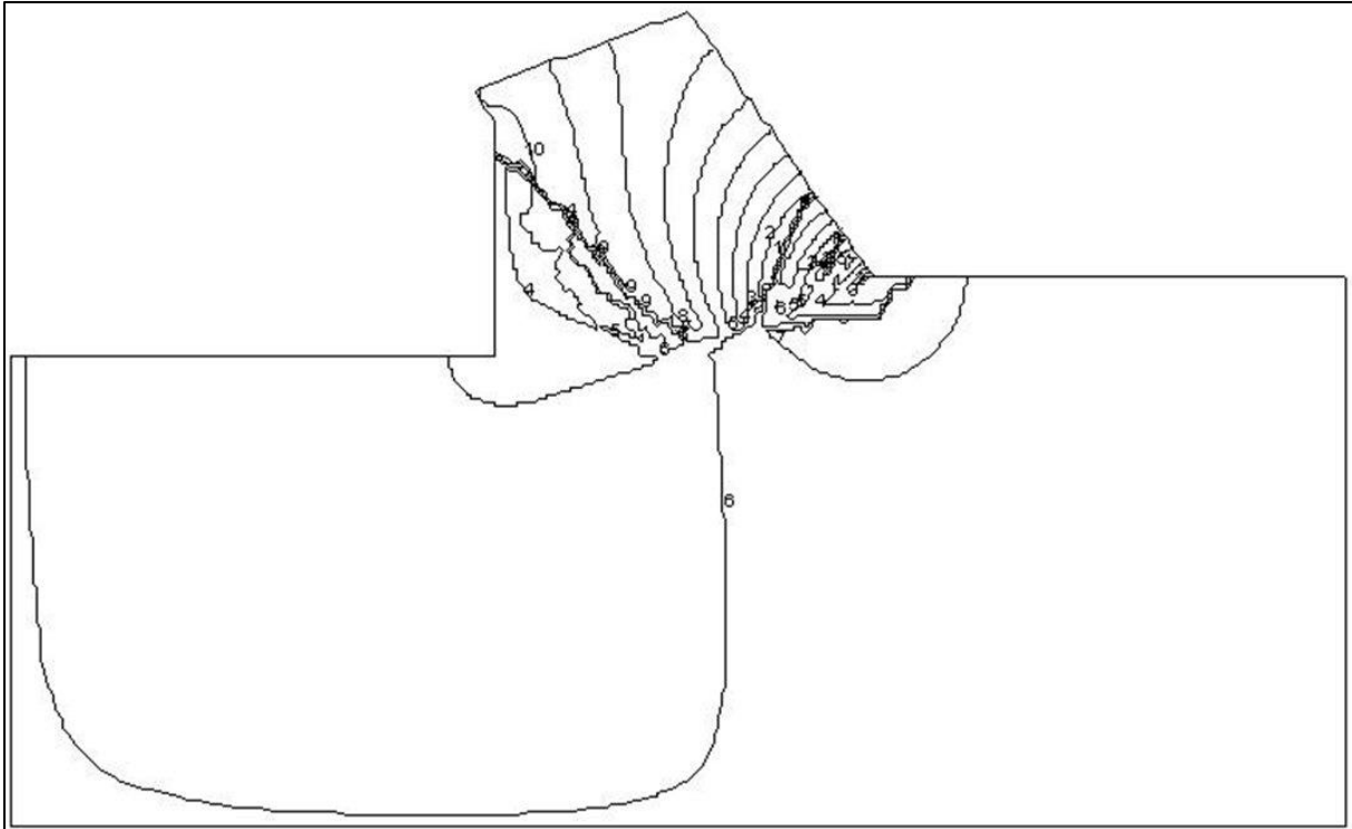
Figure 12-16: The flow lines or stream function.
