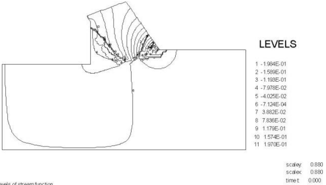
Figure S-15: The flow lines or stream function.
