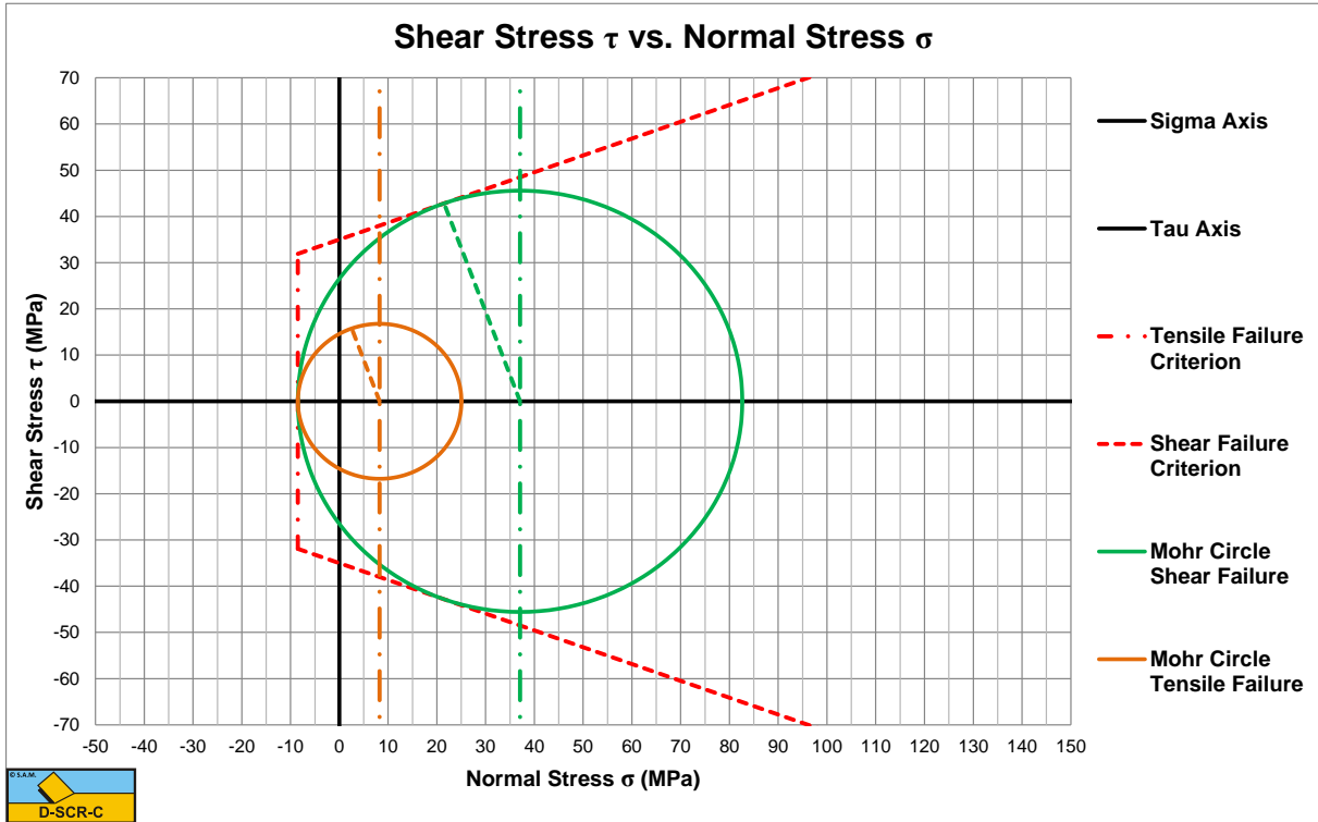
Figure 8-51: Mohr circles tensile strength -8.5 MPa.
