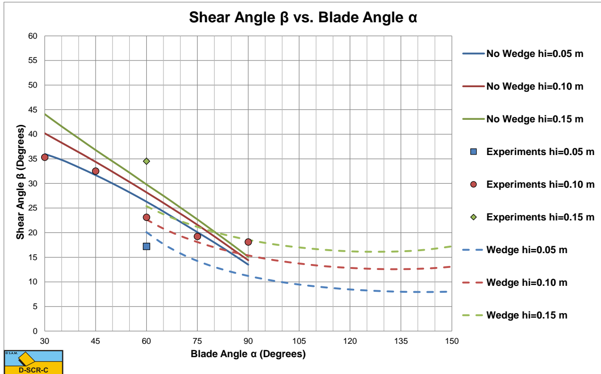
Figure 11-11: The shear angle of Hatamura & Chijiwa (1977B) versus the calculated shear angles, with and without wedge.
