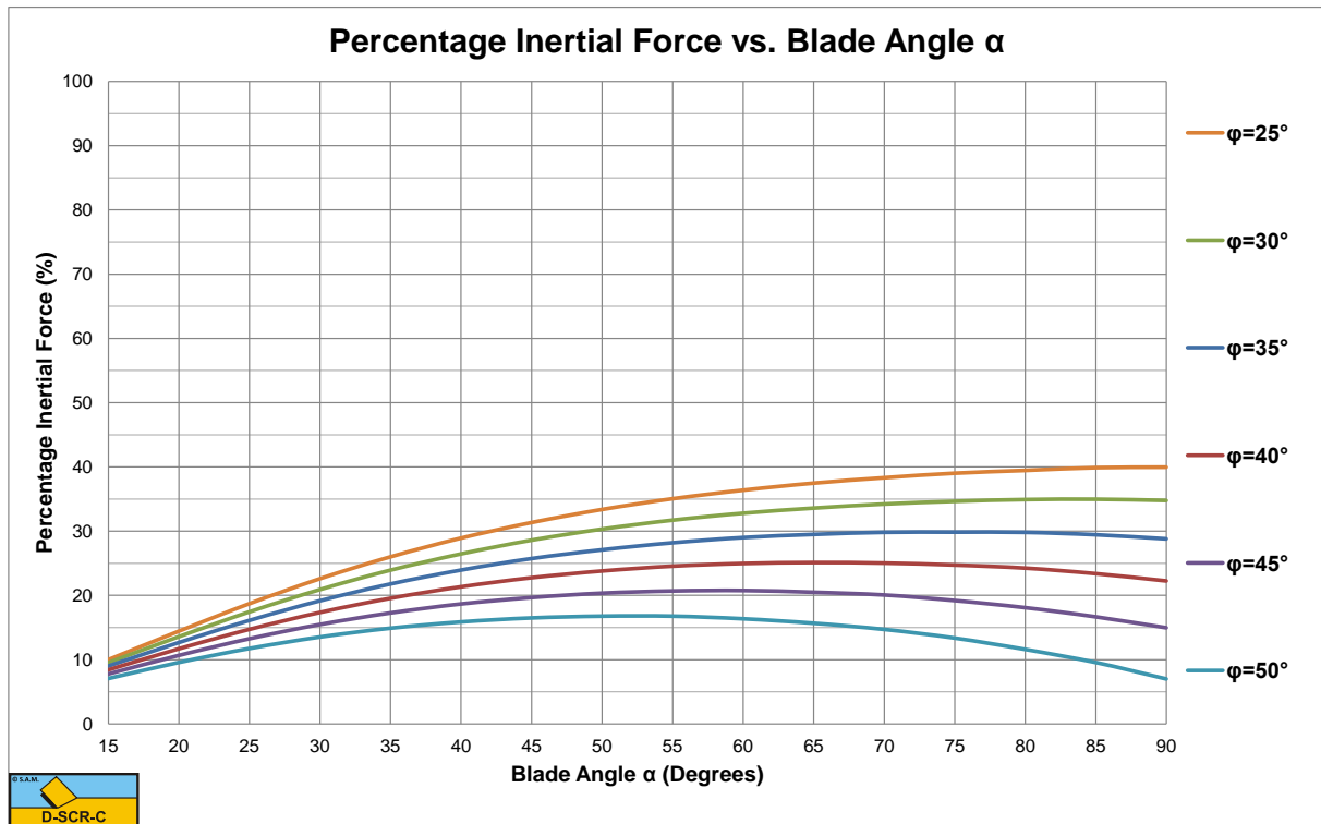
Figure B-21: The percentage inertial force for a dimensionless inertial effect parameter \lambda_i=2.5 .
