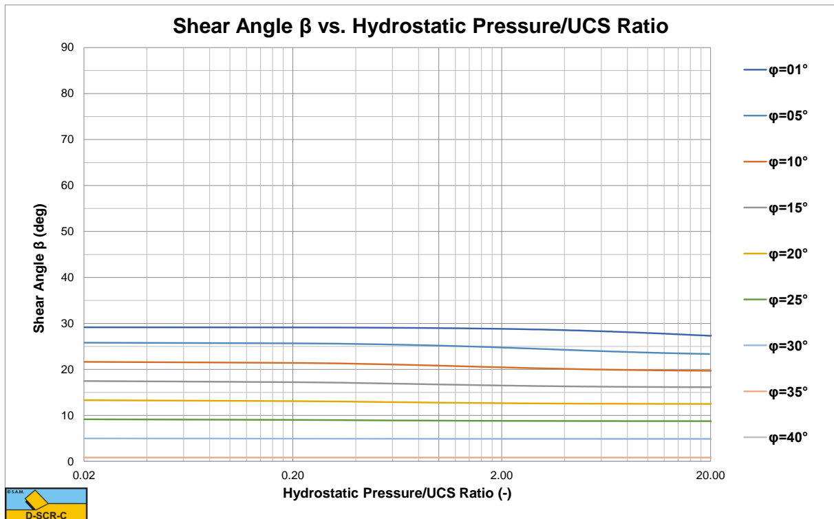
Figure X-32: The shear angle \beta for a 120 degree blade.
