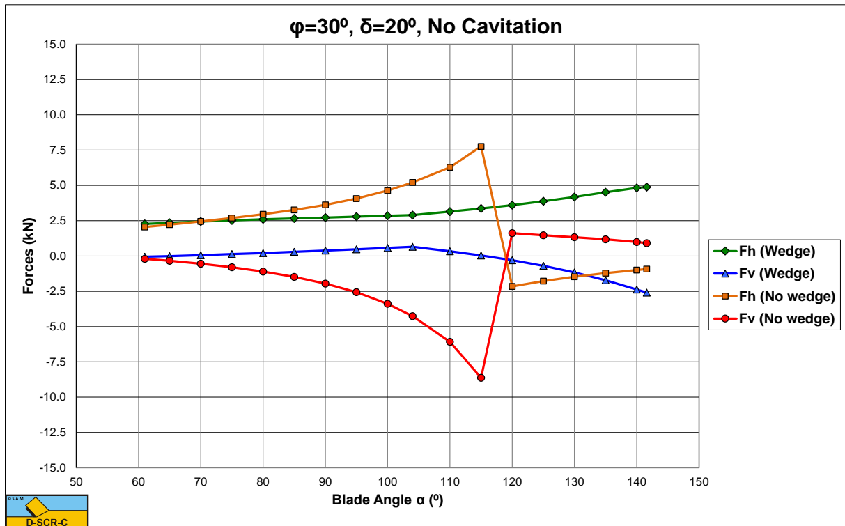
Figure P-2: No cavitation, the cutting forces as a function of the blade angle \alpha for \varphi=30^\circ and \delta=20^\circ .
