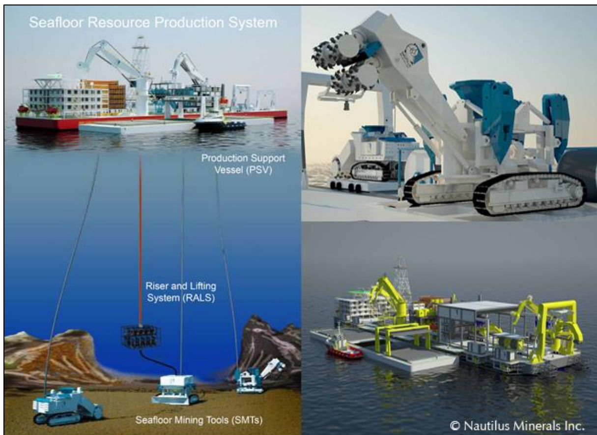
Figure Y-45: Deep sea mining, the Solwara Field.
