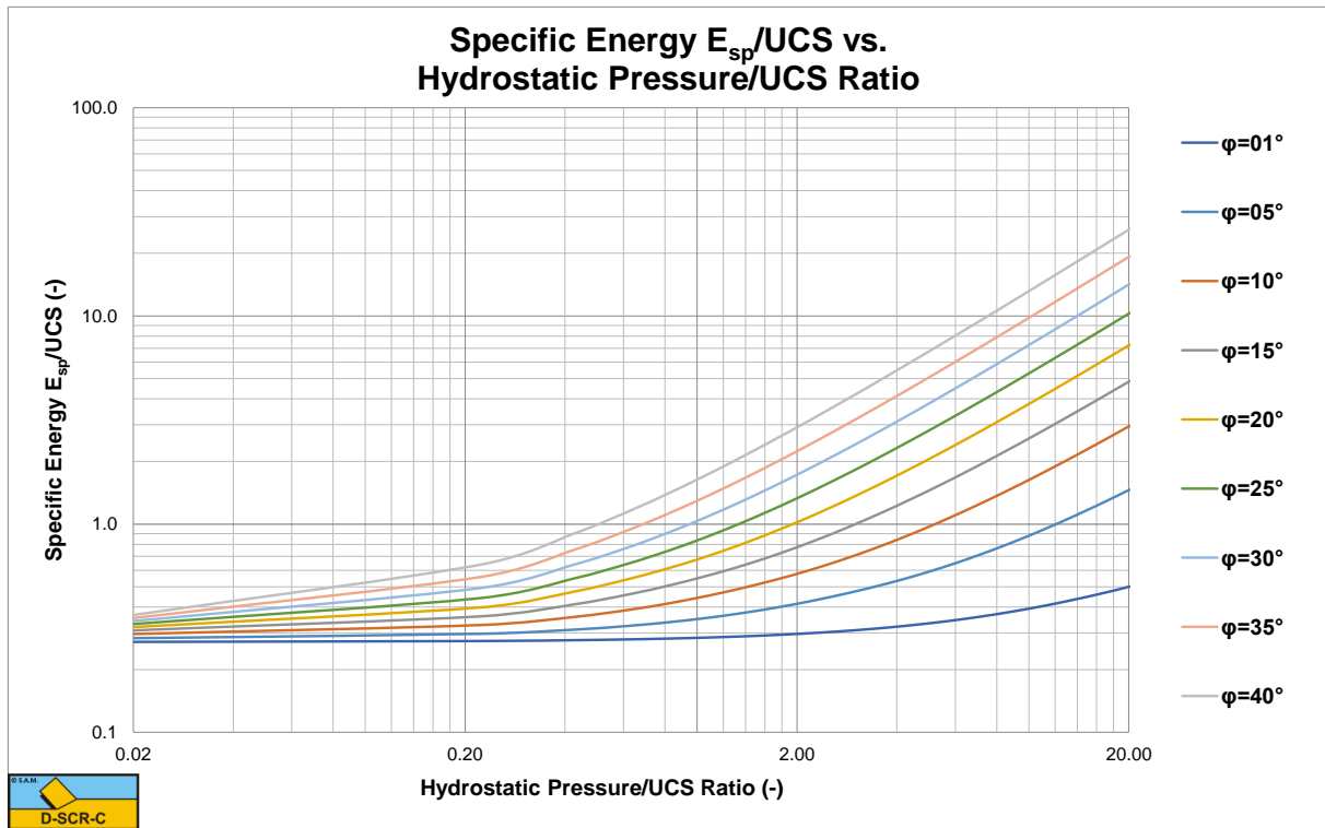
Figure X-5: The specific energy to UCS ratio for a 30 degree blade.
