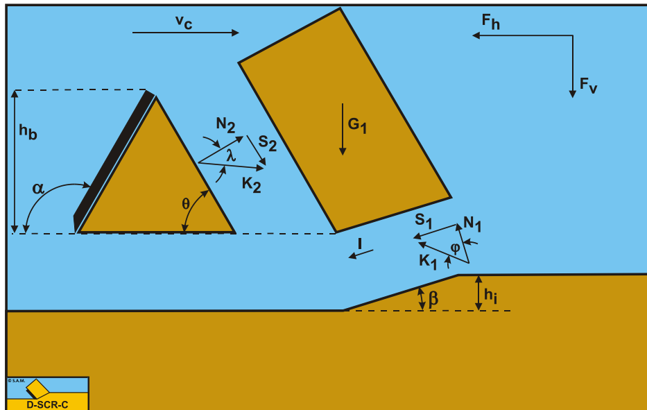
Figure 11-4: The forces on the layer cut when a wedge is present.
