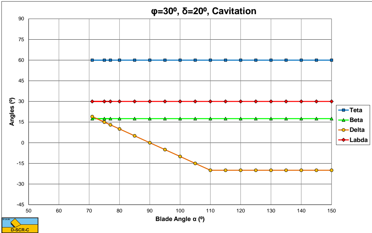
Figure 12-24: Cavitating, the angles \theta , \beta , \delta_m and \lambda as a function of the blade angle \alpha for \phi=30^\circ and \delta=20^\circ .
