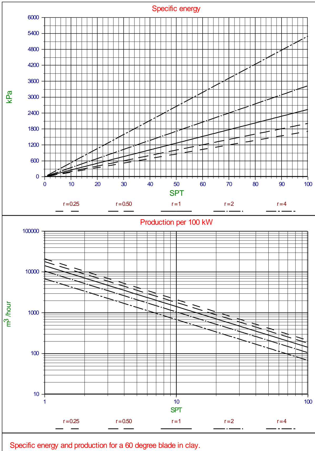
Figure 7-25: Specific energy and production in clay for a 60 degree blade.
