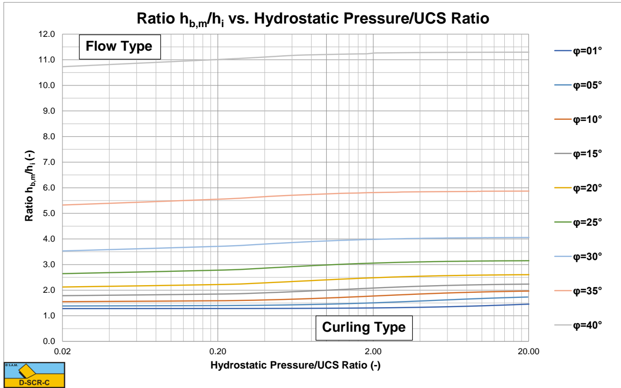
Figure X-26: The ratio h_{b,m}/h_i for a 105 degree blade.
