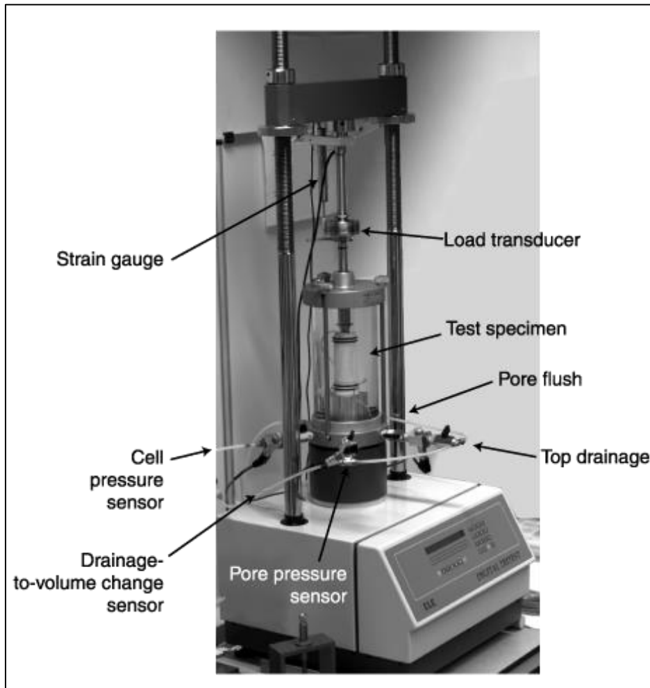
Figure 2-35: The Triaxial apparatus ( www.geotechdata.info ).
