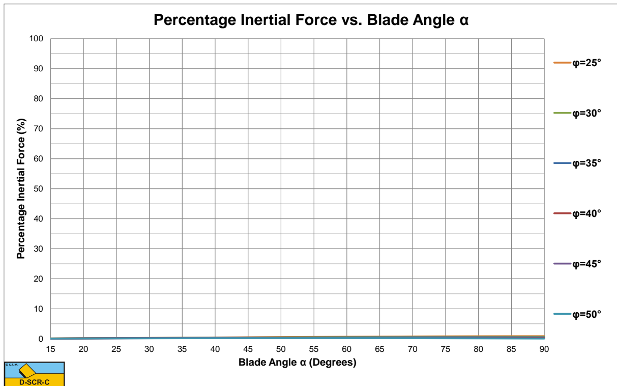
Figure B-19: The percentage inertial force for a dimensionless inertial effect parameter \lambda_i=0.025 .
