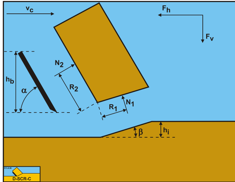
Figure 8-40: The moments on the layer cut.
