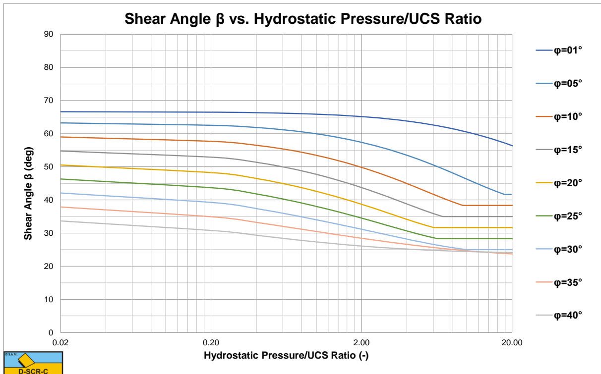
Figure X-7: The shear angle \beta for a 45 degree blade.
