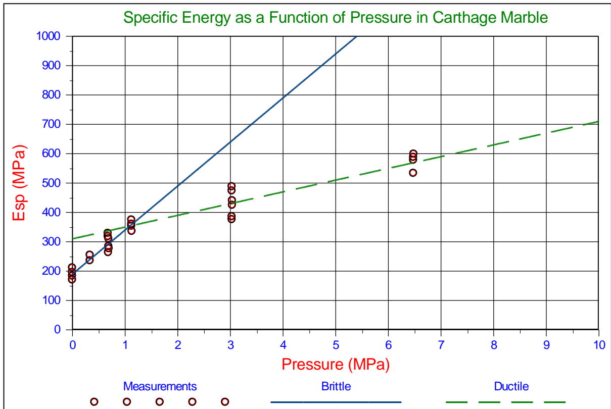
Figure 9-2: MSE versus confining pressure for Carthage marble in light and viscous mineral oil, Rafatian et al. (2009).
