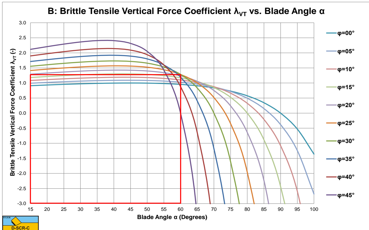
Figure W-37: The brittle (tensile failure) vertical force coefficient \lambda_{VT} , corrected.
