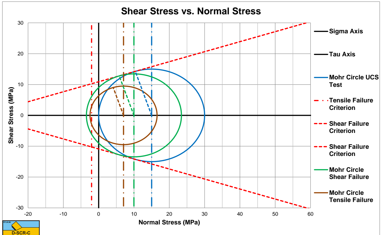
Figure 16-8: The Mohr circles for a tensile strength of -2 MPa. Tensile Failure.
