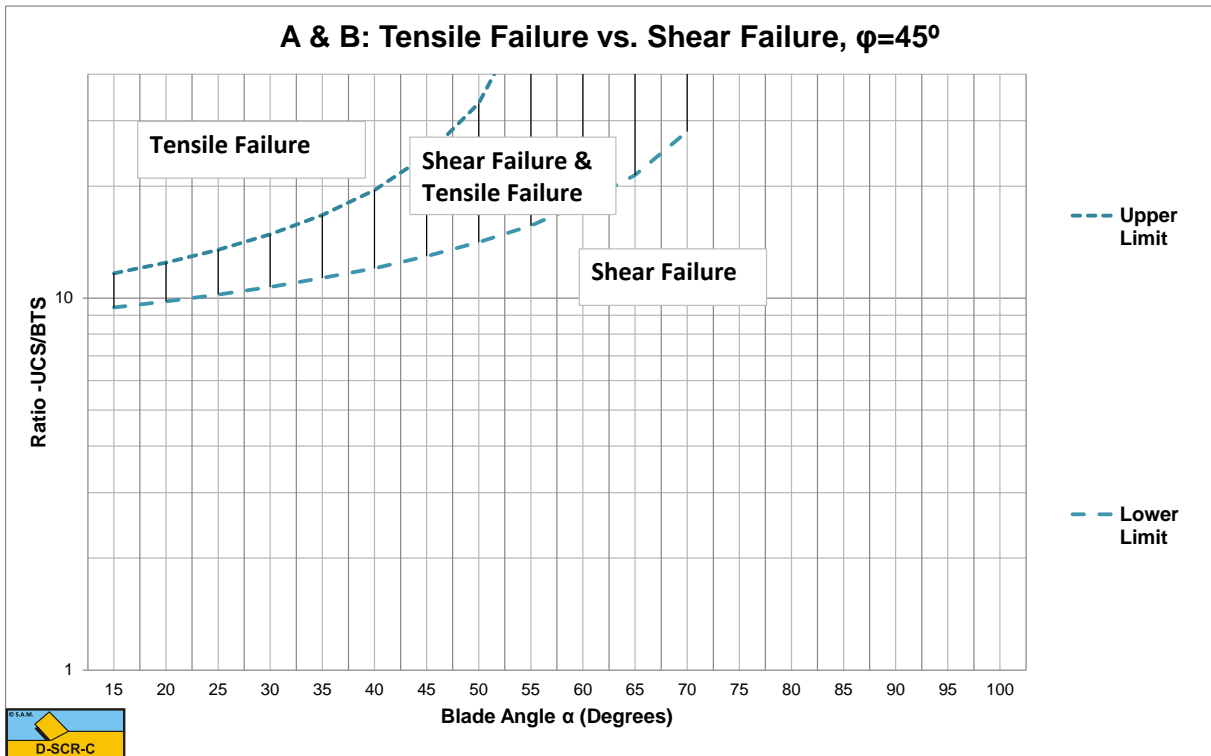
Figure W-30: The tensile/shear failure range based on UCS/BTS for \phi=45^\circ .
