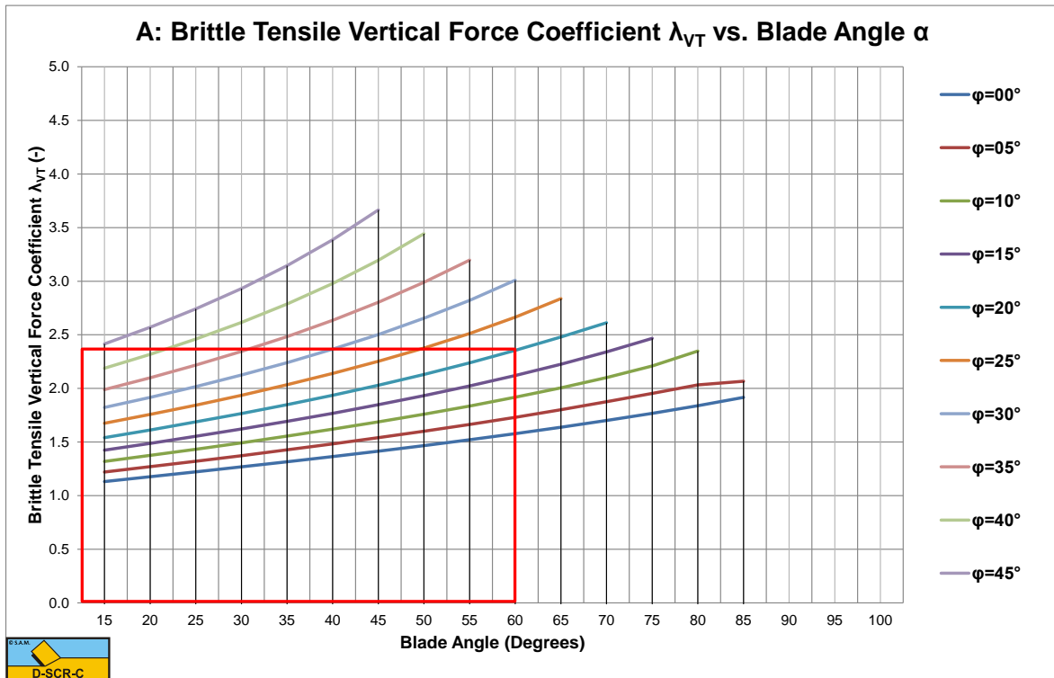
Figure 8-43: The brittle (tensile failure) vertical force coefficient \lambda_{VT} .
