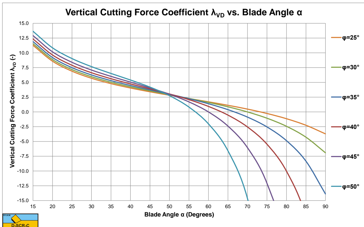
Figure B-18: The vertical cutting force coefficient \lambda_{VD} as a function of the blade angle \alpha for h_b/h_i=3 .
