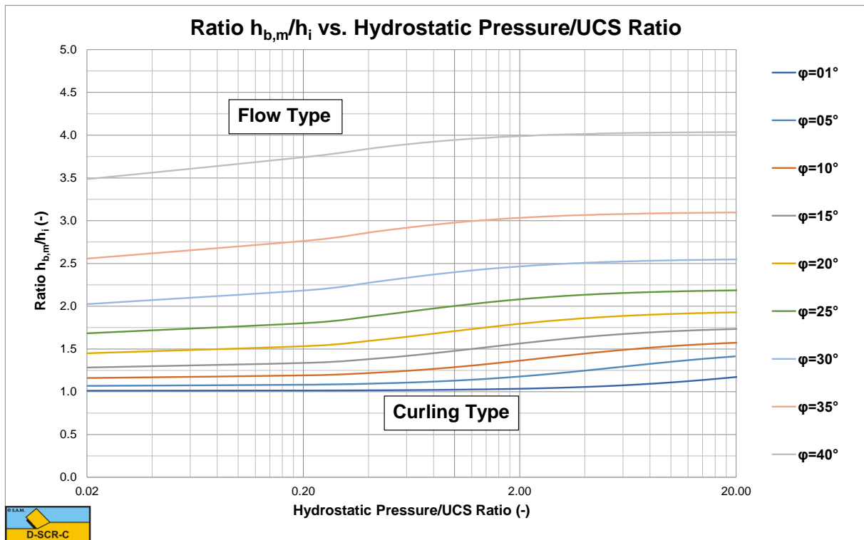
Figure X-21: The ratio h_{b,m}/h_i for a 90 degree blade.
