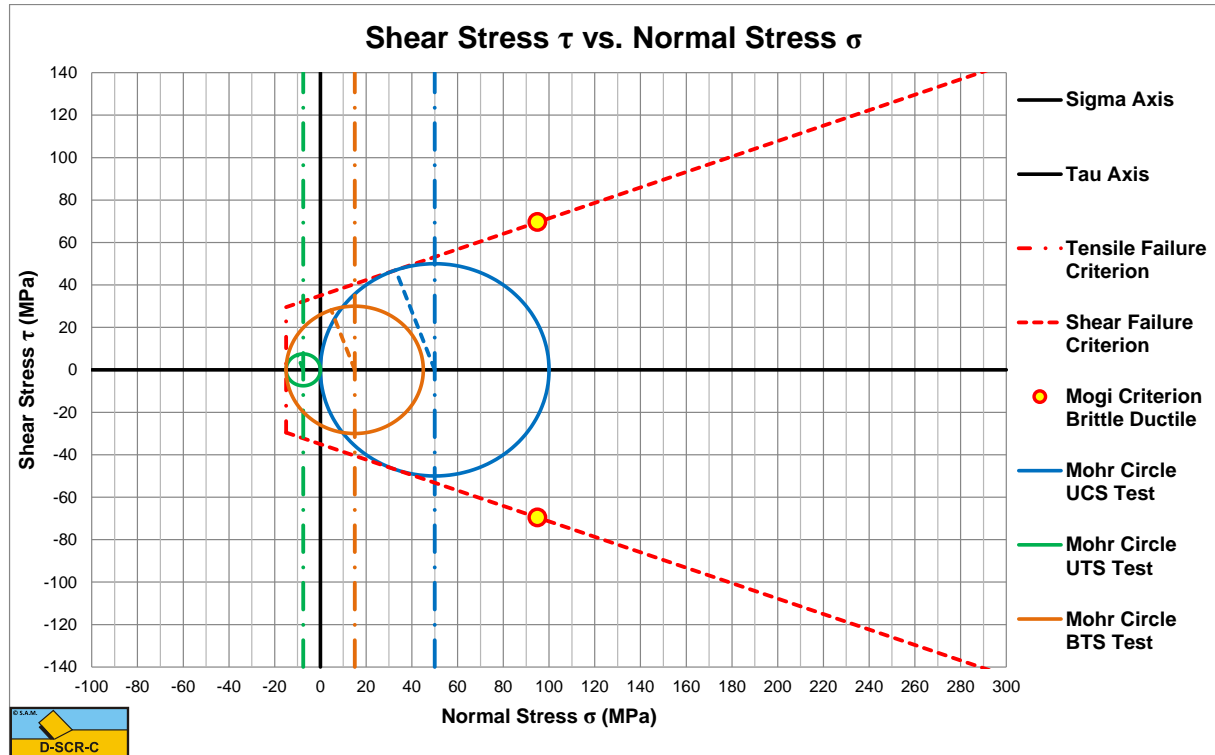
Figure 8-16: The linear failure criterion.
