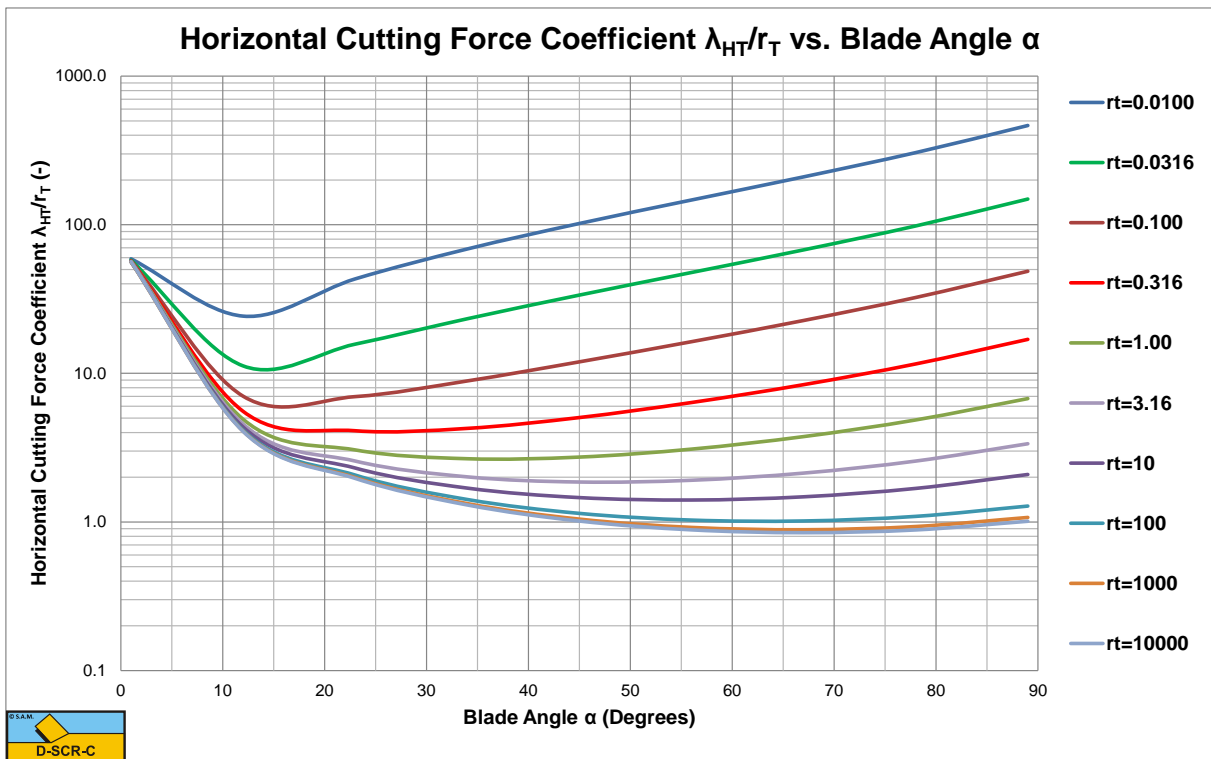
Figure V-9: The horizontal cutting force coefficient \lambda_{HT}/r_T .
