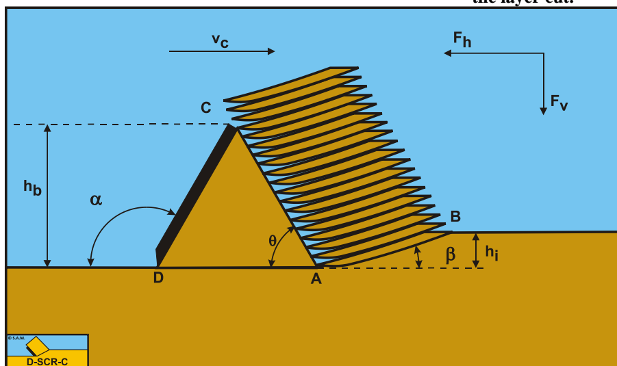
Figure 11-3: The cutting mechanism.
