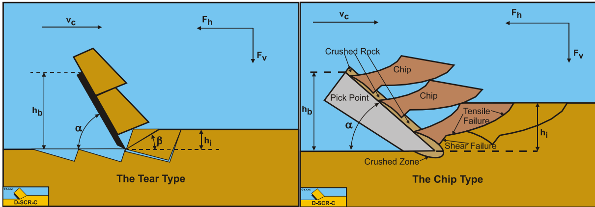
Figure 3-10: The Tear Type cutting mechanism in clay.
