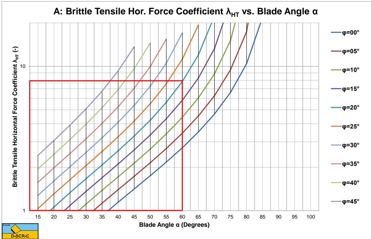
Figure W-33: The brittle (tensile failure) horizontal force coefficient \lambda_{HT} (DSCRCM, logarithmic).
