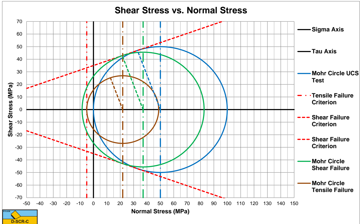
Figure 16-11: The Mohr circles with tensile strength of -5 MPa (UCS=100 MPa, \varphi=20^\circ ). Tensile Failure.
