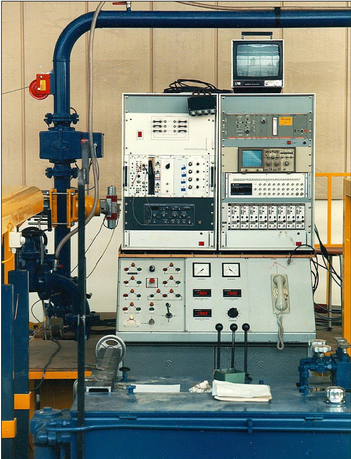
Figure 6-47: The pre-amplifiers and filters on the carriage.
