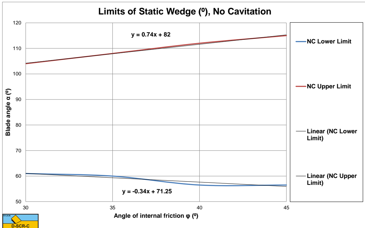
Figure 12-26: The lower and upper limit where a static wedge can exist for the non-cavitating cutting process.
