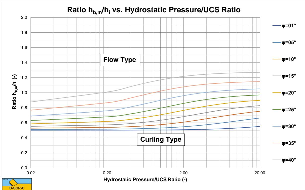
Figure X-11: The ratio h_{b,m}/h_i for a 60 degree blade.
