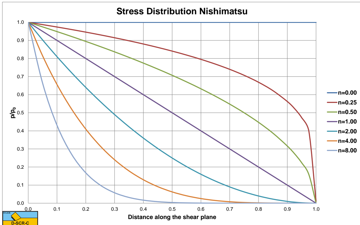
Figure 8-25: The stress distribution along the shear plane.
