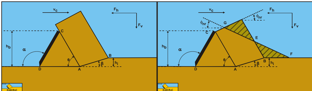
Figure 11-1: Definitions.
