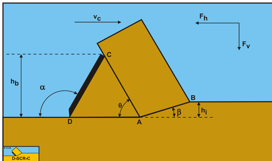
Figure 10-1: The occurrence of a wedge.
