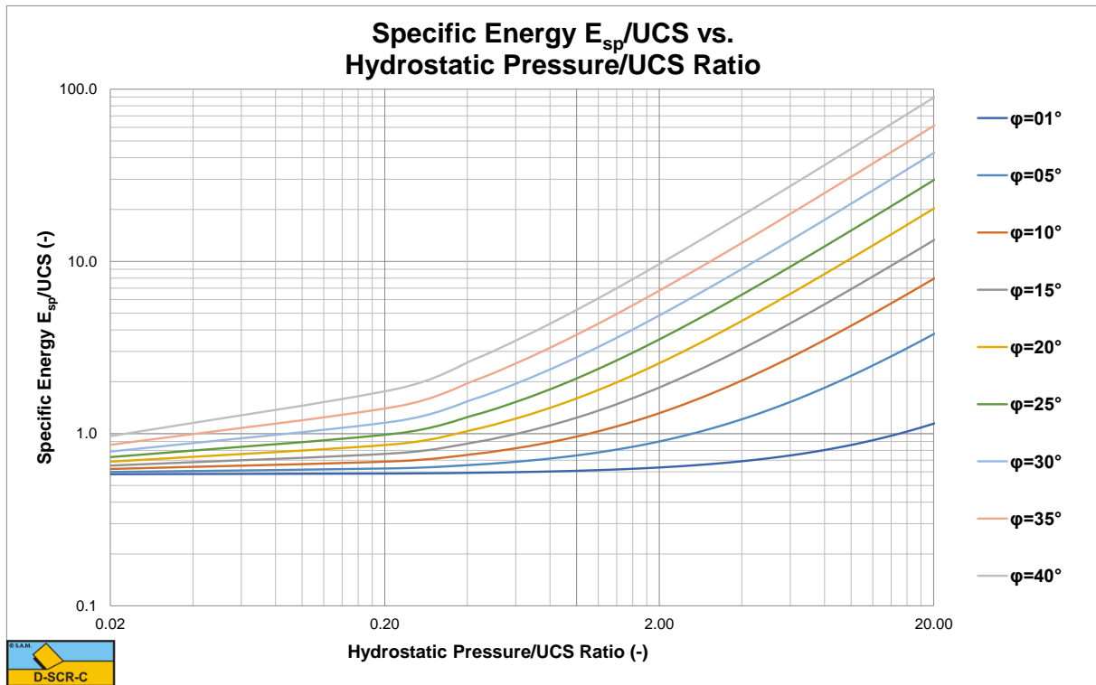
Figure X-15: The specific energy to UCS ratio for a 60 degree blade.
