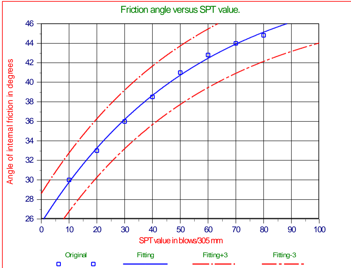
Figure 2-23: Friction angle versus SPT value (Miedema (1995)).
