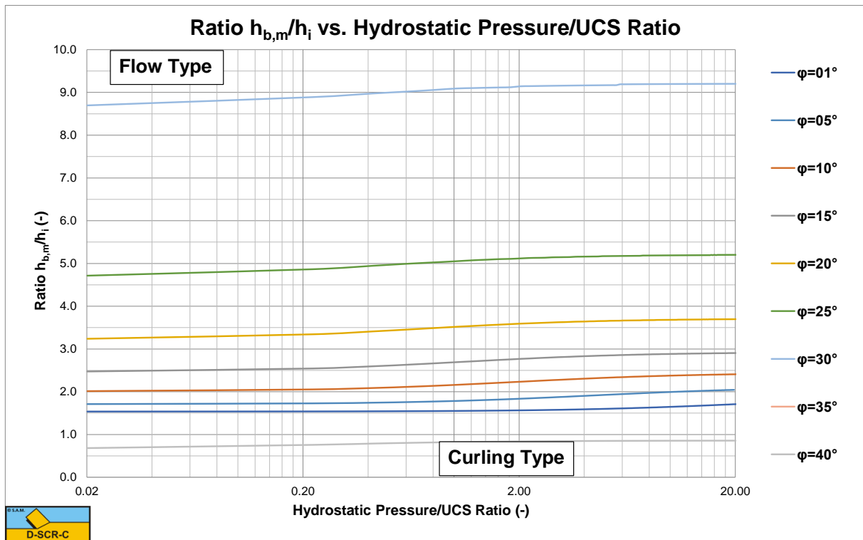
Figure X-31: The ratio h_{b,m}/h_i for a 120 degree blade.
