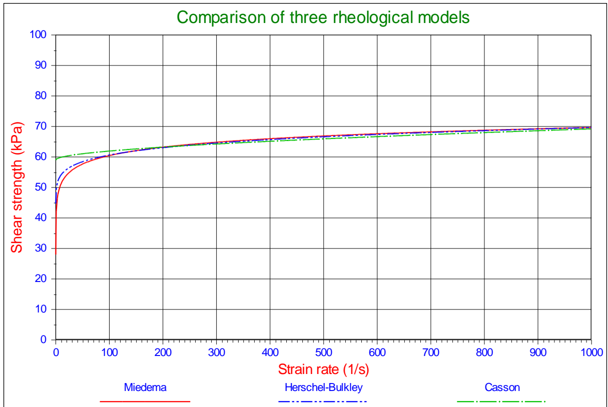
Figure 7-15: Comparison of 3 rheological models.
