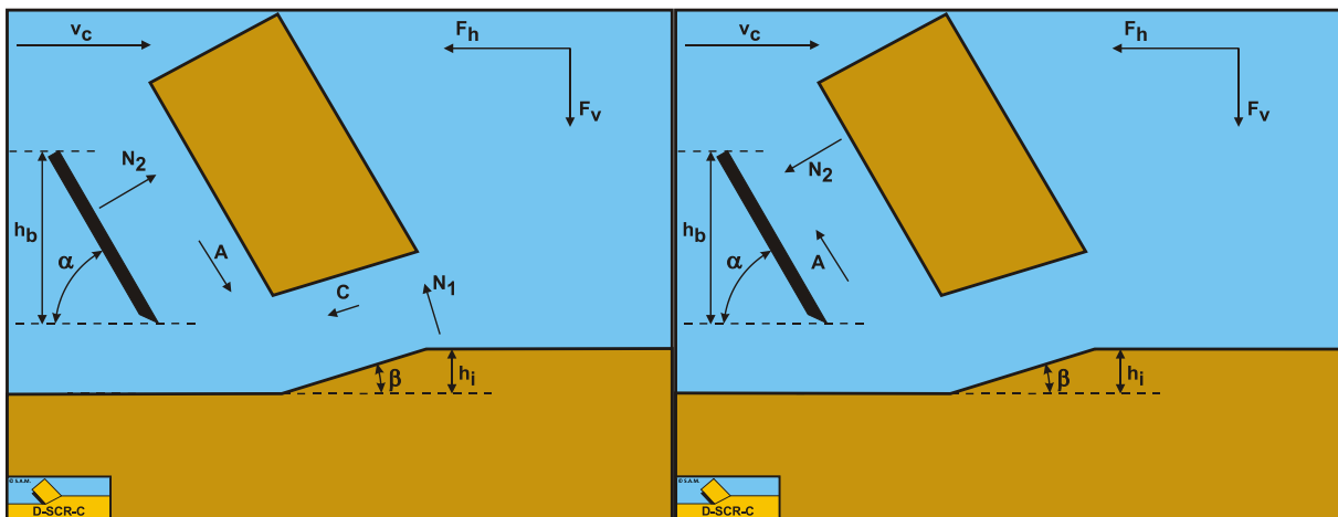
Figure 7-19: The forces on the layer cut in clay.
