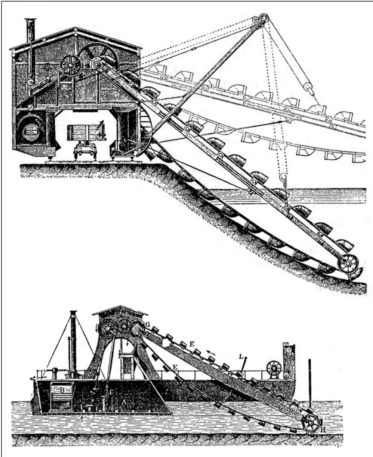
Figure Y-3: A dredge for canal works and a bucket ladder dredge (Swedish encyclopedia 1914).
