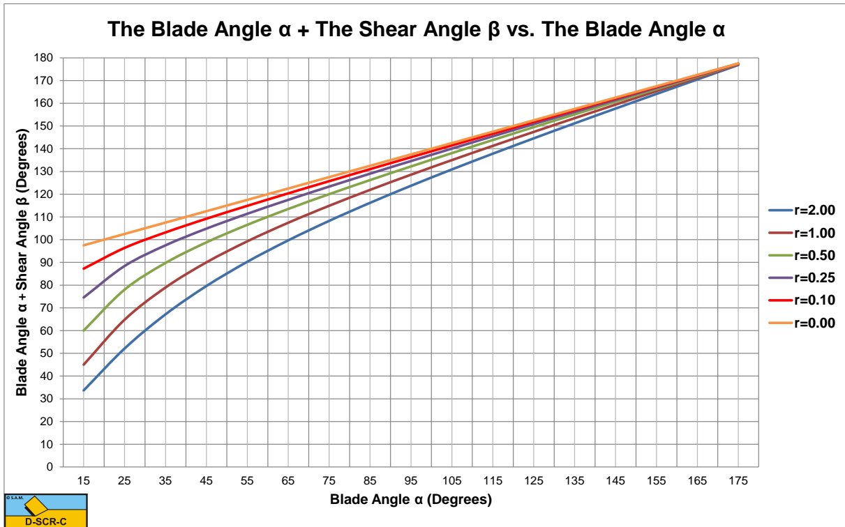
Figure 7-22: The blade angle \alpha + the shear angle \beta .
