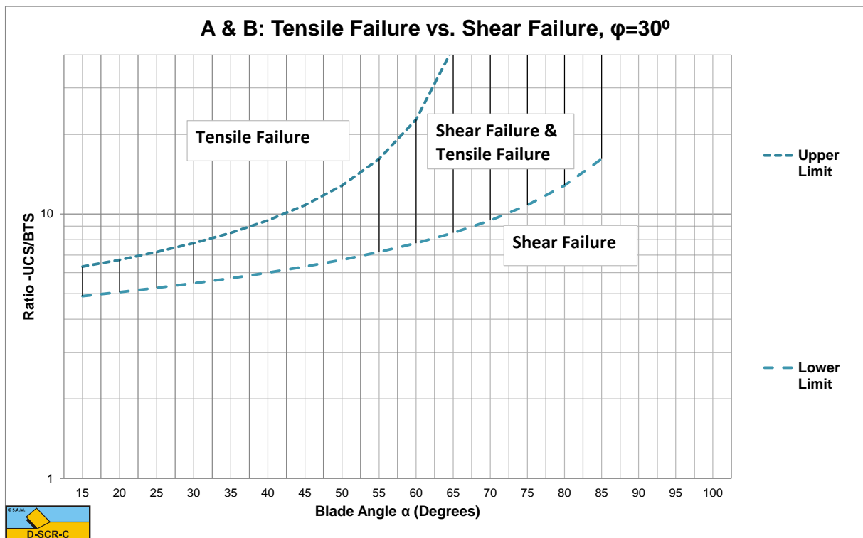
Figure W-24: The tensile/shear failure range based on UCS/BTS for \phi=30^\circ .
