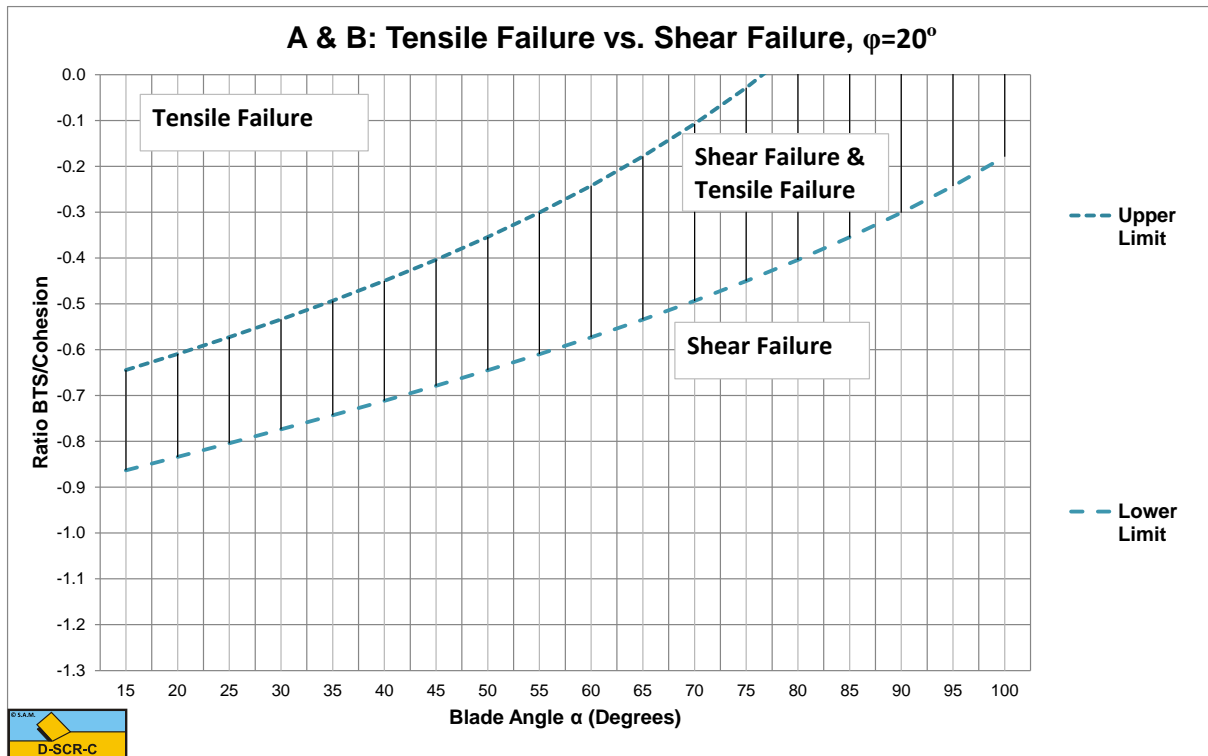
Figure W-19: The tensile/shear failure range based on BTS/Cohesion for \phi=20^\circ .
