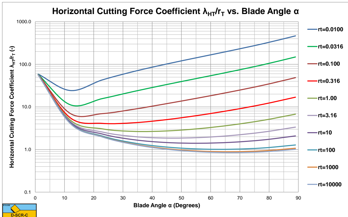
Figure 7-30: The horizontal cutting force coefficient \lambda_{HT}/r_T .
