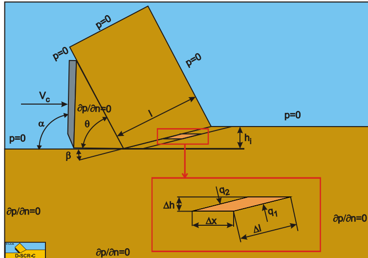
Figure 12-7: The volume balance over the shear zone.
