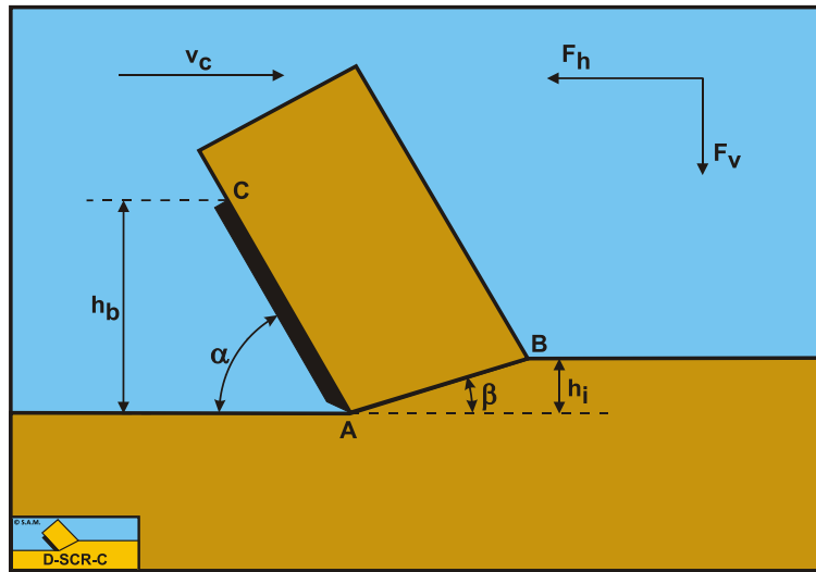
Figure 7-1: The cutting process, definitions.
