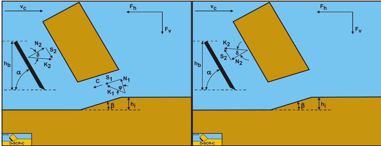
Figure 8-28: The forces on the layer cut in rock (atmospheric).
