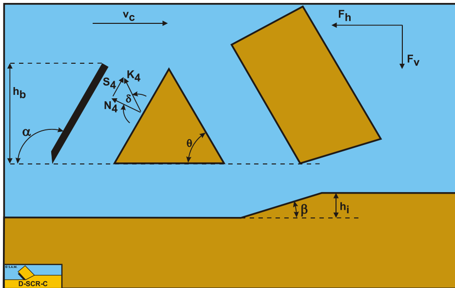
Figure 11-6: The forces on the blade when a wedge is present.
