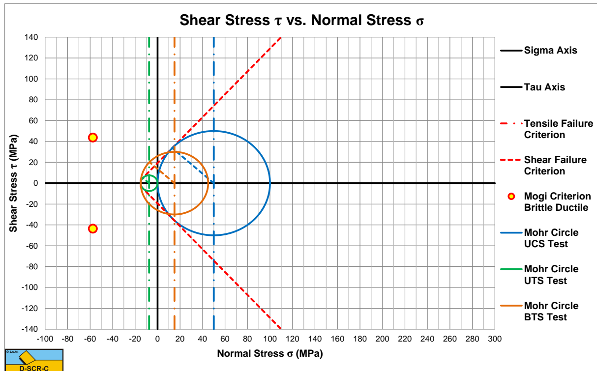
Figure 8-9: Construction of the angle of internal friction UTS-UCS based.
