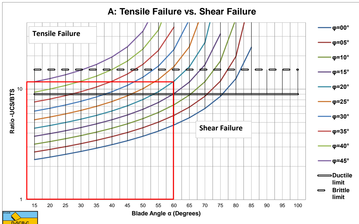
Figure 8-39: The ratio UCS/BTS, below the lines there is brittle (shear failure), above the lines it is brittle (tensile failure).
