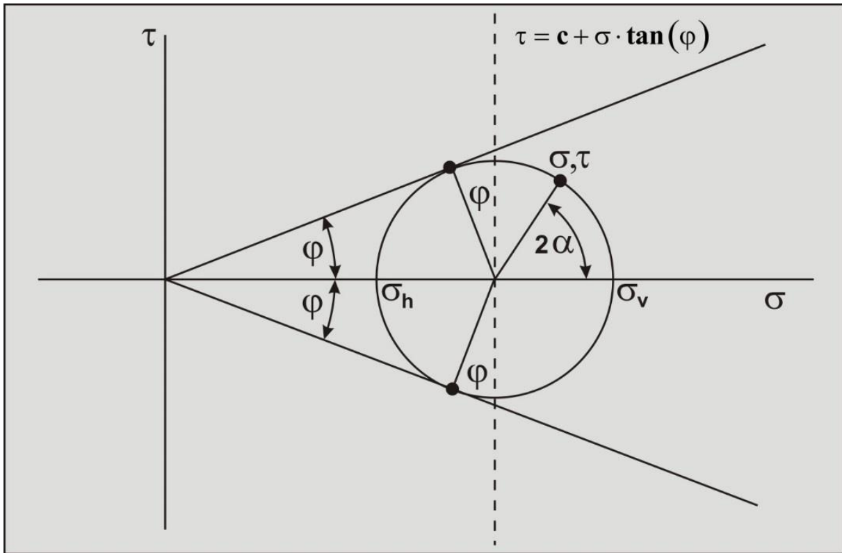
Figure 2-46: The resulting Mohr circle for cohesion less soil.
