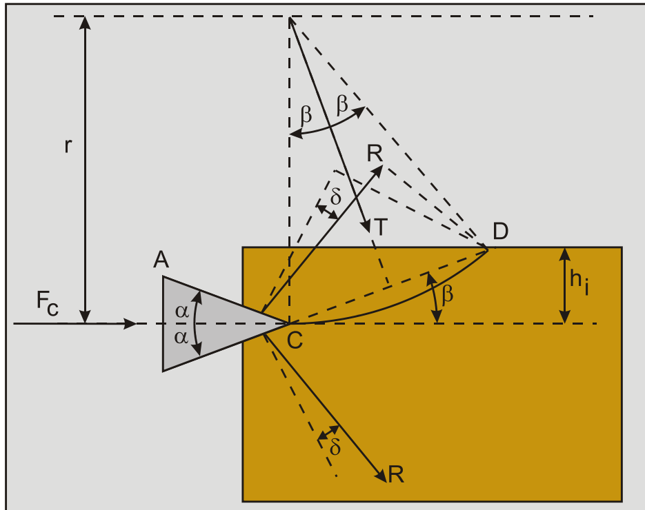
Figure 8-21: The model of Evans.
