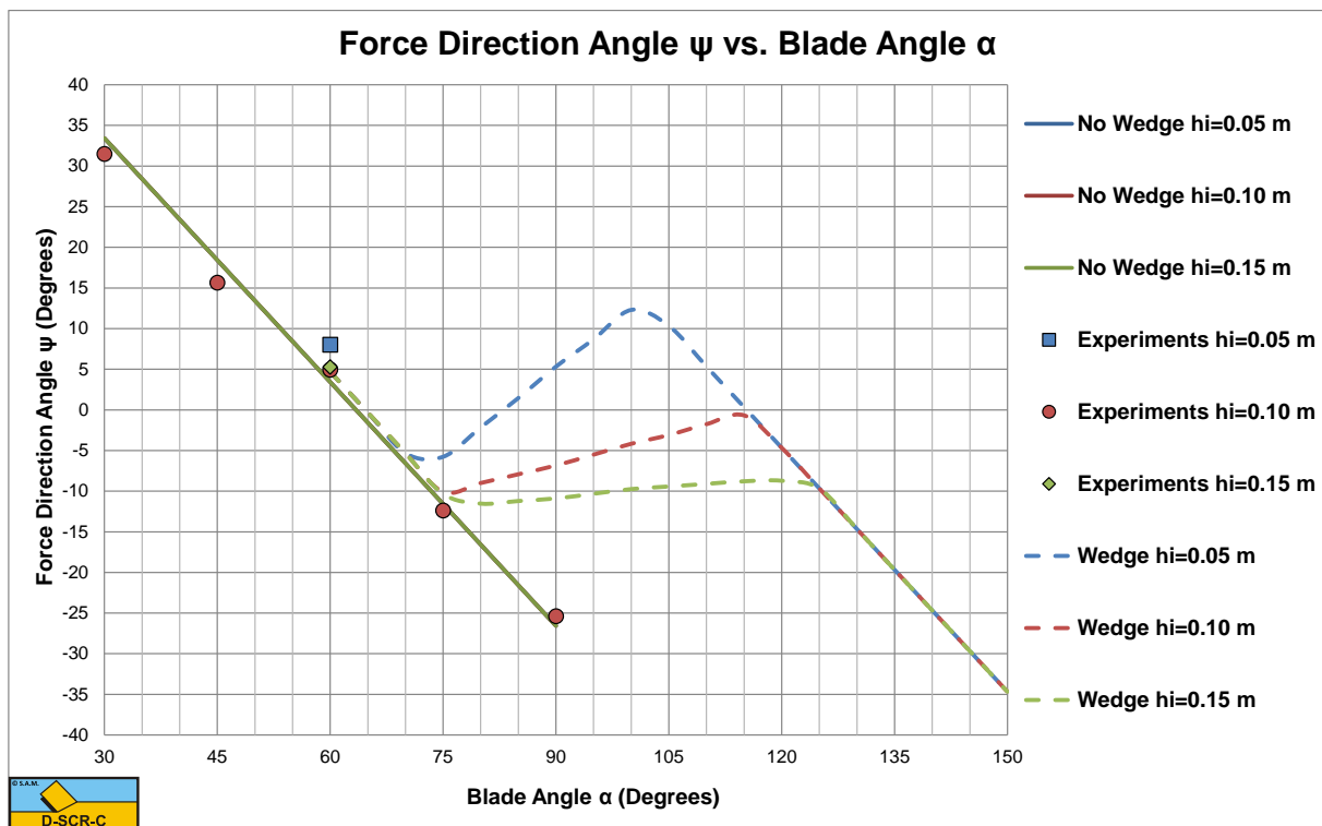
Figure 11-14: The direction of the cutting force of Hatamura & Chijiwa (1977B) versus the calculated force direction, with and without wedge.
