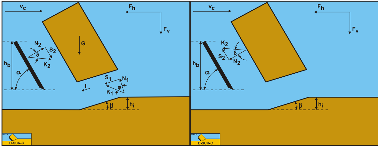
Figure 5-4: The forces on the layer cut in dry sand.
