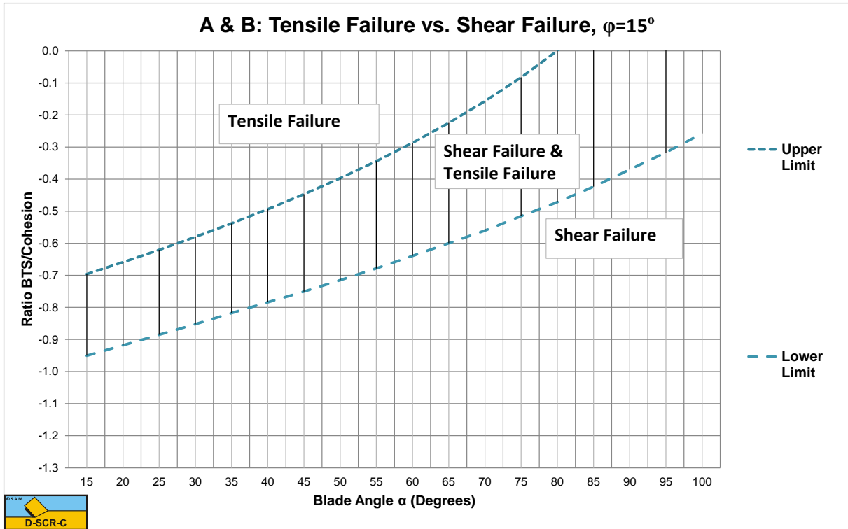
Figure W-17: The tensile/shear failure range based on BTS/Cohesion for \phi=15^\circ .
