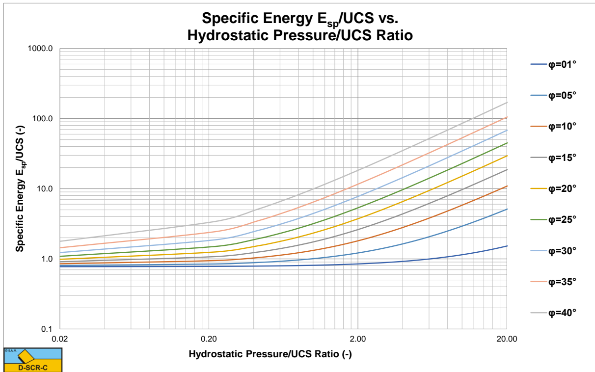
Figure X-20: The specific energy to UCS ratio for a 75 degree blade.
