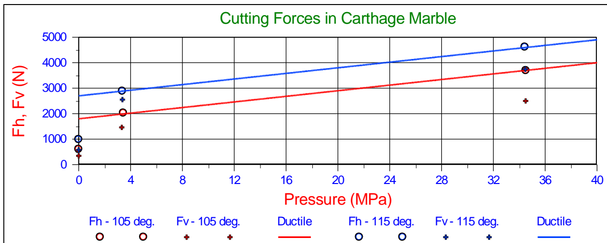
Figure 9-1: Variations of average cutting forces with hydrostatic pressure, Kaitkay & Lei (2005).
