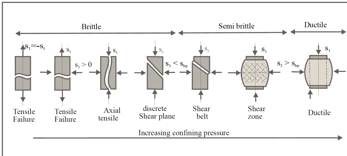
Figure 8-8: Brittle, semi brittle and ductile failure.
