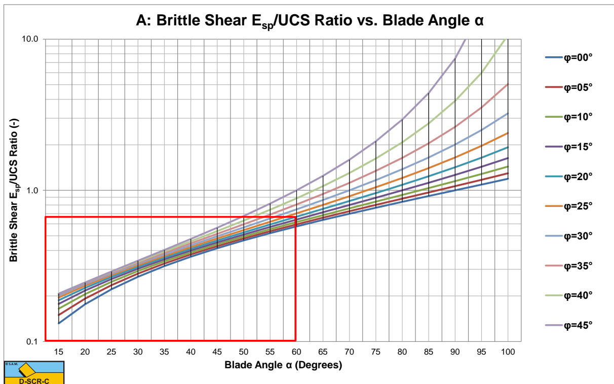
Figure W-4: The specific energy to UCS ratio.
