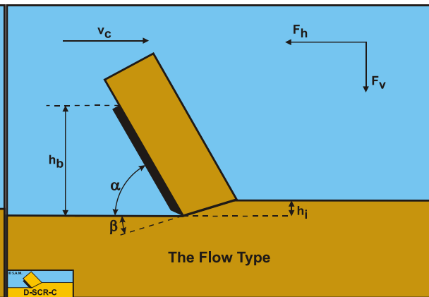
Figure 7-3: The Flow Type in clay.
