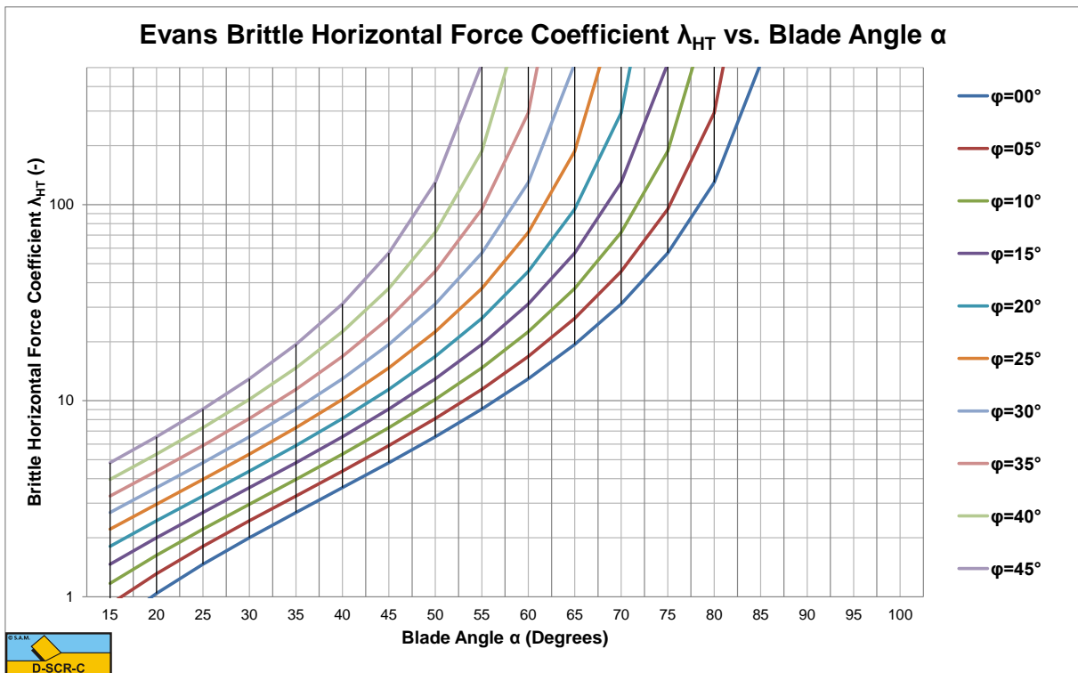
Figure W-34: The brittle (tensile failure) horizontal force coefficient \lambda_{HT} (Evans, logarithmic).
