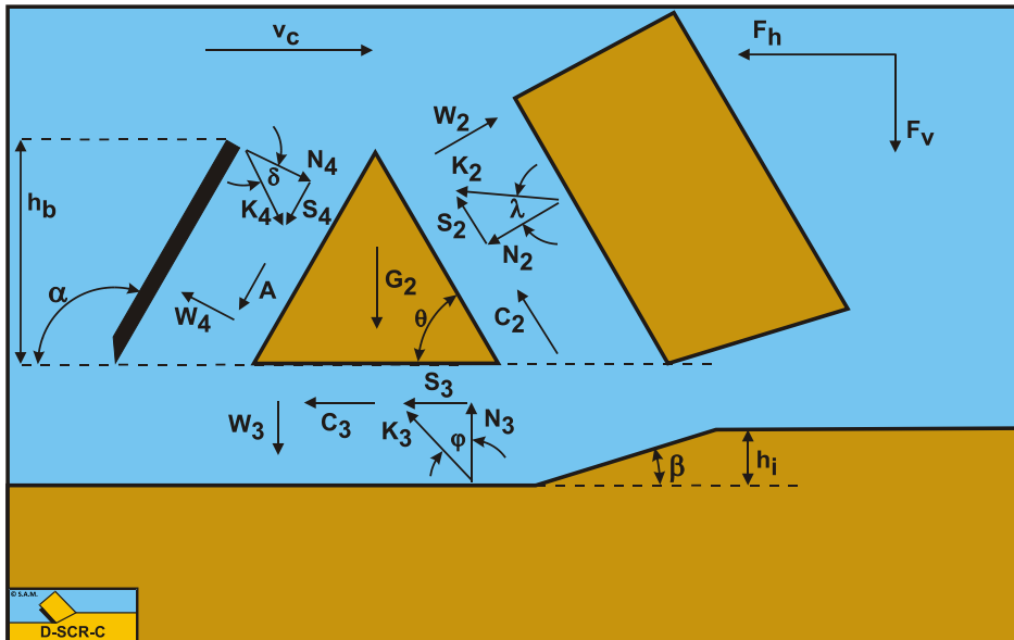
Figure 10-3: The forces on the wedge.
