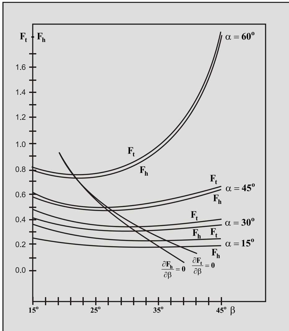
Figure 6-25: The forces F_h and F_t as function of the shear angle \beta and the blade angle \alpha .
