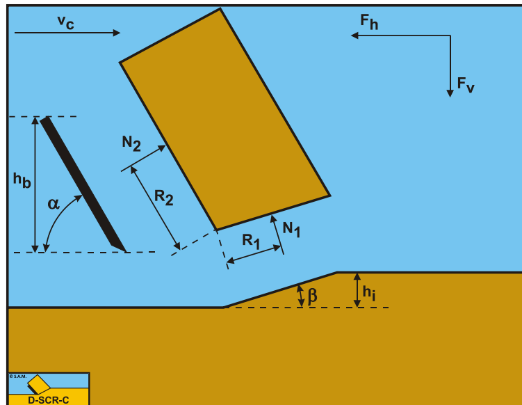
Figure 7-34: The equilibrium of moments on the layer cut in clay.
