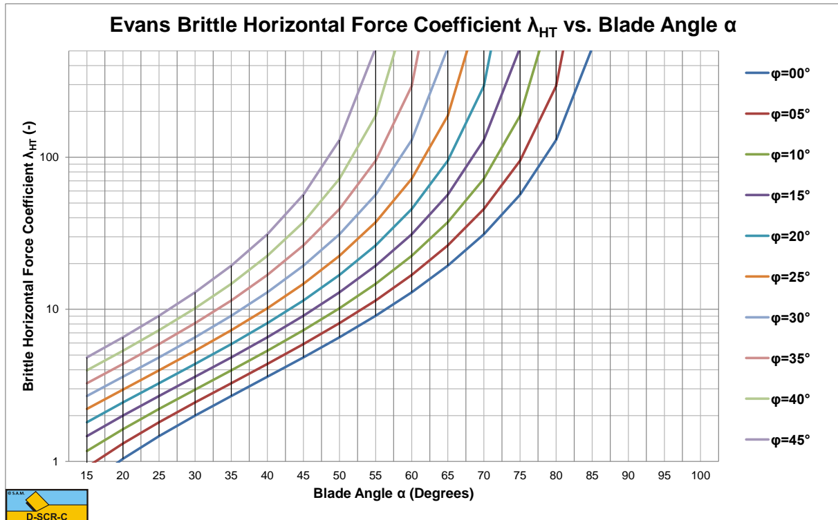
Figure 8-20: The brittle-tear horizontal force coefficient \lambda_{HT} (Evans).
