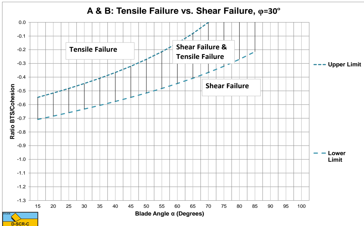
Figure W-23: The tensile/shear failure range based on BTS/Cohesion for \phi=30^\circ .
