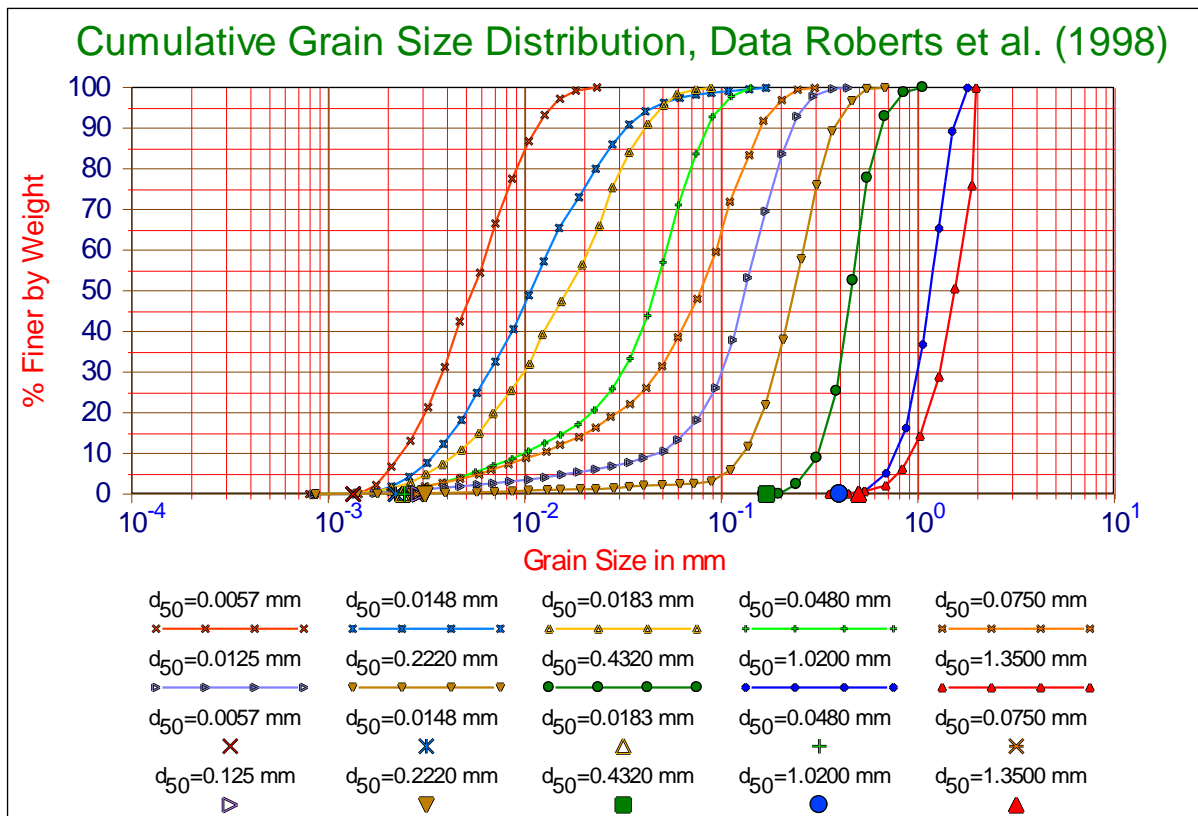
Figure 2-18: The particle size distributions of the sands used by Roberts et al. (1998).
