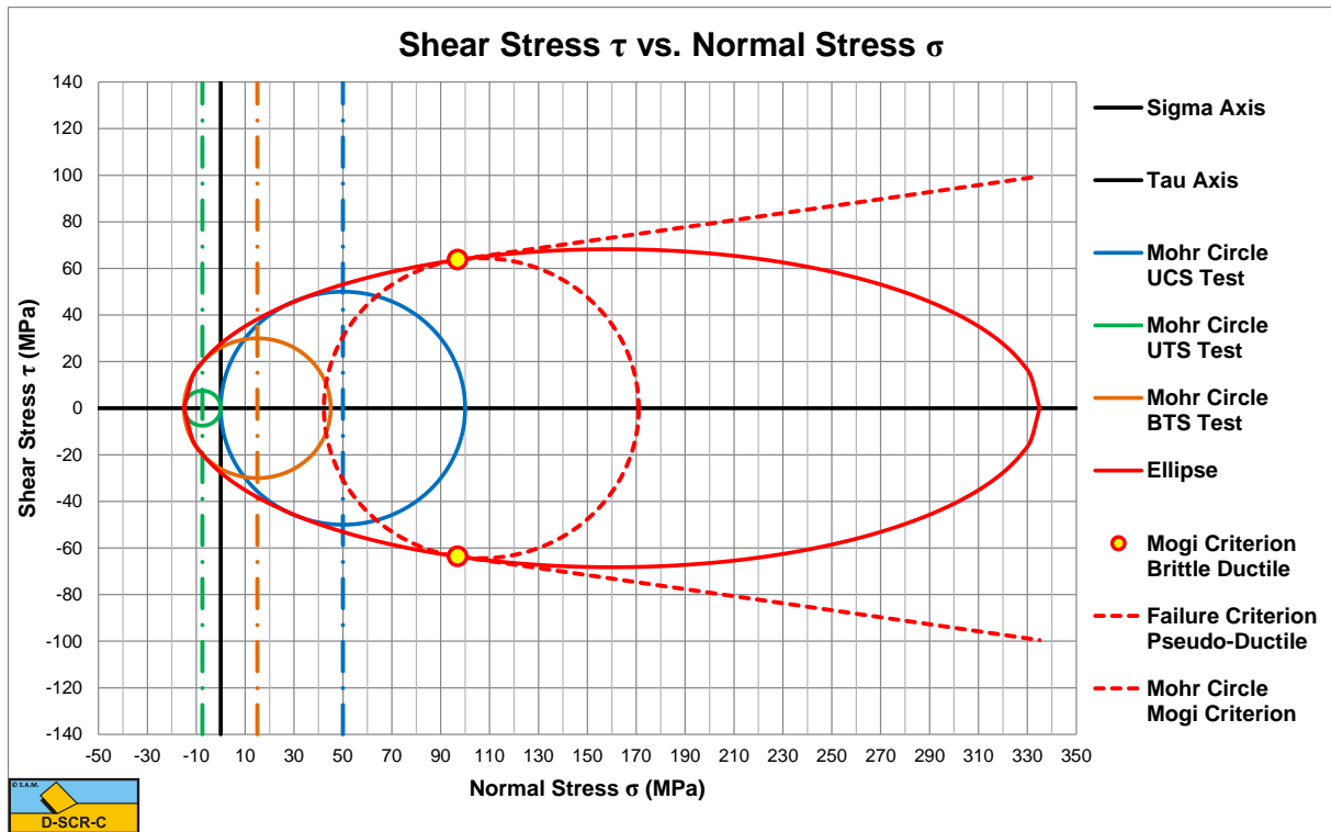
Figure 8-6: Resulting failure curve for Mancos Shale like rocks.
