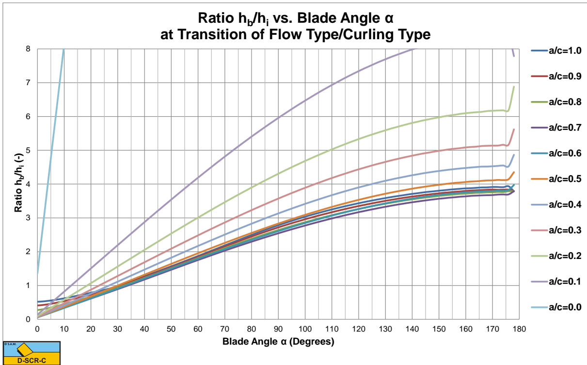
Figure V-12: The ratio h_b/h_i at the transition Flow Type/Curling Type.
