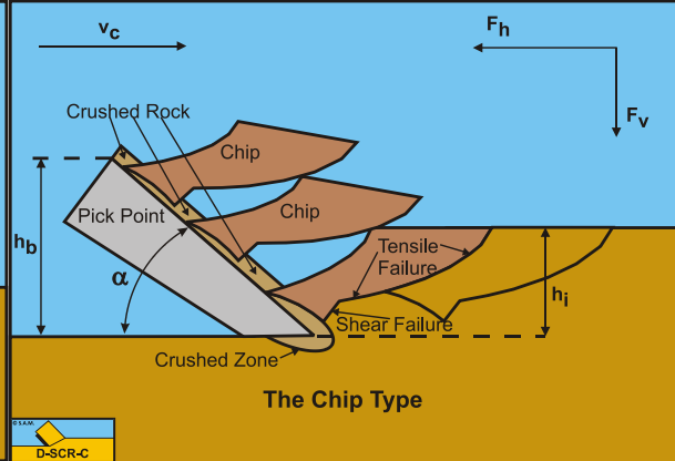
Figure 9-14: The Chip Type cutting mechanism in rock under hyperbaric conditions.
