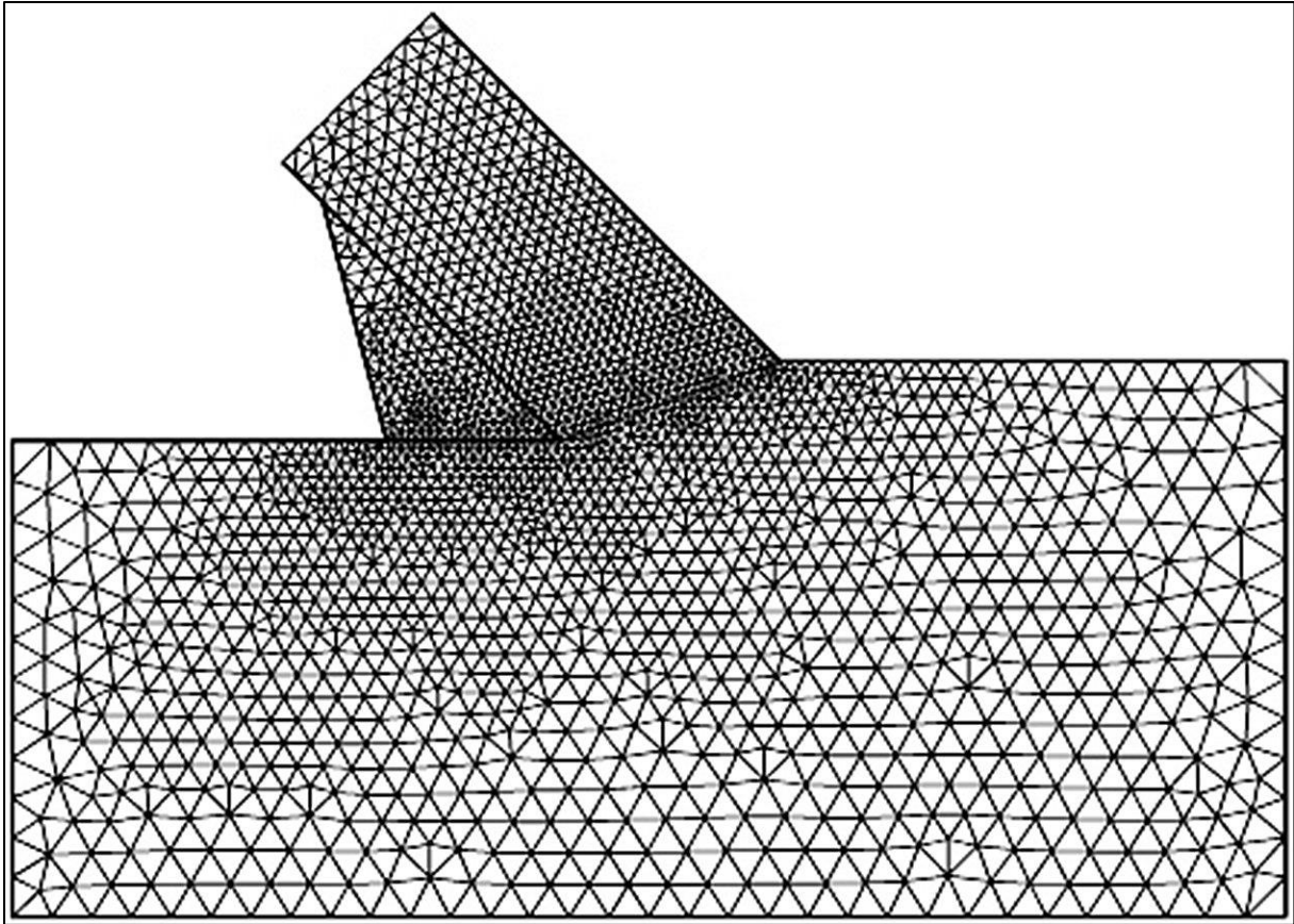
Figure 12-12: The coarse mesh.
