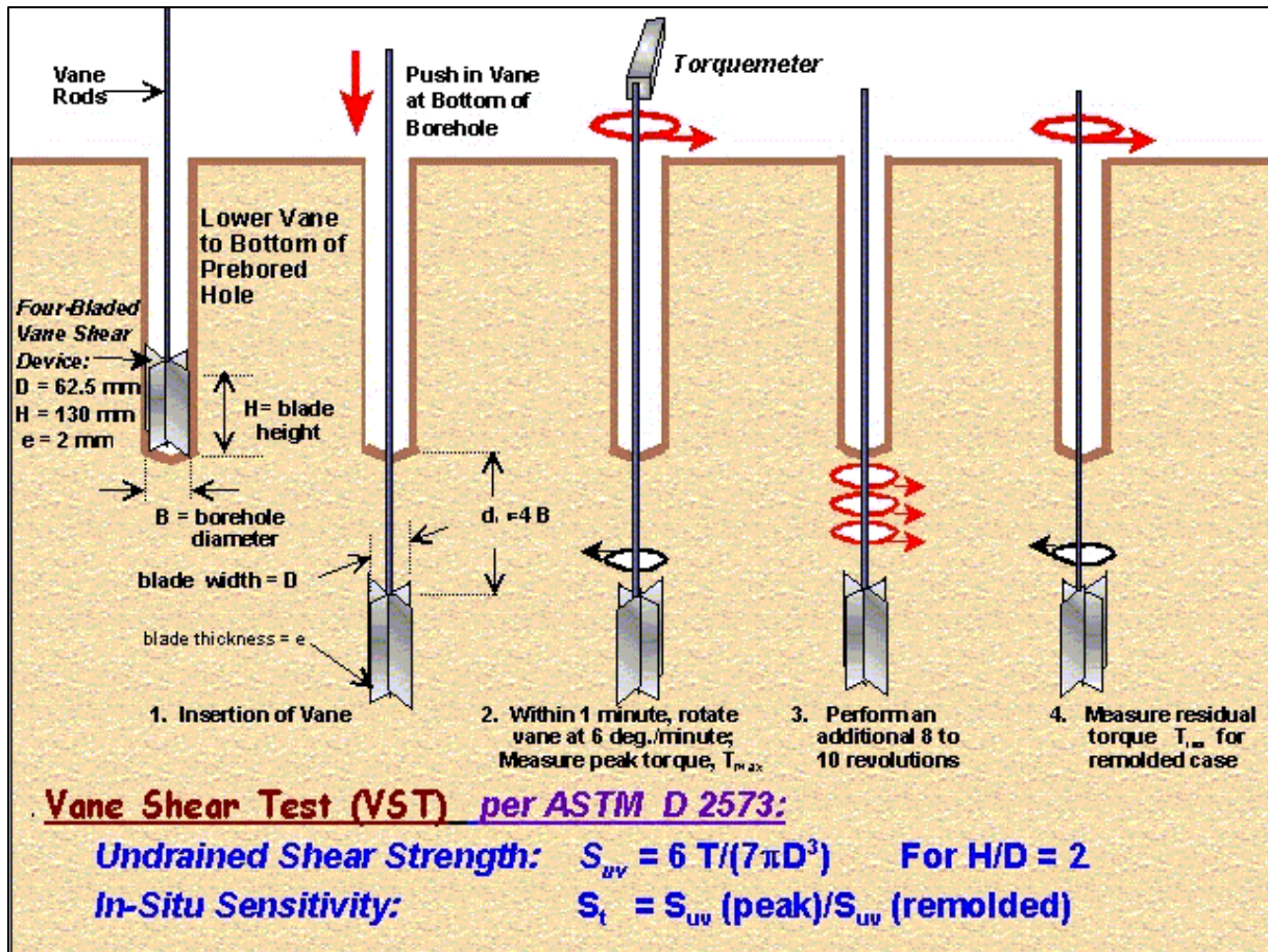
Figure 2-38: The vane shear test (English.geocpt.es).
