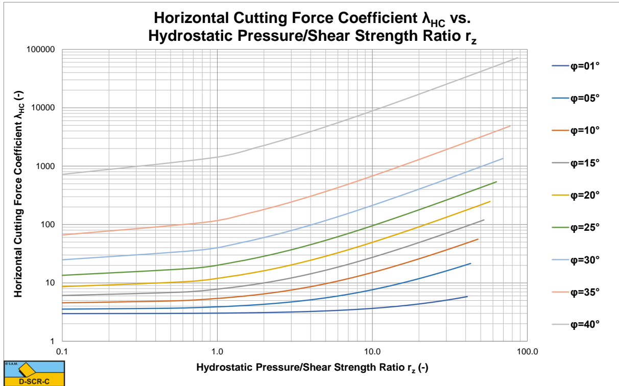
Figure 9-26: The horizontal cutting force coefficient \lambda_{HC} for a 110 degree blade.
