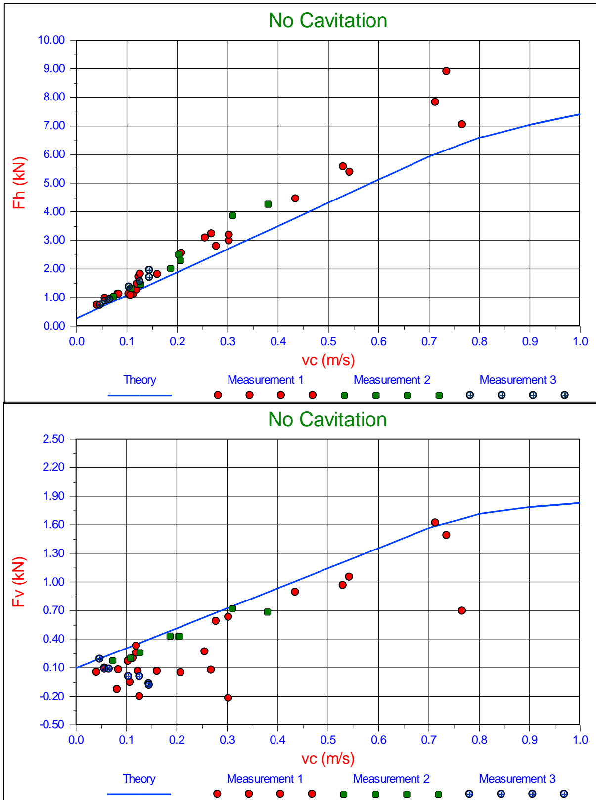
Figure M-25: \alpha=45^\circ , h_i=141 mm, h_b=141 mm.
