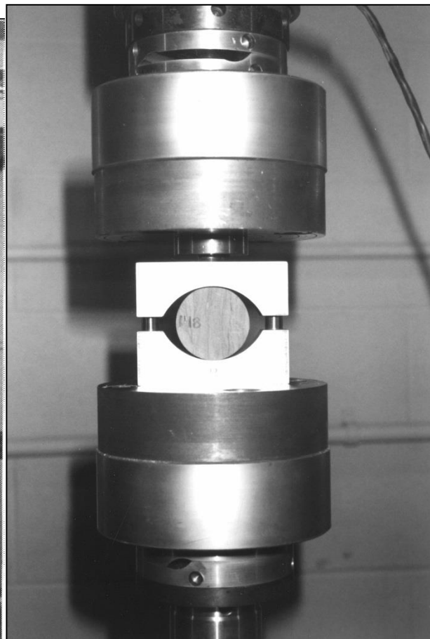
Figure 2-42: BTS zoomed.
