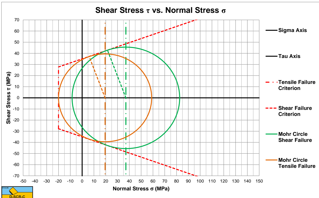
Figure 8-52: Mohr circles tensile strength -20 MPa.
