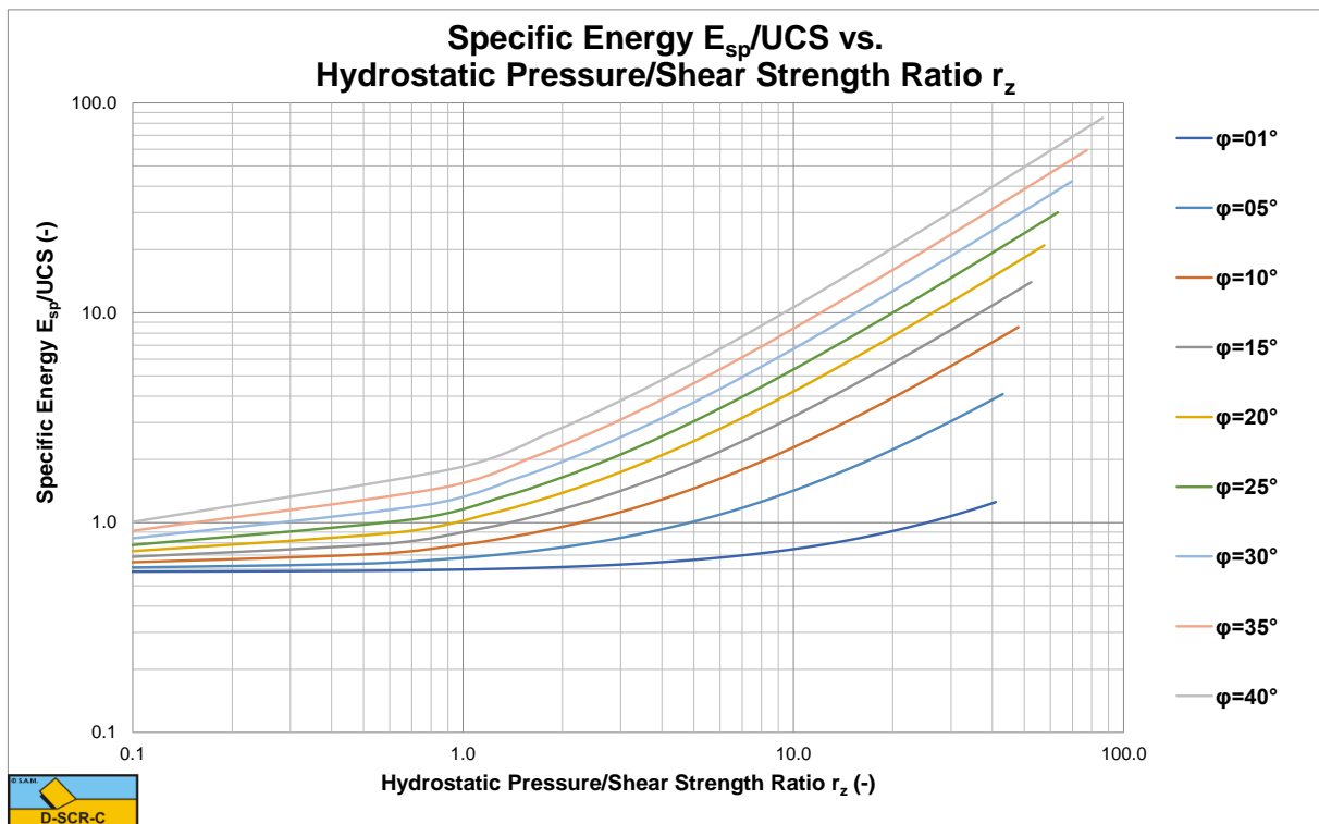
Figure 9-12: The E_{sp}/UCS ratio, for a 60 degree blade, h_b/h_i=1 .
