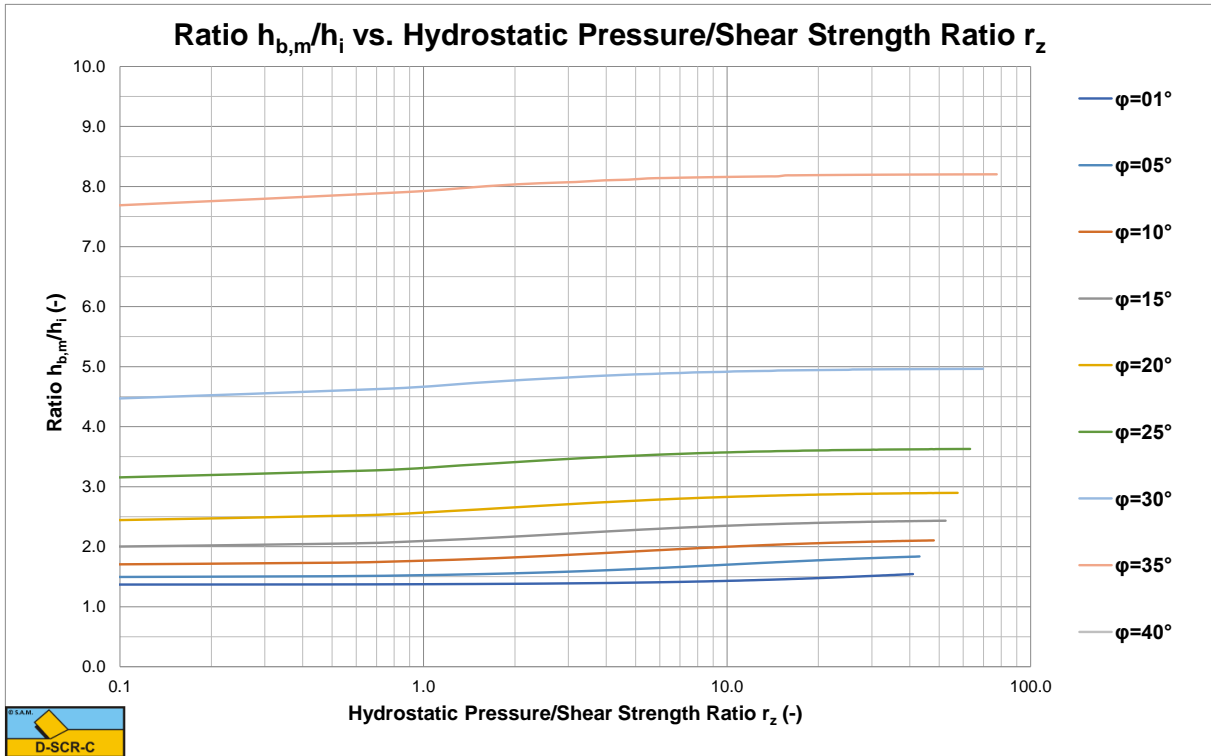
Figure 9-24: The ratio h_{b,m}/h_i for a 110 degree blade.
