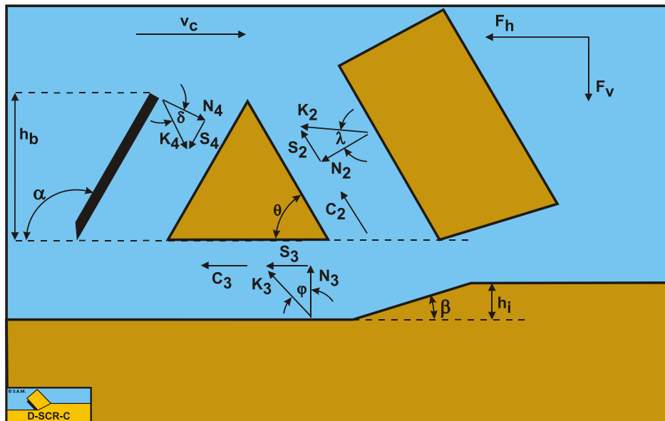
Figure 14-3: The forces on the wedge.
