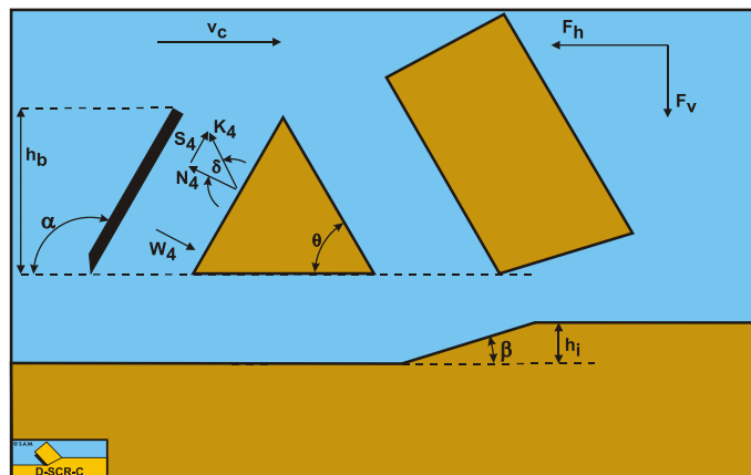
Figure 12-6: The forces on the blade in saturated sand with a wedge.
