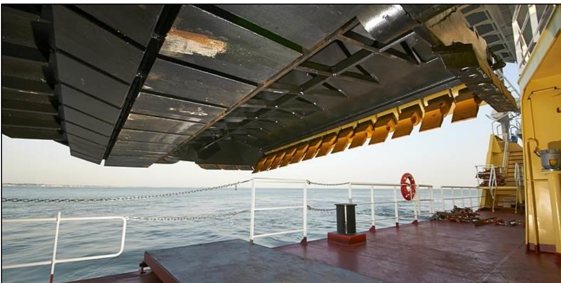
Figure Y-25: Drag head (Damen Dredging).
