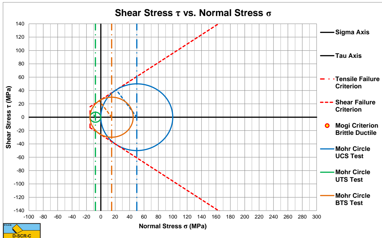
Figure 8-10: Construction of the angle of internal friction BTS-UCS based.
