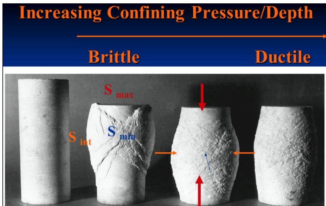
Figure 2-29: Brittle-ductile failure of marble (M.S. Patterson, Australian National University).
