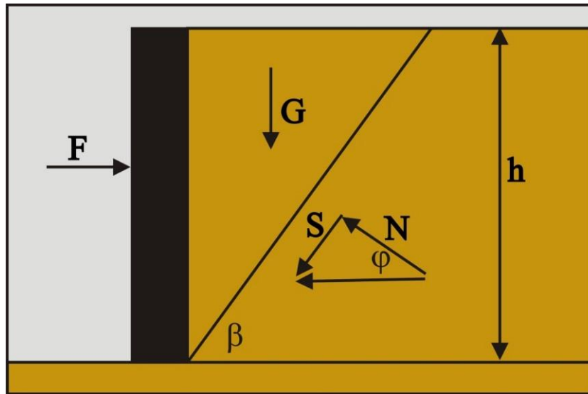
Figure 2-54: Passive soil failure.
