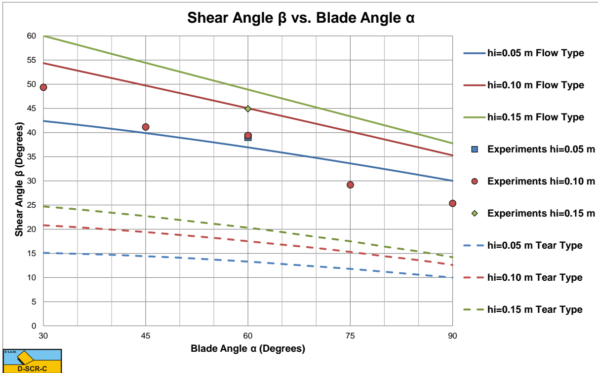
Figure 7-44: The shear angles measured and calculated.
