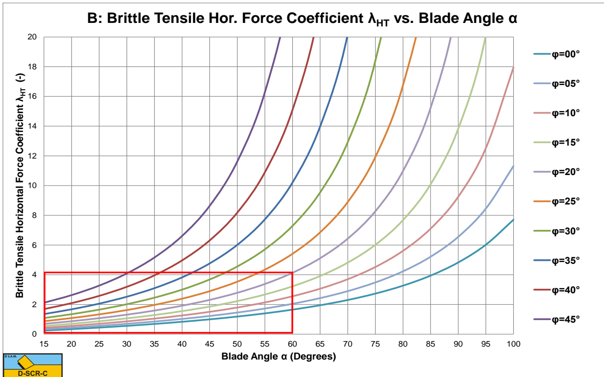
Figure W-2: The brittle (shear failure) horizontal force coefficient \lambda_{HF} .
