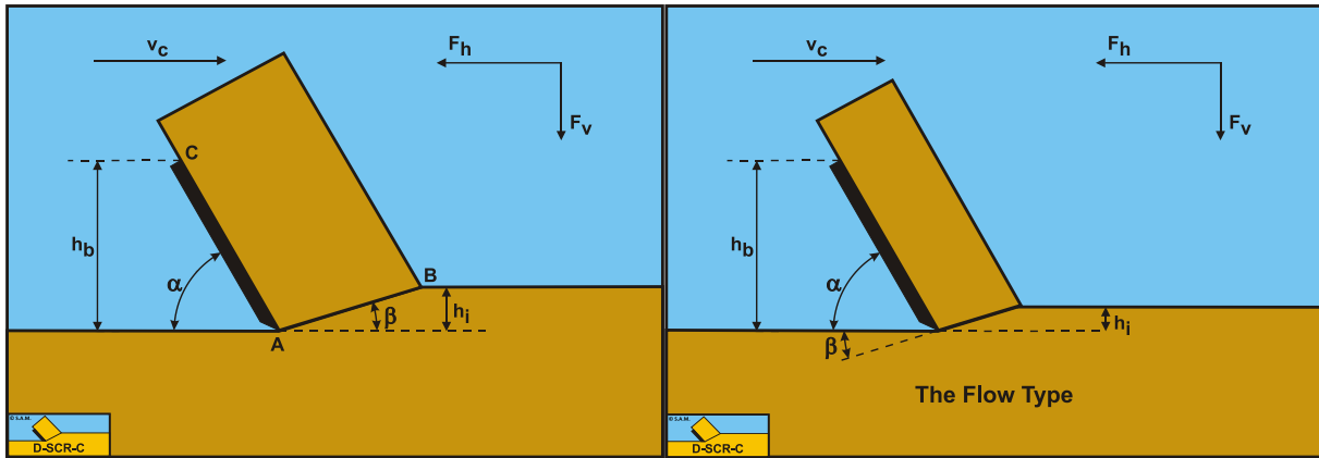
Figure 9-4: The definitions of the cutting process.
