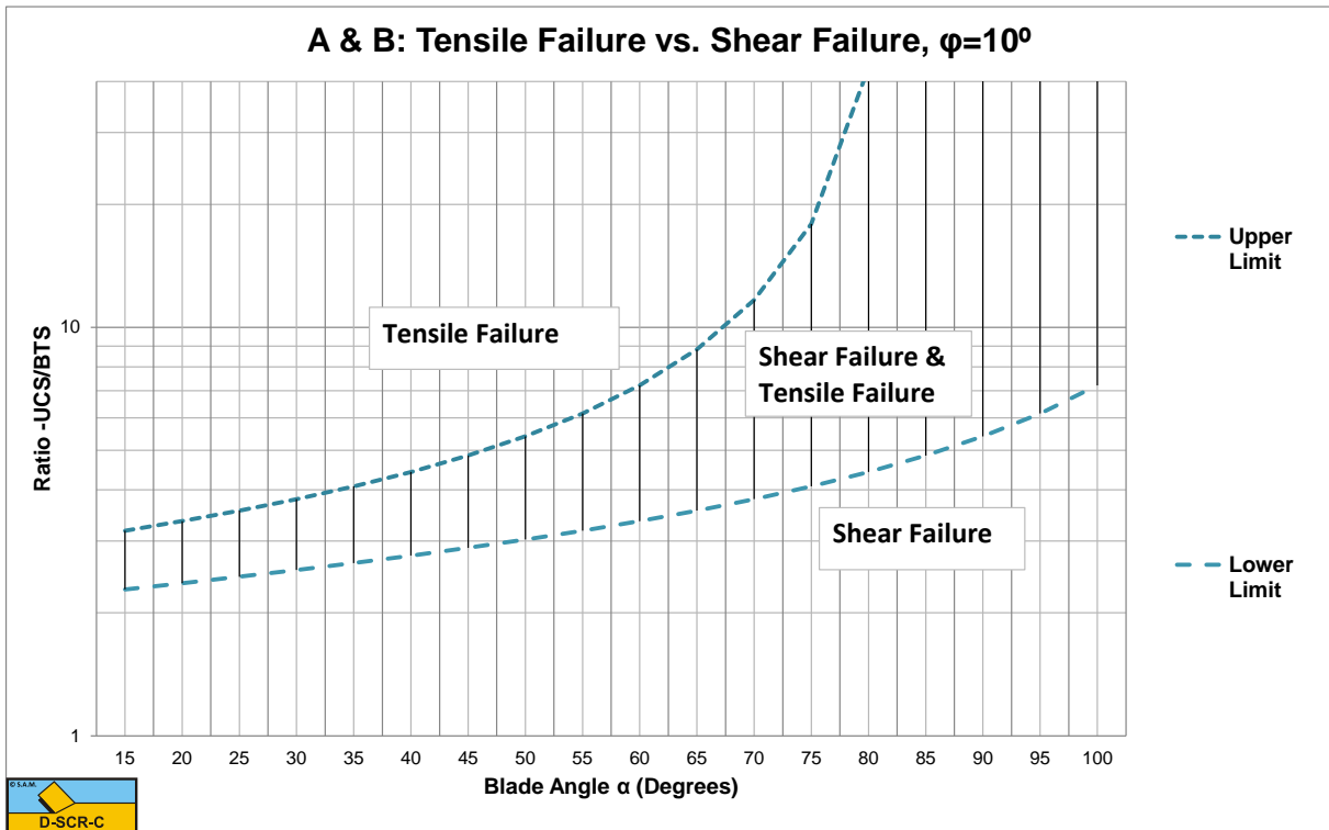
Figure W-16: The tensile/shear failure range based on UCS/BTS for \phi=10^\circ .
