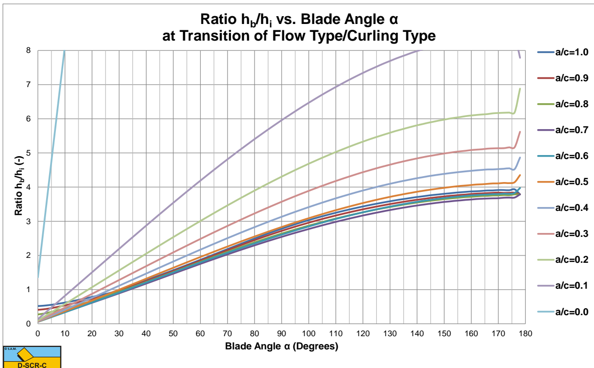
Figure 7-38: The ratio h_b/h_i at the transition Flow Type/Curling Type.
