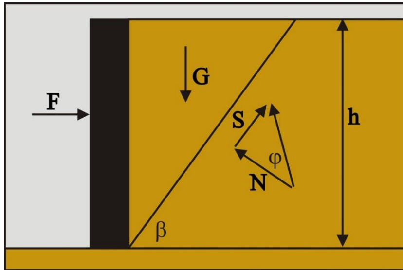
Figure 2-51: Active soil failure.
