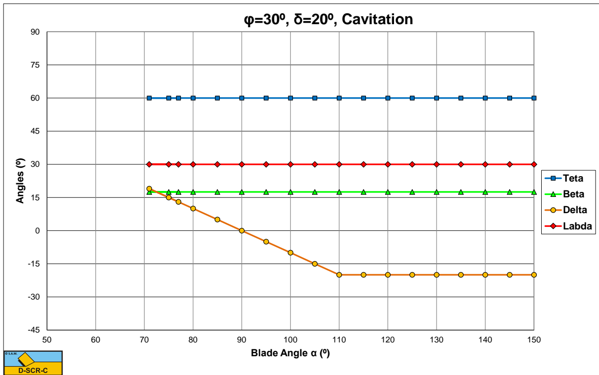
Figure Q-1: Cavitating, the angles \theta , \beta , \delta_m and \lambda as a function of the blade angle \alpha for \varphi=30^\circ and \delta=20^\circ .
