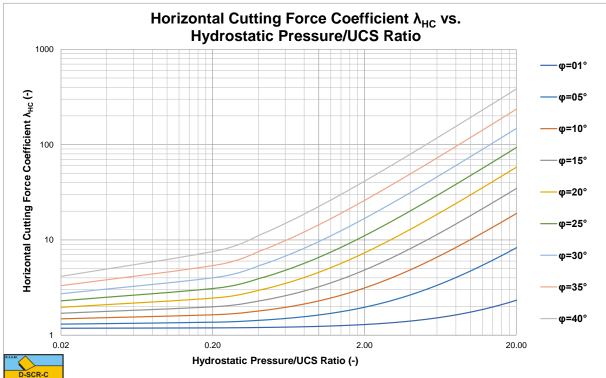
Figure X-13: The horizontal cutting force coefficient \lambda_{HC} for a 60 degree blade.
