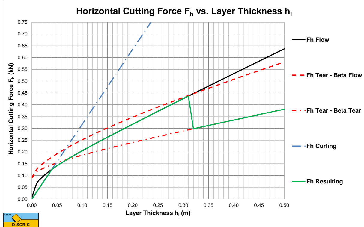
Figure 7-39: Horizontal force; cohesion c=1 kPa, adhesion a=1 kPa, tensile strength \sigma_T=-0.3 kPa, blade height h_b=0.1 m, blade angle \alpha=55^\circ
