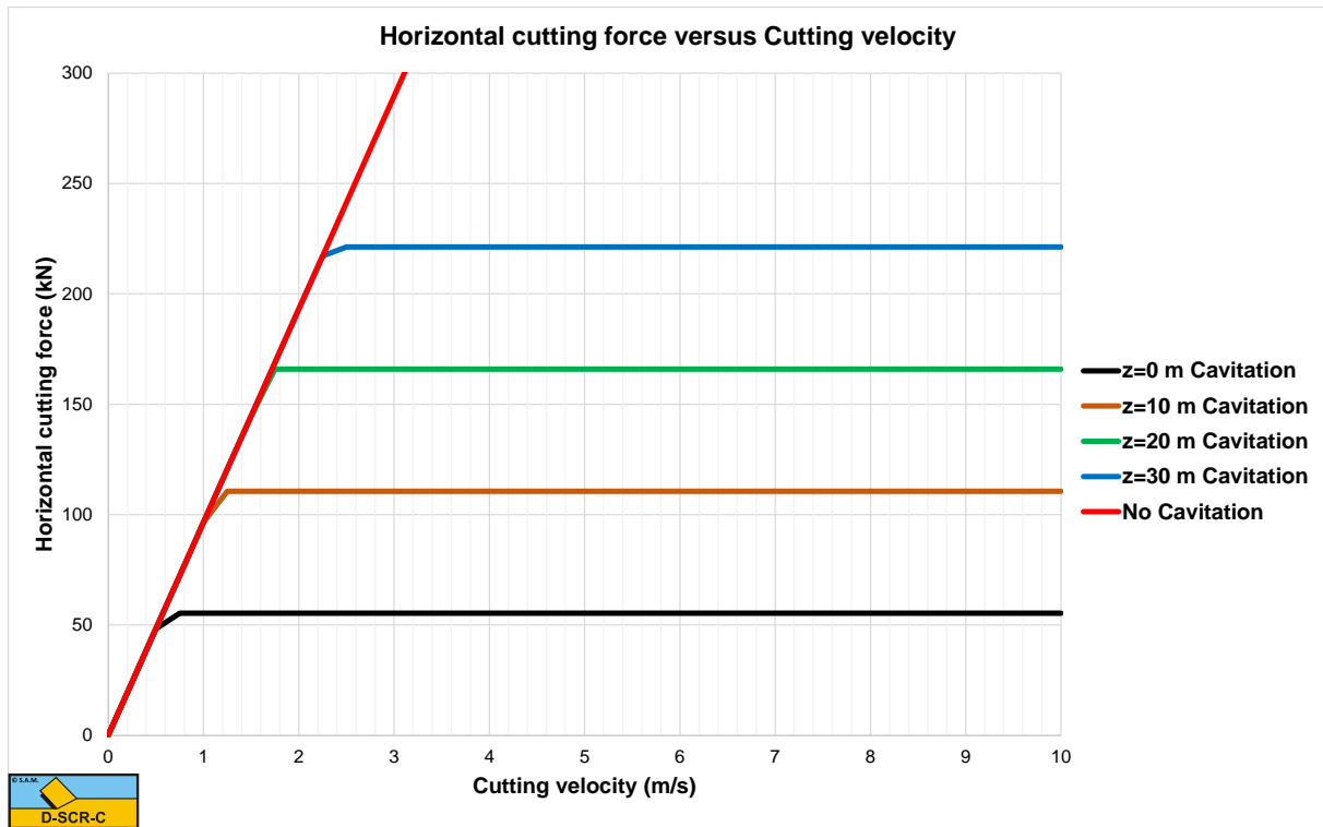
Figure 16-4: The horizontal cutting forces.
