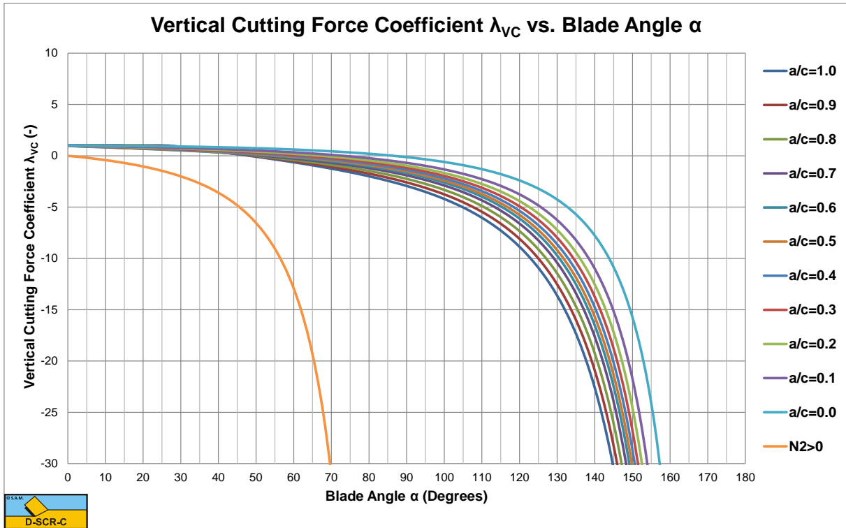
Figure 7-37: The vertical cutting force coefficient \lambda_{Vc} .
