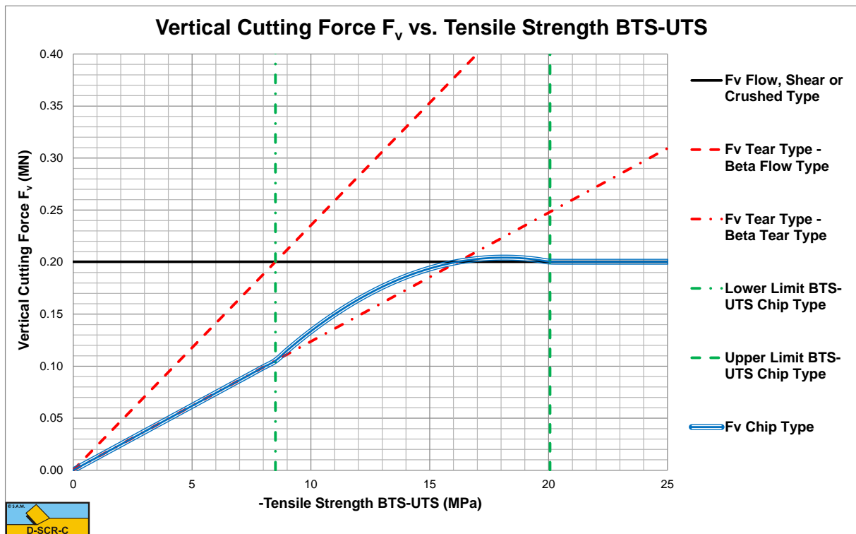
Figure 8-50: Vertical cutting force: \alpha=60^\circ , UCS=100 MPa, \phi=20^\circ , h_i=0.1 m & w=0.1 m.
