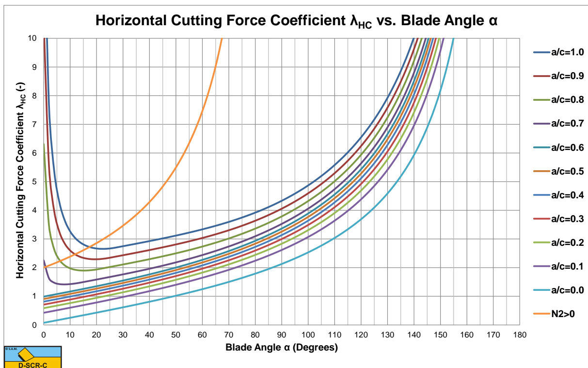
Figure 7-36: The horizontal cutting force coefficient \lambda_{HC} .
