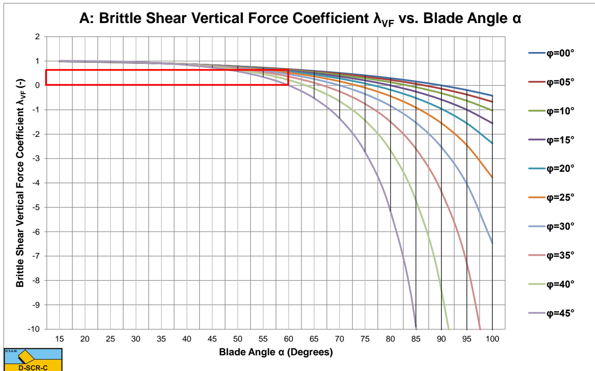
Figure W-3: The brittle (shear failure) vertical force coefficient \lambda_{VF} .
