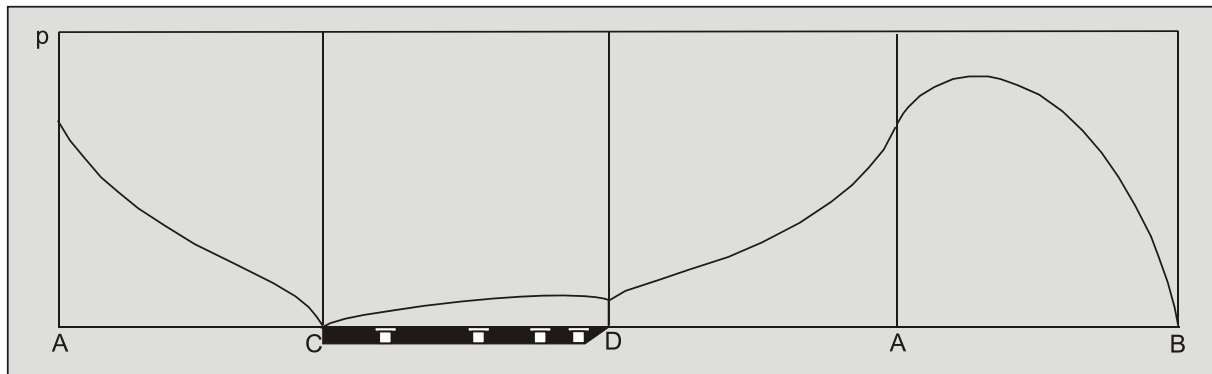
Figure S-17: Pore pressure distribution on the shear plane A-B, the bottom of the wedge A-D, the blade D-C and the front of the wedge A-C.
