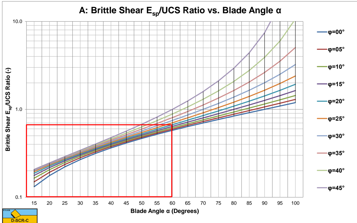
Figure 8-33: The specific energy E_{sp} to UCS ratio.
