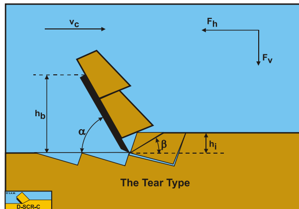
Figure 7-4: The Tear Type in clay.
