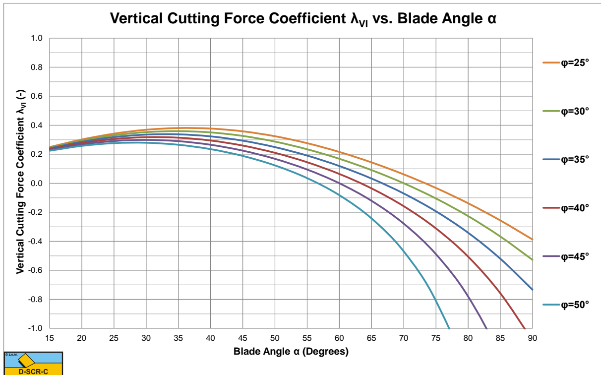
Figure 5-17: The vertical cutting force coefficient \lambda_{VI} .
