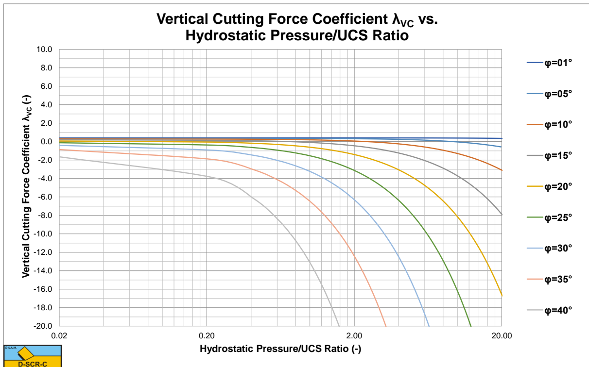
Figure X-19: The vertical cutting force coefficient \lambda_{VC} for a 75 degree blade.
