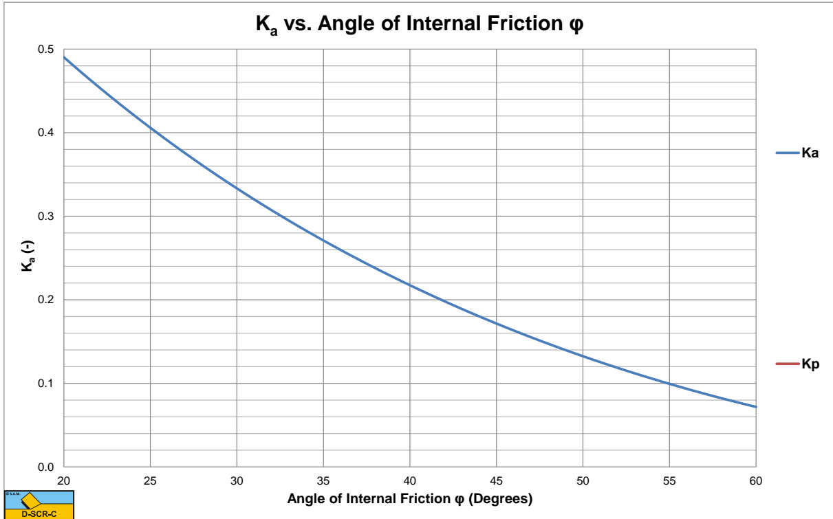
Figure 2-60: The coefficient of active soil failure K_a .
