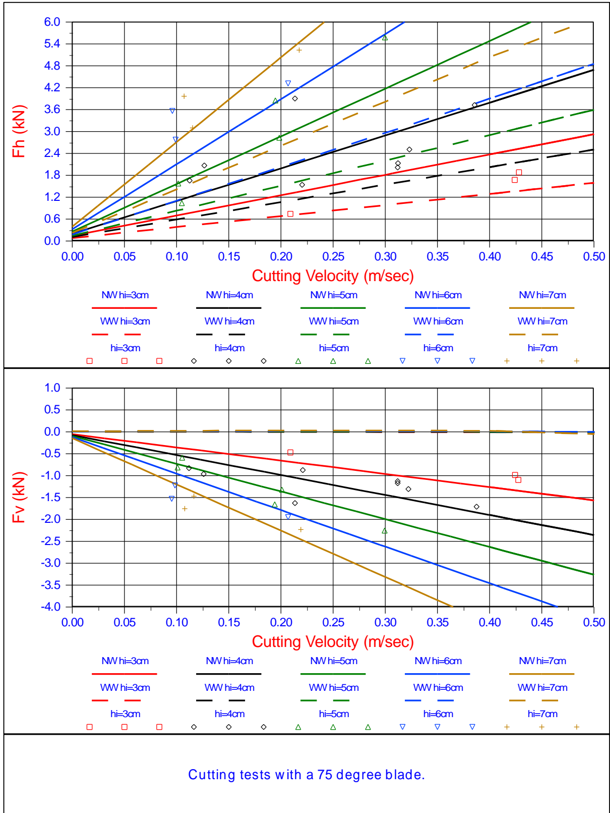
Figure 12-37: Cutting forces for cutting depths ( h_i ) from 3 to 7 cm; blade angle 75^\circ .
