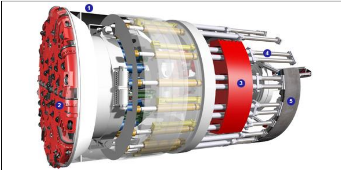
Figure Y-77: A TBM of Herrenknecht.
