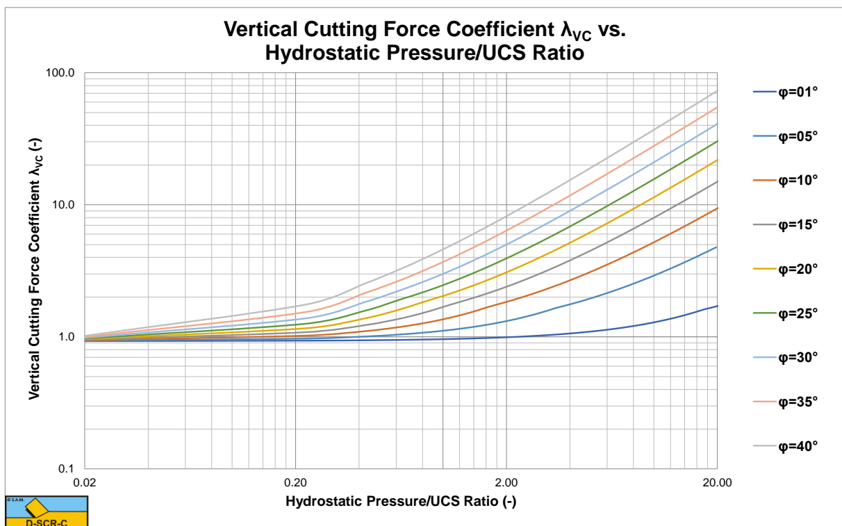
Figure X-4: The vertical cutting force coefficient \lambda_{VC} for a 30 degree blade.
