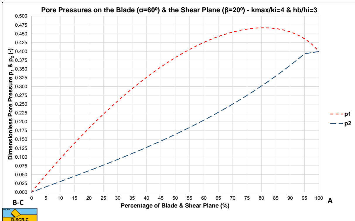
Figure 6-24: The dimensionless pressures on the blade and the shear plane, \alpha=60^\circ , \beta=20^\circ , k_i/k_{max}=0.25 , h_i/h_b=1/1 .
