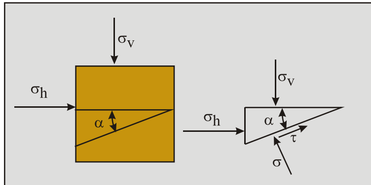
Figure 2-44: The stresses on a soil element.
