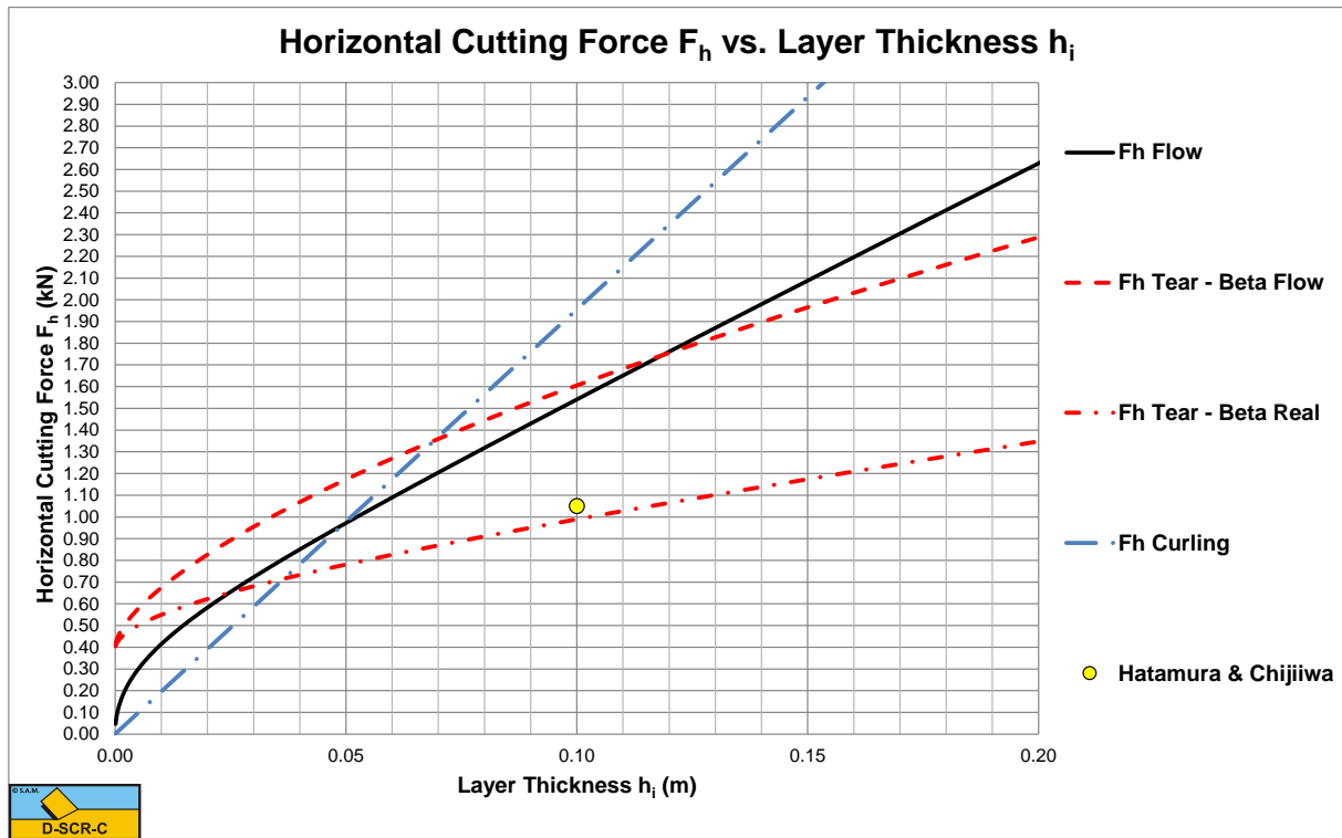
Figure 7-48: The 30 degree experiment.
