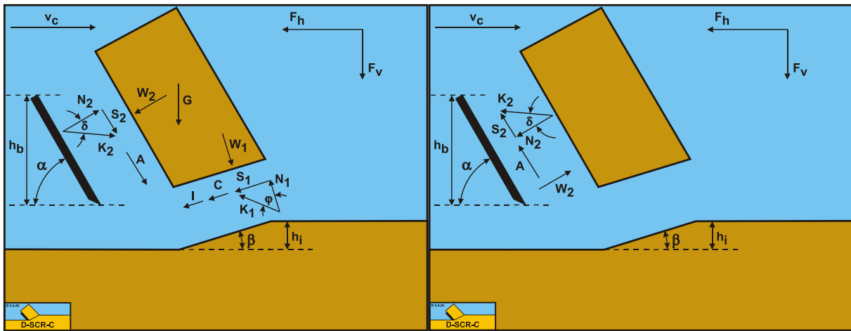
Figure 3-6: The forces on the layer cut.
