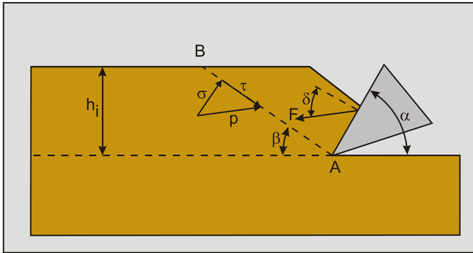
Figure 8-24: Model for shear failure by Nishimatsu (1972).
