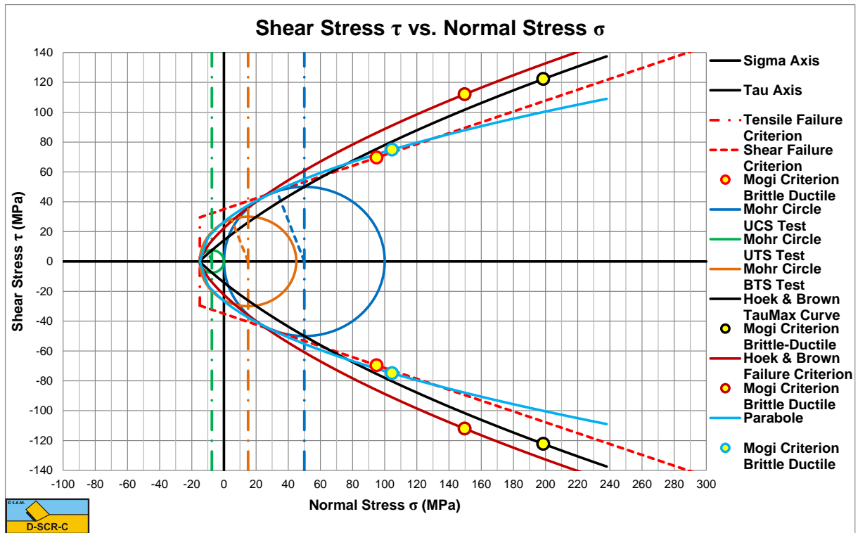
Figure 8-17: The failure criteria.
