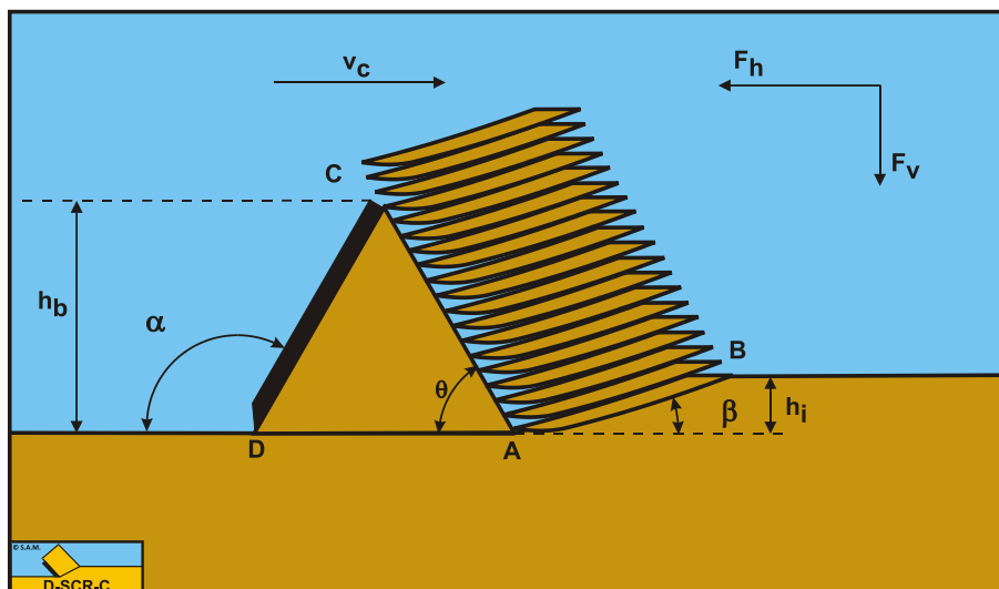
Figure 12-3: The cutting mechanism.
