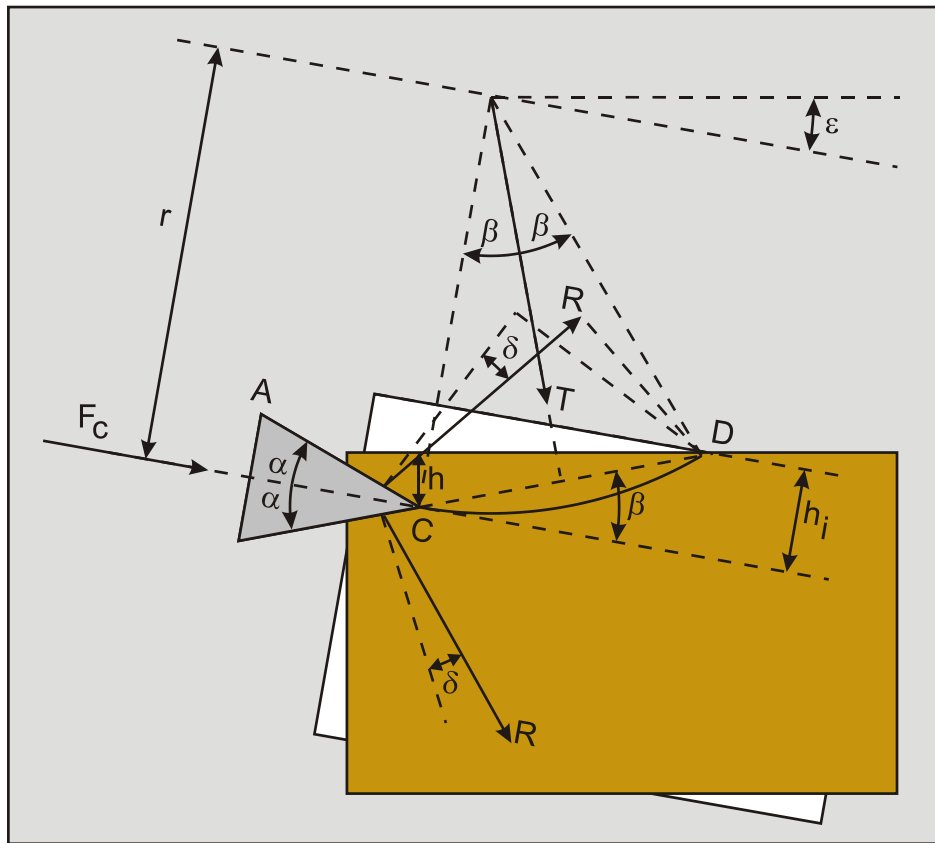
Figure 8-22: The model of Evans under an angle \epsilon .
