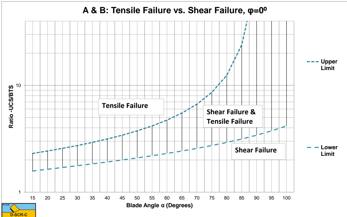
Figure W-12: The tensile/shear failure range based on UCS/BTS for \phi=0^\circ .
