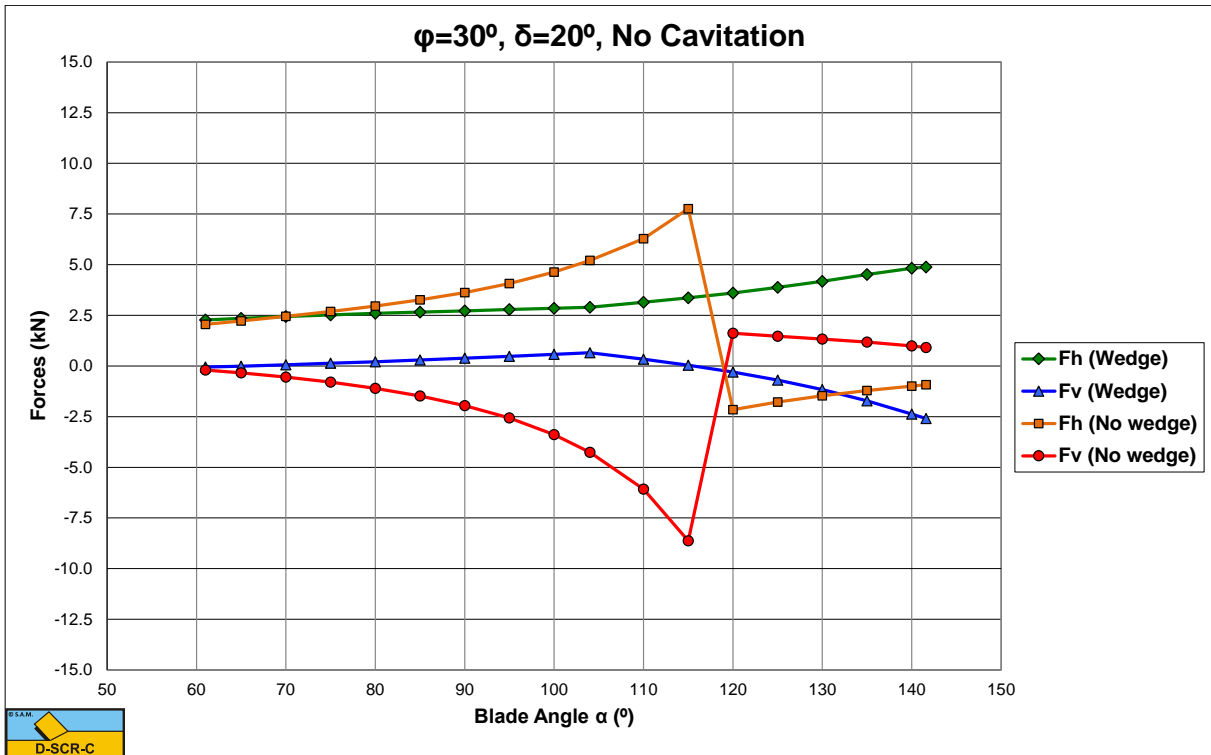
Figure 12-23: No cavitation, the cutting forces as a function of the blade angle \alpha for \phi=30^\circ and \delta=20^\circ .
