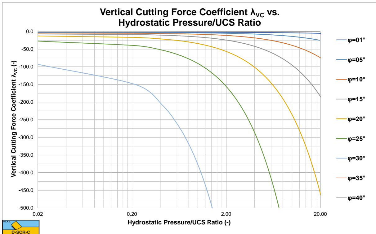
Figure X-34: The vertical cutting force coefficient \lambda_{VC} for a 120 degree blade.
