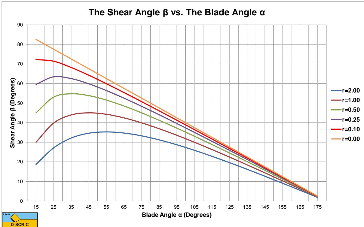
Figure 7-21: The shear angle as a function of the blade angle and the ac ratio r .
