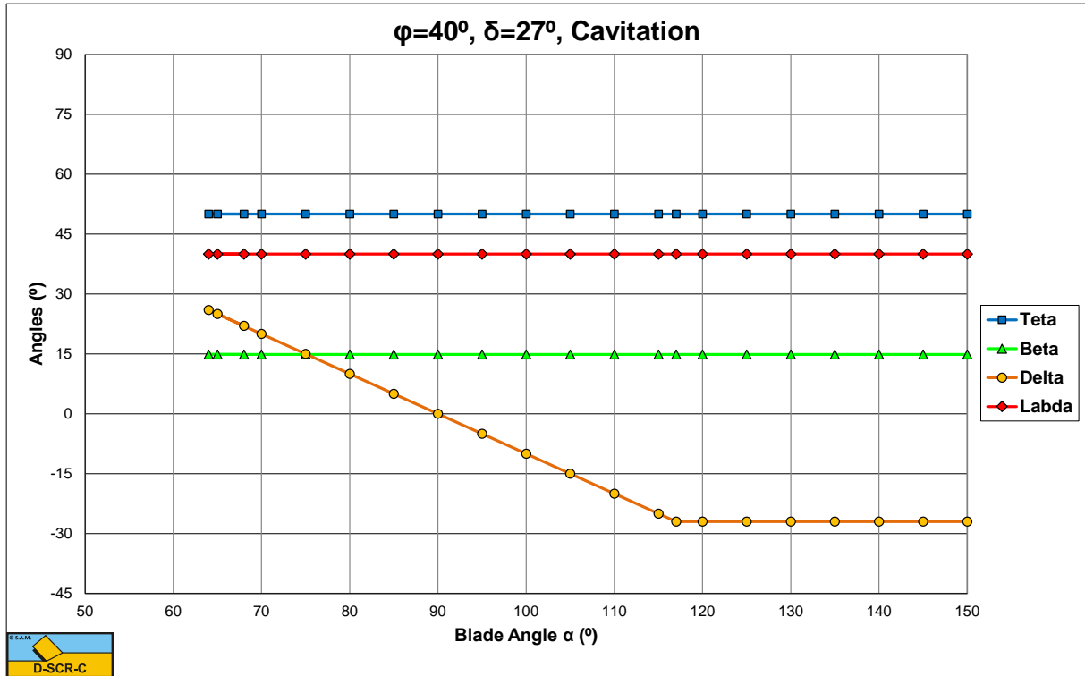
Figure Q-5: Cavitating, the angles \theta , \beta , \delta_m and \lambda as a function of the blade angle \alpha for \varphi=40^\circ and \delta=27^\circ .
