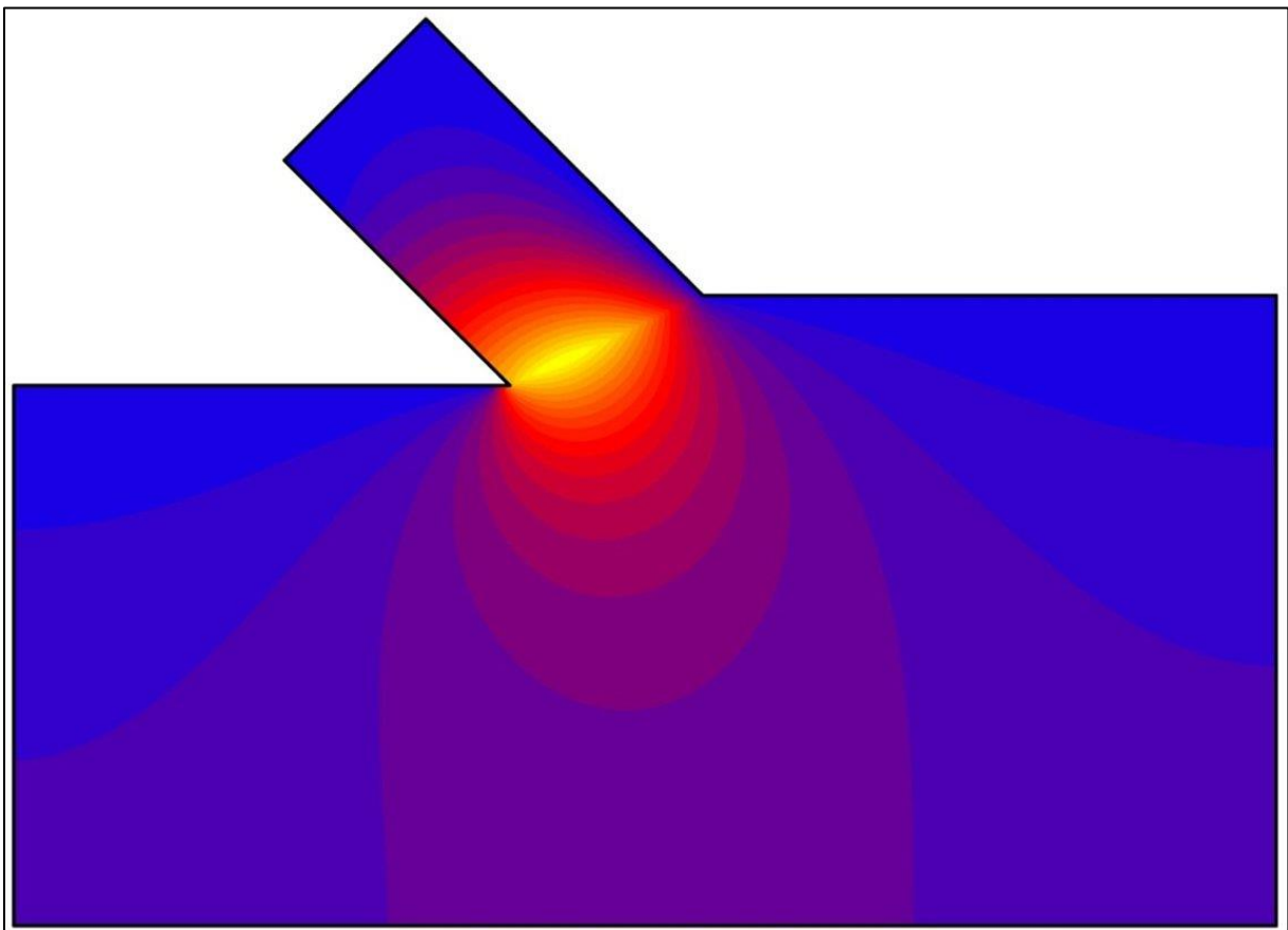
Figure 6-15: The equipotential lines in color.
