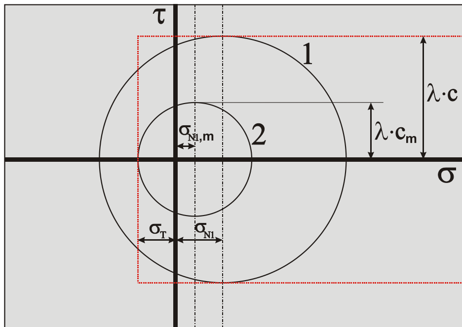
Figure 7-28: The Mohr circles when cutting clay.
