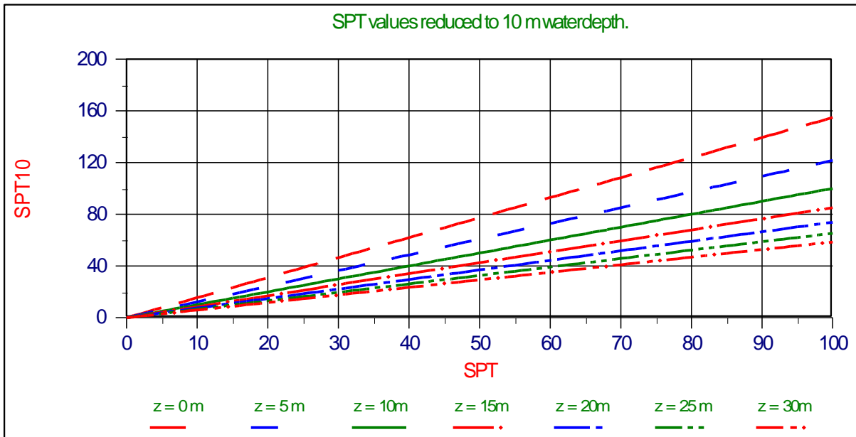
Figure 6-30: SPT values reduced to 10m water depth.
