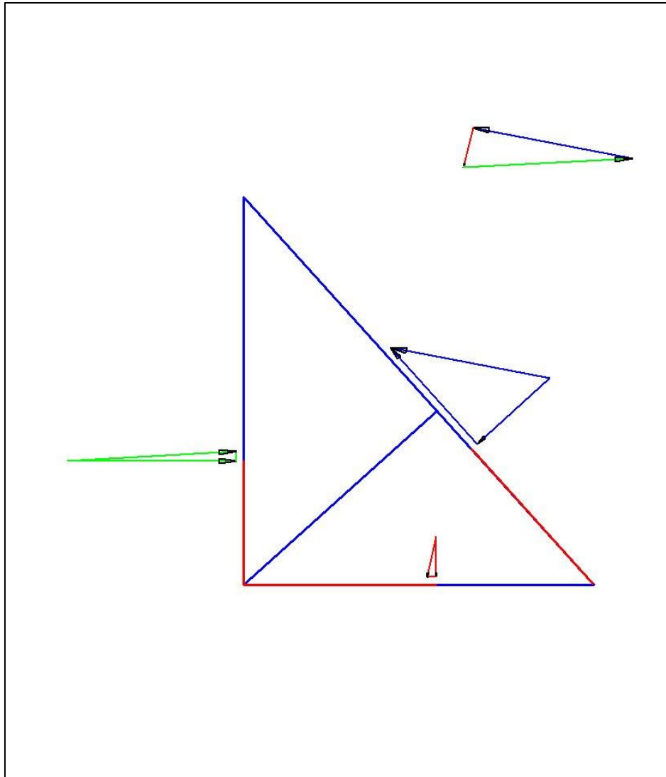
Figure T-3: The forces on the wedge for a 90^\circ blade.
