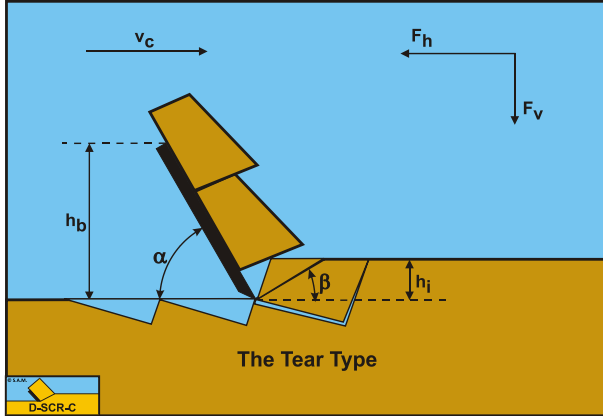
Figure 9-13: The Tear Type cutting mechanism in rock under hyperbaric conditions.
