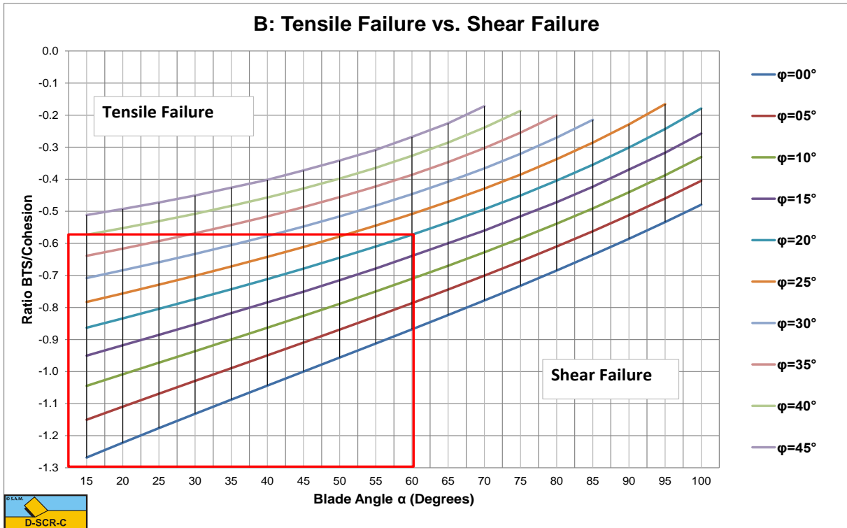
Figure W-7: The tensile/shear failure criterion based on BTS/Cohesion.
