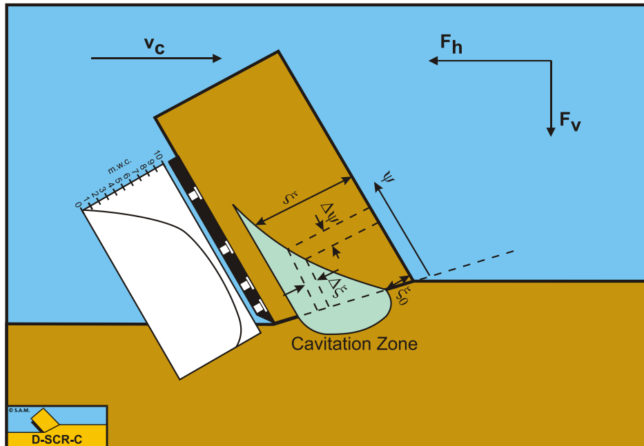
Figure 6-49: The development of cavitation over the blade.
