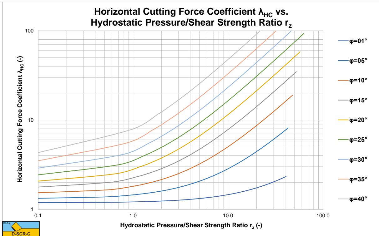
Figure 9-19: The horizontal cutting force coefficient \lambda_{HC} for a 60 degree blade.
