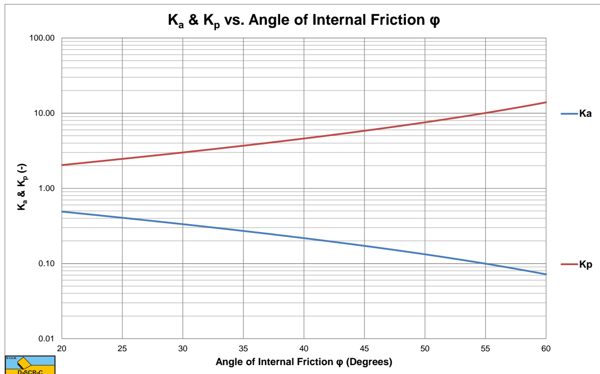
Figure 2-59: The coefficients of active and passive soil failure K_a & K_p .
