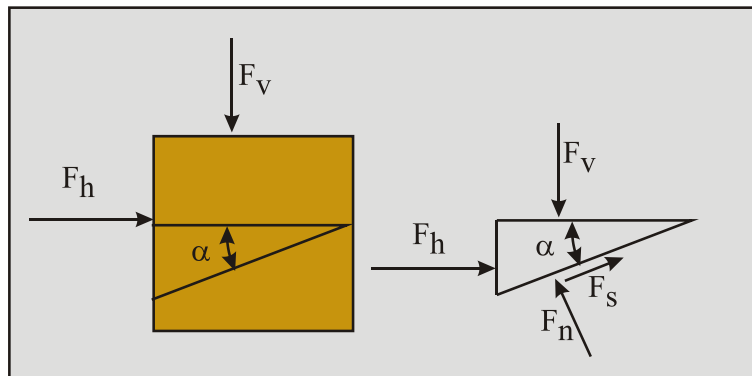
Figure 2-45: The forces on a soil element.
