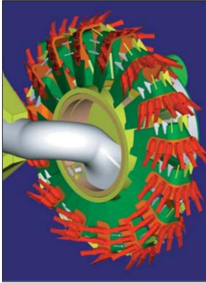
Figure Y-39: Dredging wheel (IHC).
