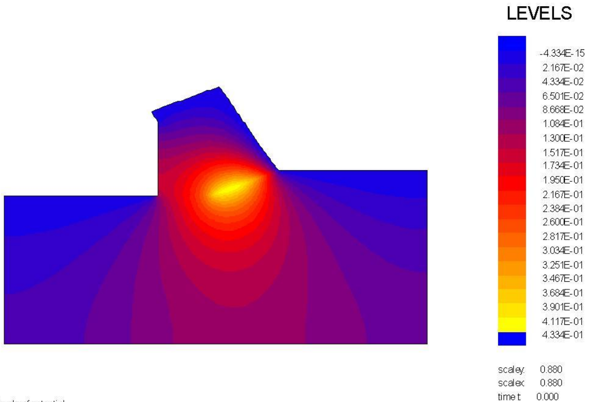
Figure S-14: Equipotential distribution in color.
