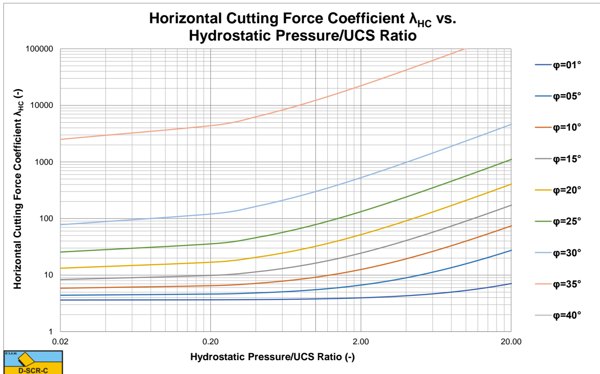
Figure X-33: The horizontal cutting force coefficient \lambda_{HC} for a 120 degree blade.
