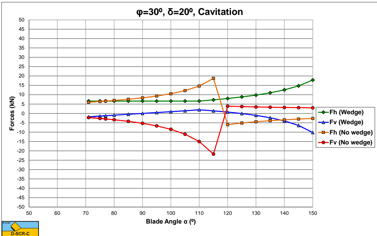
Figure 12-25: Cavitating, the cutting forces as a function of the blade angle \alpha for \phi=30^\circ and \delta=20^\circ .
