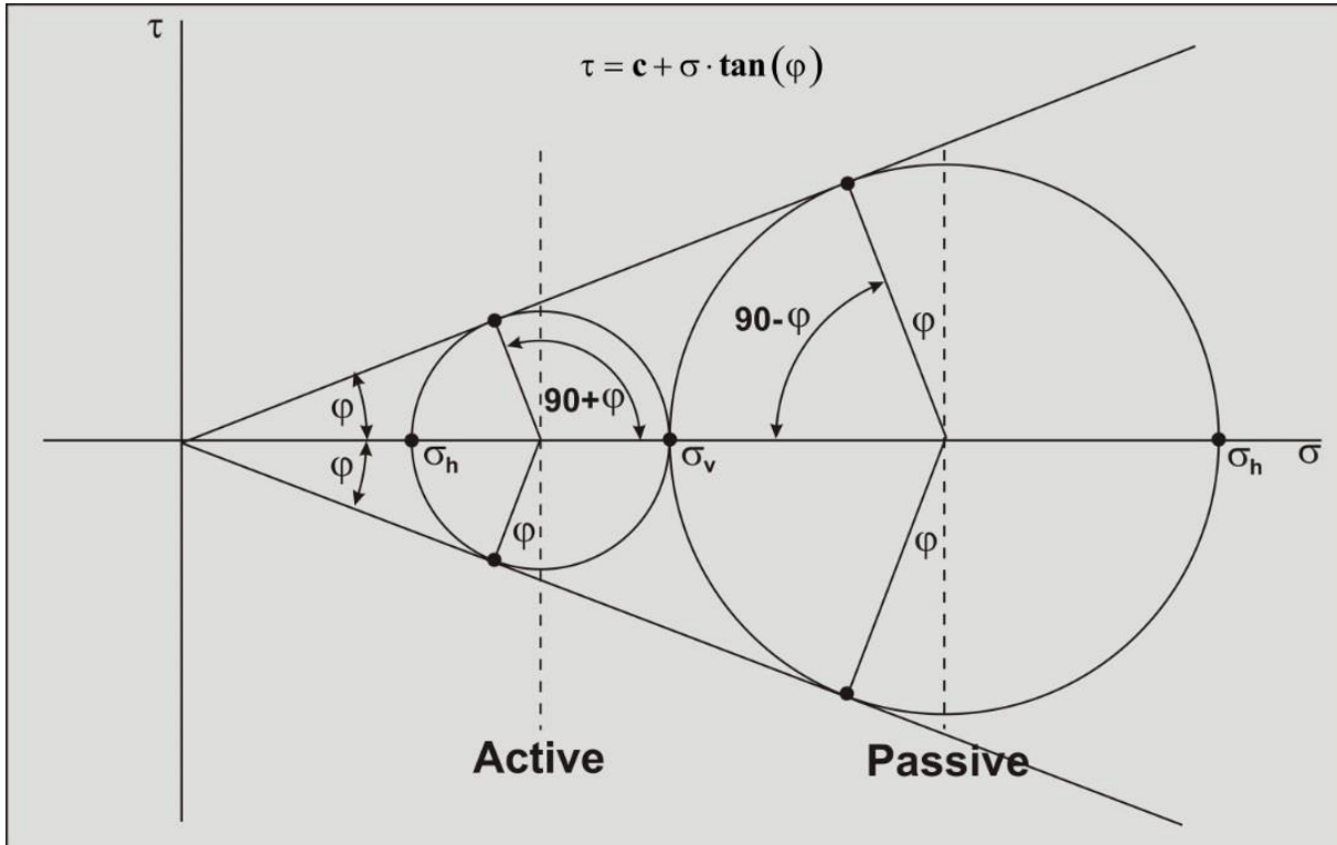
Figure 2-57: The Mohr circles for active and passive failure for a cohesion less soil.
