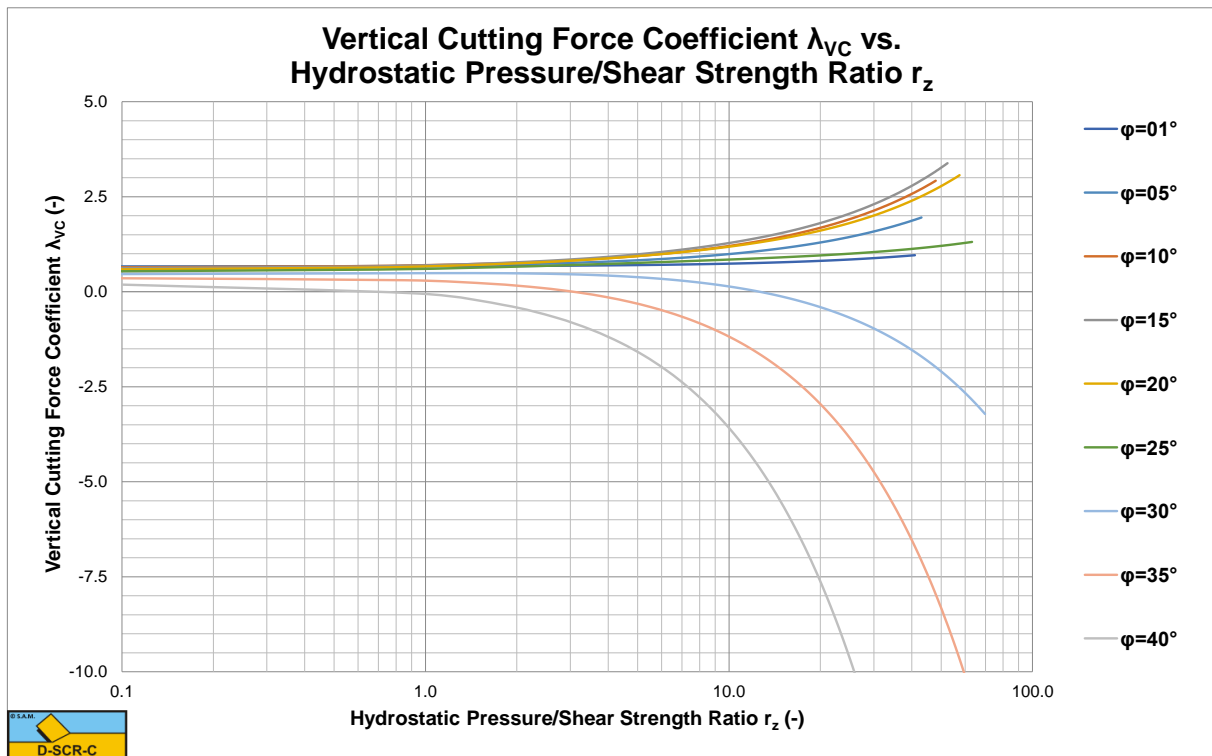
Figure 9-20: The vertical cutting force coefficient \lambda_{VC} for a 60 degree blade. Positive downwards.
