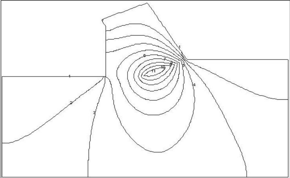
Figure 12-14: Equipotential lines of pore pressures.
