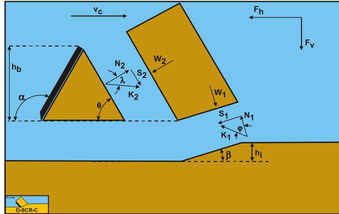
Figure 12-4: The forces on the layer cut in saturated sand with a wedge.
