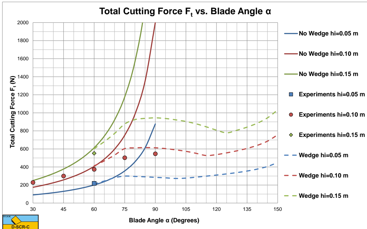
Figure 11-13: The total force of Hatamura & Chijiwa (1977B) versus the calculated total force, with and without wedge.
