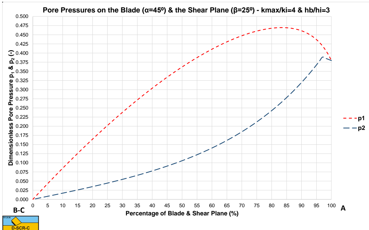
Figure 6-23: The dimensionless pressures on the blade and the shear plane, \alpha=45^\circ , \beta=25^\circ , k_i/k_{max}=0.25 , h_i/h_b=1/2 .
