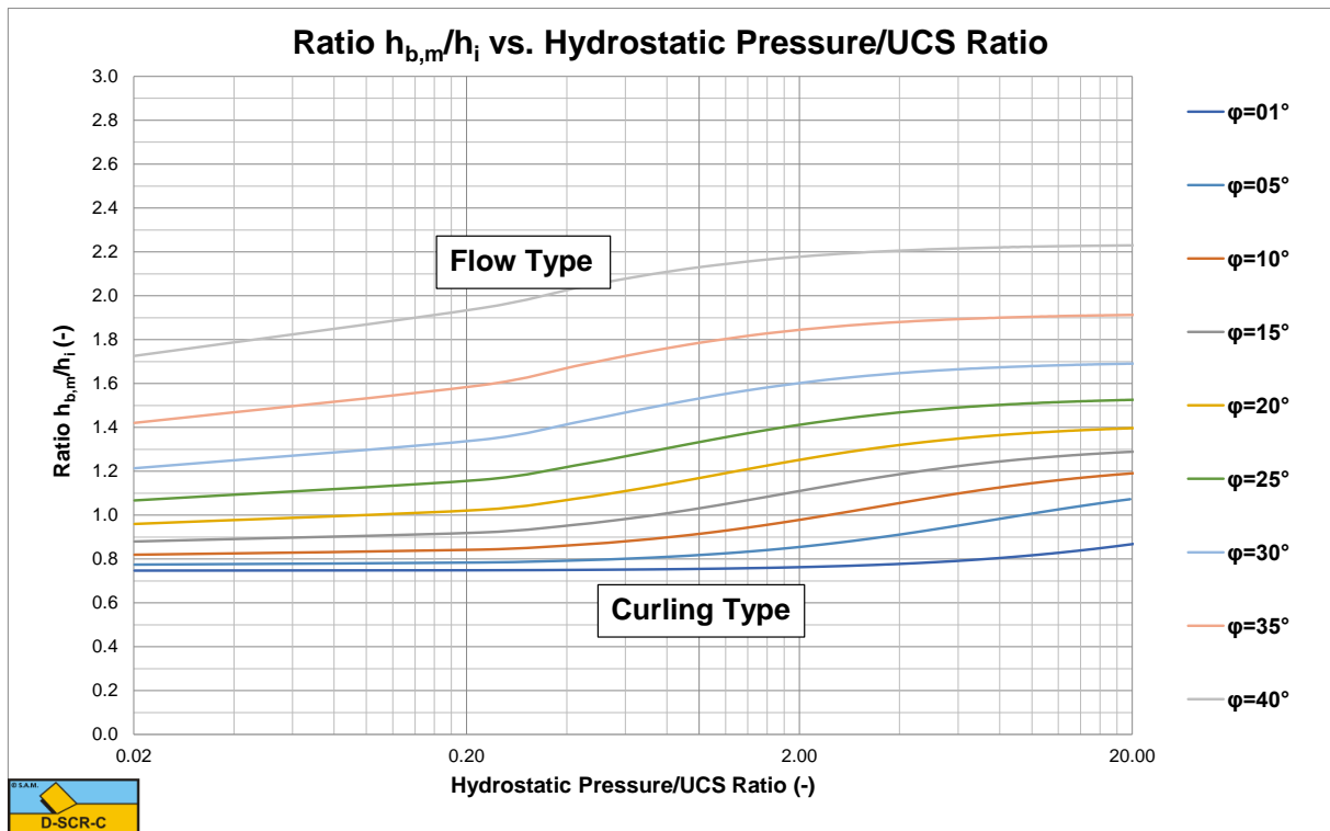
Figure X-16: The ratio h_{b,m}/h_i for a 75 degree blade.
