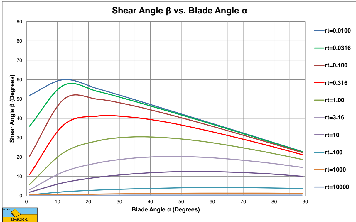
Figure 7-29: The shear angle \beta vs. the blade angle \alpha for the Tear Type.
