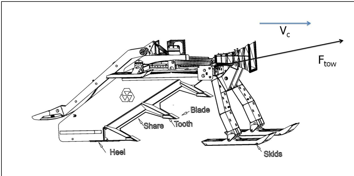
Figure Y-52: Subsea Cable Trench Plough Sea Stallion 4 (IHC).
