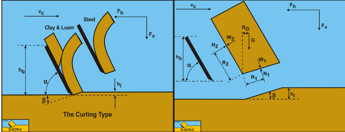
Figure 3-8: The Curling Type of cutting mechanism. Figure 3-9: The general equilibrium of moments.
