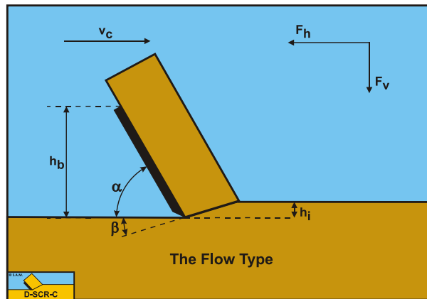
Figure 7-18: The Flow Type cutting mechanism when cutting clay.
