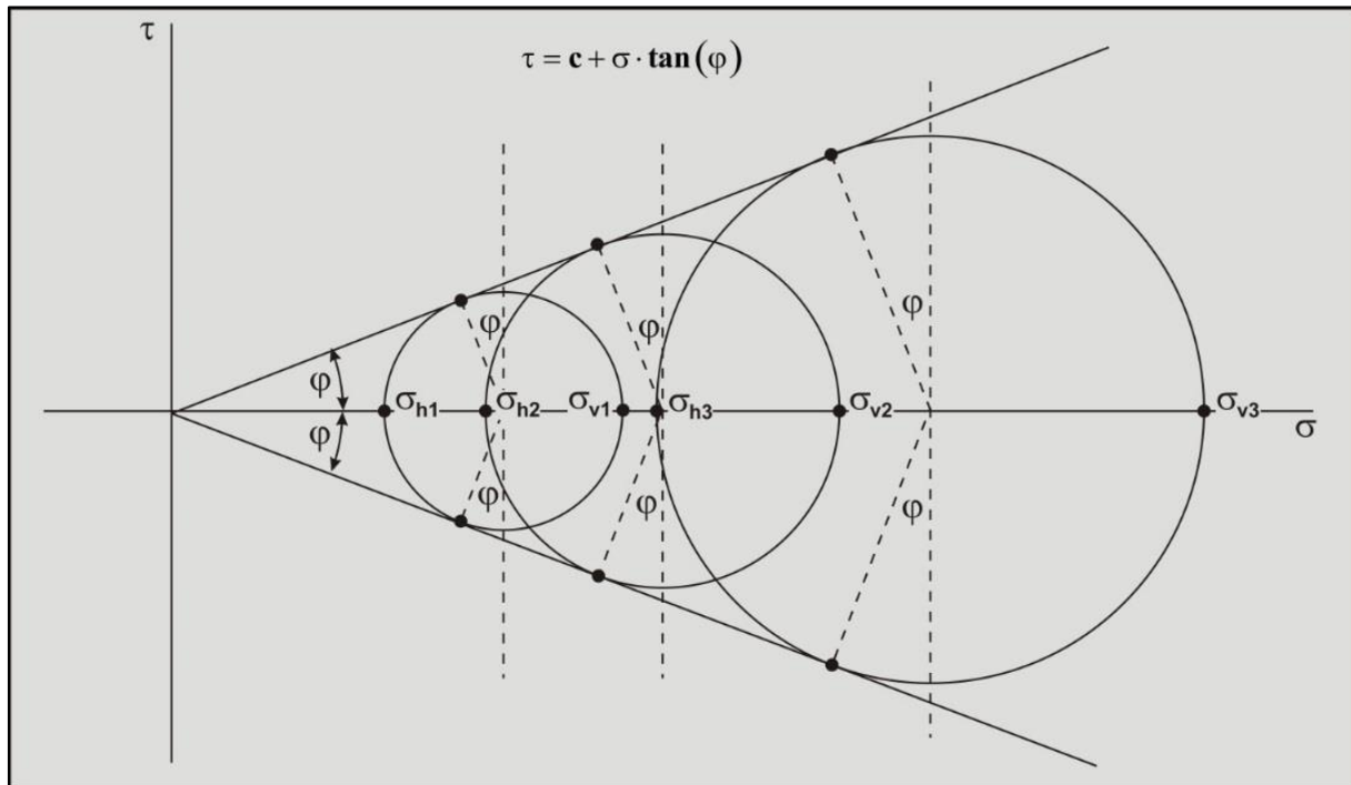
Figure 2-47: Determining the angle of internal friction from tri-axial tests of cohesion less soil.
