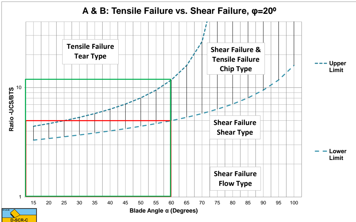
Figure 8-54 The tensile vs. shear failure range based on the UCS to BTS ratio.
