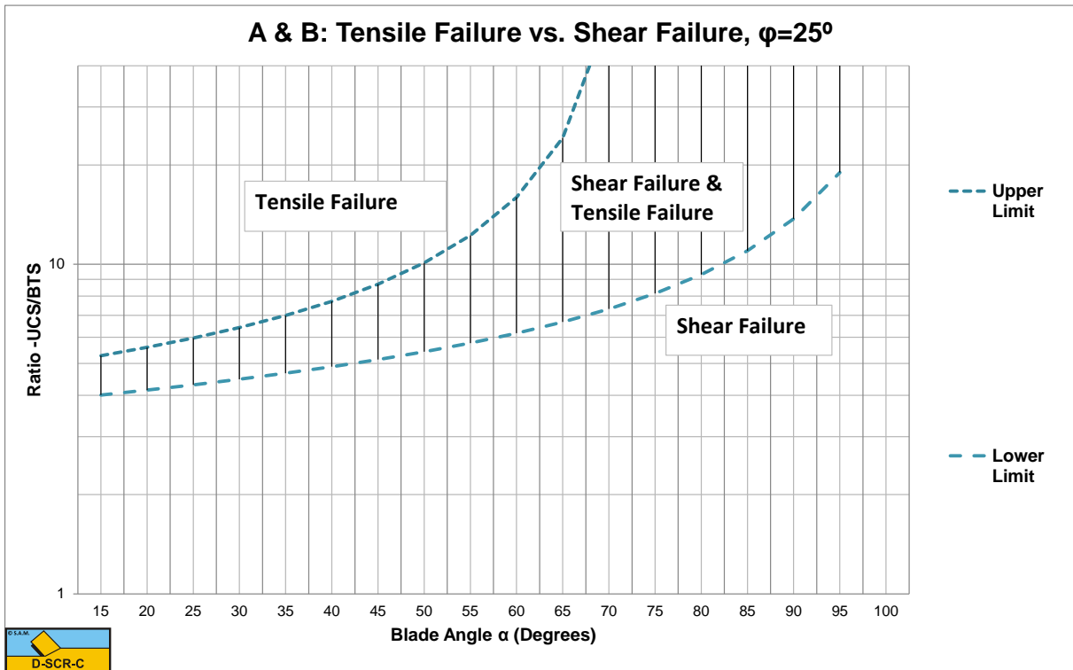
Figure W-22: The tensile/shear failure range based on UCS/BTS for \phi=25^\circ .
