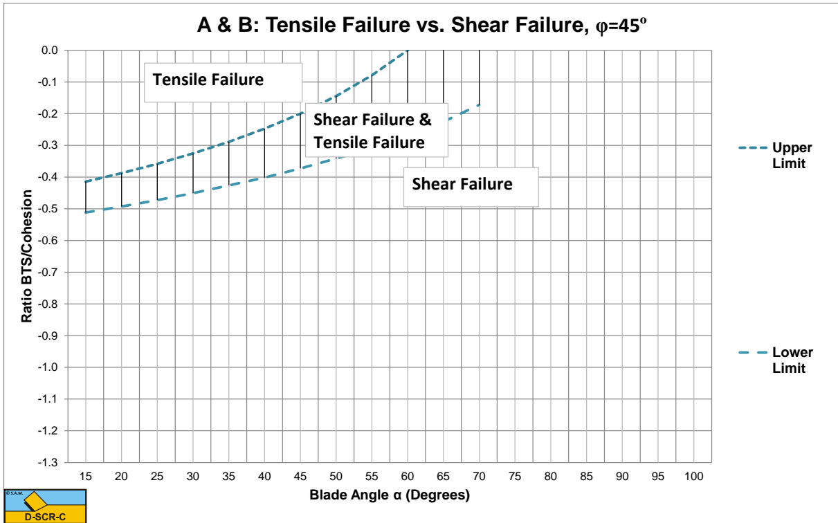
Figure W-29: The tensile/shear failure range based on BTS/Cohesion for \phi=45^\circ .
