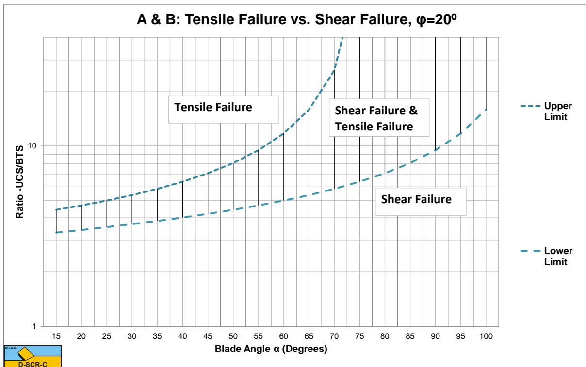
Figure W-20: The tensile/shear failure range based on UCS/BTS for \phi=20^\circ .
