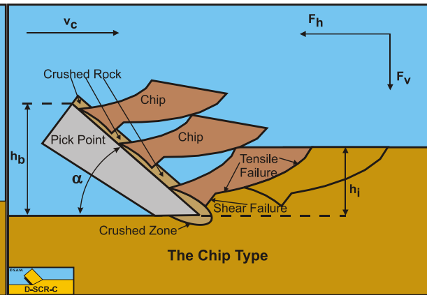
Figure 8-19: The Chip Type.
