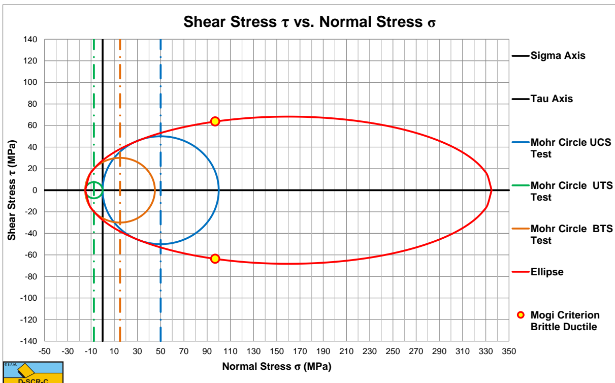
Figure 8-4: Failure envelope according to Verhoef (1997) (Figure 9.4) of intact rock.
