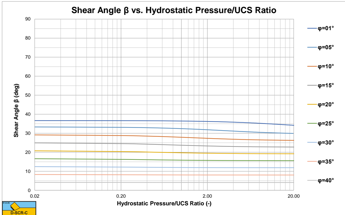
Figure X-27: The shear angle \beta for a 105 degree blade.
