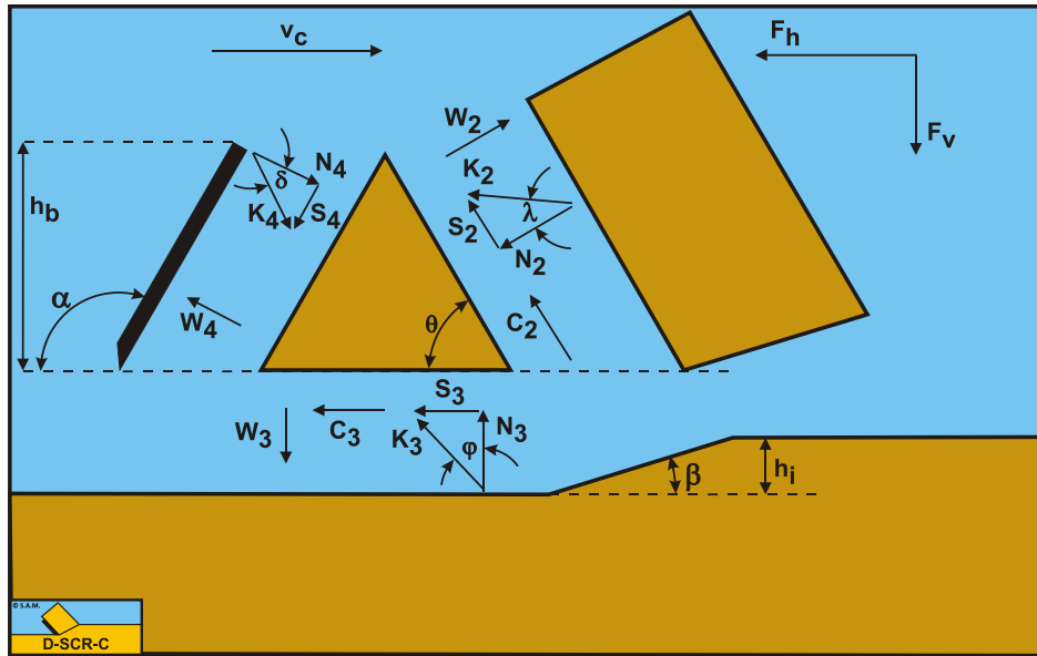
Figure 15-3: The forces on the wedge.
