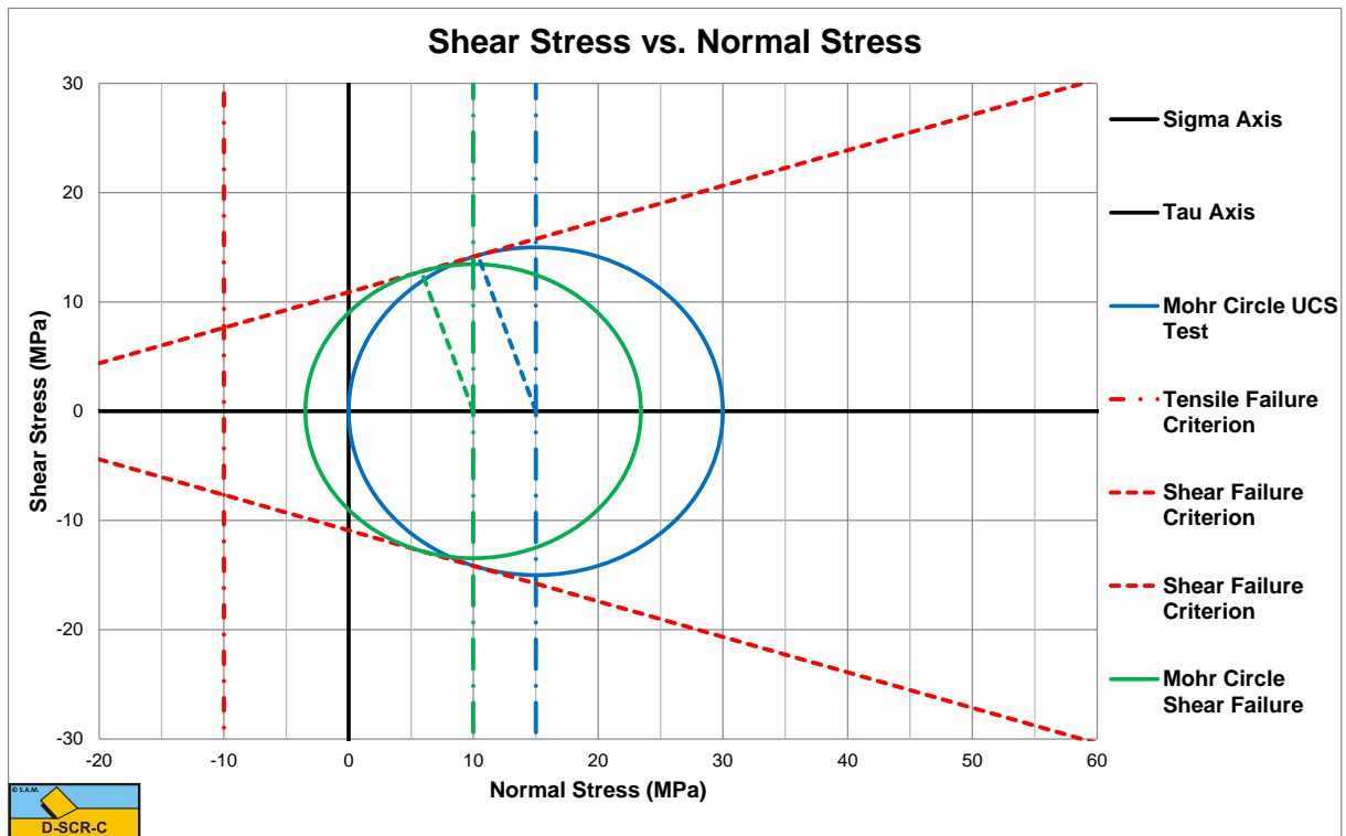
Figure 16-9: The Mohr circles for a tensile strength of -10 MPa. Shear Failure.
