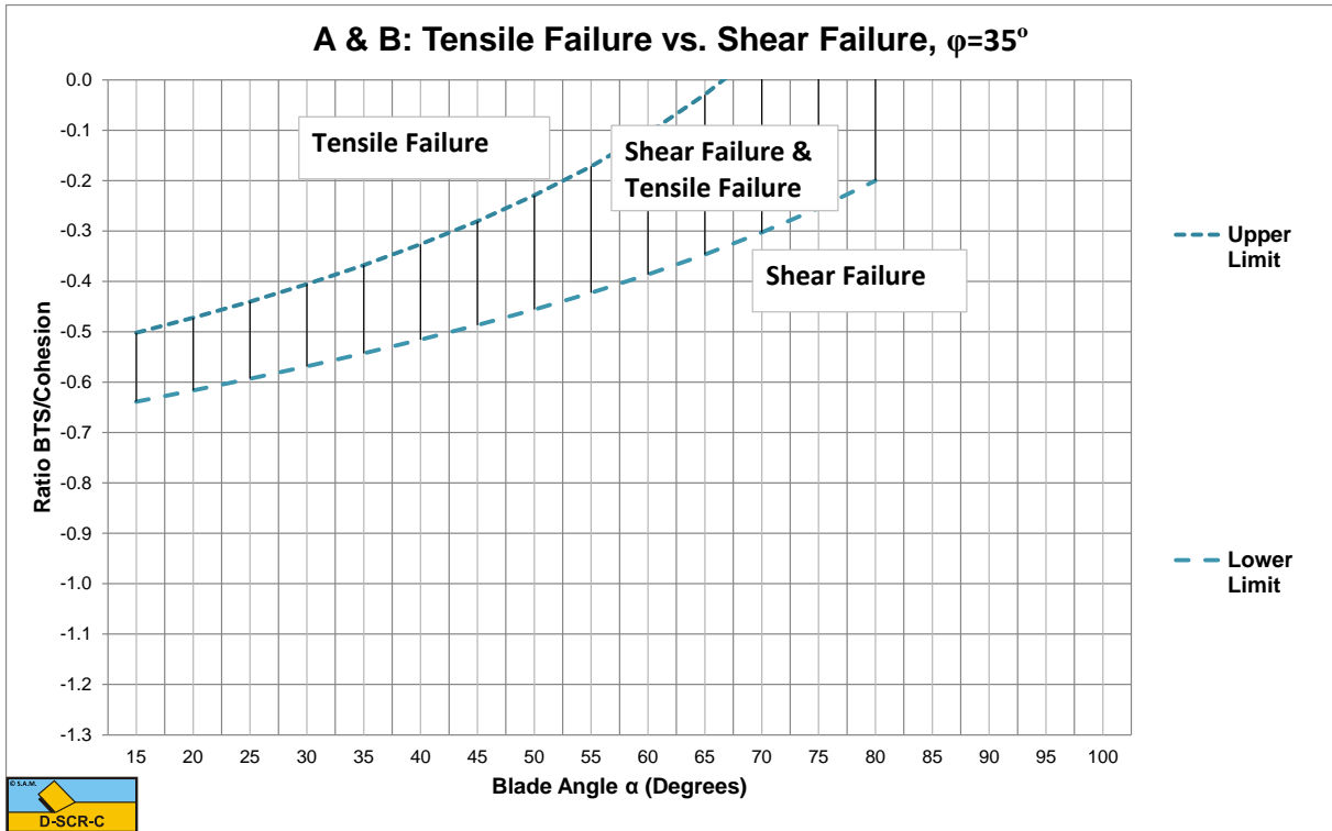
Figure W-25: The tensile/shear failure range based on BTS/Cohesion for \phi=35^\circ .
