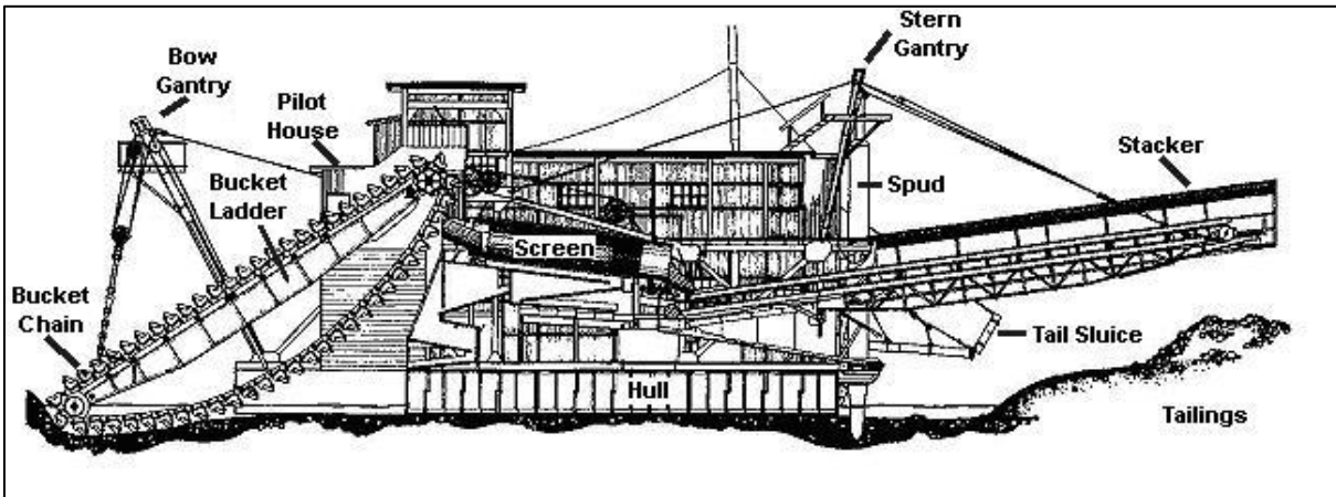
Figure Y-2: A gold dredging bucket ladder dredge (www.miningandmetallurgy.com).
