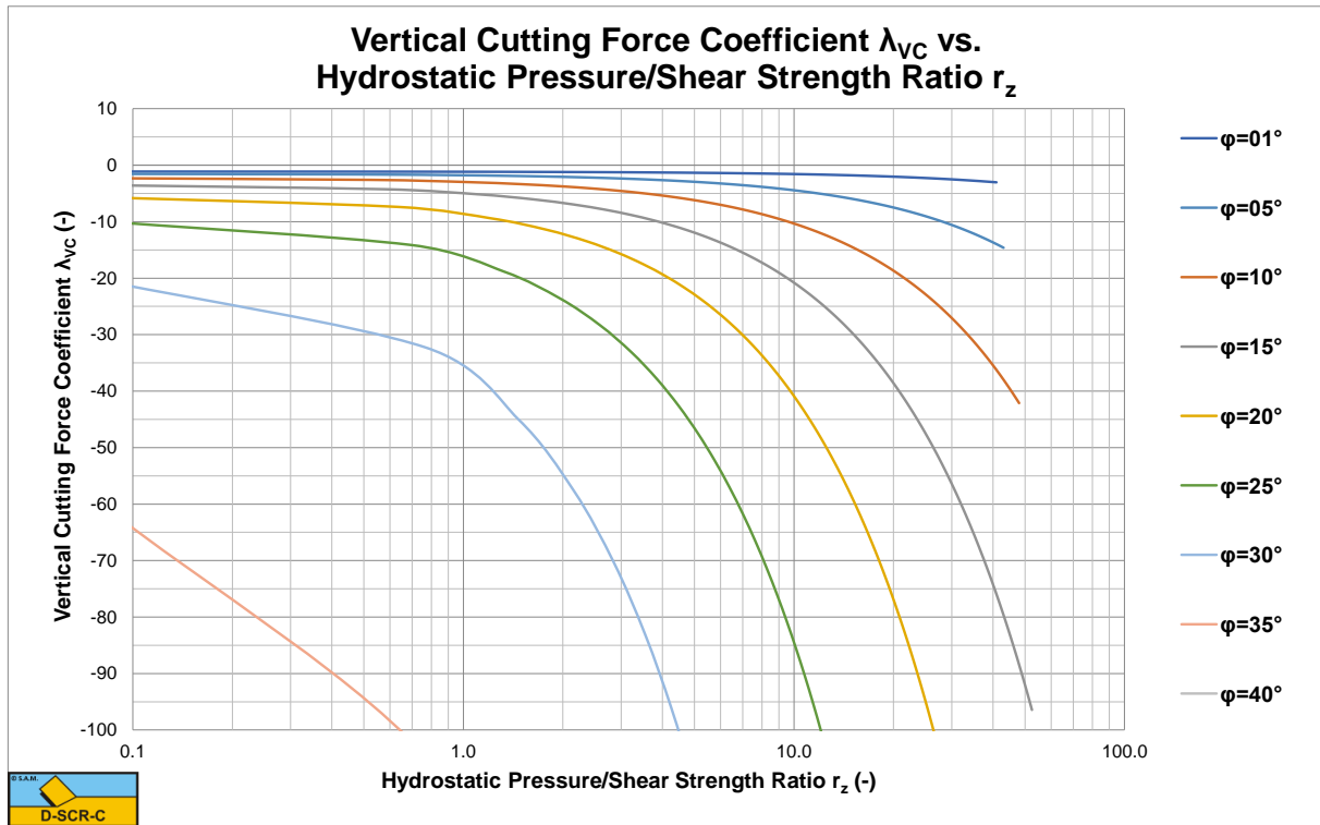
Figure 9-27: The vertical cutting force coefficient \lambda_{VC} for a 110 degree blade. Positive upwards.
