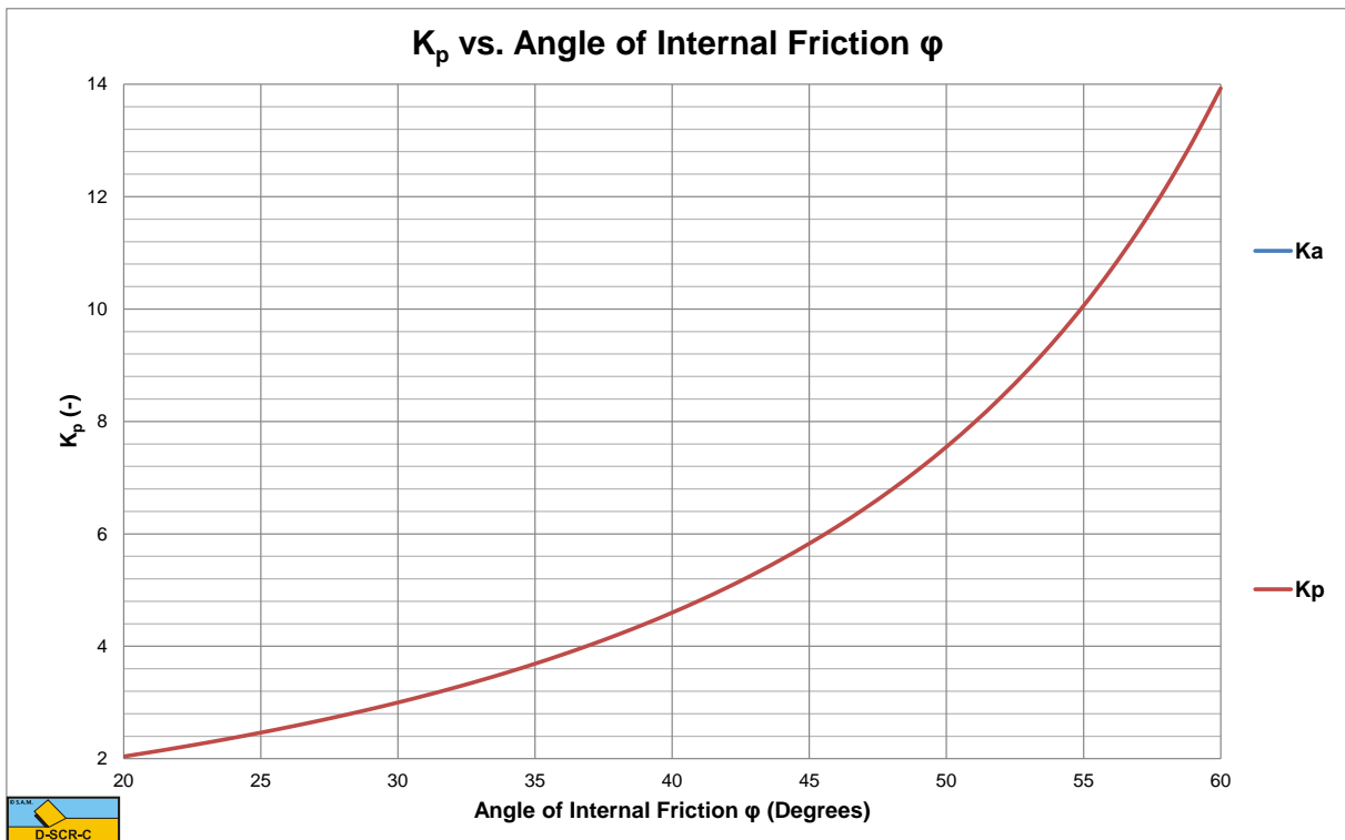
Figure 2-61: The coefficient of passive soil failure K_p .
