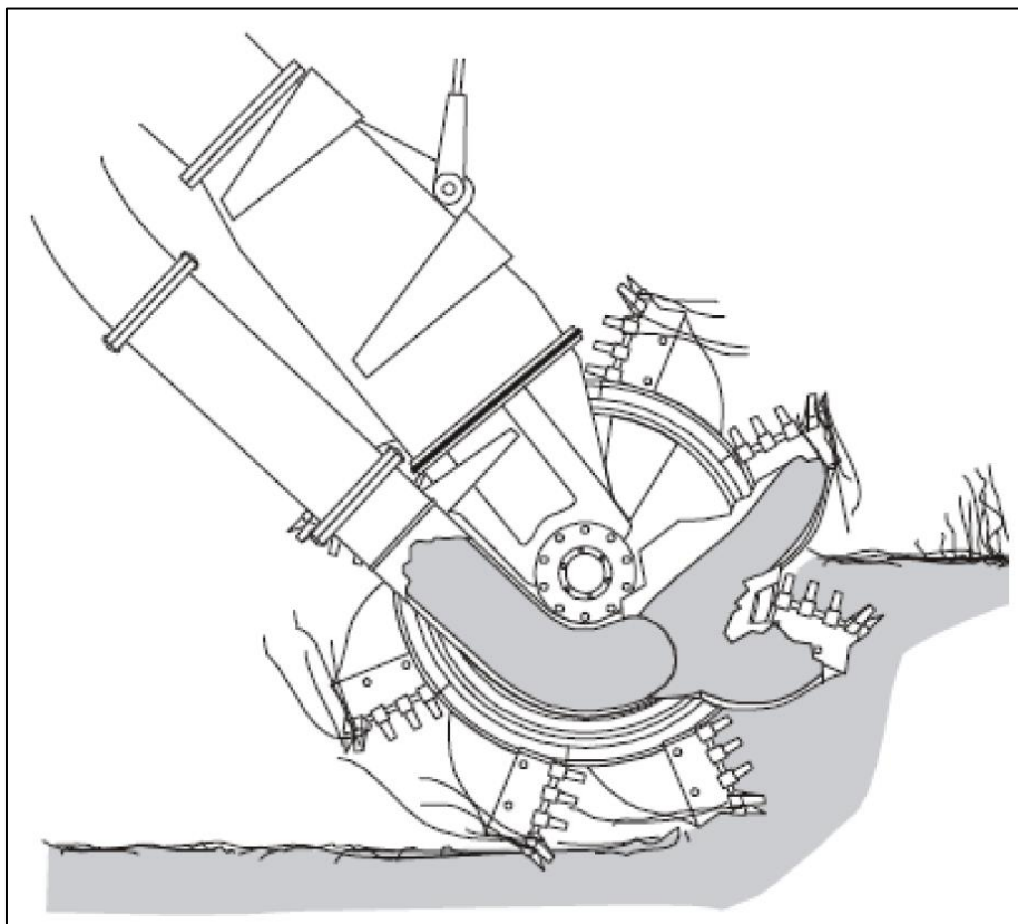
Figure Y-40: Dredging wheel (IHC).
