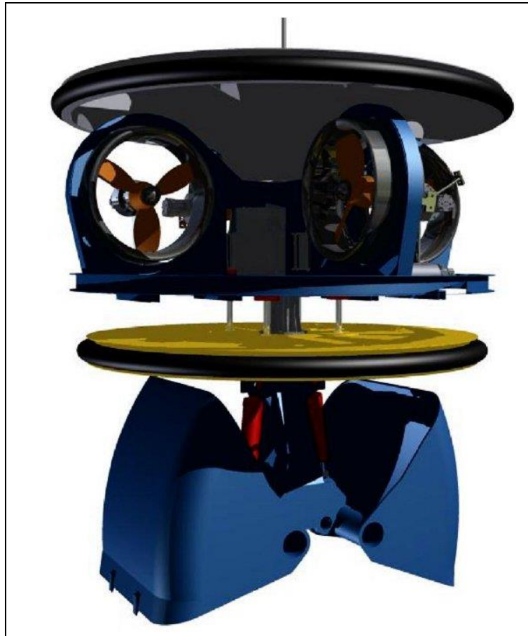
Figure Y-35: A deep sea mining clamshell (Seatools).
