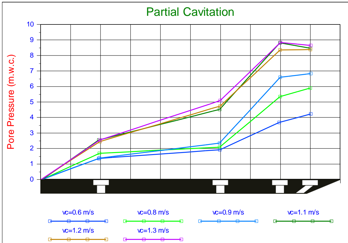
Figure M-8: Measured absolute pore pressures.
