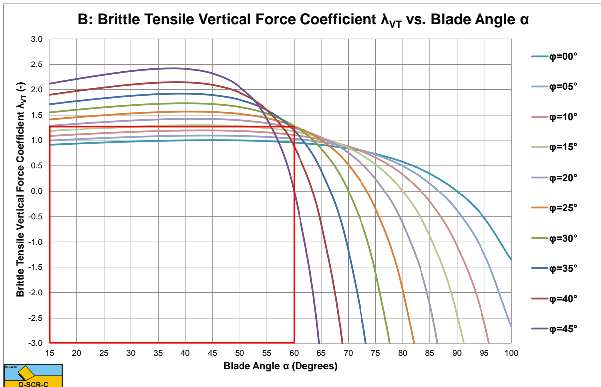
Figure 8-46: The brittle (tensile failure) vertical force coefficient \lambda_{VT} .
