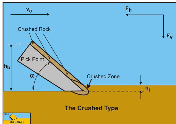
Figure 3-5: The Crushed Type.
