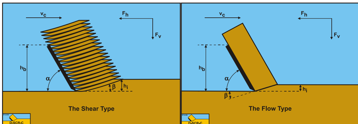
Figure 6-2: The cutting mechanism in water saturated sand, the Shear Type.
