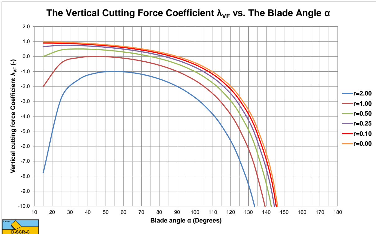
Figure 7-24: The vertical cutting force coefficient \lambda_{VF} as a function of the blade angle and the ac ratio r .
