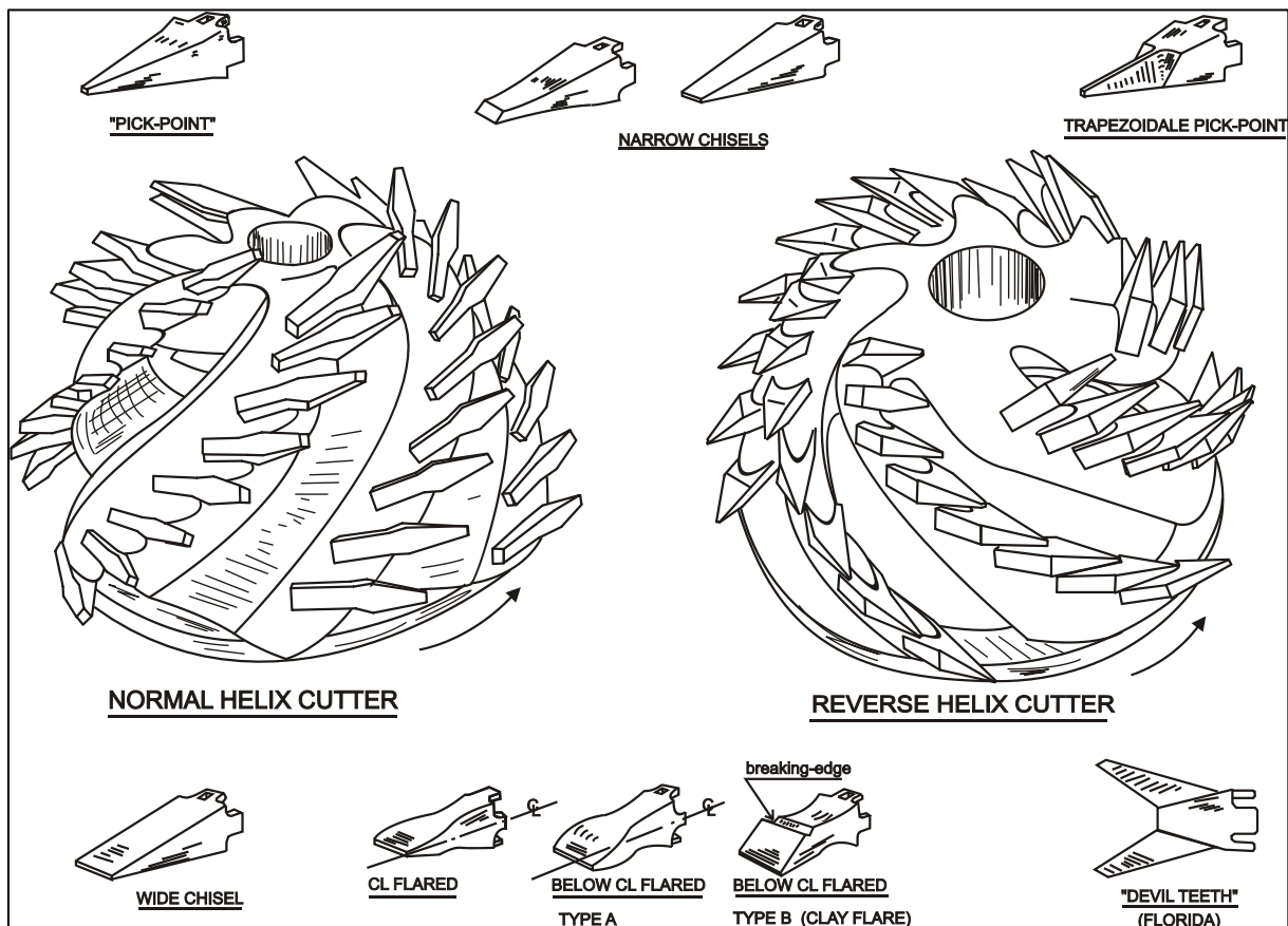
Figure 1-2: A rock cutter head with pick points.
