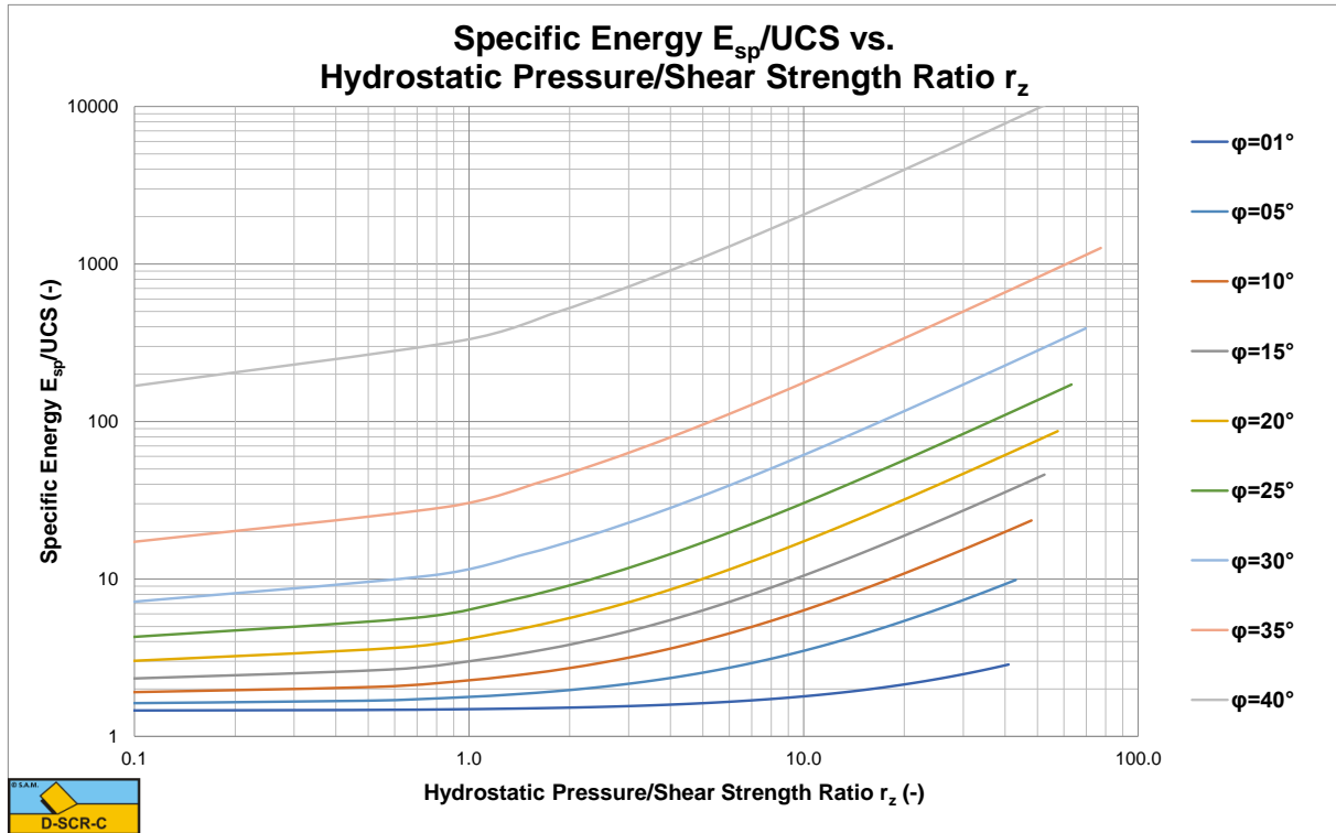
Figure 9-28: The E_{sp}/UCS ratio, for a 110 degree blade.
