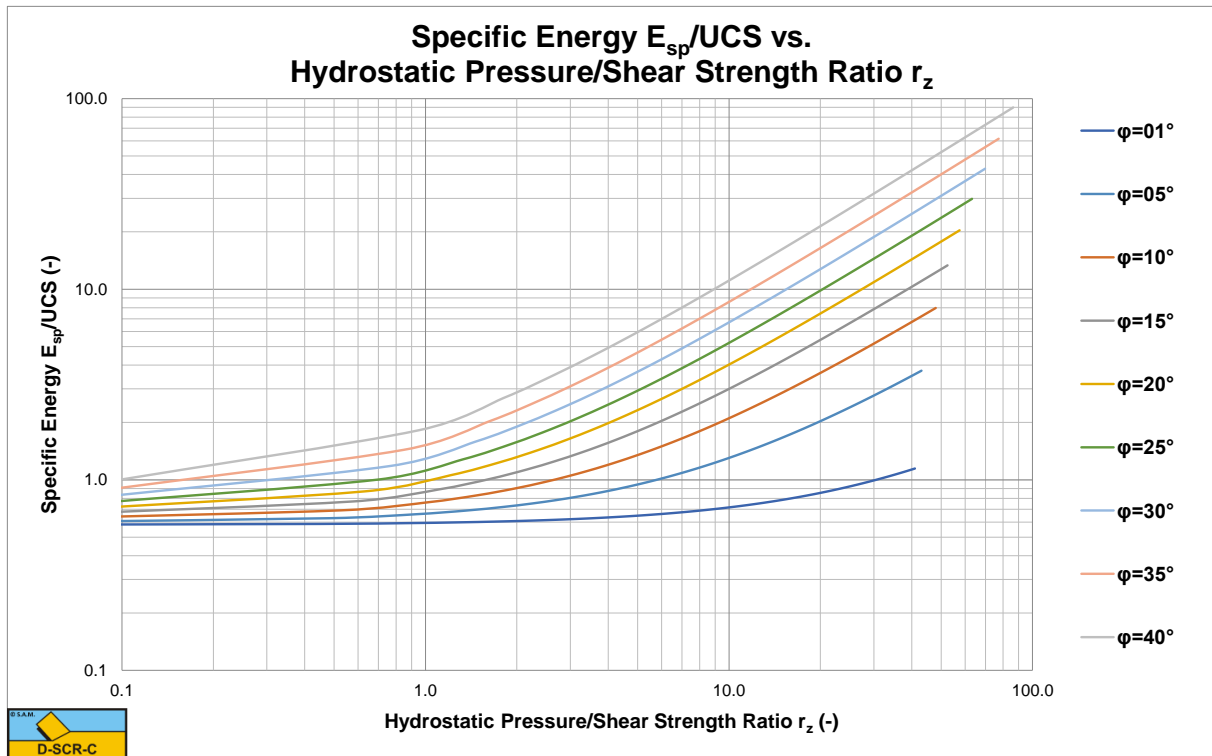
Figure 9-21: The E_{sp}/UCS ratio, for a 60 degree blade.
