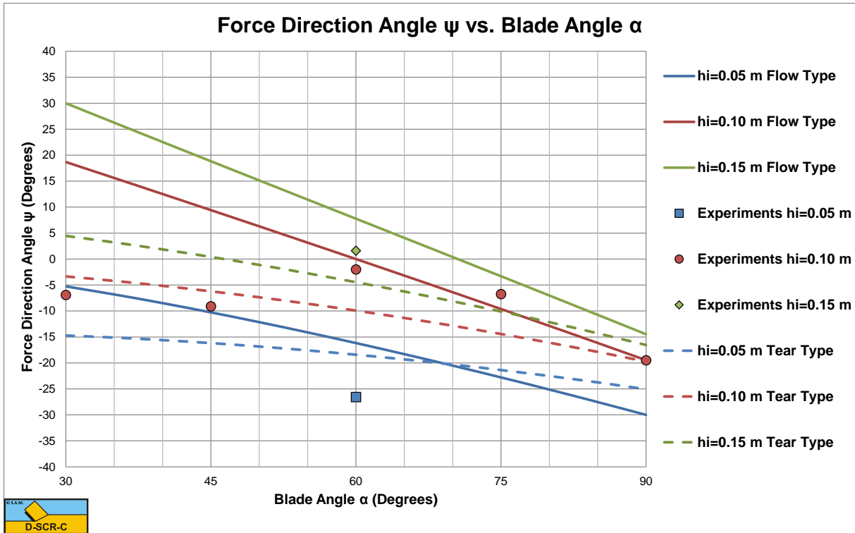
Figure 7-46: The direction of the total cutting force measured and calculated.
