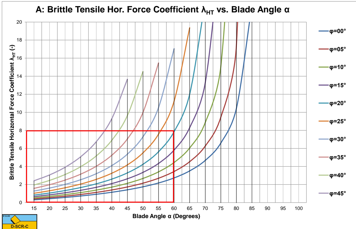
Figure 8-42: The brittle (tensile failure) horizontal force coefficient \lambda_{HT} .
