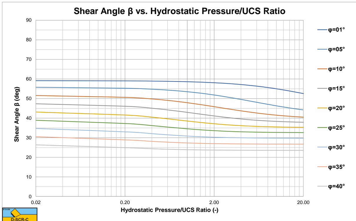
Figure X-12: The shear angle \beta for a 60 degree blade.
