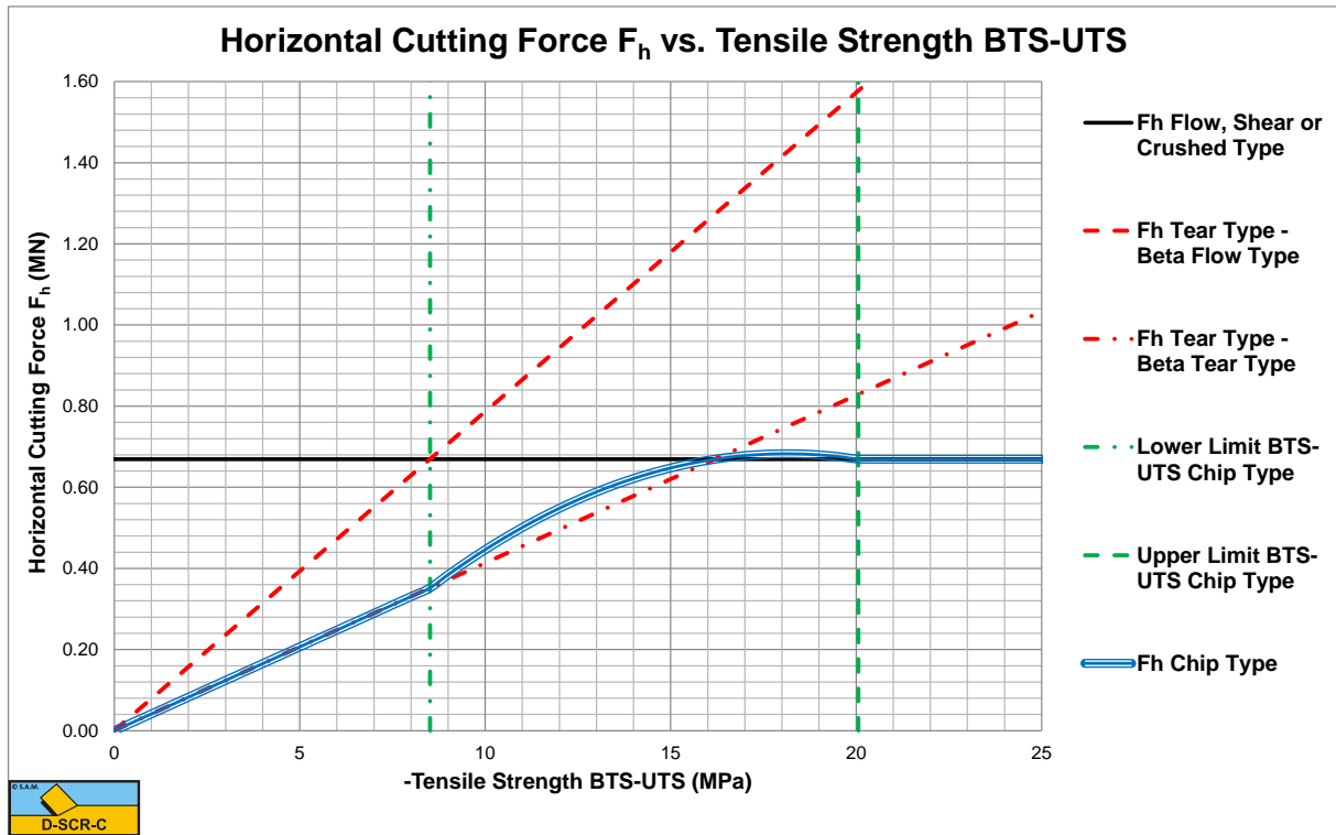
Figure 8-49: Horizontal cutting force: \alpha=60^\circ , UCS=100 MPa, \phi=20^\circ , h_i=0.1 m & w=0.1 m.
