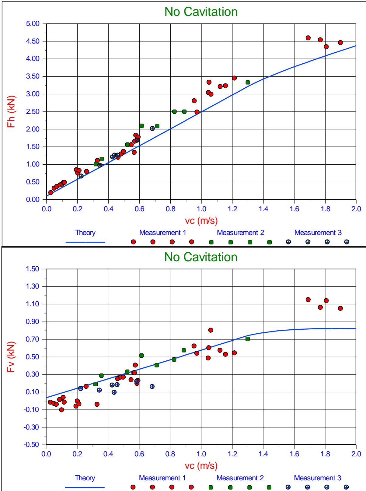
Figure M-24: \alpha=45^\circ , h_i=70 mm, h_b=141 mm.
