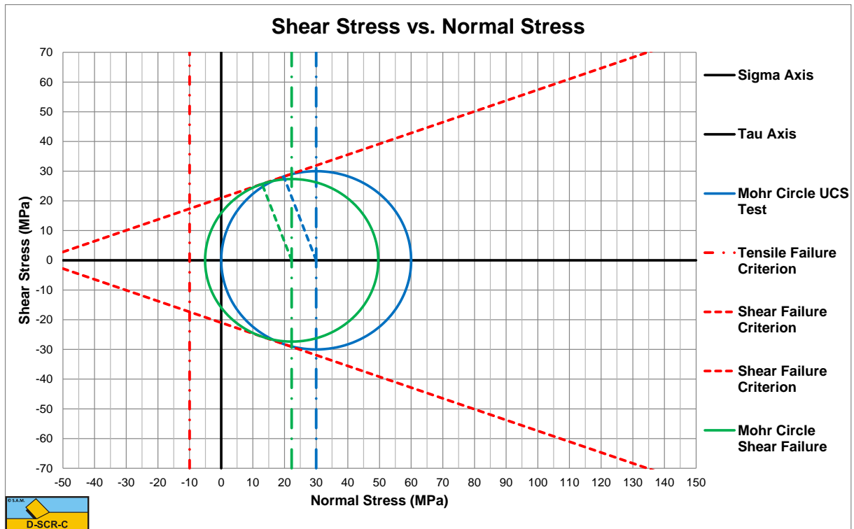
Figure 16-12: The Mohr circles with tensile strength of -10 MPa (UCS=60 MPa, \phi=20^\circ ). Shear Failure.
