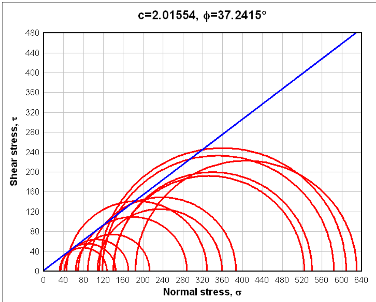
Figure 2-50: An example of Mohr circles resulting in an internal friction angle and cohesion ( www.dplot.com ).
