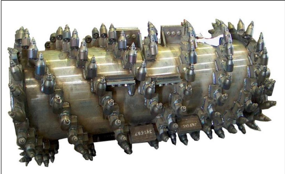
Figure Y-74: Drumcutter for dry mining applications.
