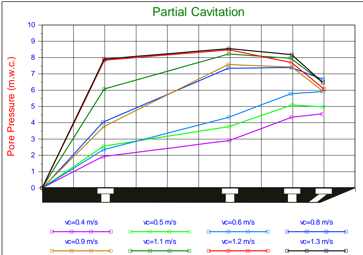
Figure 6-50: Partial cavitation limited by dissolved air, \alpha=45^\circ , h_i=7\text{cm} .
