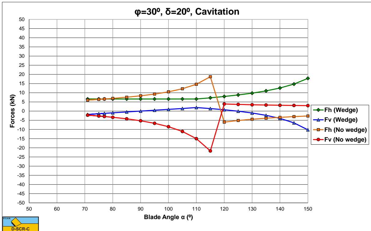
Figure Q-2: Cavitating, the cutting forces as a function of the blade angle \alpha for \varphi=30^\circ and \delta=20^\circ .
