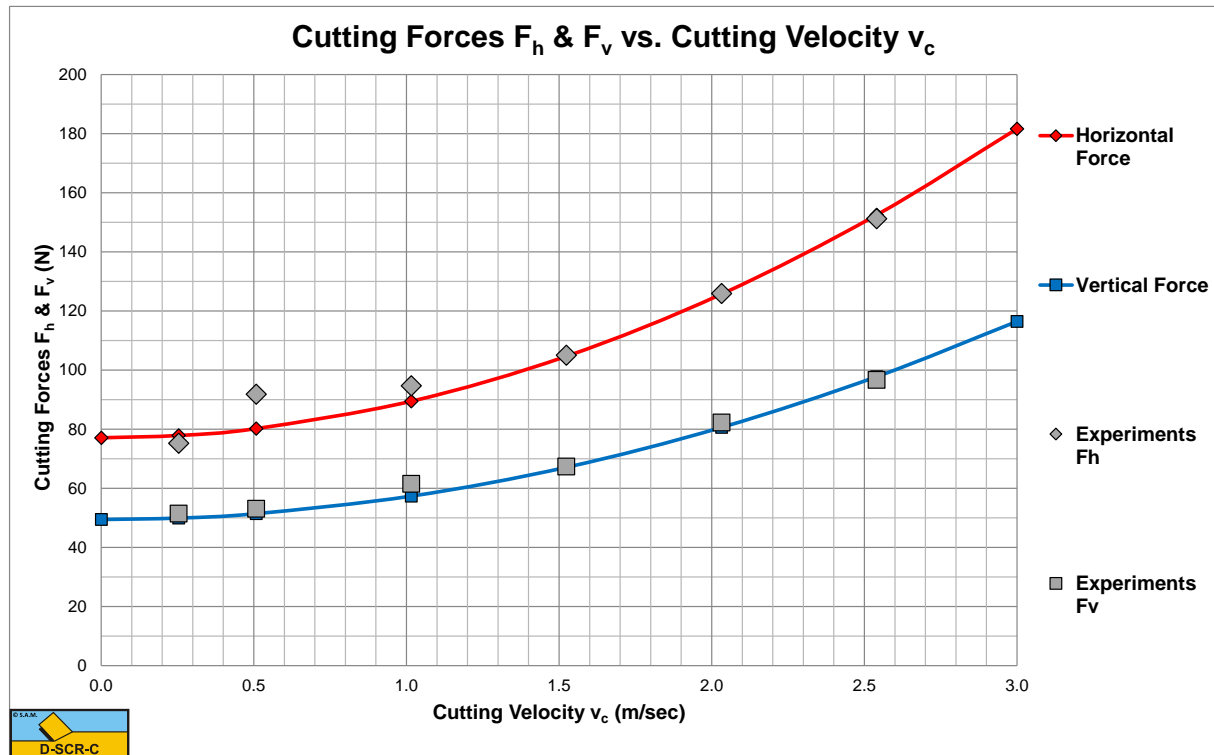
Figure 5-22: Cutting forces versus cutting velocity.
