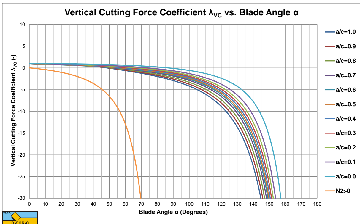
Figure V-15: The vertical cutting force coefficient \lambda_{VC} .
