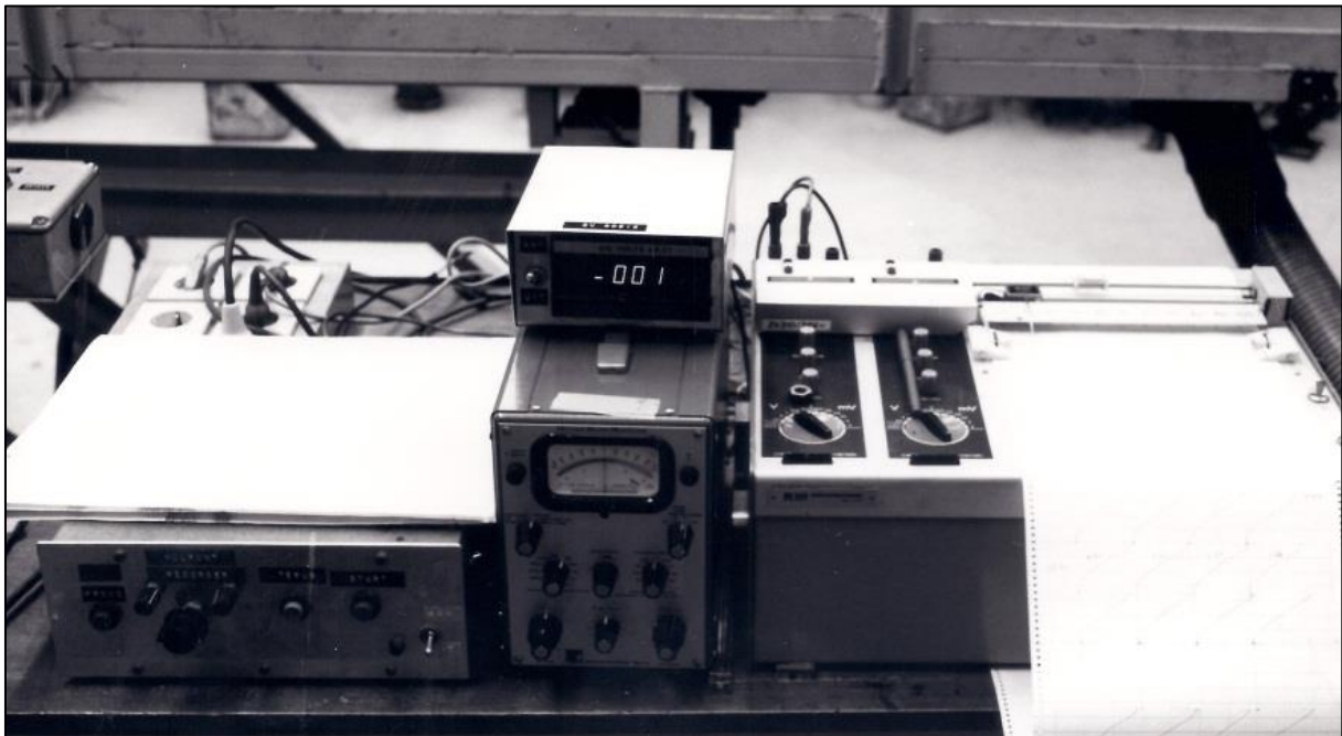
Figure 6-46: Measuring the cone resistance of the sand.
