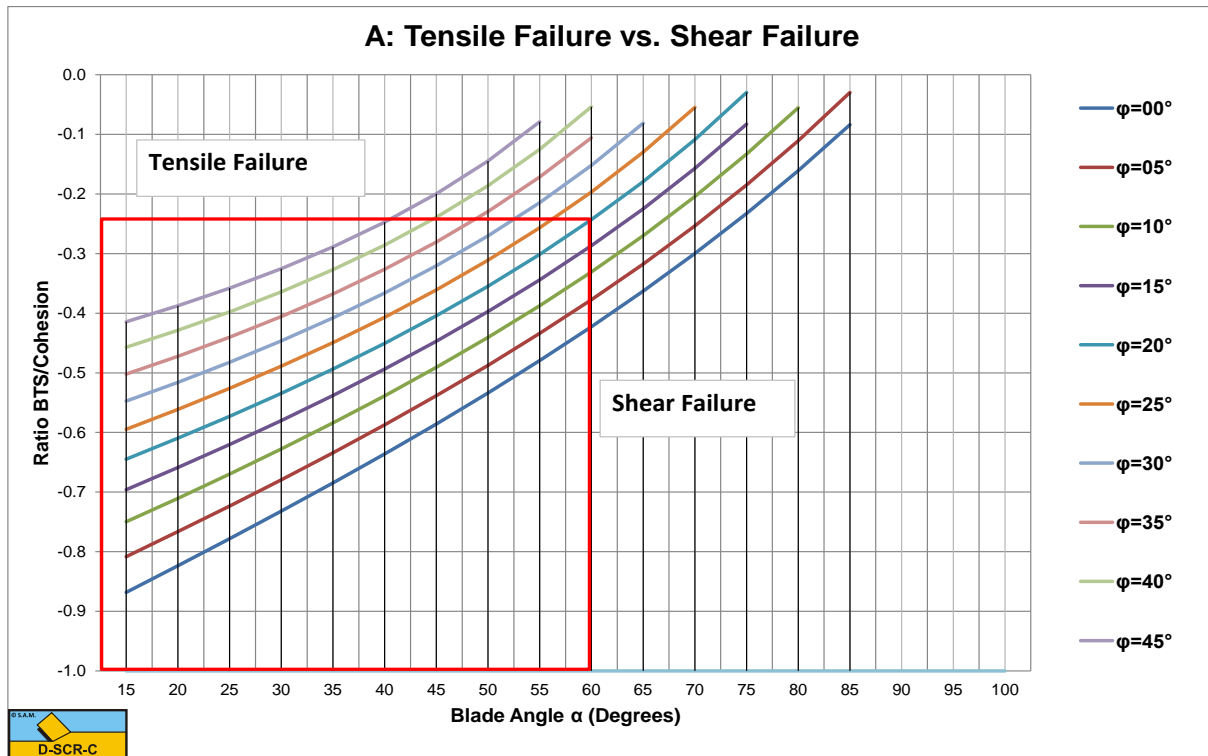
Figure 8-38: Below the lines (equation (8-125)) the cutting process is brittle (shear failure); above the lines it is brittle (tensile failure).
