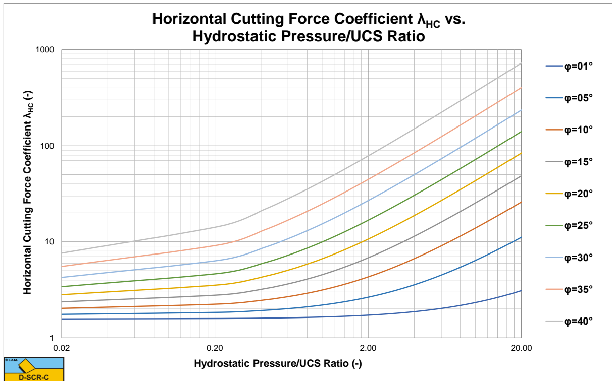
Figure X-18: The horizontal cutting force coefficient \lambda_{HC} for a 75 degree blade.
