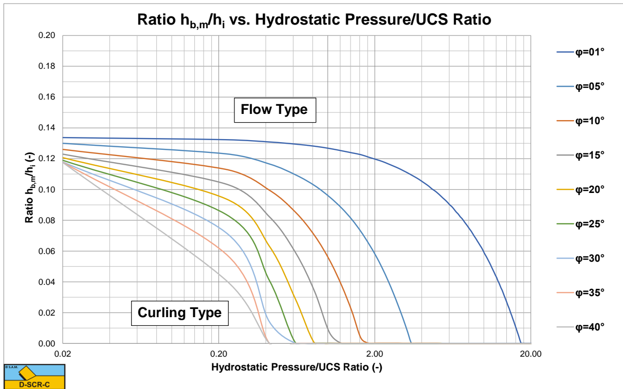
Figure X-1: The ratio h_{b,m}/h_i for a 30 degree blade.
