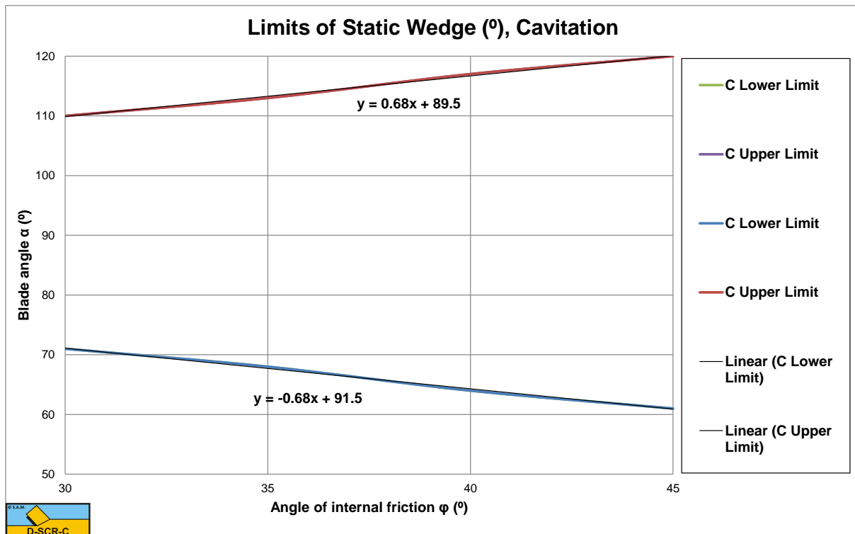
Figure 12-27: The lower and upper limit where a static wedge can exist for the cavitating cutting process.
