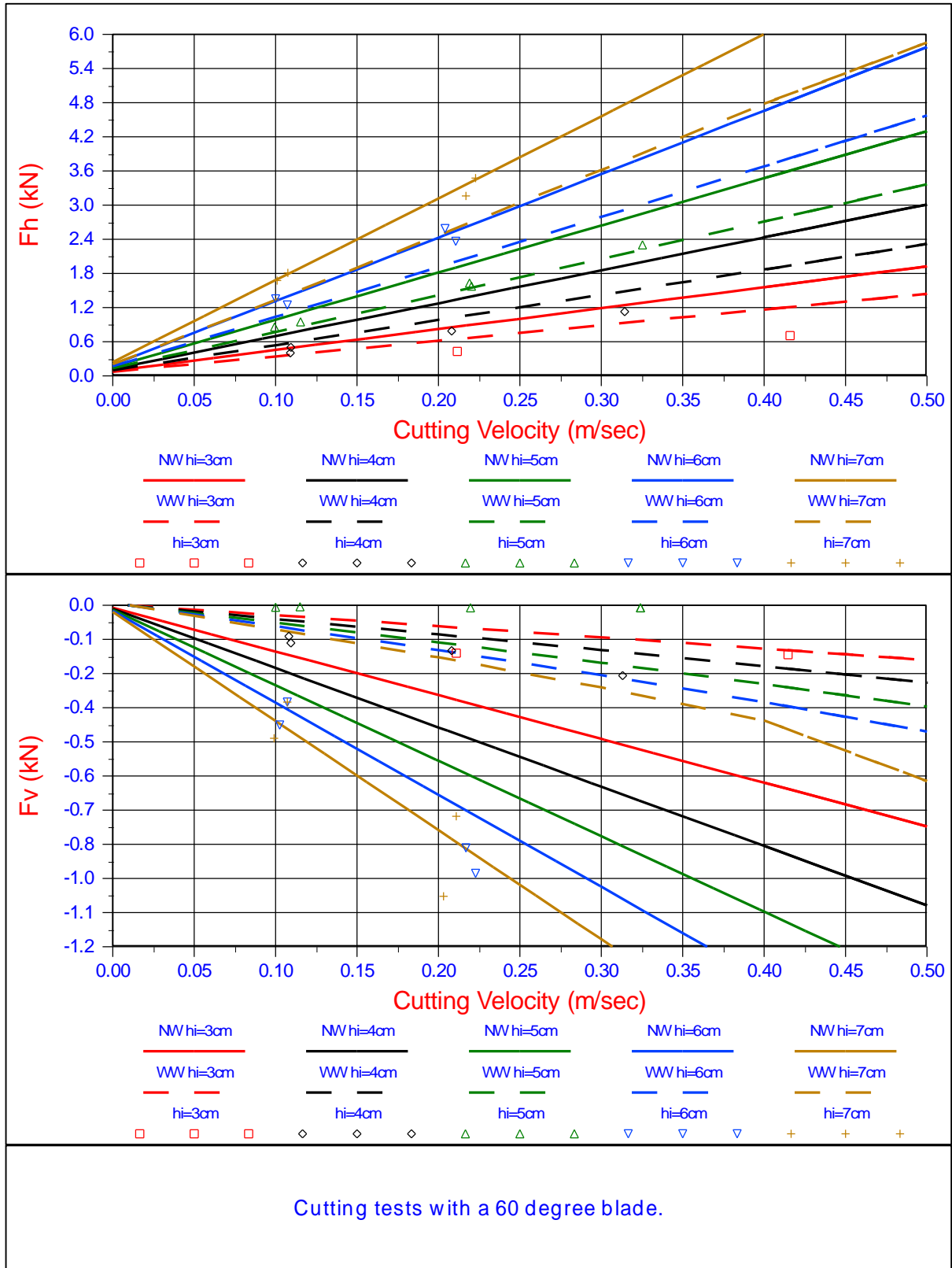
Figure 12-36: Cutting forces for cutting depths ( h_i ) from 3 to 7 cm; blade angle 60^\circ .
