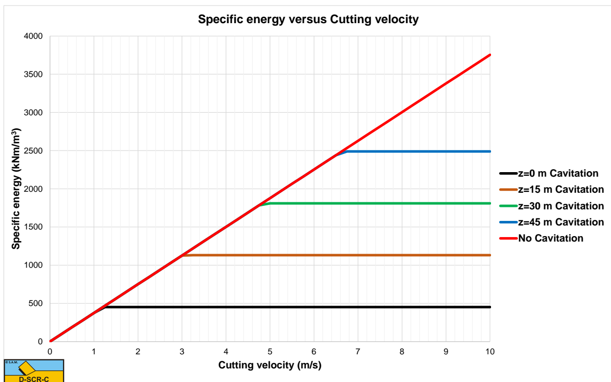
Figure 16-2: The specific energy.
