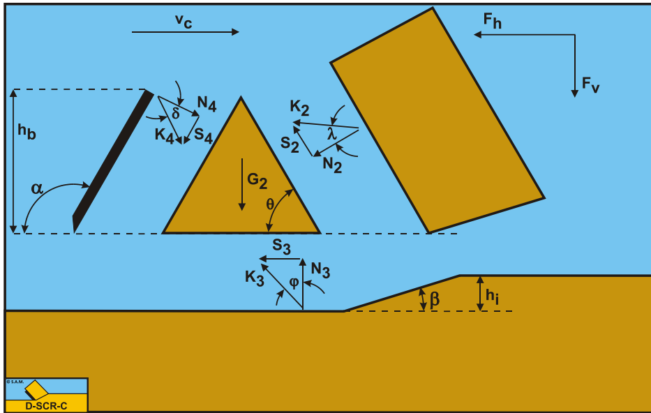
Figure 11-5: The forces on the wedge.
