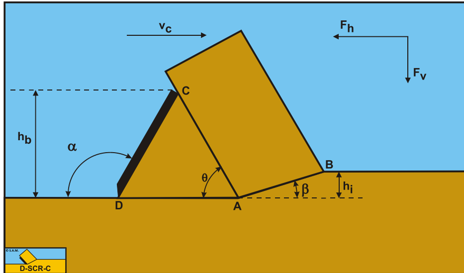
Figure 14-1: Definitions.
