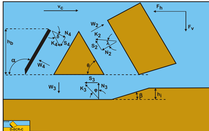
Figure 12-5: The forces on the wedge in saturated sand.
