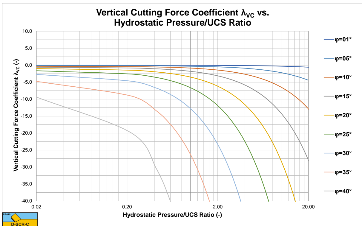
Figure X-24: The vertical cutting force coefficient \lambda_{VC} for a 90 degree blade.
