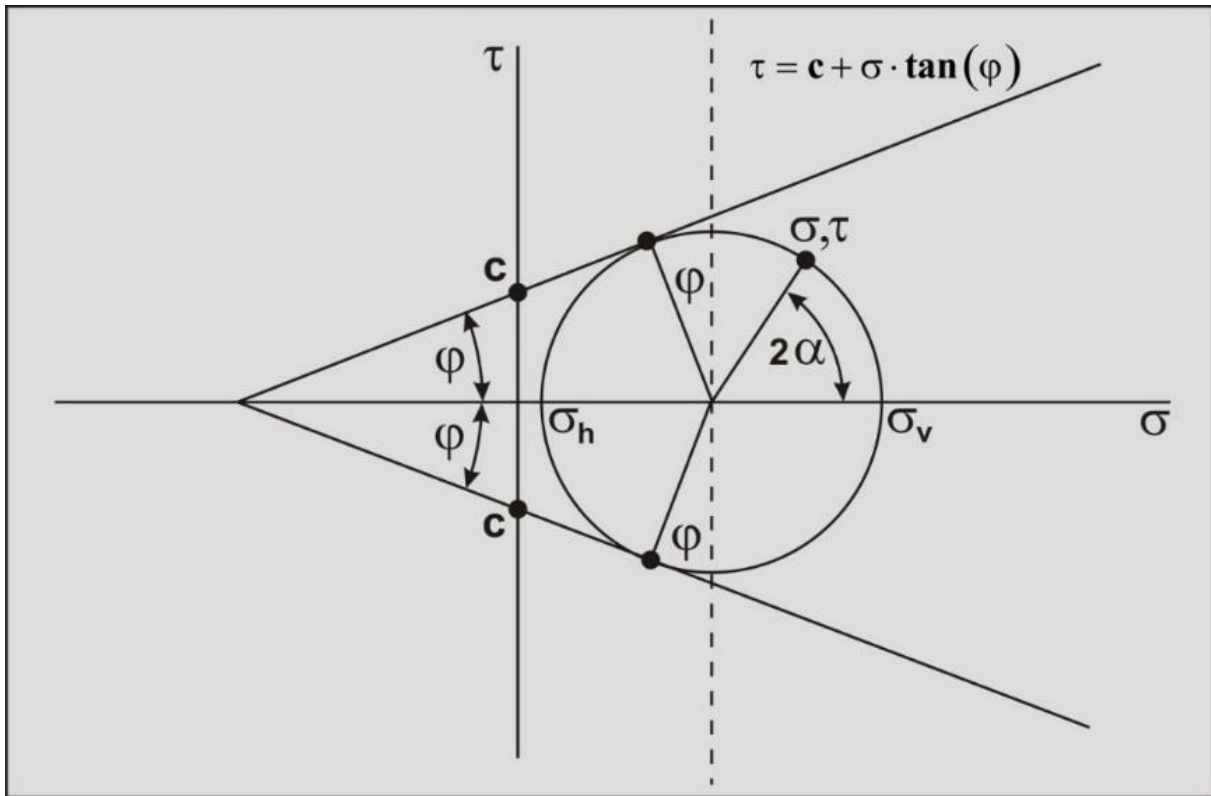
Figure 2-48: The Mohr circle for soil with cohesion.
