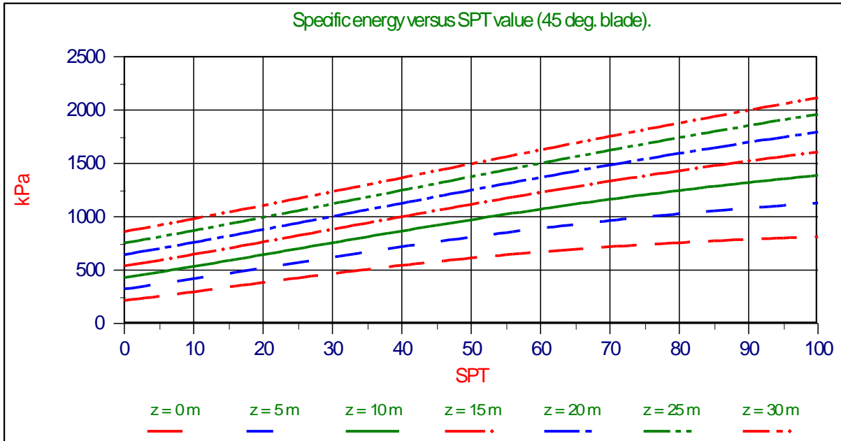
Figure 6-31: Specific energy versus SPT value (45 deg. blade).
