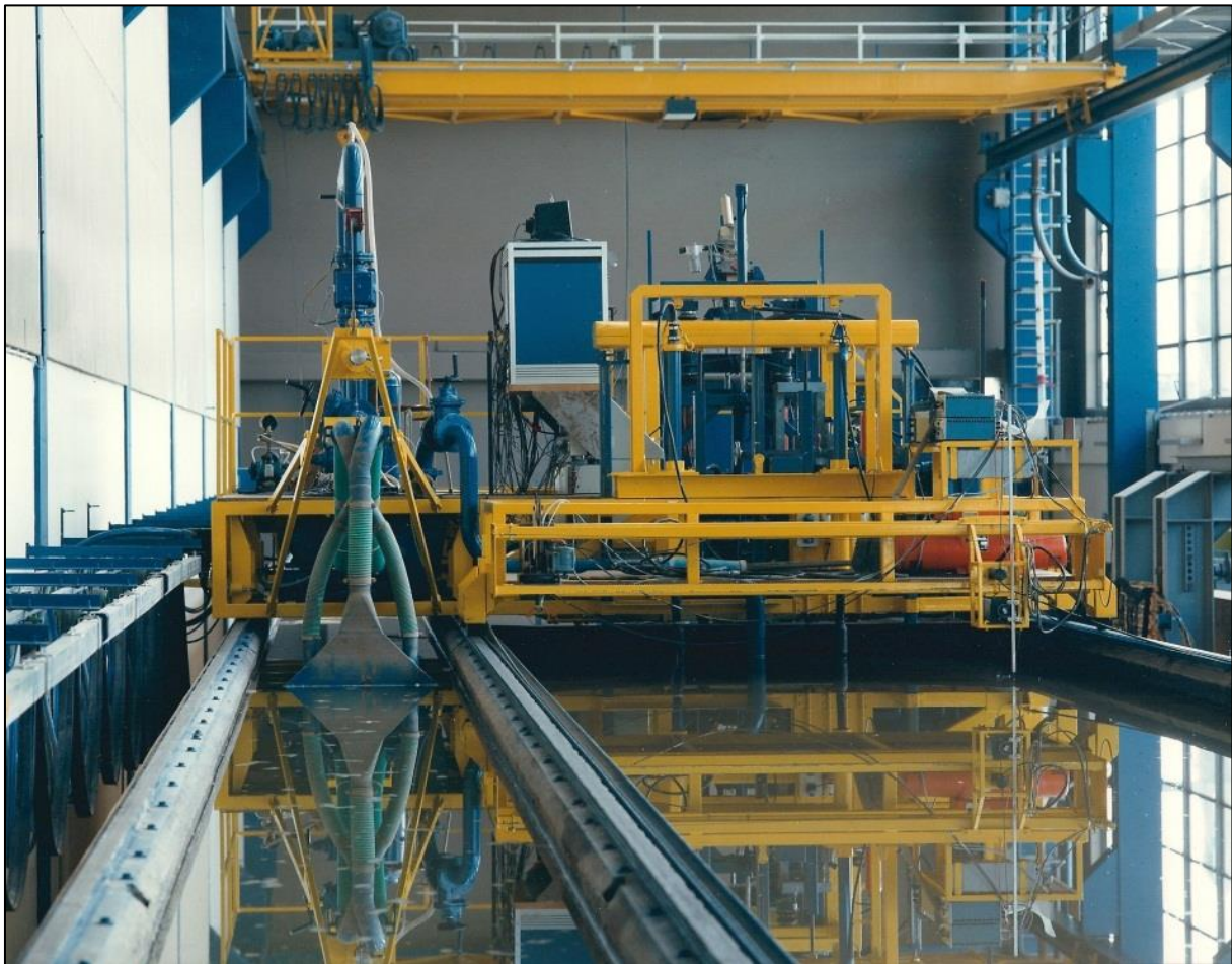
Figure 6-39: An overview of the new laboratory DE.
