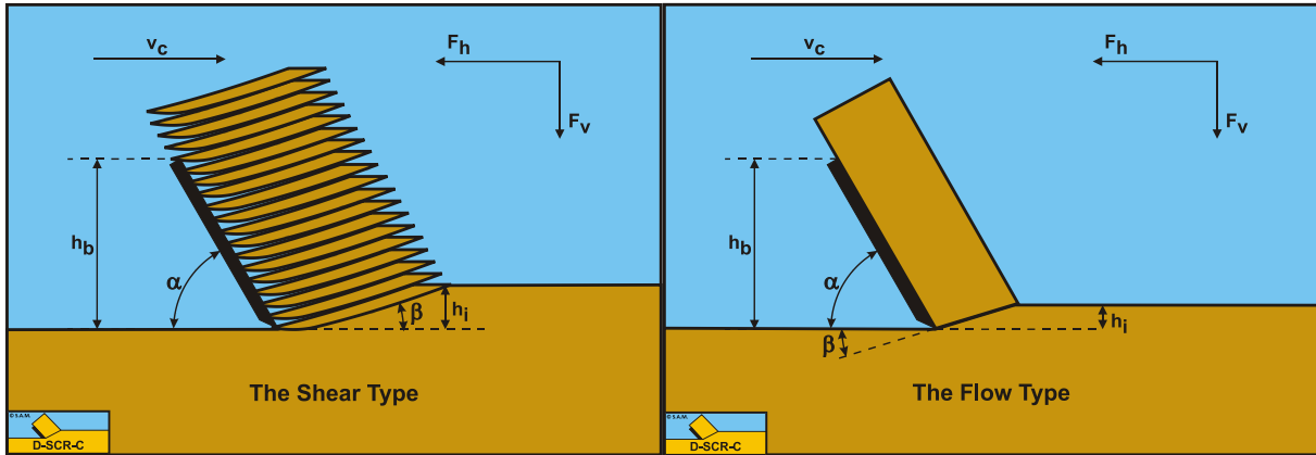
Figure 5-1: The cutting mechanism in dry sand, the Shear Type.
