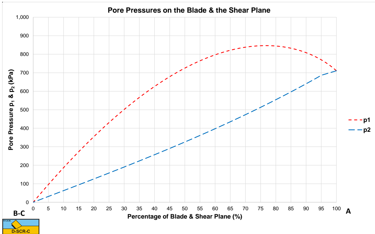
Figure 16-6: The pore pressures on blade and shear plane.
