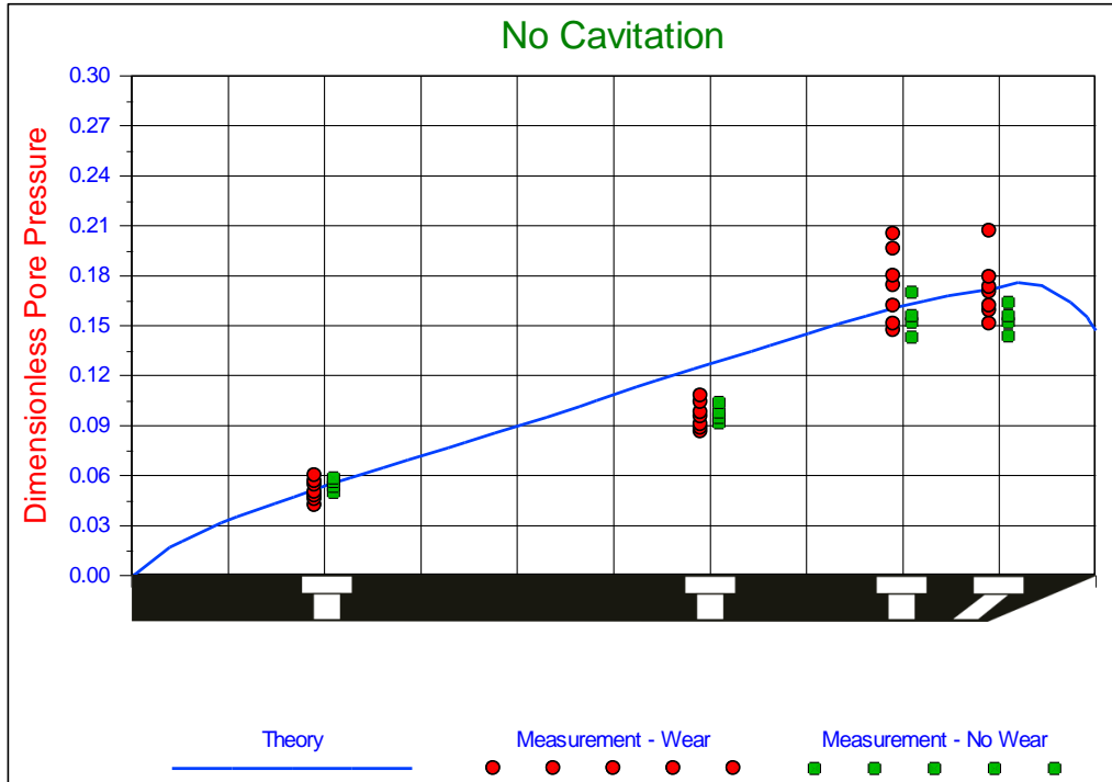
Figure M-18: \alpha=60^\circ , h_i=87 mm, h_b=173 mm.
