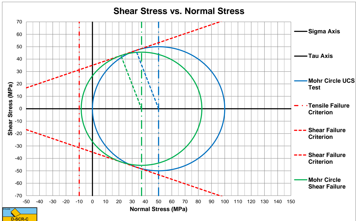
Figure 16-10: The Mohr circles with tensile strength of -10 MPa (UCS=100 MPa, \varphi=20^\circ ). Shear Failure.
