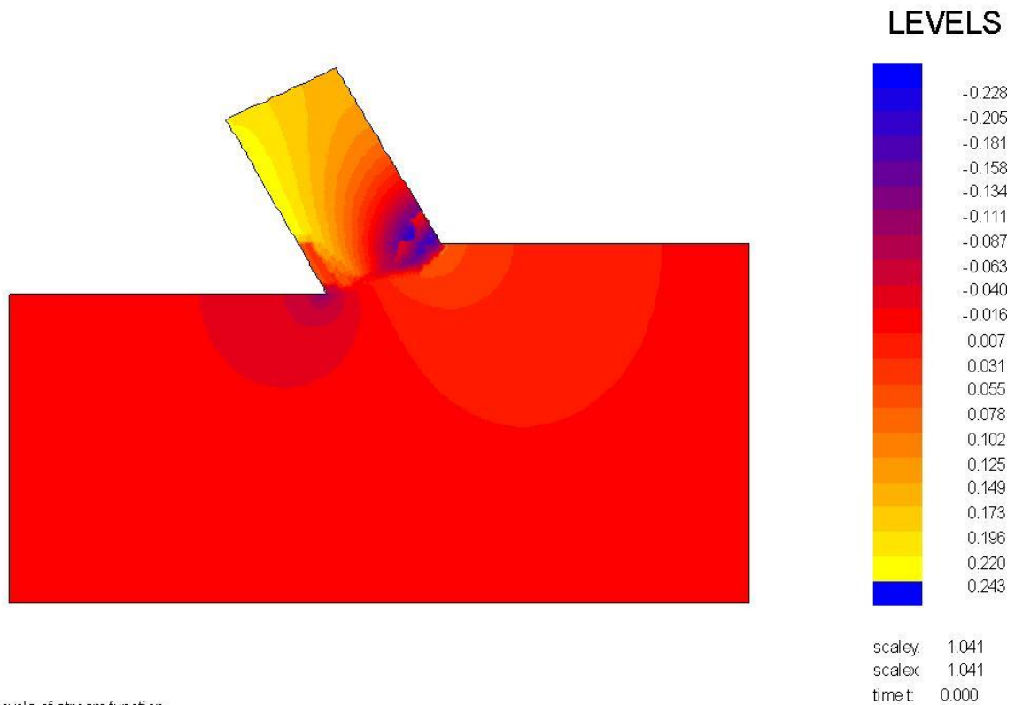
Figure S-6: The stream function in colors.
