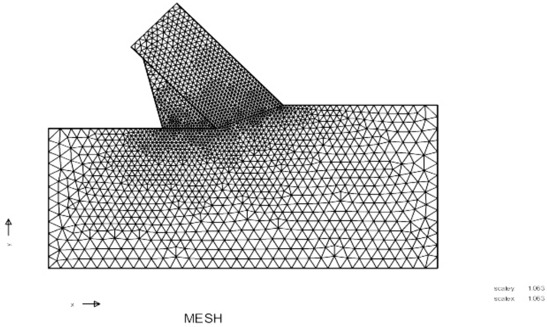
Figure S-8: The coarse mesh.
