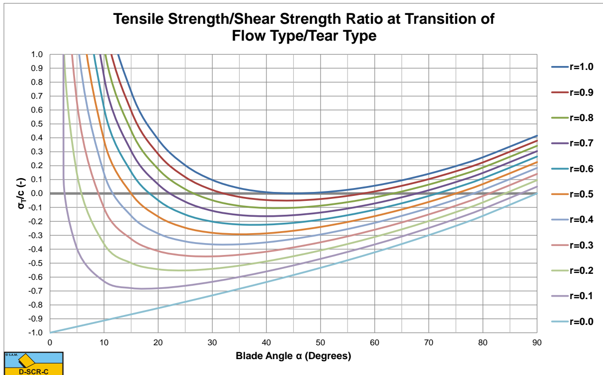
Figure 7-27: The transition Flow Type vs. Tear Type.
