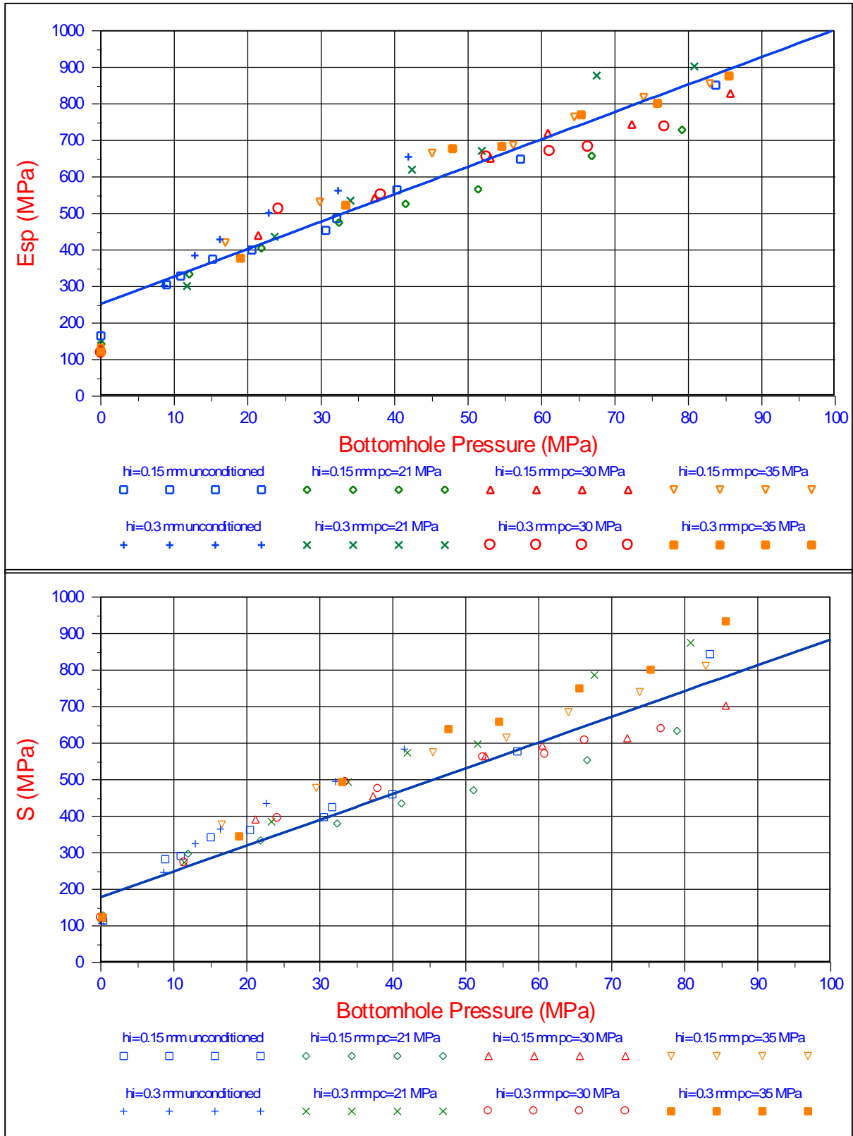
Figure 9-23: The specific energy E_{sp} and the drilling strength S , theory versus the Zijlsling (1987) experiments.
