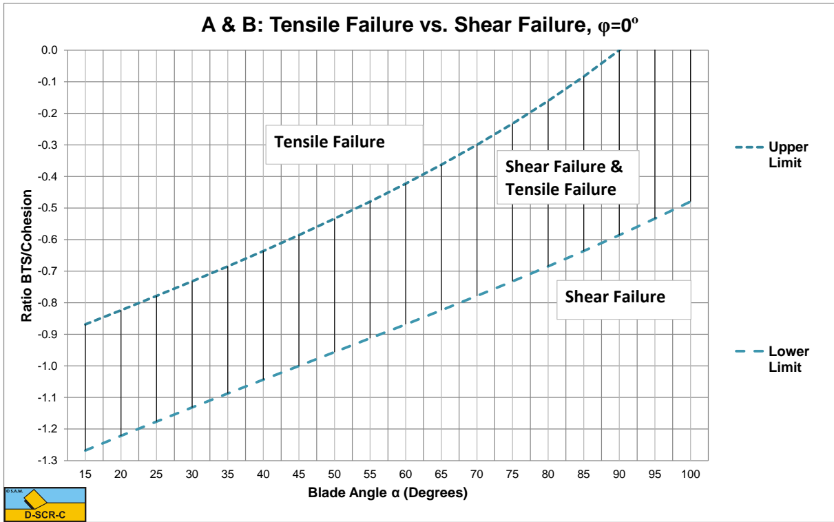
Figure W-11: The tensile/shear failure range based on BTS/Cohesion for \phi=0^\circ .
