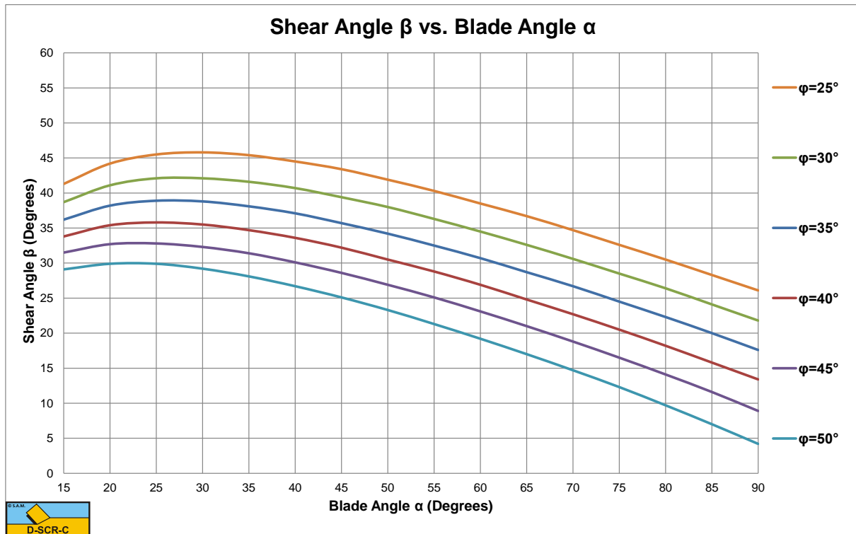
Figure 5-10: The shear angle \beta as a function of the blade angle \alpha for h_b/h_i=2 .
