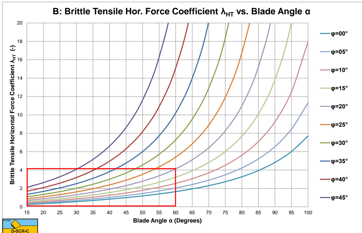
Figure 8-45: The brittle (tensile failure) horizontal force coefficient \lambda_{HT} .
