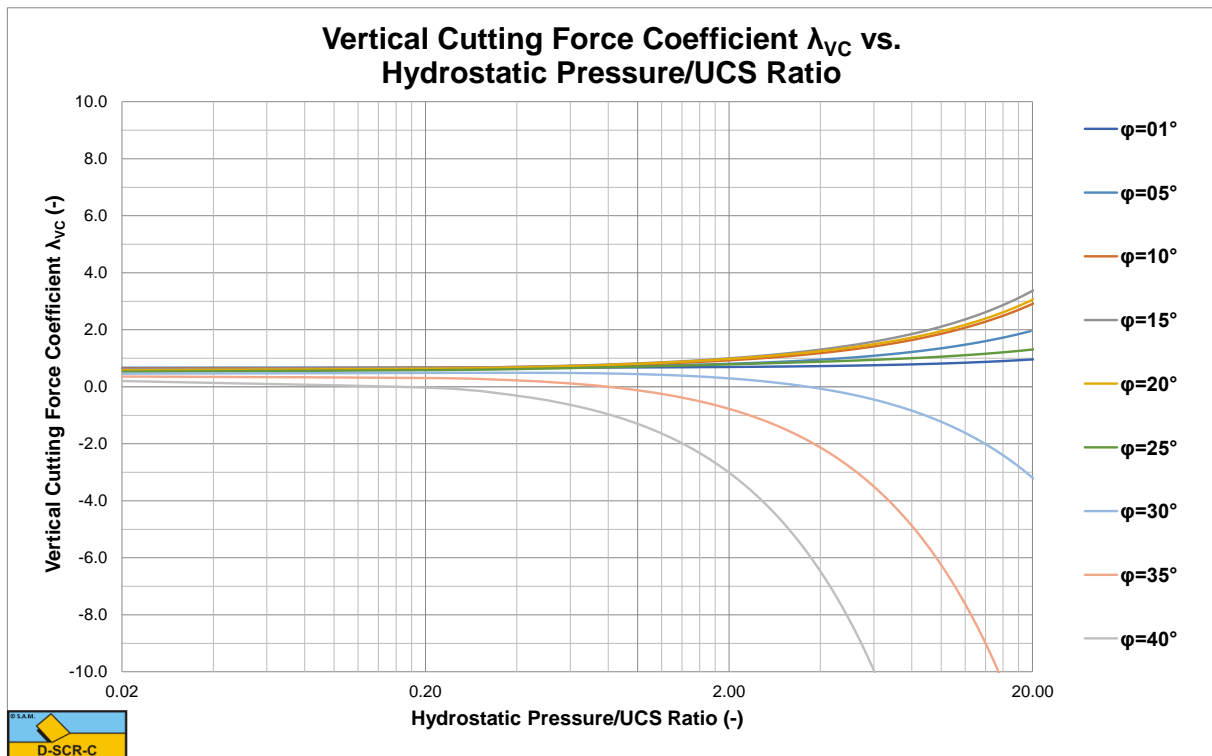
Figure X-14: The vertical cutting force coefficient \lambda_{VC} for a 60 degree blade.
