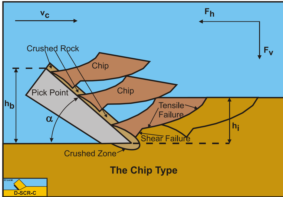
Figure 8-3: The Chip Type.
