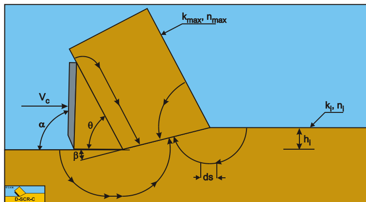
Figure 12-8: Possible flow lines.
