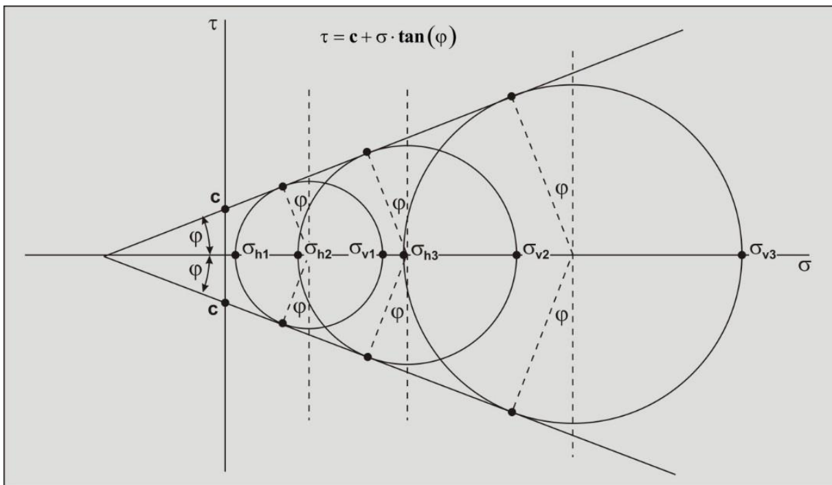
Figure 2-49: Determining the angle of internal friction from tri-axial tests of soil with cohesion.
