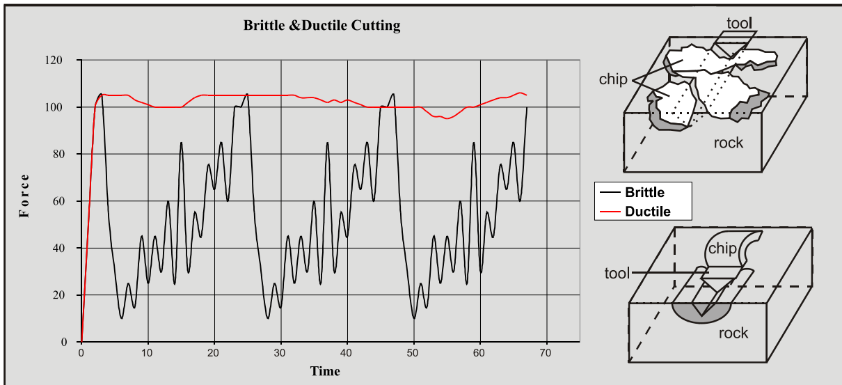
Figure 8-1: Ductile and brittle cutting Verhoef (1997).
