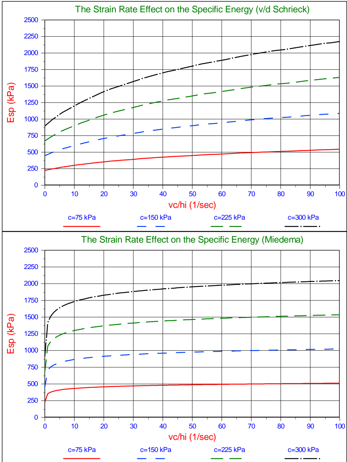
Figure 7-17: Comparison of the model developed with the v/d Schrieck (1996) model.
