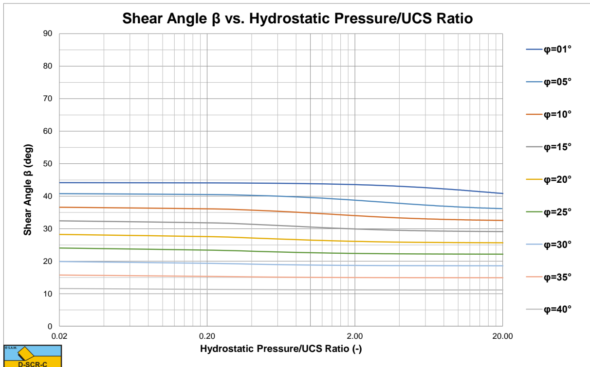
Figure X-22: The shear angle \beta for a 90 degree blade.
