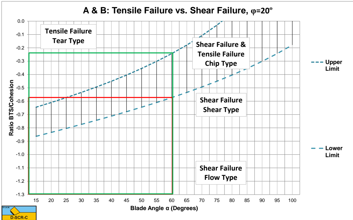
Figure 8-53: The tensile vs. shear failure range based on the BTS to cohesion ratio.
