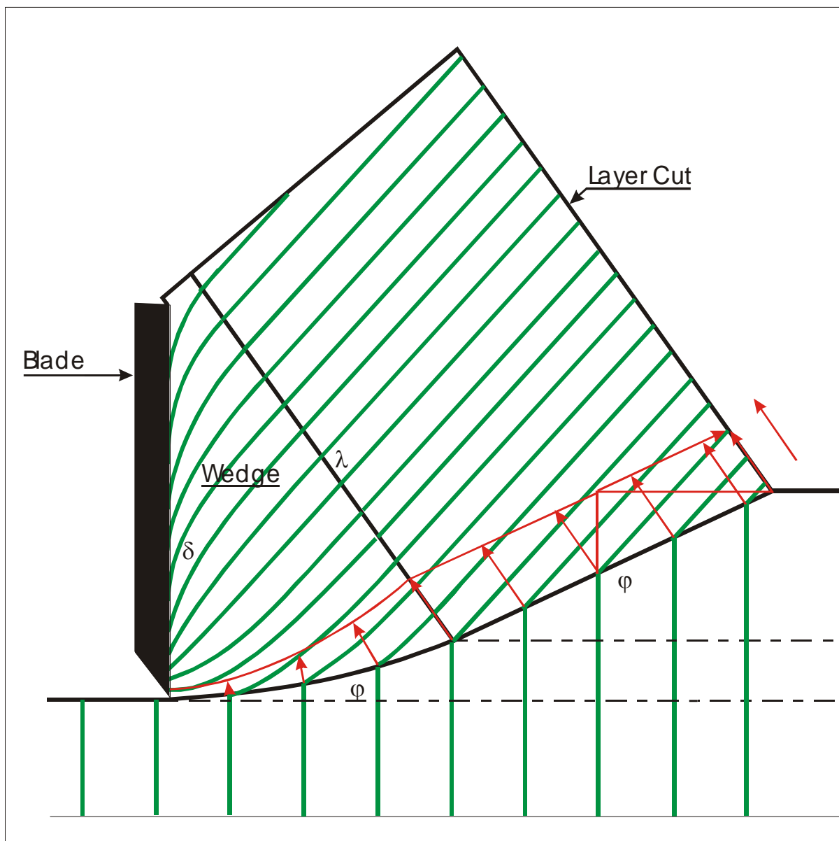
Figure 12-39: The dynamic wedge.
