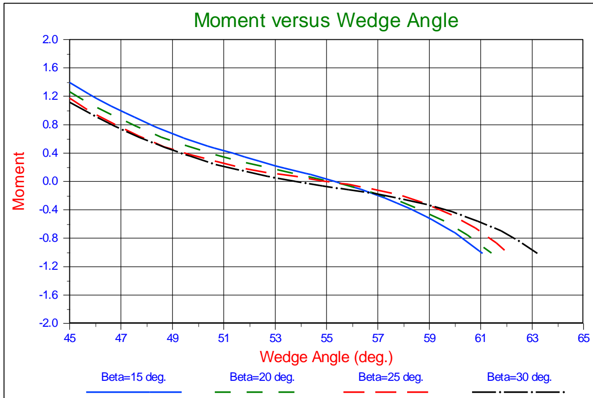
Figure 12-19: Moment versus wedge angle \theta by using polynomial regression for: \alpha=90^\circ ; \beta=15^\circ, 20^\circ, 25^\circ, 30^\circ ; \delta=28^\circ ; \varphi=42^\circ ; h_i=1 ; h_b=3 ; k_i/k_{max}=0.25
