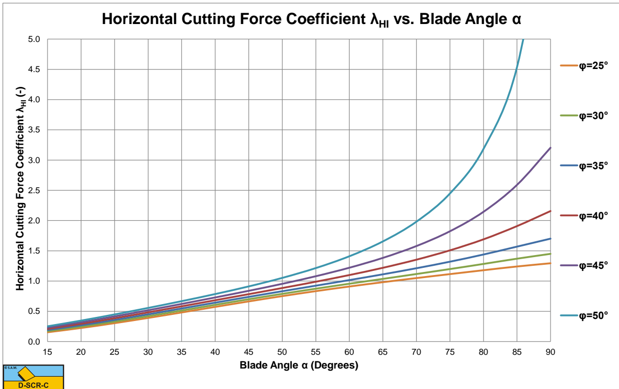
Figure 5-16: The horizontal cutting force coefficient \lambda_{HI} .
