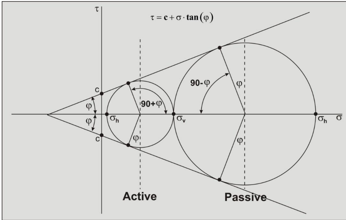
Figure 2-58: The Mohr circles for active and passive failure for a soil with cohesion.
