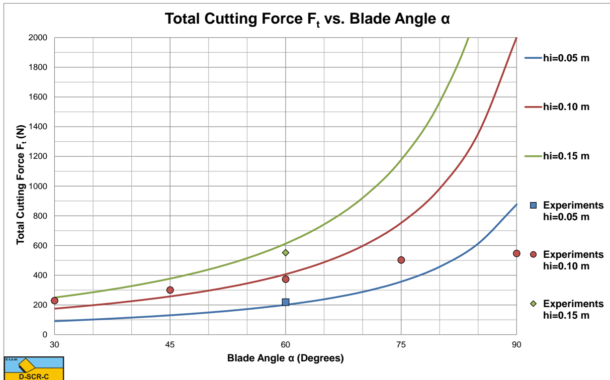
Figure 5-20: The total cutting force versus the blade angle.
