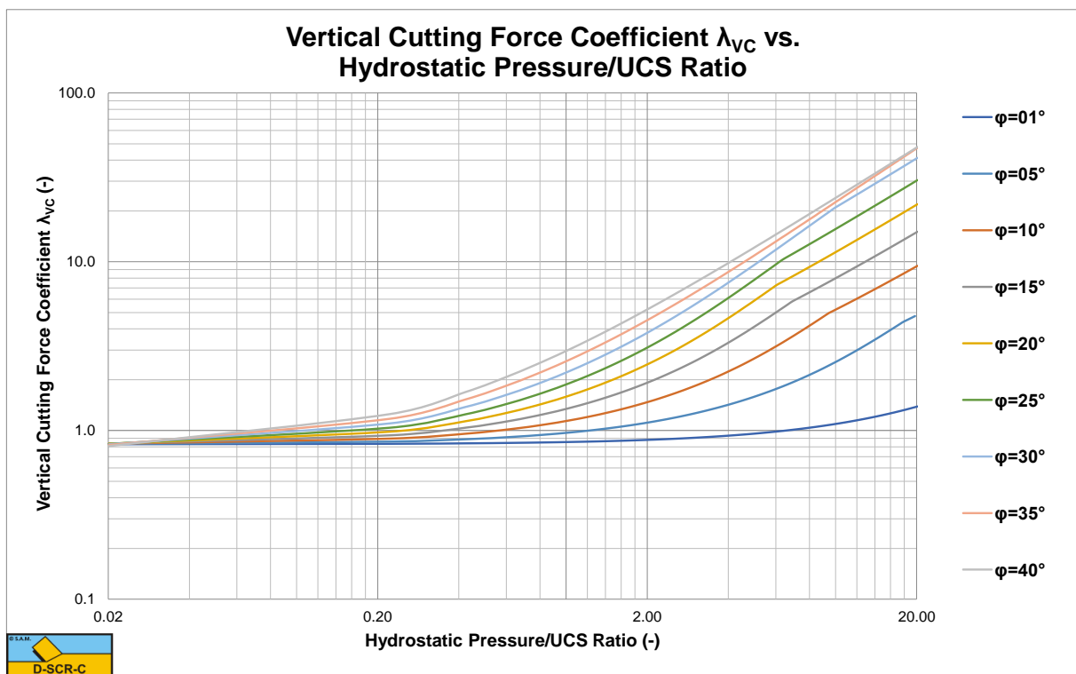
Figure X-9: The vertical cutting force coefficient \lambda_{VC} for a 60 degree blade.
