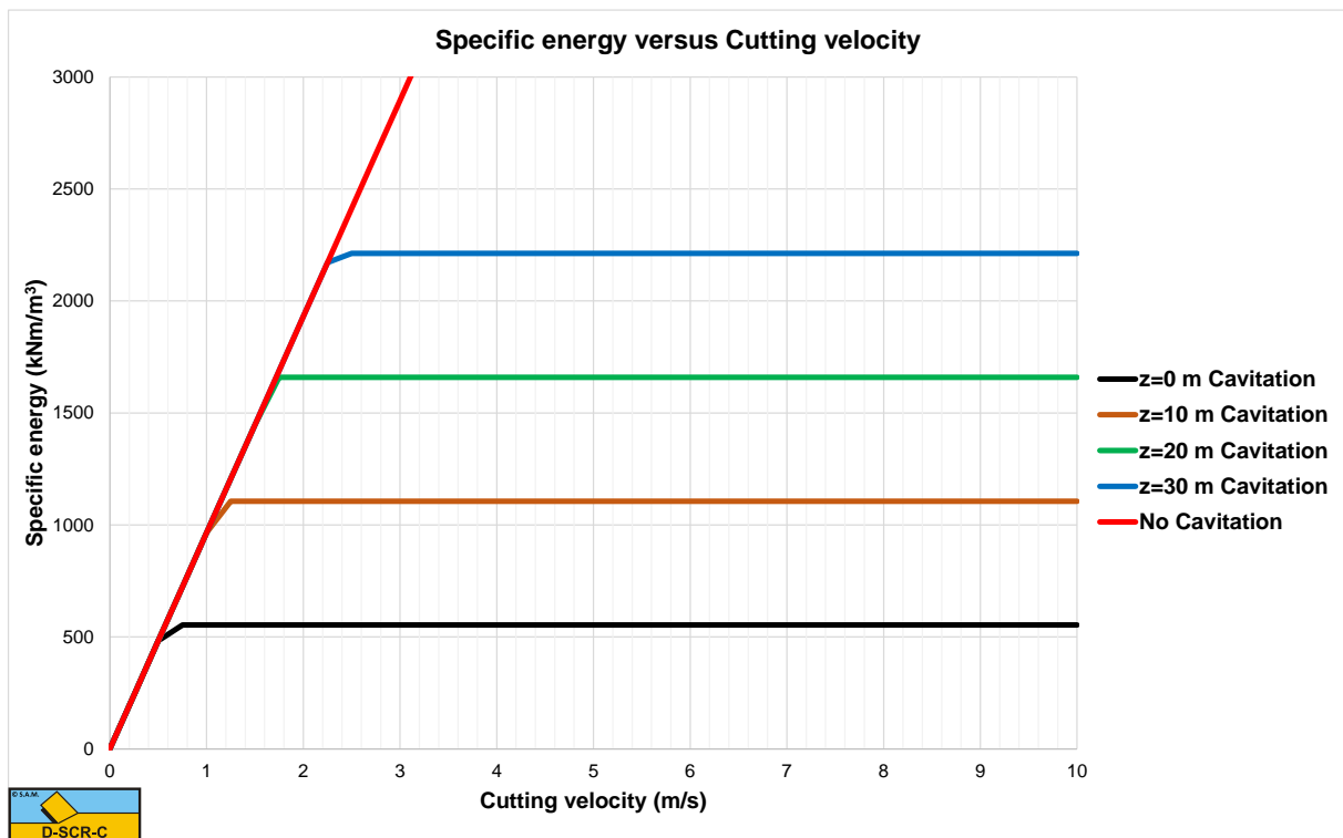
Figure 16-5: The specific energy.
