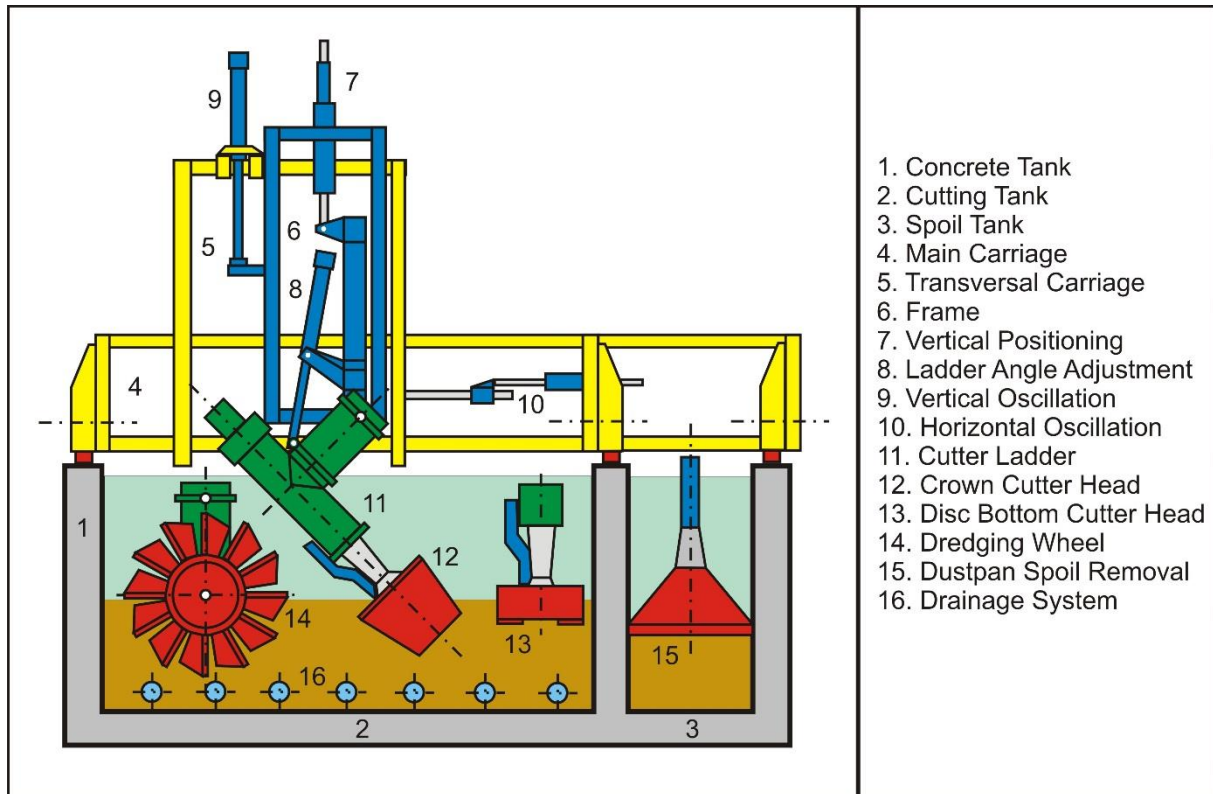
Figure 6-37: The cross section of the new laboratory DE.
