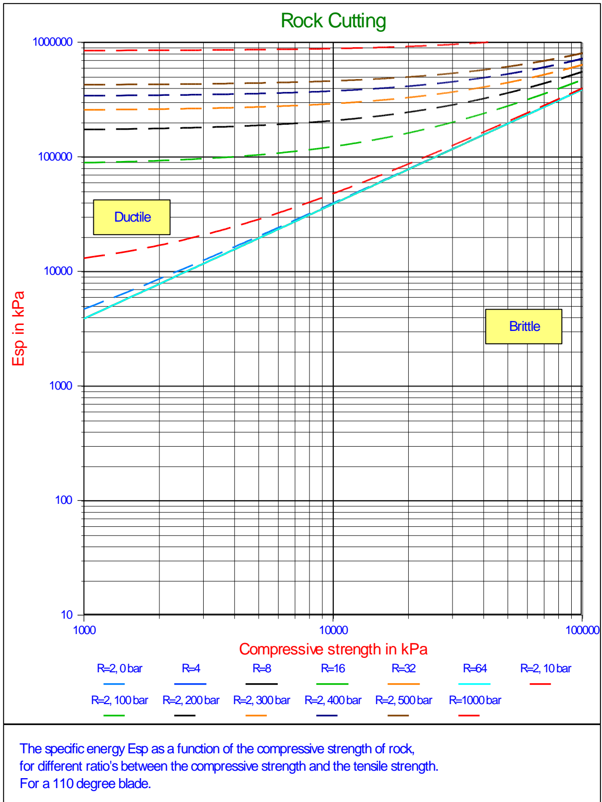
Figure 9-29: The specific energy E_{sp} in rock versus the compressive strength (UCS) for a 110° blade.
