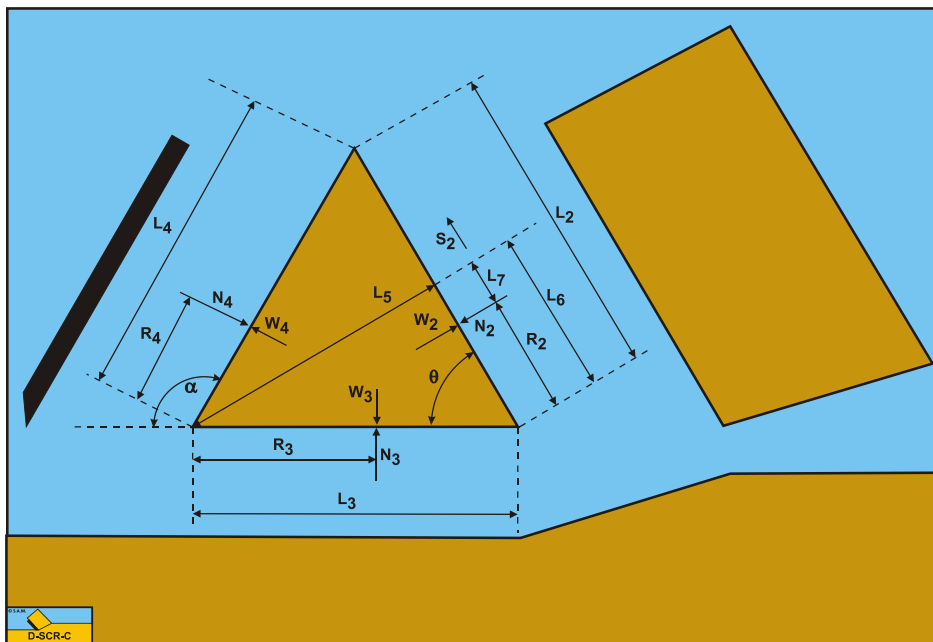
Figure 12-18: The equilibrium of moments on the wedge in water saturated sand.
