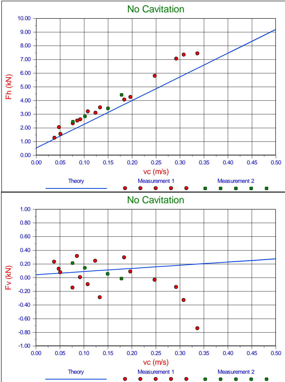
Figure M-28: \alpha=60^\circ , h_i=173 mm, h_b=173 mm.
