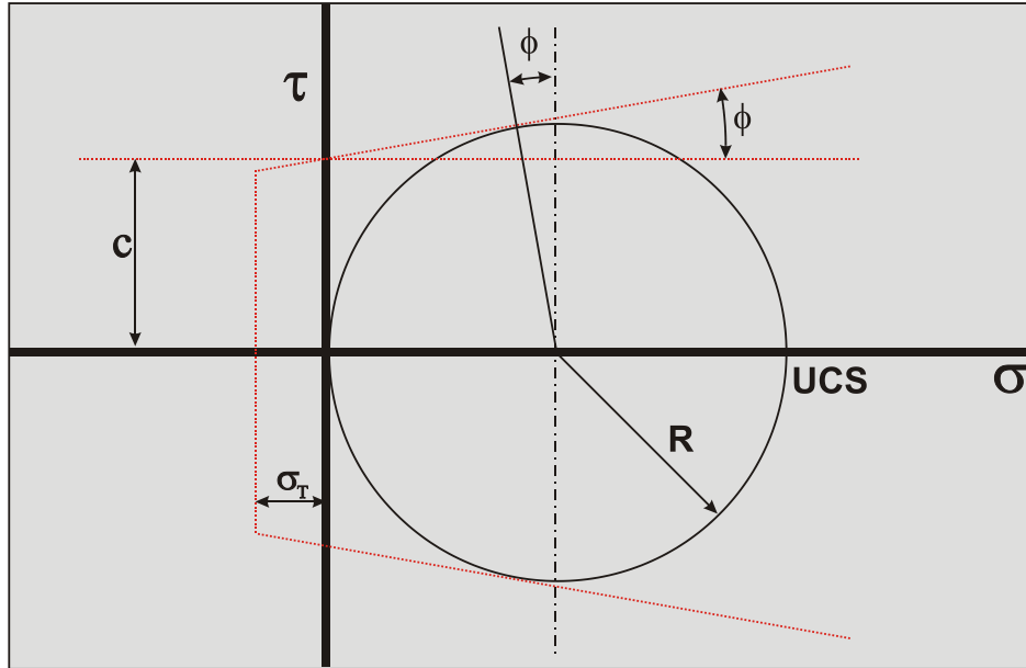
Figure 8-36: The Mohr circle for UCS and cohesion.
