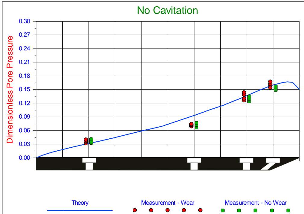
Figure M-14: \alpha=45^\circ , h_i=70 mm, h_b=141 mm.
