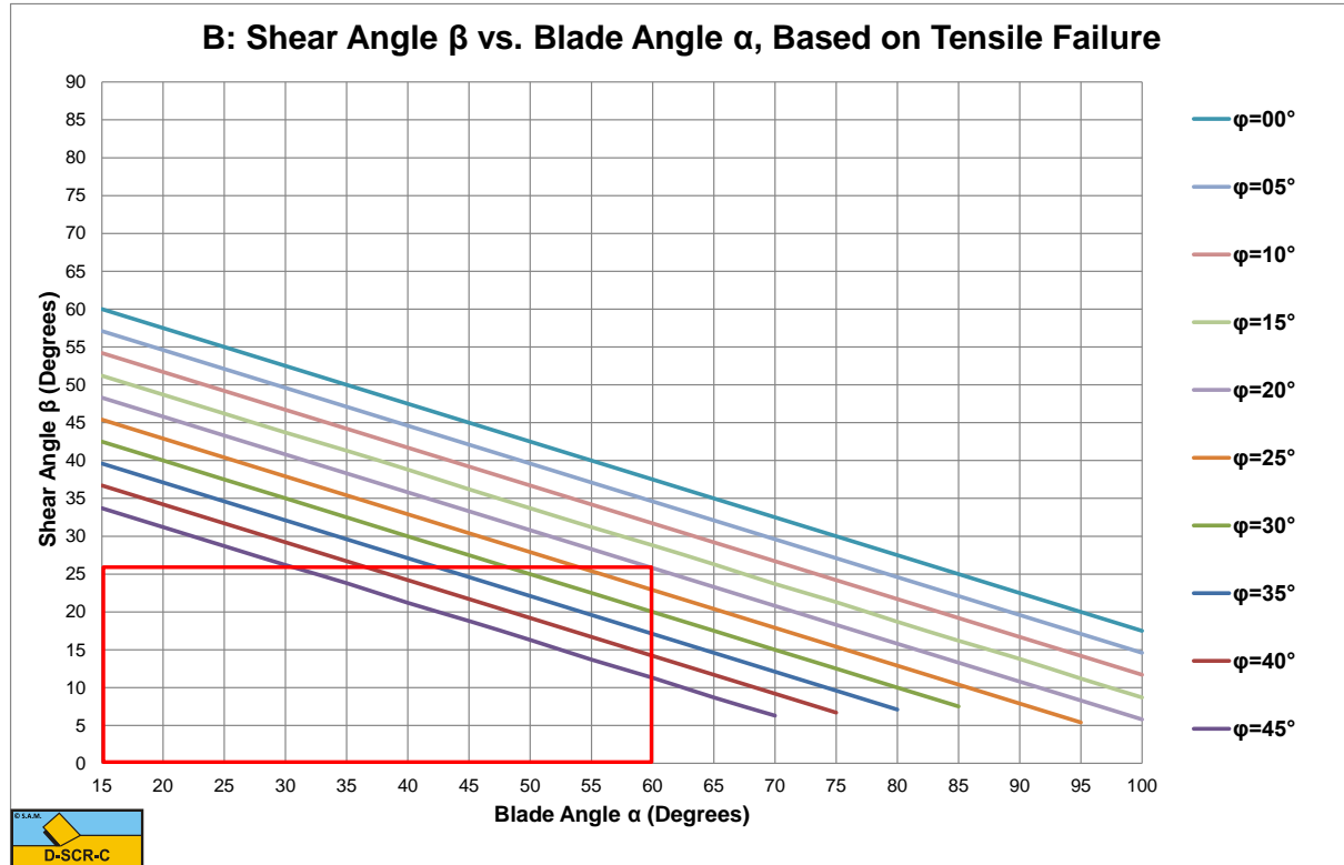
Figure 8-44: The shear angle \beta as a function of the blade angle \alpha and the internal friction angle \phi .
