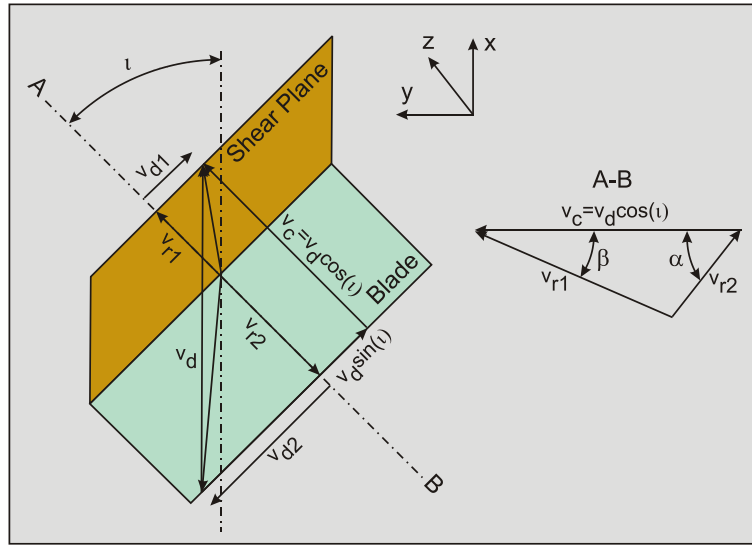
Figure 3-17: Velocity conditions.
