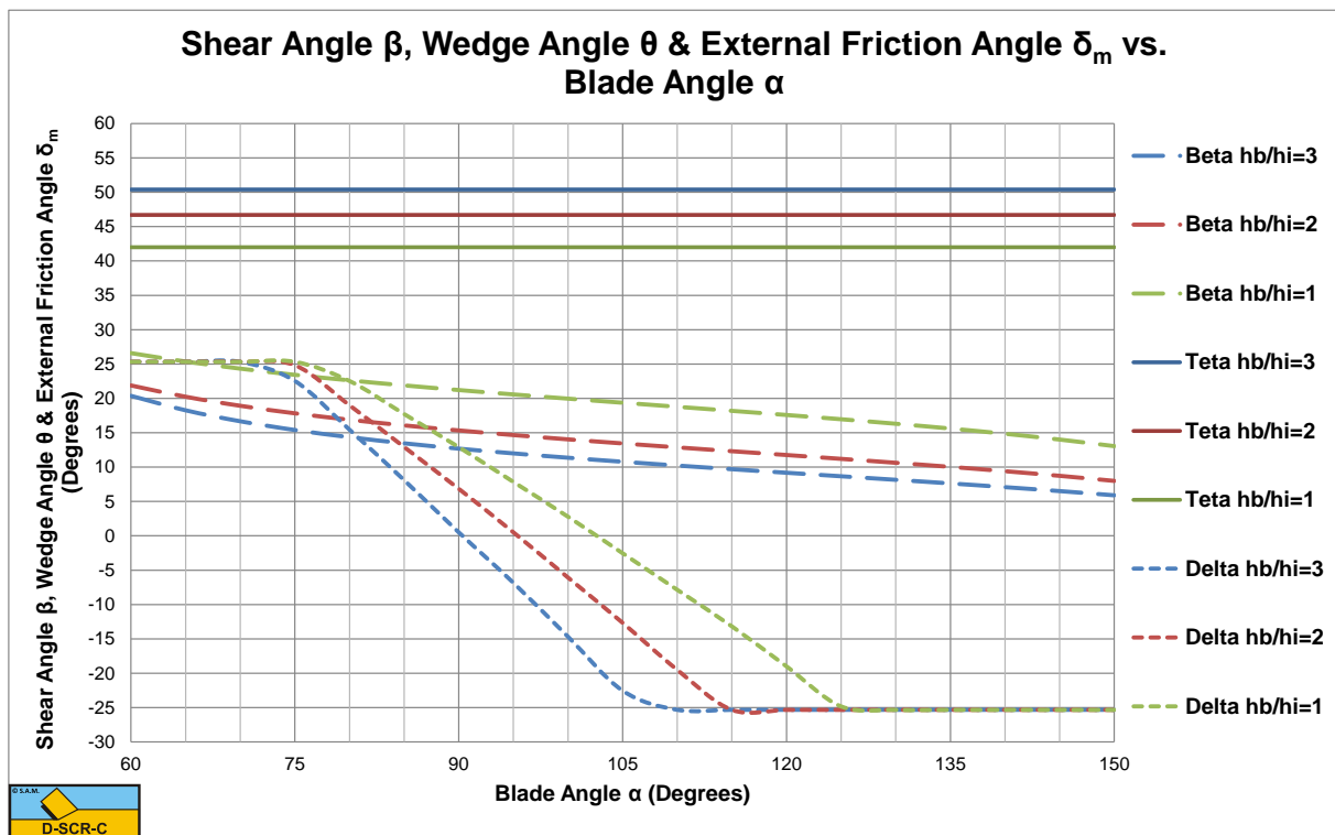
Figure 11-8: The shear angle, wedge angle and mobilized external friction angle calculated with wedge.
