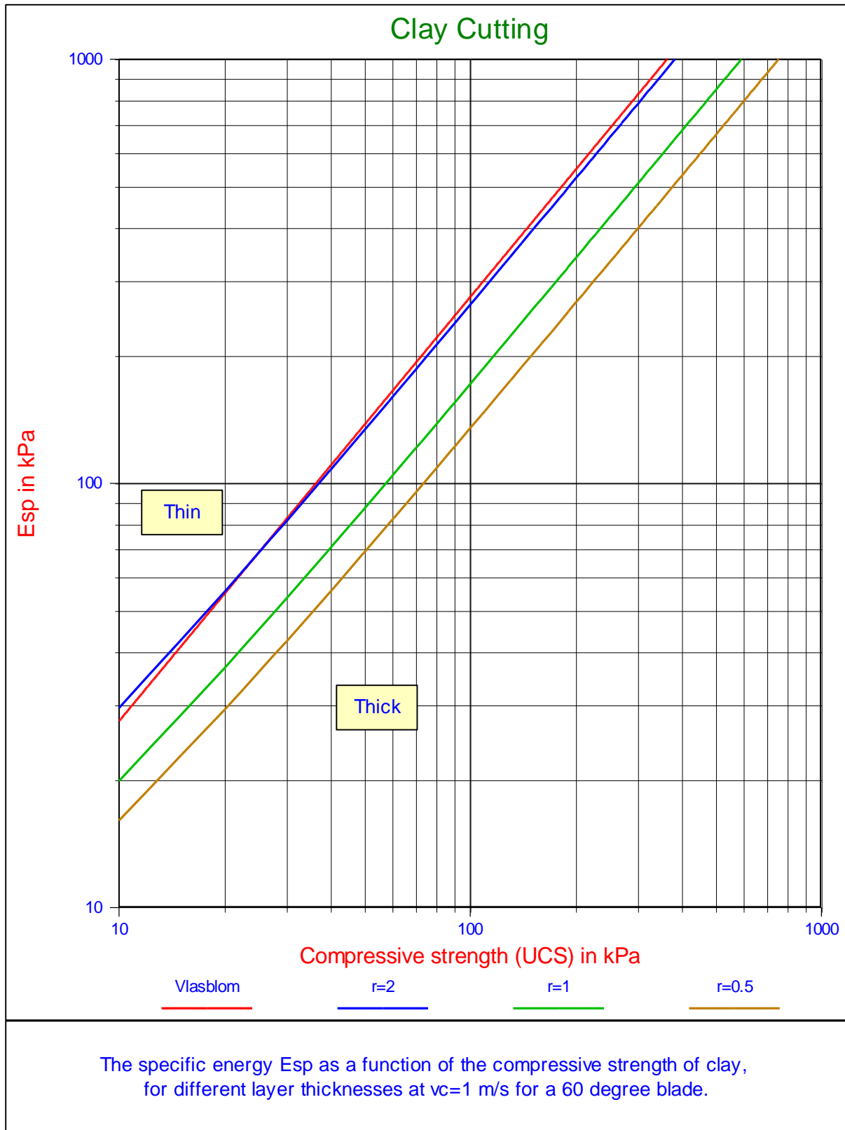
Figure 7-43: The specific energy E_{sp} in clay as a function of the compressive strength (UCS).
