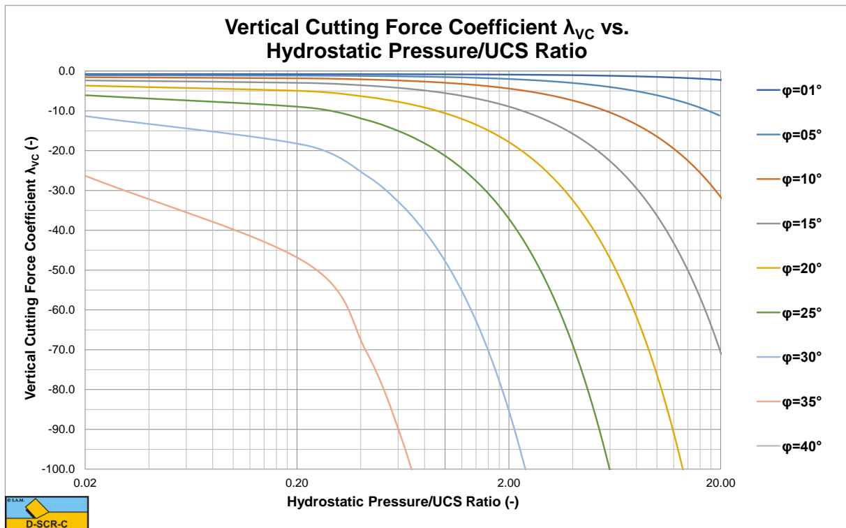
Figure X-29: The vertical cutting force coefficient \lambda_{VC} for a 105 degree blade.
