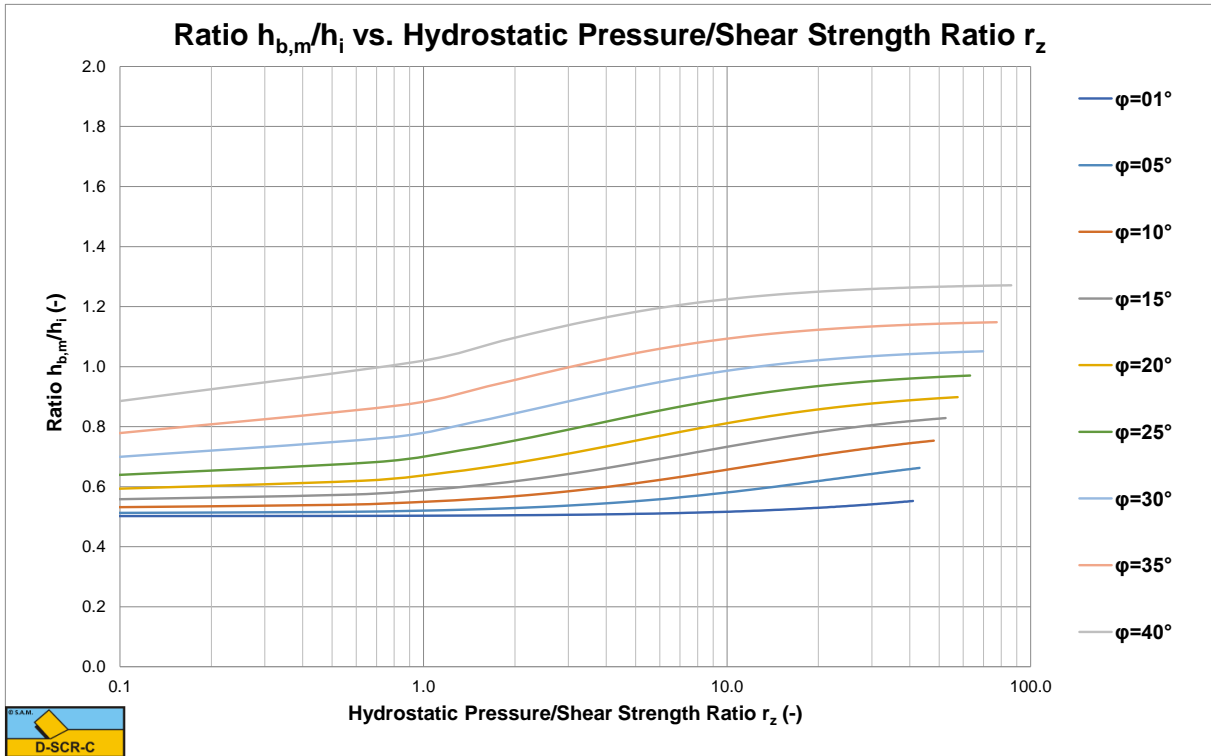
Figure 9-17: The ratio h_{b,m}/h_i for a 60 degree blade.
