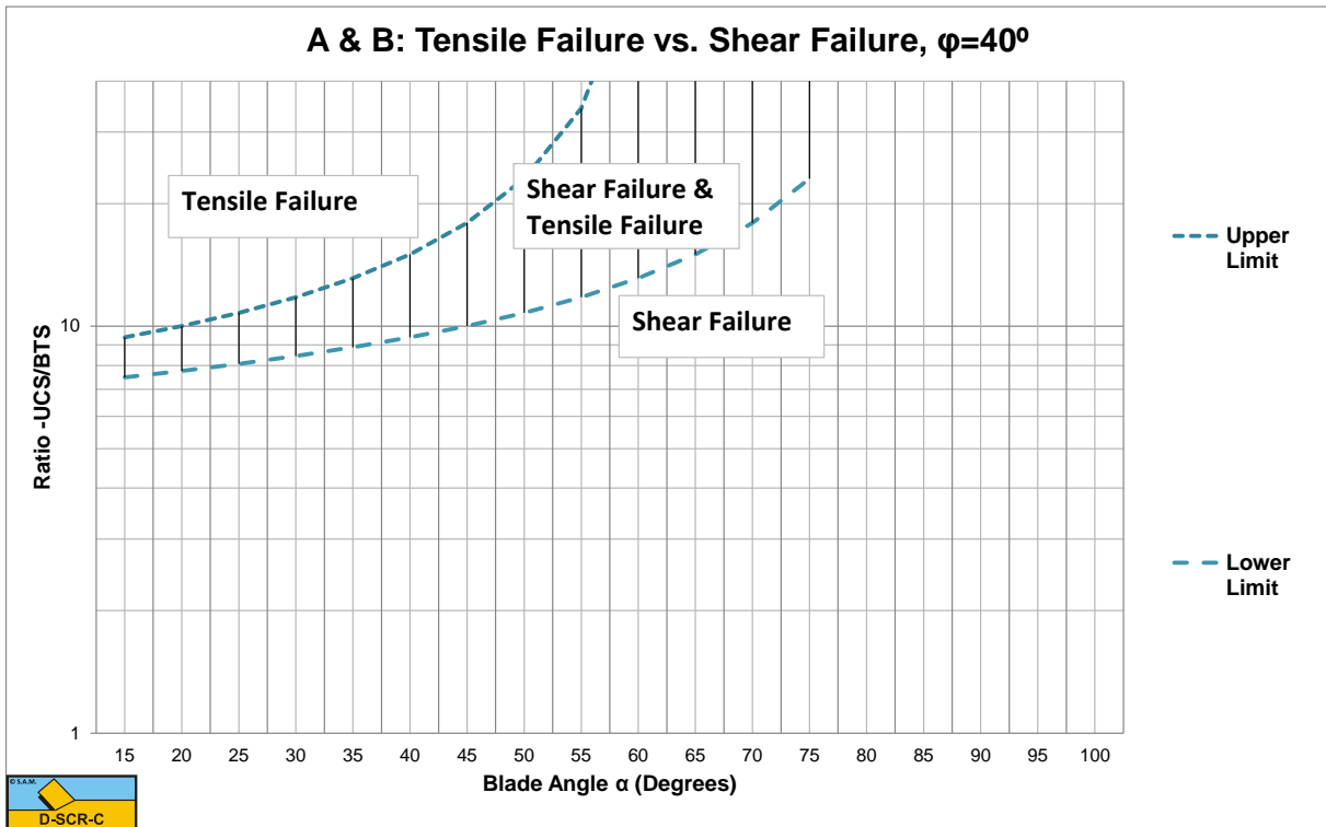
Figure W-28: The tensile/shear failure range based on UCS/BTS for \phi=40^\circ .
