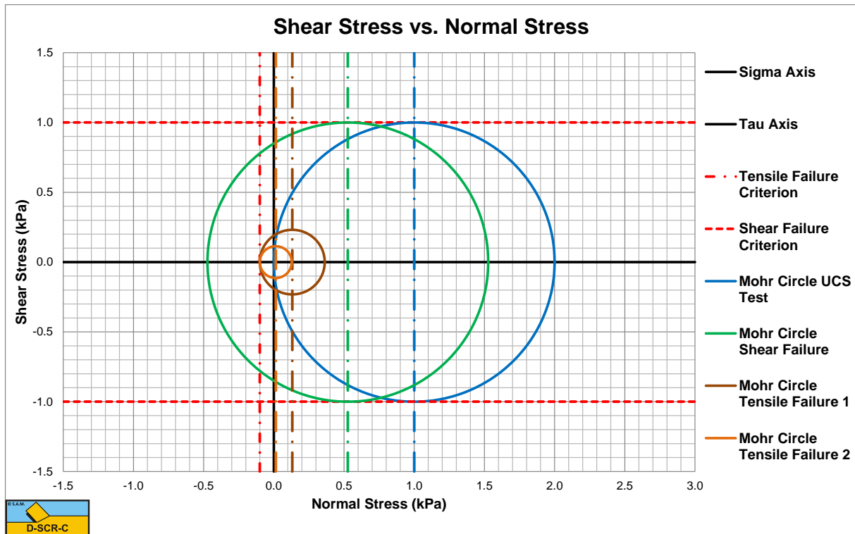
Figure 16-7: The Mohr circles.
