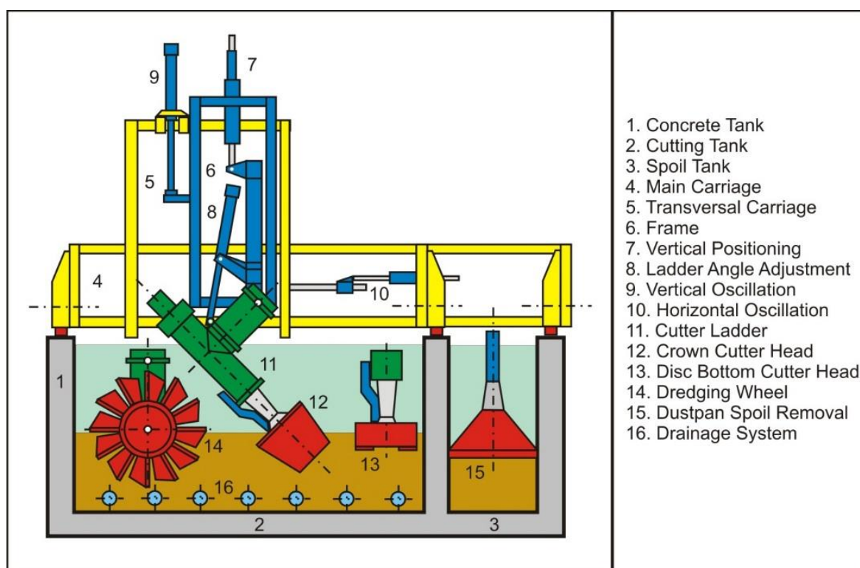
Figure 12-29: Cross section of the cutting tank.
