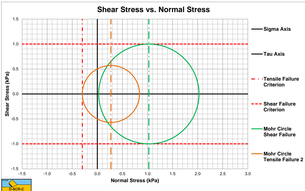
Figure 7-41: The Mohr circles for h_i=0.1 m, two possibilities.
