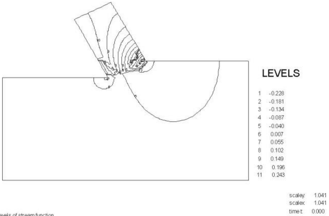
Figure S-5: The flow lines or stream function.
