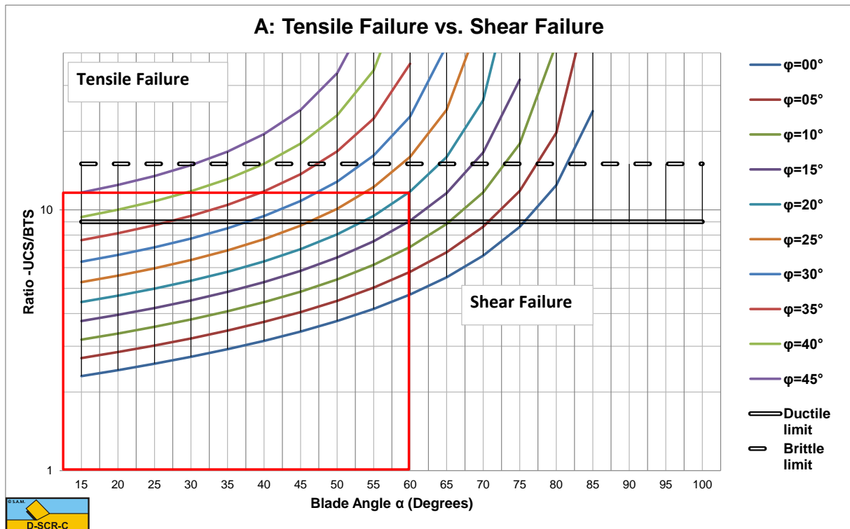
Figure W-6: The tensile/shear failure criterion based on UCS/BTS.
