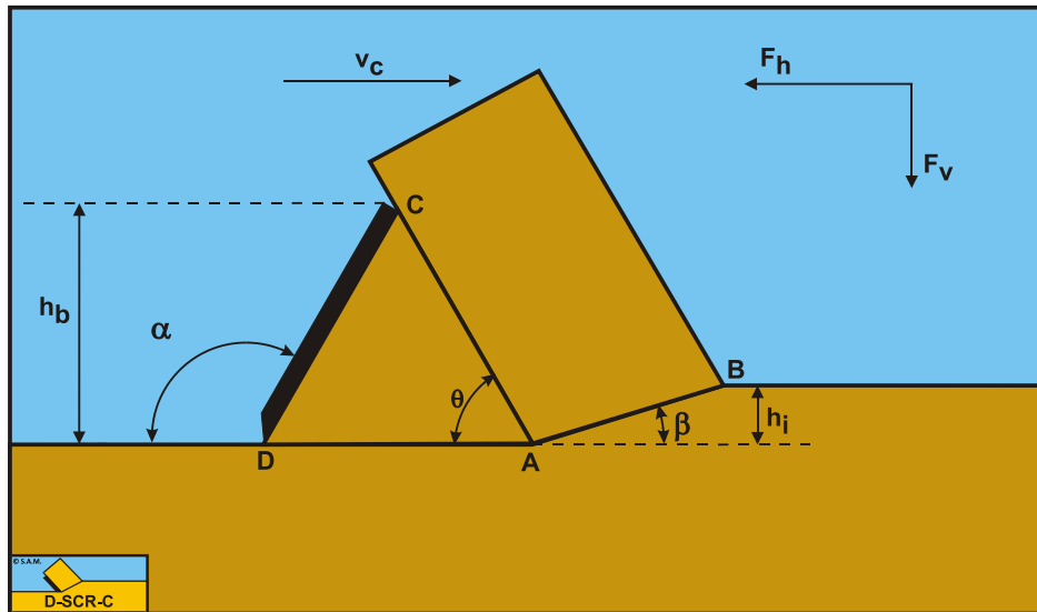
Figure 15-1: Definitions.
