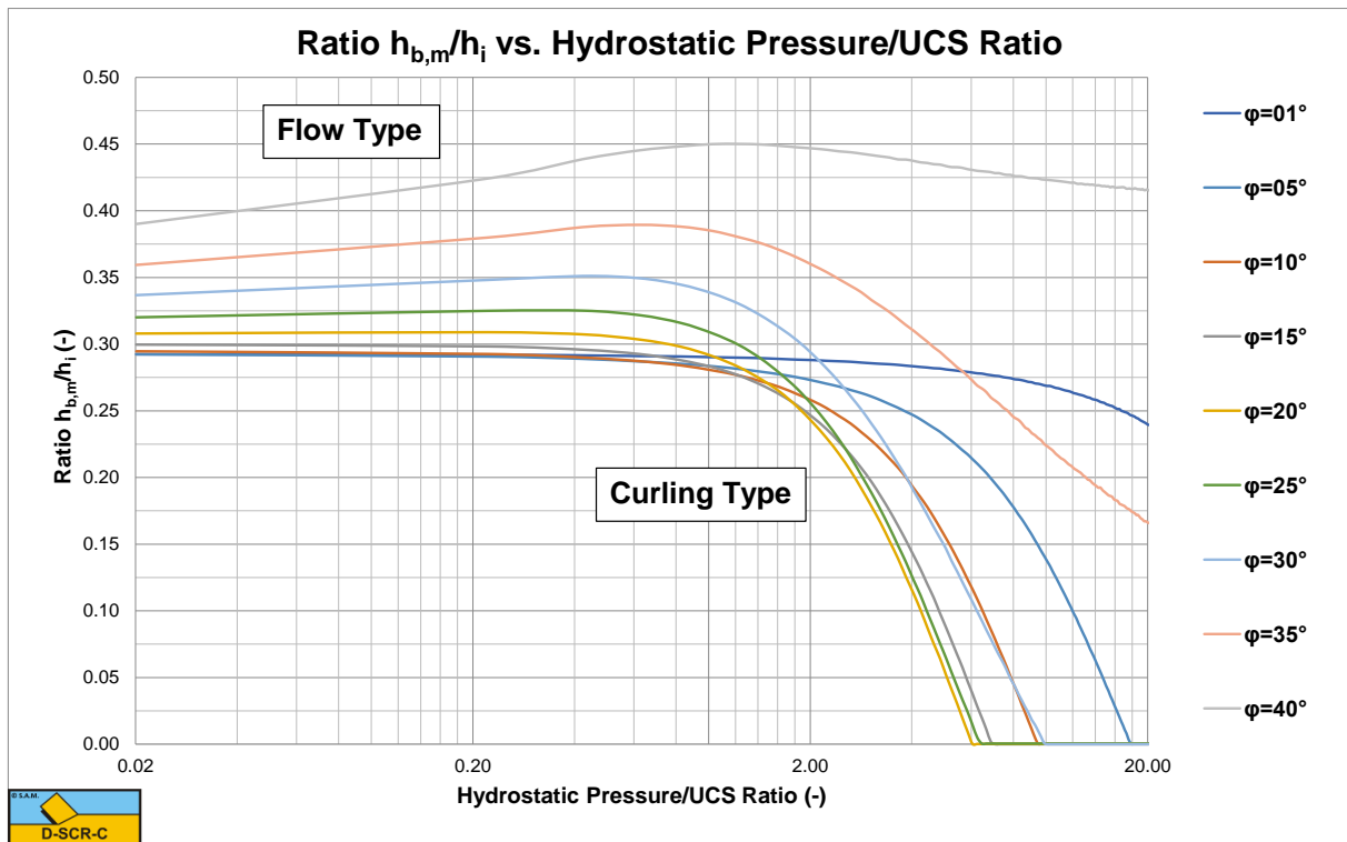
Figure X-6: The ratio h_{b,m}/h_i for a 45 degree blade.
