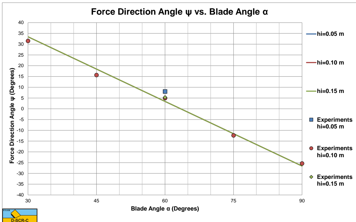
Figure 5-21: The direction of the total cutting force versus the blade angle.
