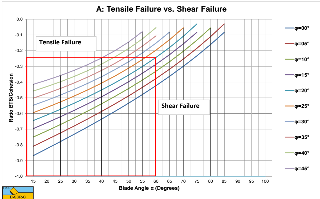
Figure W-5: The tensile/shear failure criterion based on BTS/Cohesion.
