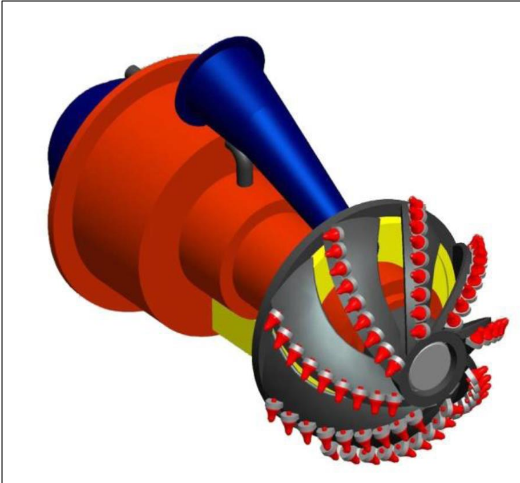
Figure Y-15: Cutterhead (IHC).
