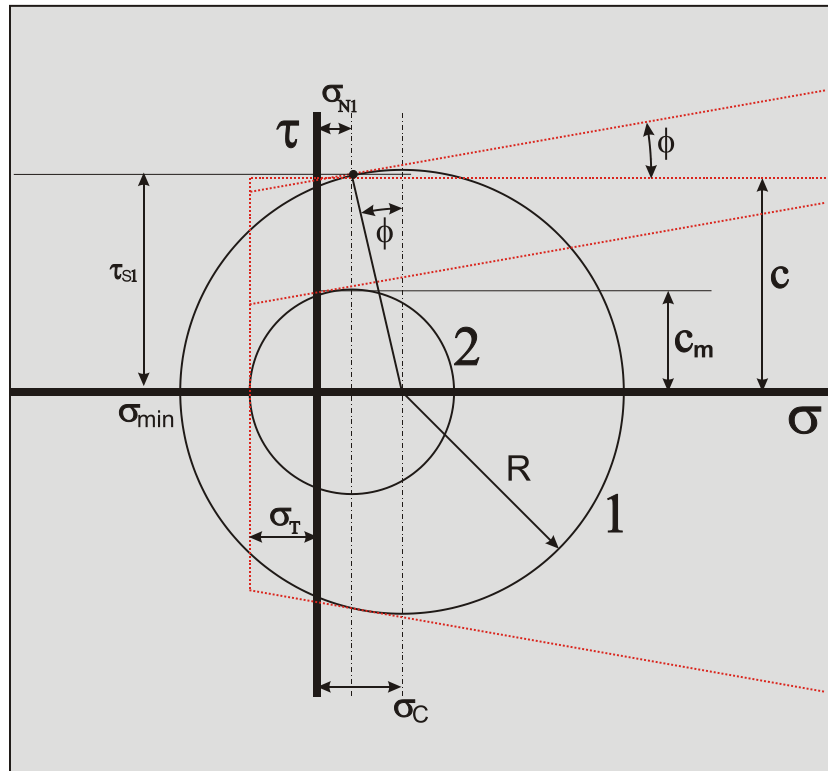
Figure 8-37: The Mohr circles of the Tear Type.
