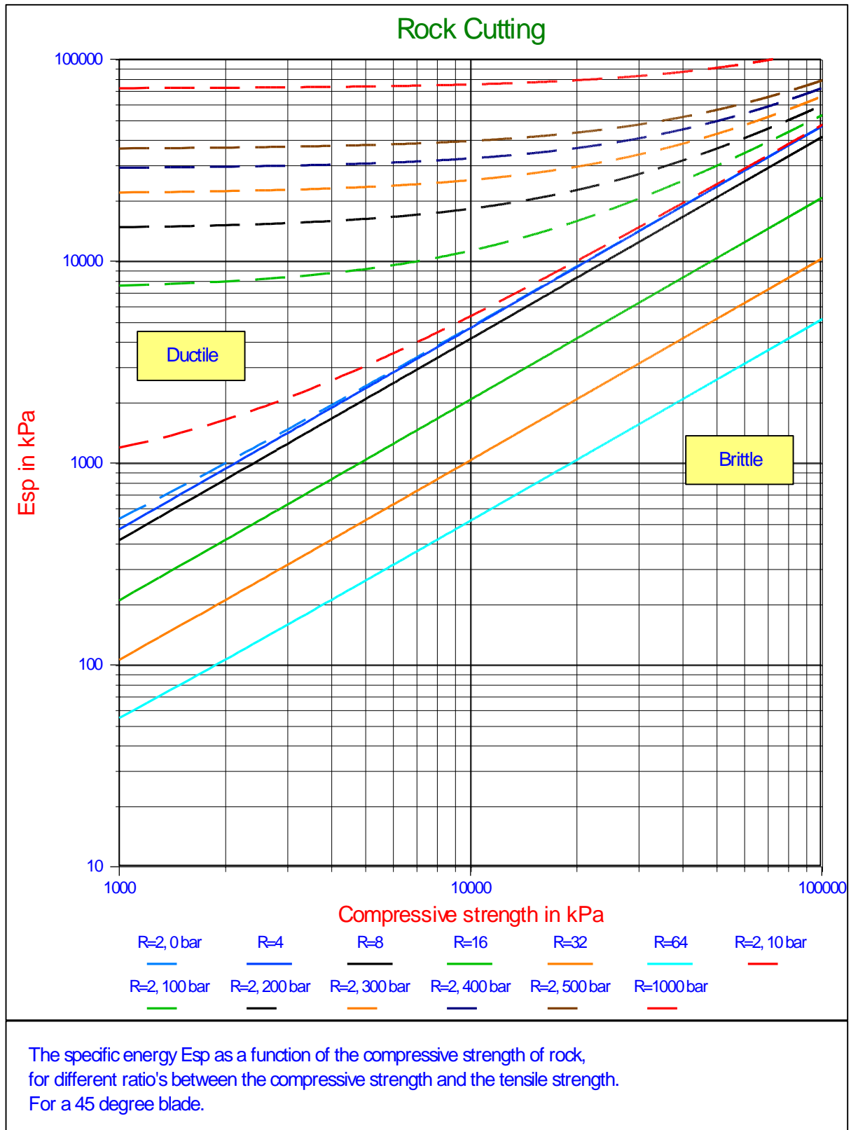
Figure 9-30: The specific energy E_{sp} in rock versus the compressive strength (UCS) for a 45° blade.
