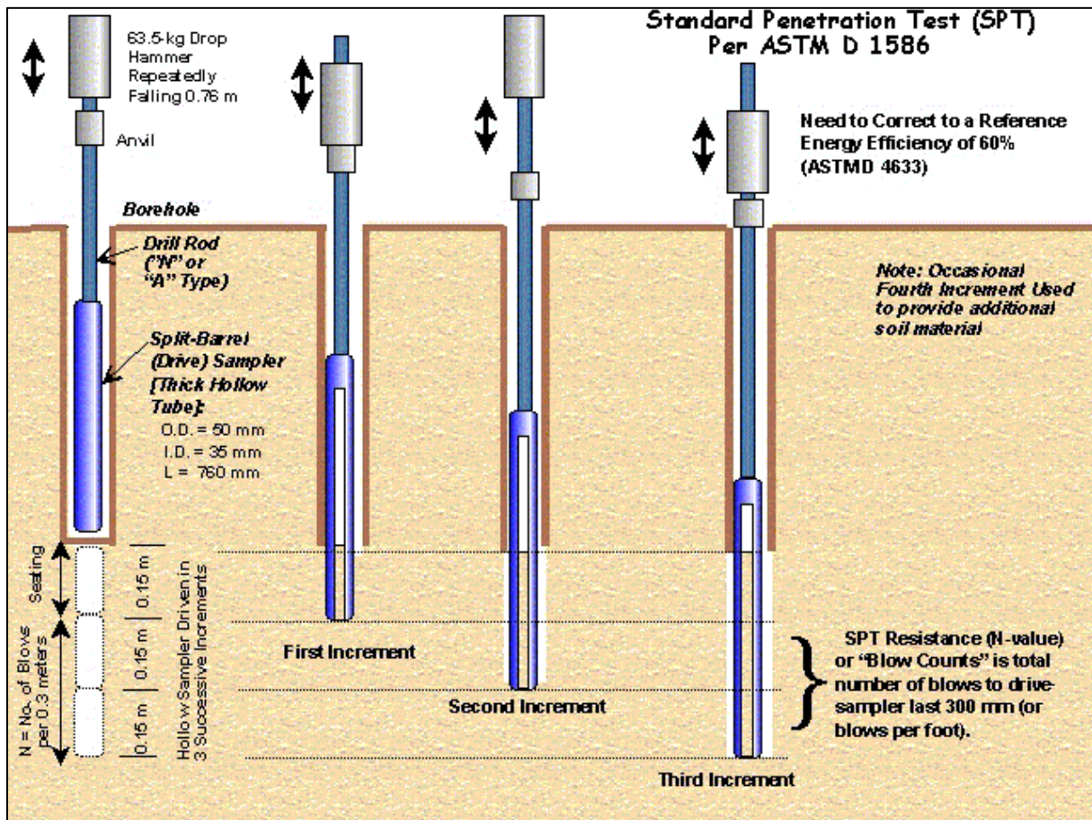
Figure 2-31: The Standard Penetration Test ( www.shalviengineering.com ).
