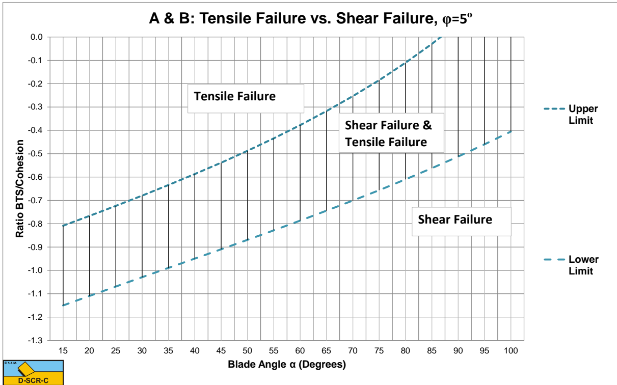
Figure W-13: The tensile/shear failure range based on BTS/Cohesion for \phi=5^\circ .
