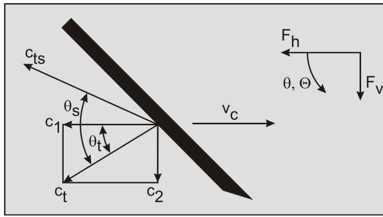
Figure 6-34: The influence of wear.
