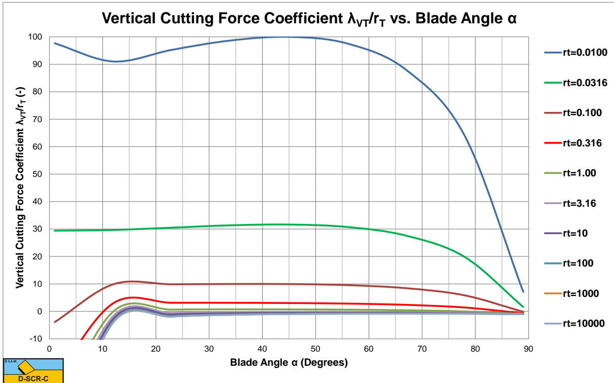
Figure 7-31: The vertical cutting force coefficient \lambda_{VT}/r_T .
