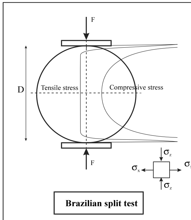
Figure 2-26: The Brazilian split test (Vlasblom (2003-2007)).
