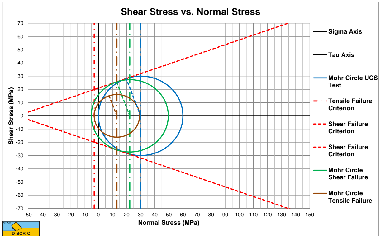
Figure 16-13: The Mohr circles with tensile strength of -3 MPa (UCS=60 MPa, \phi=20^\circ ). Tensile Failure.
