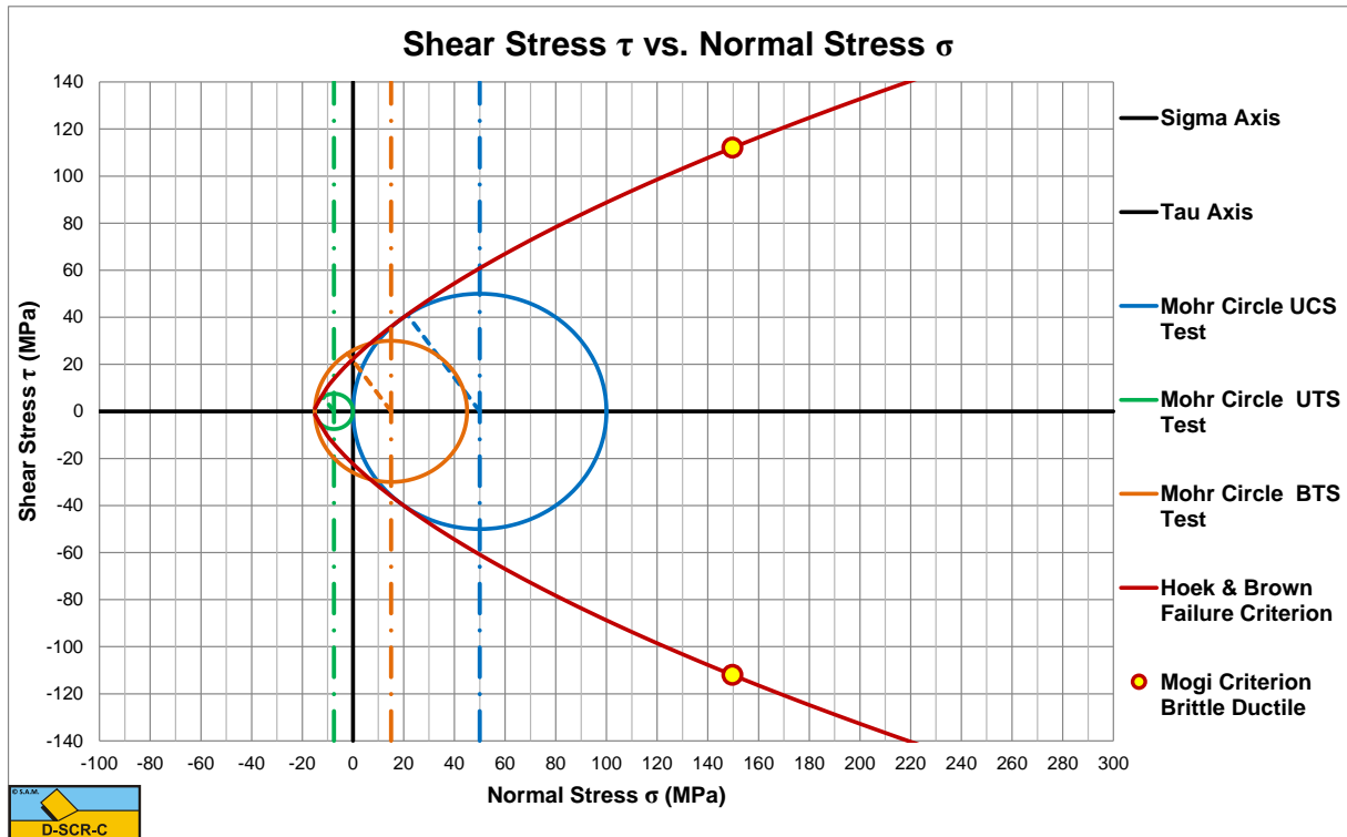
Figure 8-12: Construction Hoek & Brown failure criterion.
