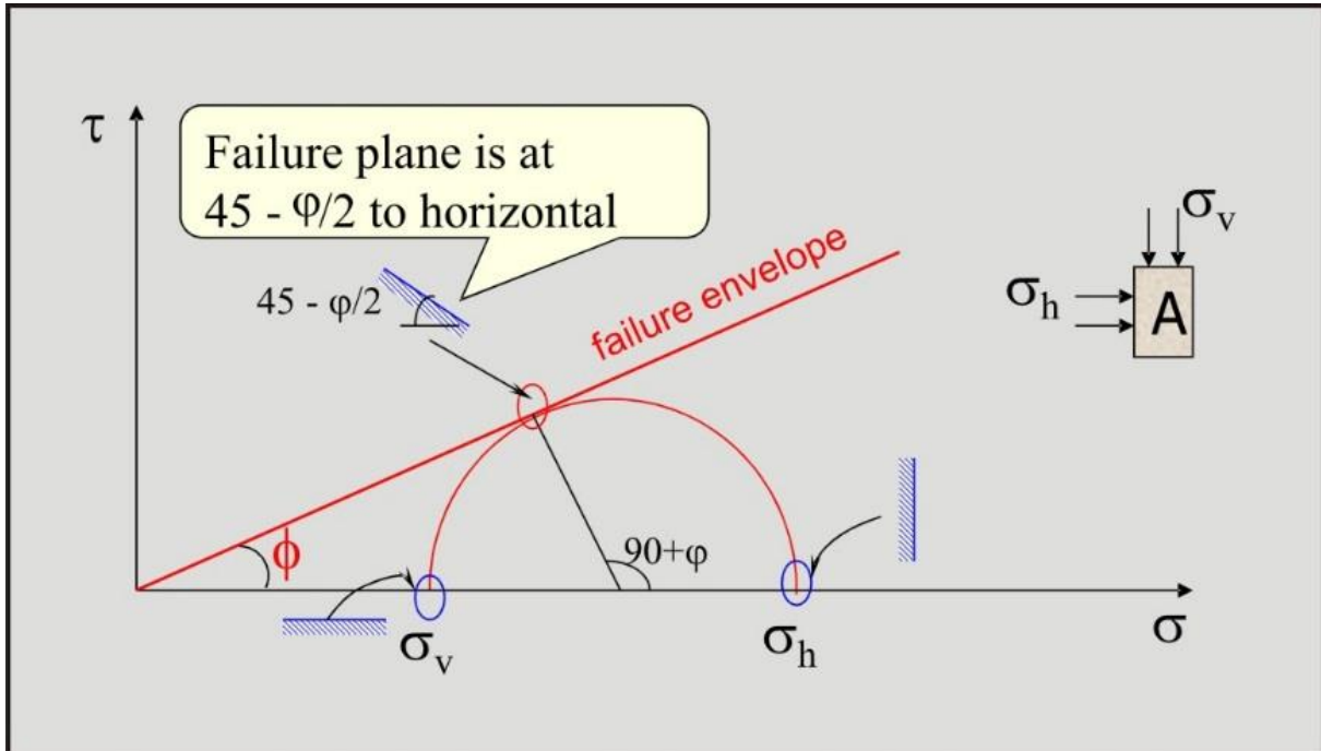
Figure 2-55: The Mohr circle for passive soil failure.
