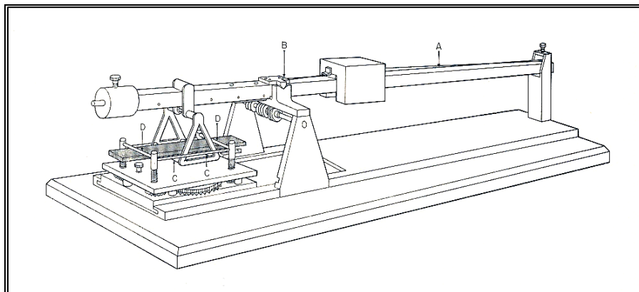
Figure 2-25: Bending (Vlasblom (2003-2007)).
