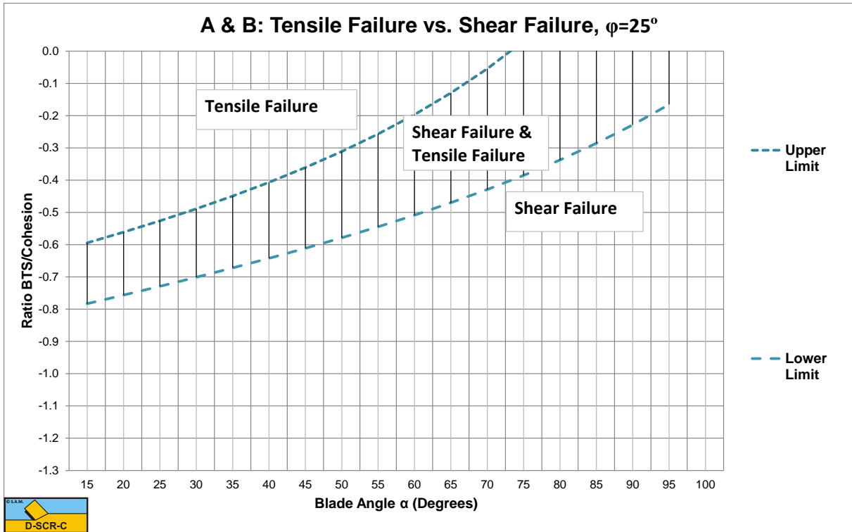
Figure W-21: The tensile/shear failure range based on BTS/Cohesion for \phi=25^\circ .
