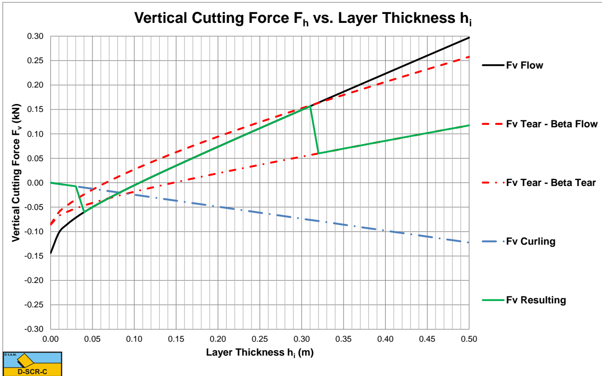
Figure 7-40: Vertical force; Cohesion c=1 kPa, adhesion a=1 kPa, tensile strength \sigma_T=-0.3 kPa, blade height h_b=0.1 m, blade angle \alpha=55^\circ
