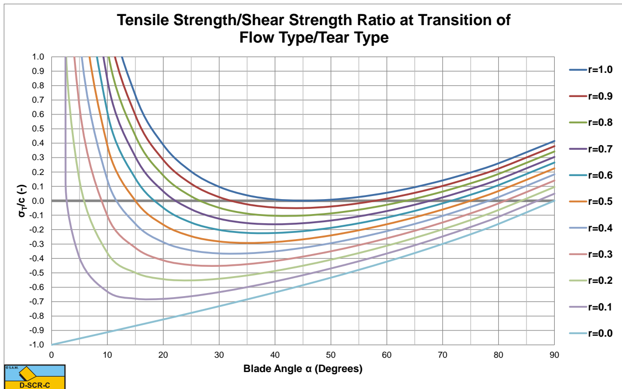
Figure V-7: The transition Flow Type vs. Tear Type.
