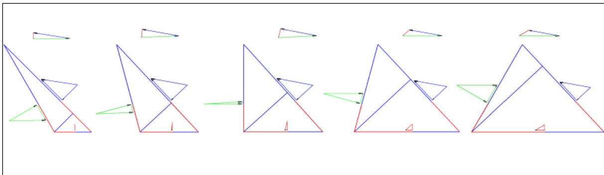
Figure 12-21: The forces on the wedges at 60°, 75°, 90°, 105° and 120° cutting angles.
