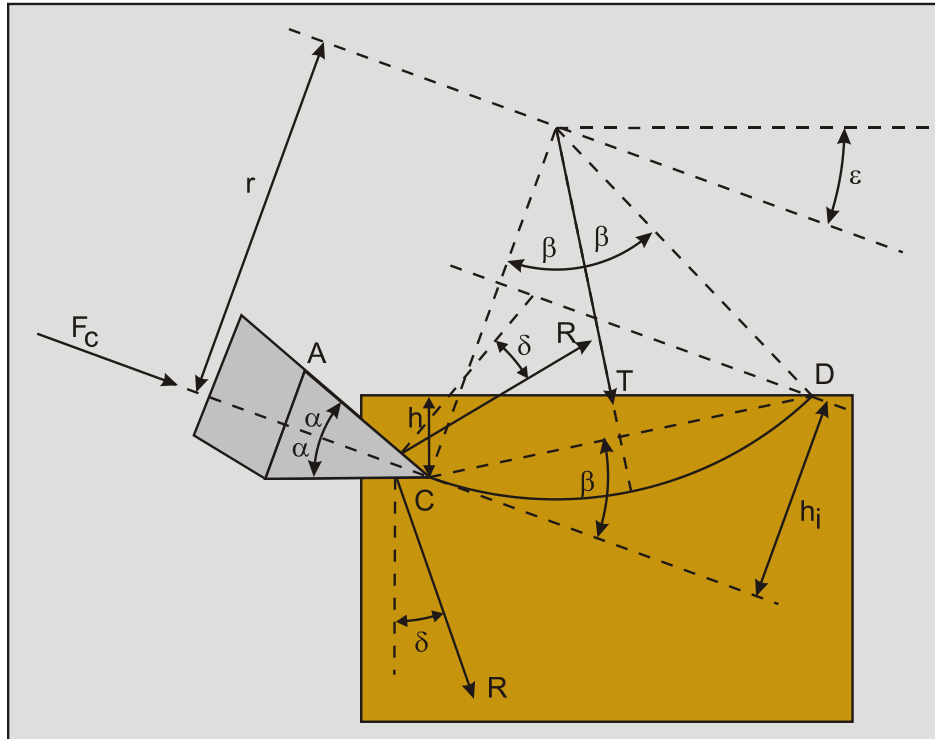
Figure 8-23: The model of Evans used for a pick point.
