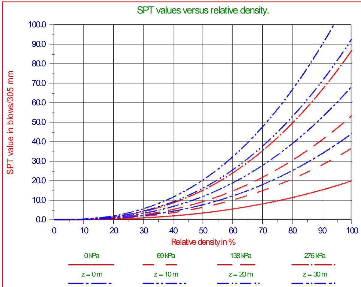
Figure 2-22: SPT values versus relative density (Miedema (1995)).
