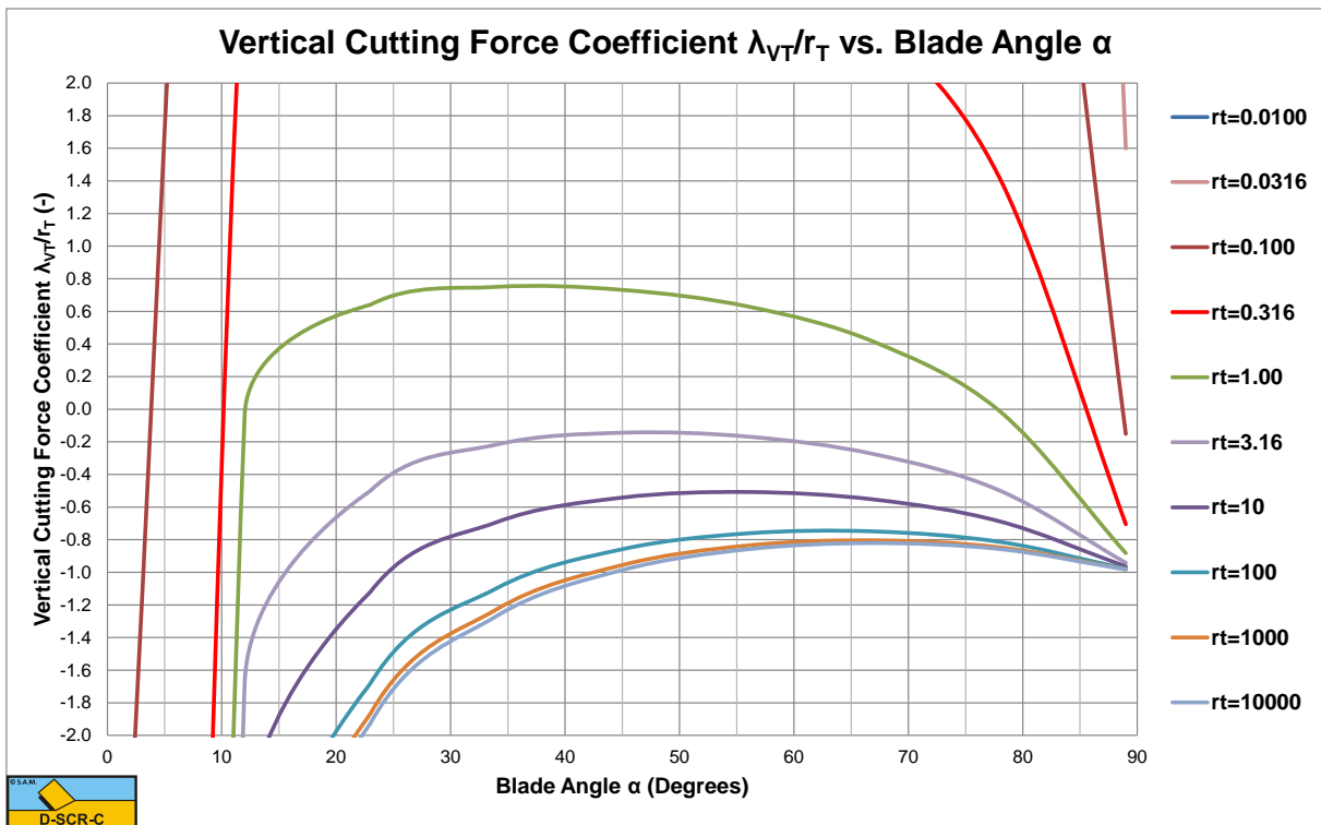
Figure V-11: The vertical cutting force coefficient \lambda_{VT}/r_T zoomed.
