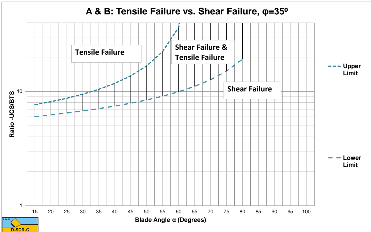
Figure W-26: The tensile/shear failure range based on UCS/BTS for \phi=35^\circ .
