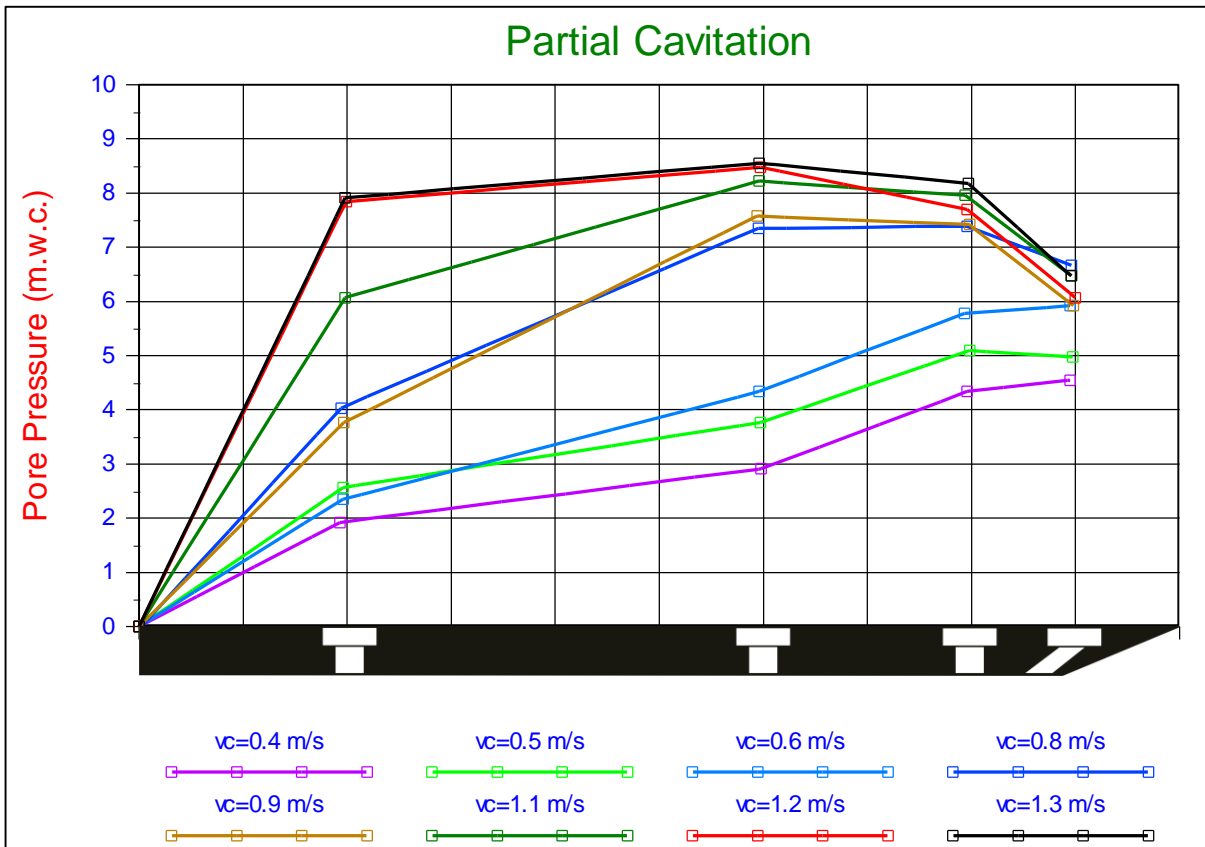
Figure M-5: Measured absolute pore pressures.
