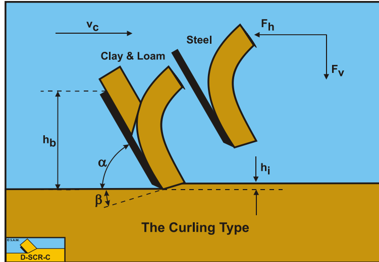
Figure 7-33: The Curling Type cutting mechanism when cutting clay.
