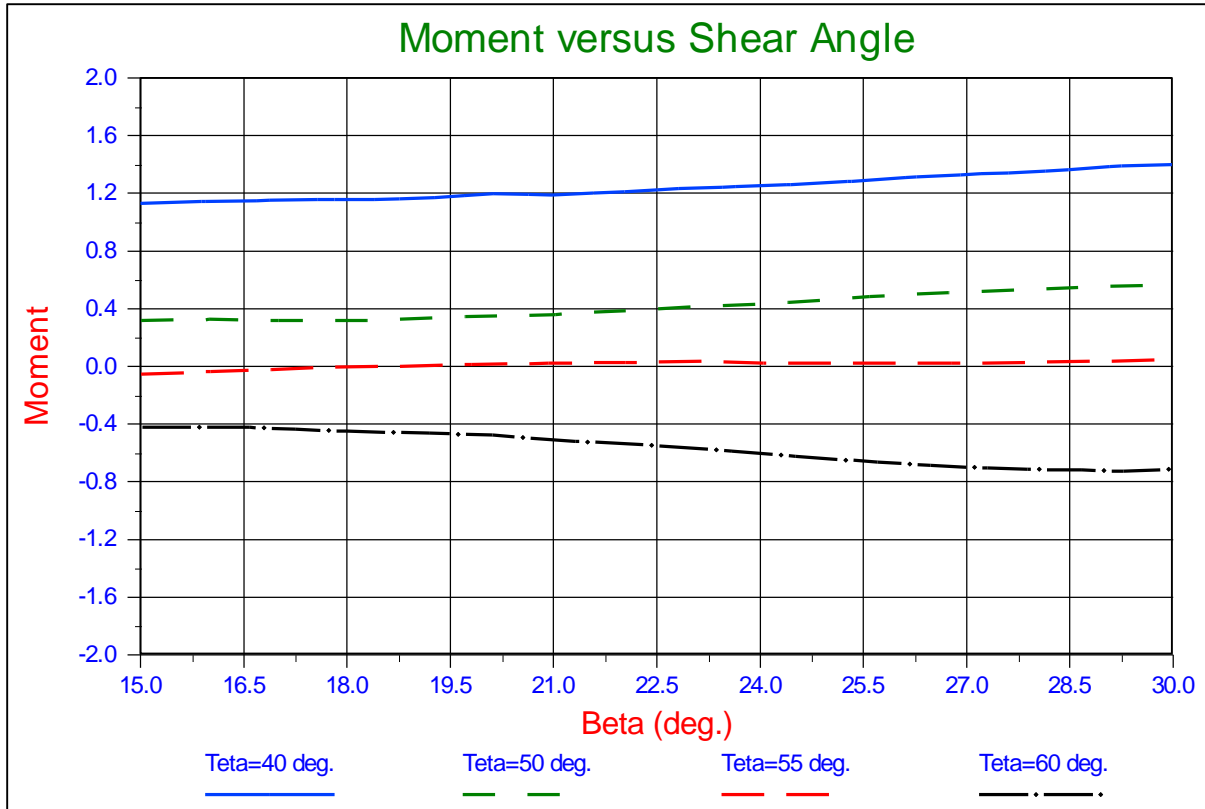
Figure 12-20: The moment versus the shear angle for 4 different wedge angles for: \alpha=90^\circ ; \delta=28^\circ ; \varphi=42^\circ ; h_i=1 ; h_b=3 ; k_i/k_{max}=0.25
