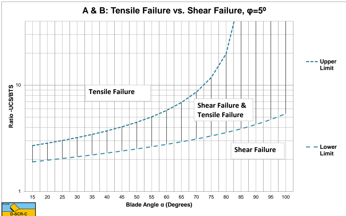
Figure W-14: The tensile/shear failure range based on UCS/BTS for \phi=5^\circ .
