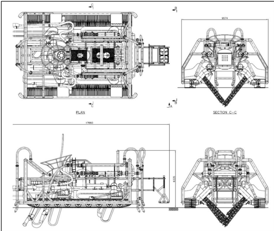
Figure Y-56: The Digging Donald (All Seas).
