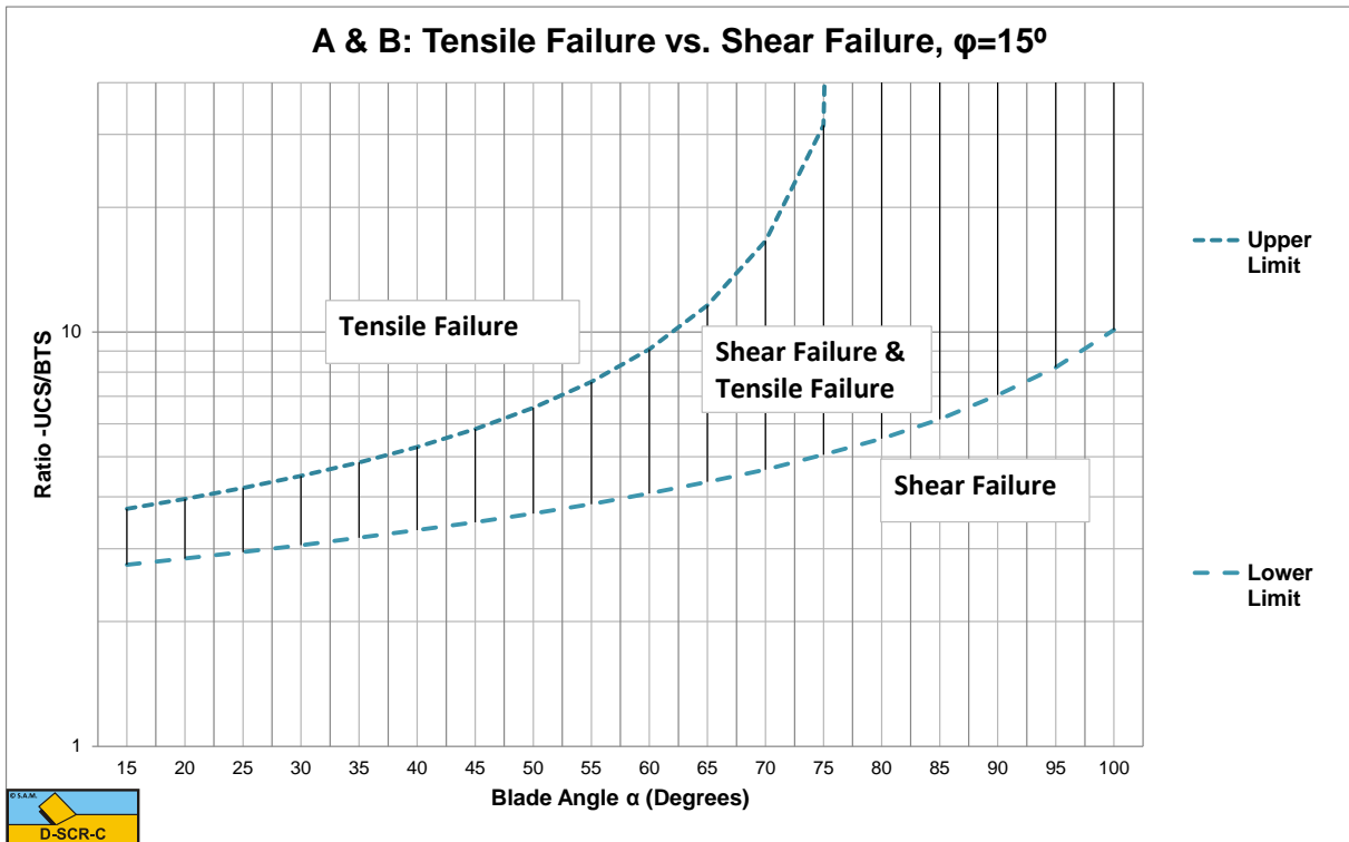
Figure W-18: The tensile/shear failure range based on UCS/BTS for \phi=15^\circ .
