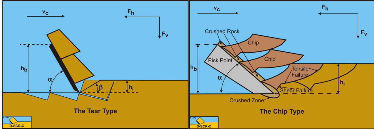
Figure 8-34: The Tear Type cutting mechanism in rock under hyperbaric conditions.
