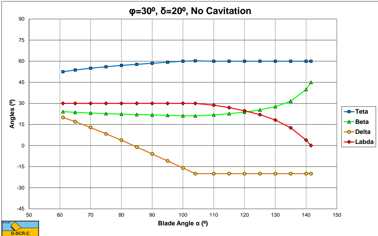
Figure 12-22: No cavitation, the angles \theta , \beta , \delta_m and \lambda as a function of the blade angle \alpha for \phi=30^\circ and \delta=20^\circ .
