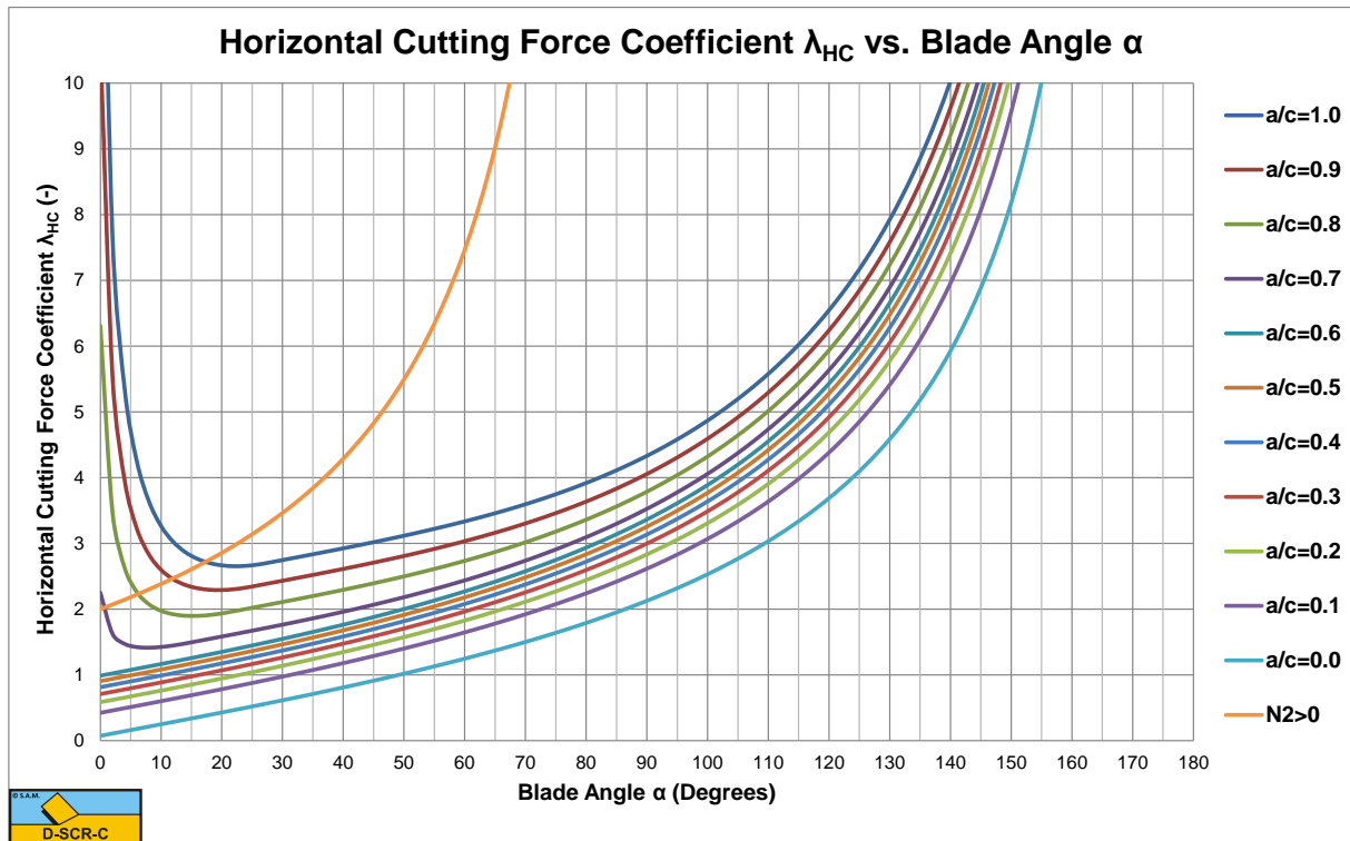
Figure V-14: The horizontal cutting force coefficient \lambda_{HC} .
