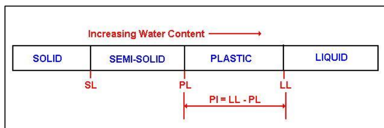
Figure 2-21: The relation between SL, PL, LL and PI.
