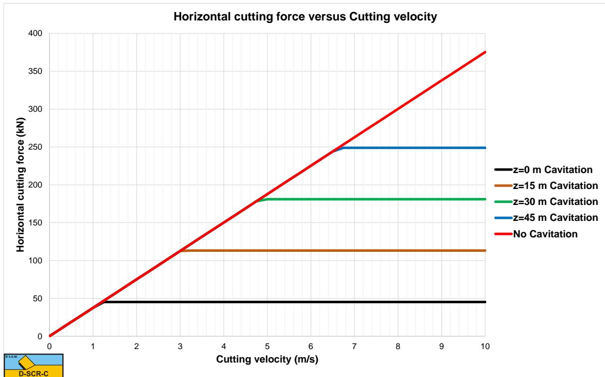
Figure 16-1: The horizontal cutting forces.
