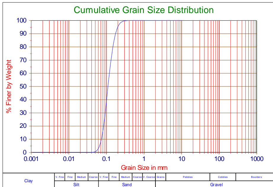
Figure L-1: The PSD of the 105 \mu\text{m} sand.
