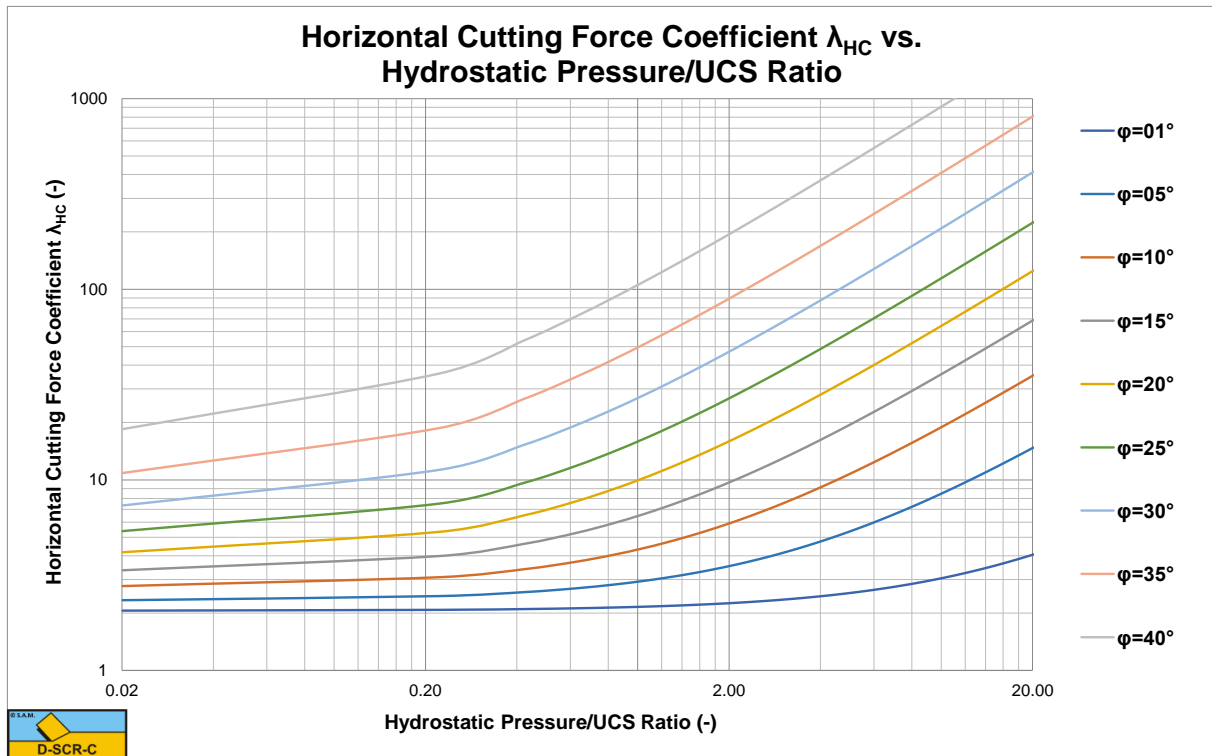
Figure X-23: The horizontal cutting force coefficient \lambda_{HC} for a 90 degree blade.
