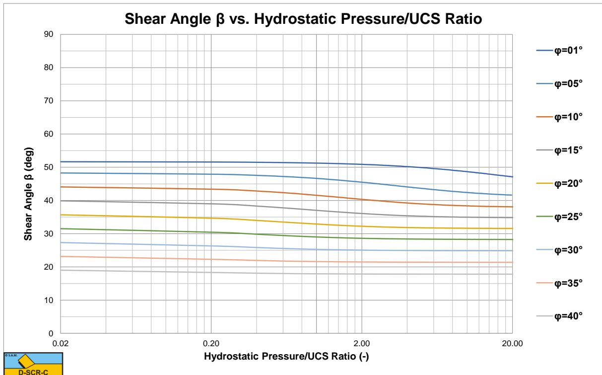
Figure X-17: The shear angle \beta for a 75 degree blade.
