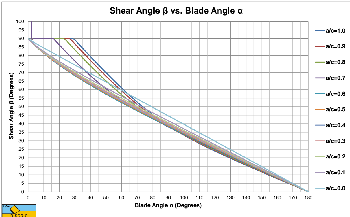
Figure V-13: The shear angle for the Curling Type
