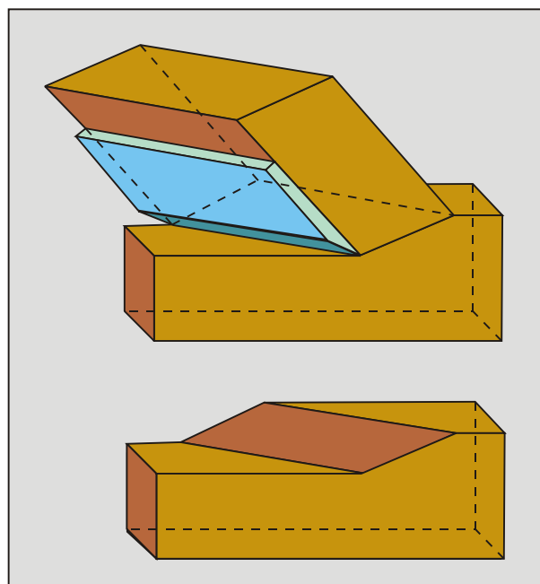
Figure 3-16: The 3D cutting process.
