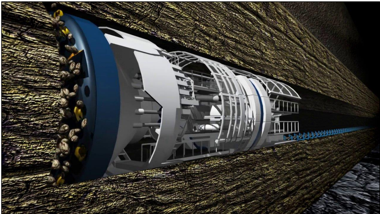
Figure Y-79: Tunnel Boring Machine ( www.imaker.ca ).
