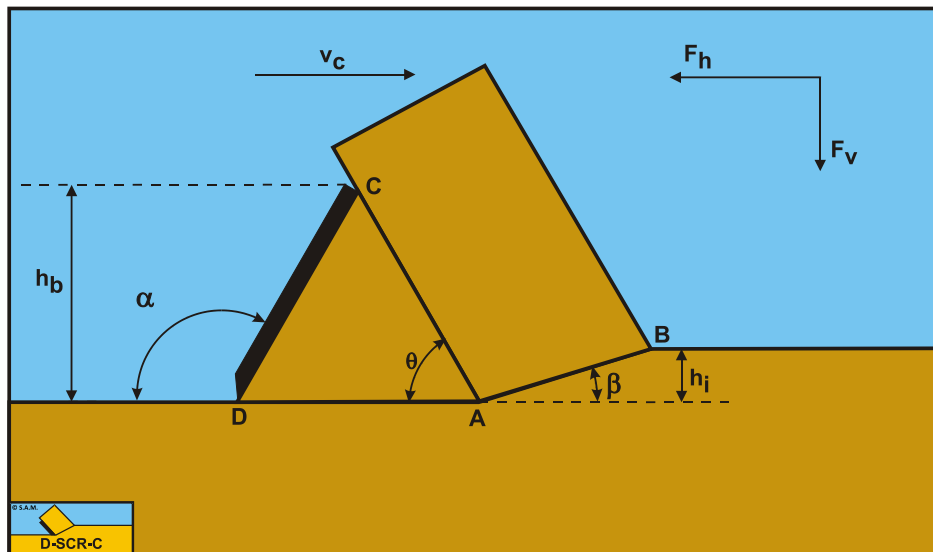
Figure 13-1: The occurrence of a wedge in clay cutting.
