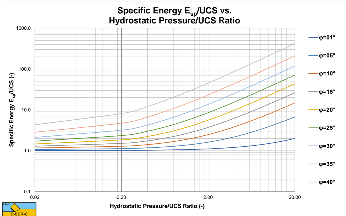
Figure X-25: The specific energy to UCS ratio for a 90 degree blade.
