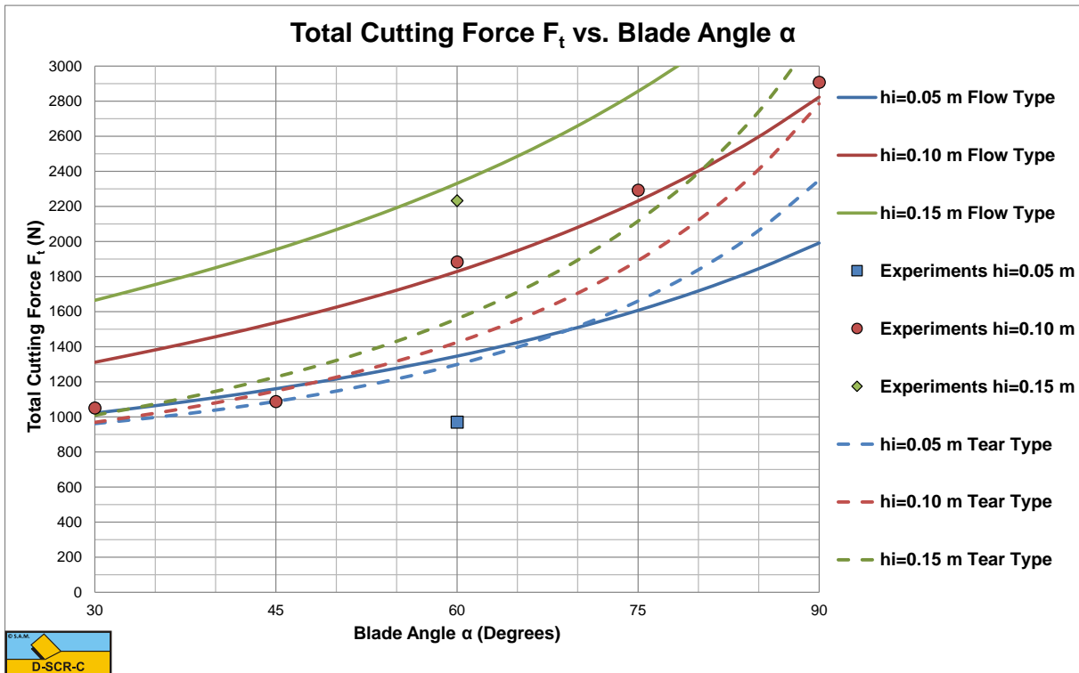
Figure 7-45: The total cutting force measured and calculated.
