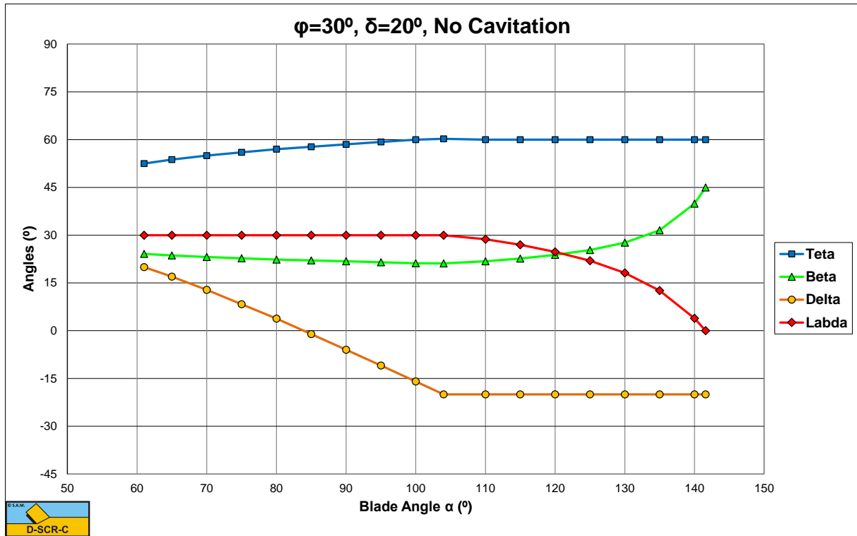
Figure P-1: No cavitation, the angles \theta , \beta , \delta_m and \lambda as a function of the blade angle \alpha for \varphi=30^\circ and \delta=20^\circ .
