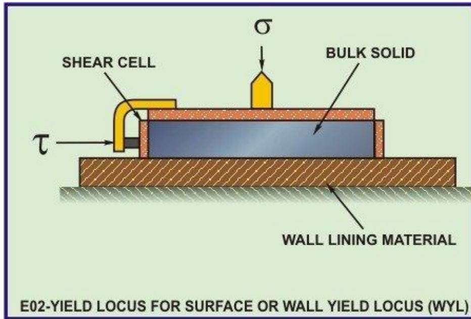
Figure 2-37: The direct shear test.
