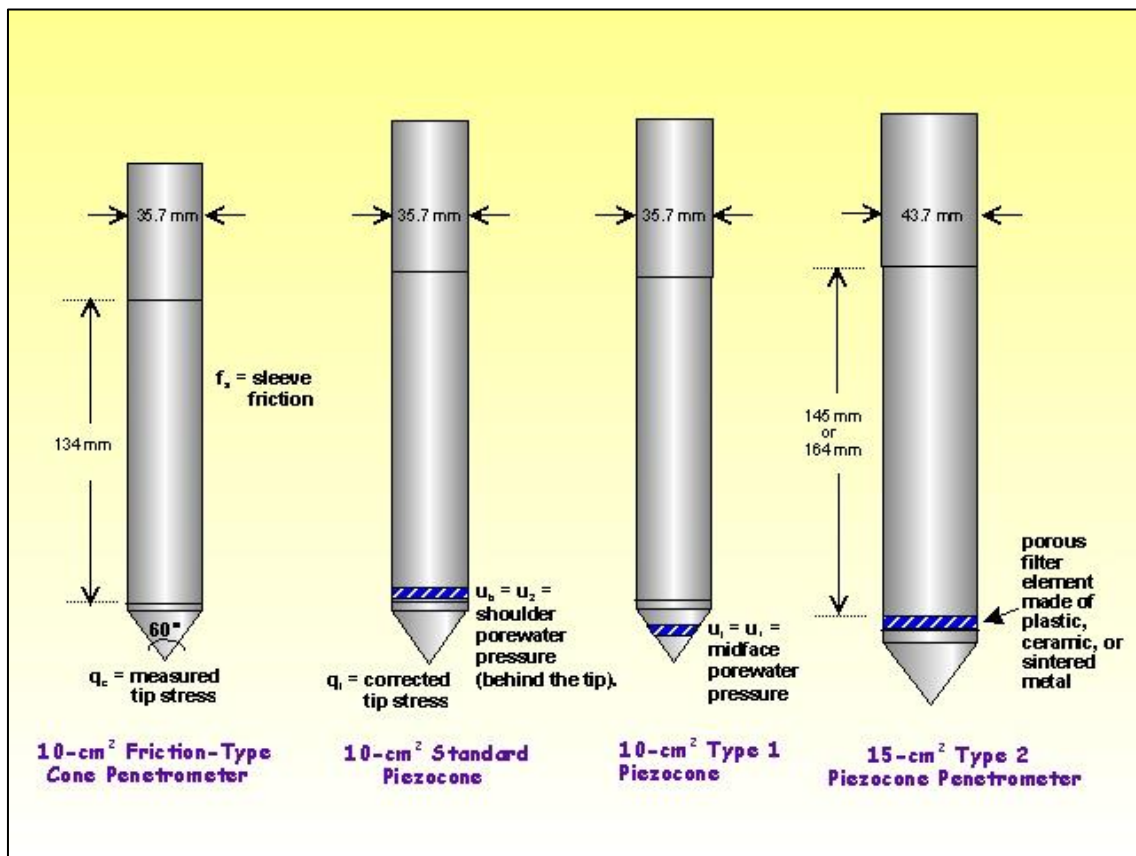
Figure 2-33: Several configurations of cones (www.geotechdata.info).
