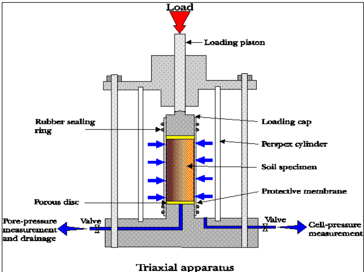
Figure 2-36: The Triaxial apparatus cross-section (civilblog.org).
