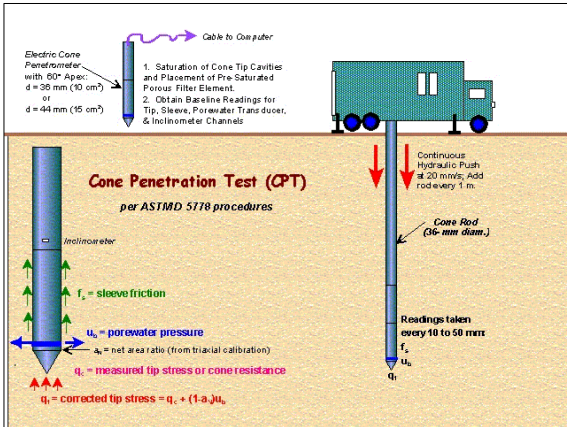
Figure 2-32: A typical CPT test setup (www.geotechdata.com).
