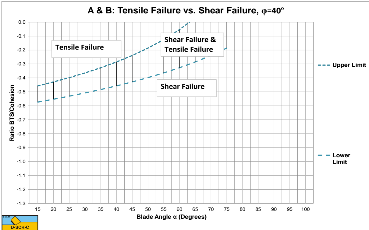
Figure W-27: The tensile/shear failure range based on BTS/Cohesion for \phi=40^\circ .
