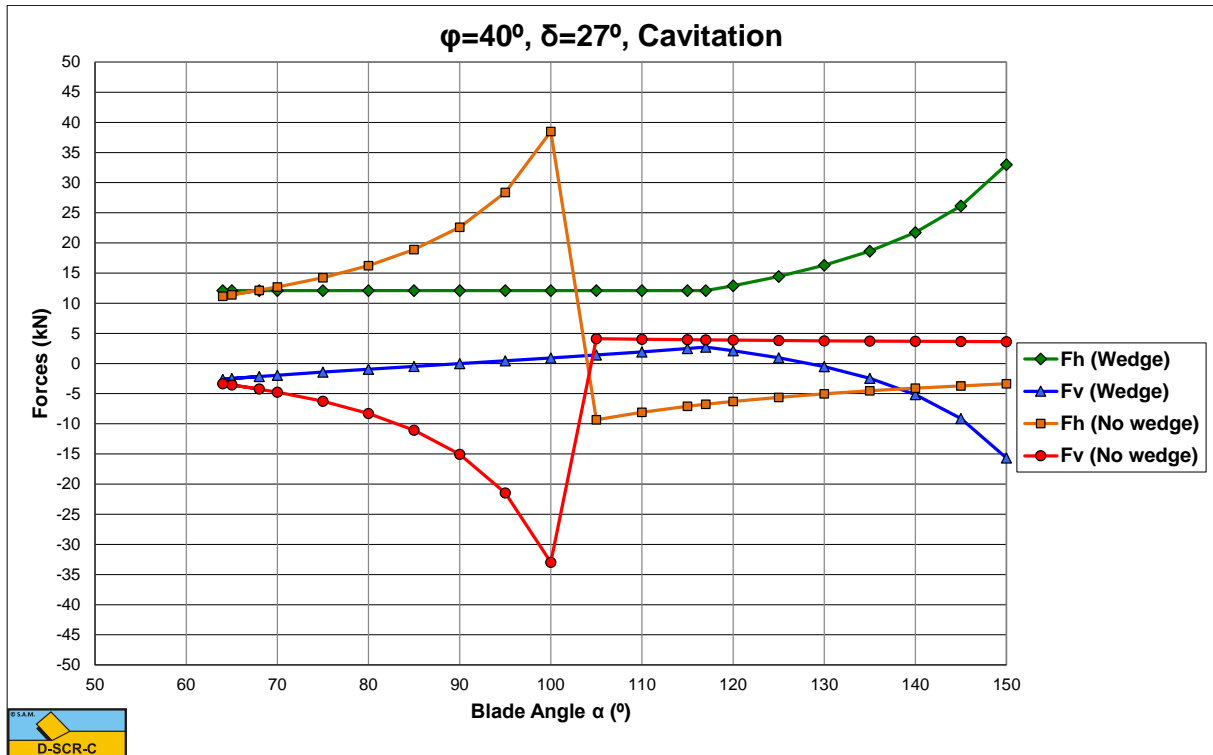
Figure Q-6: Cavitating, the cutting forces as a function of the blade angle \alpha for \varphi=40^\circ and \delta=27^\circ .
