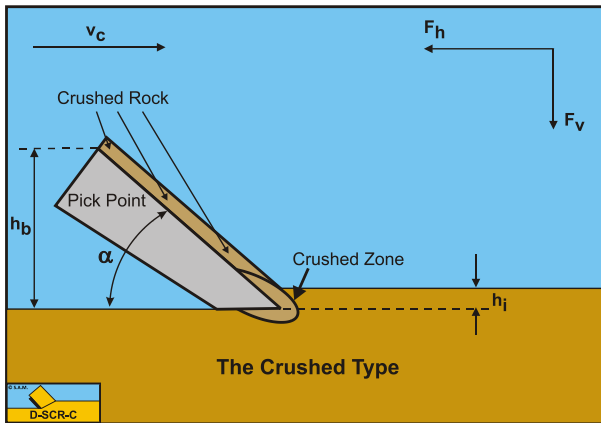
Figure 8-18: The Crushed Type.
