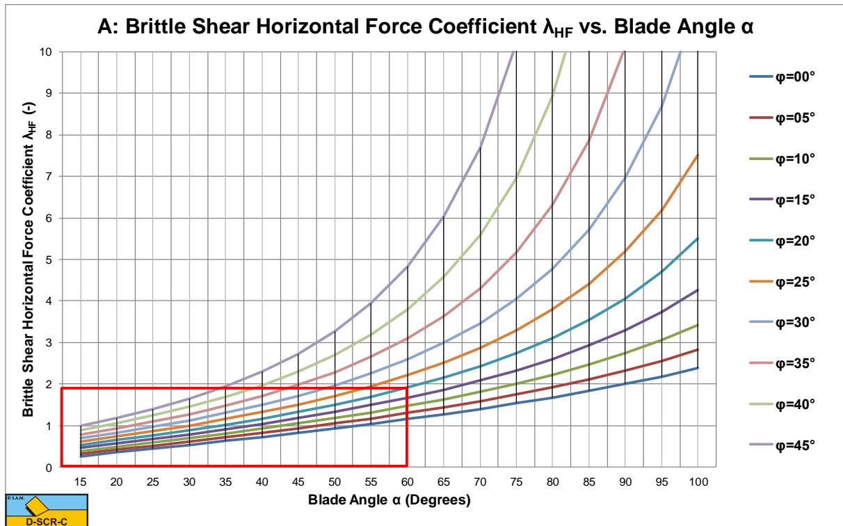
Figure 8-31: The brittle (shear failure) horizontal force coefficient \lambda_{HF} .
