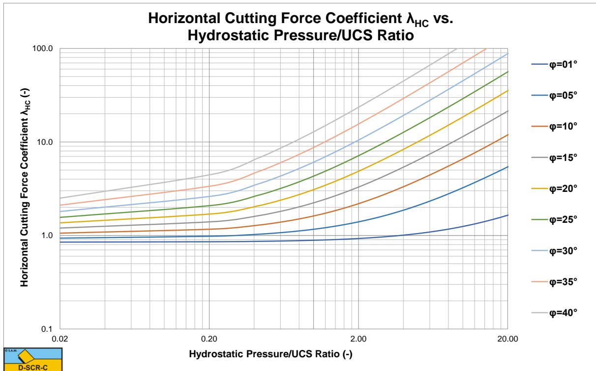
Figure X-8: The horizontal cutting force coefficient \lambda_{HC} for a 45 degree blade.
