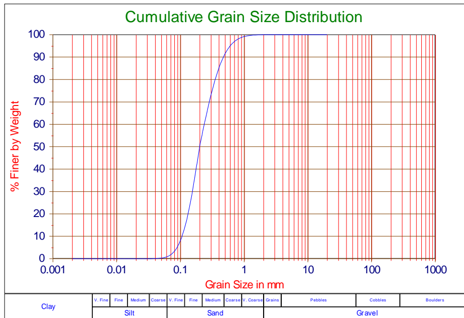
Figure K-1: The PSD of the 200 \mu\text{m} sand.
