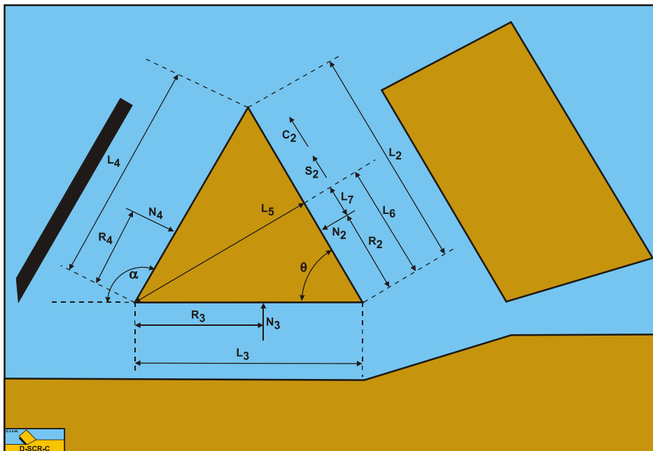
Figure 14-5: The moments on the wedge.
