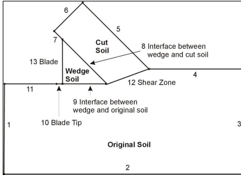
Figure 12-9: The boundaries of the FEM model.
