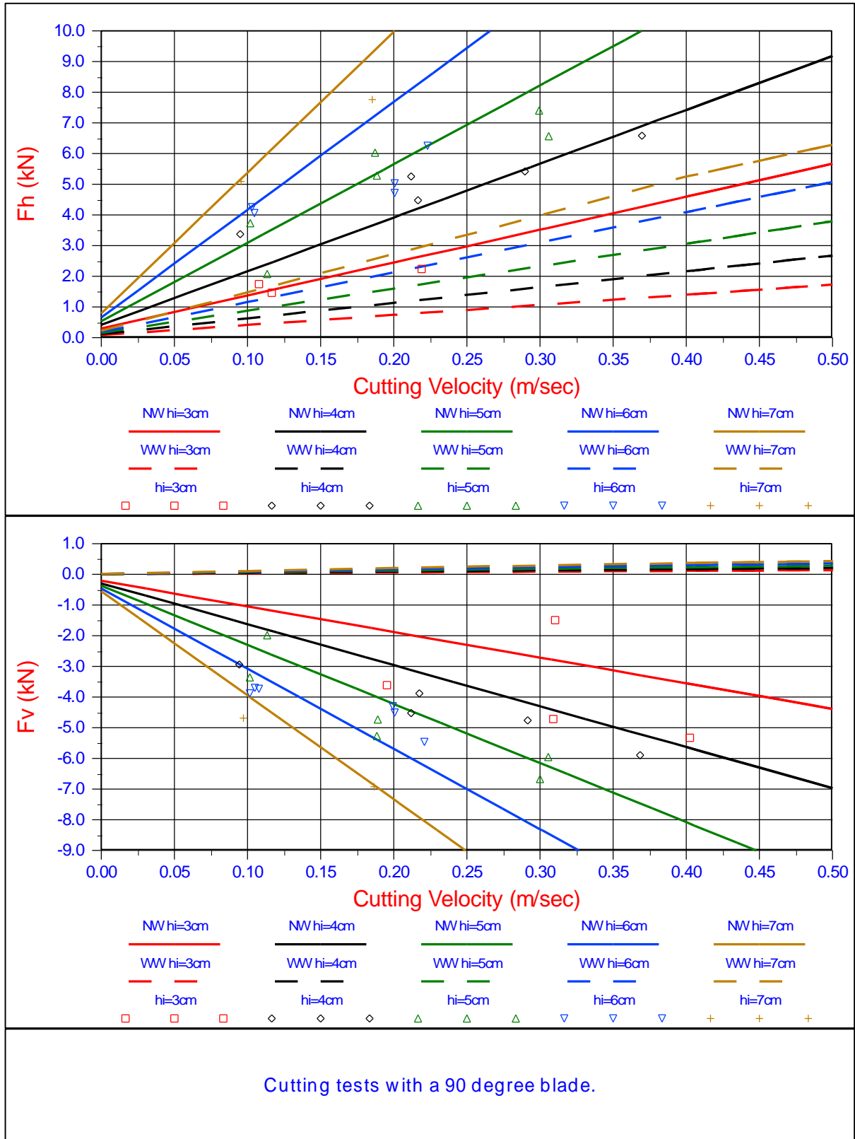
Figure 12-38: Cutting forces for cutting depths ( h_i ) from 3 to 7 cm; blade angle 90^\circ .
