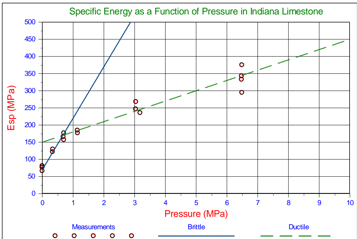
Figure 9-3: MSE versus confining pressure for Indiana limestone in light mineral oil, Rafatian et al. (2009).
