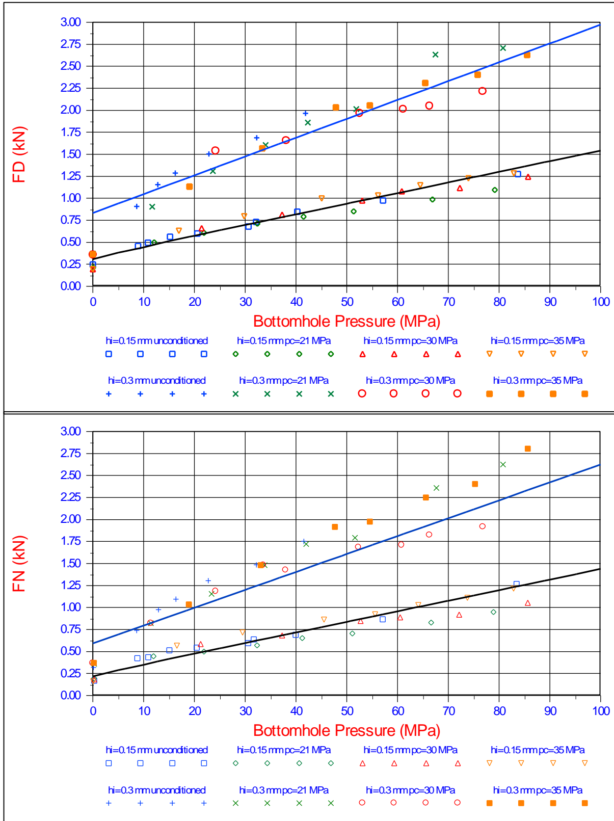
Figure 9-22: The theory of hyperbaric cutting versus the Zijssling (1987) experiments.
