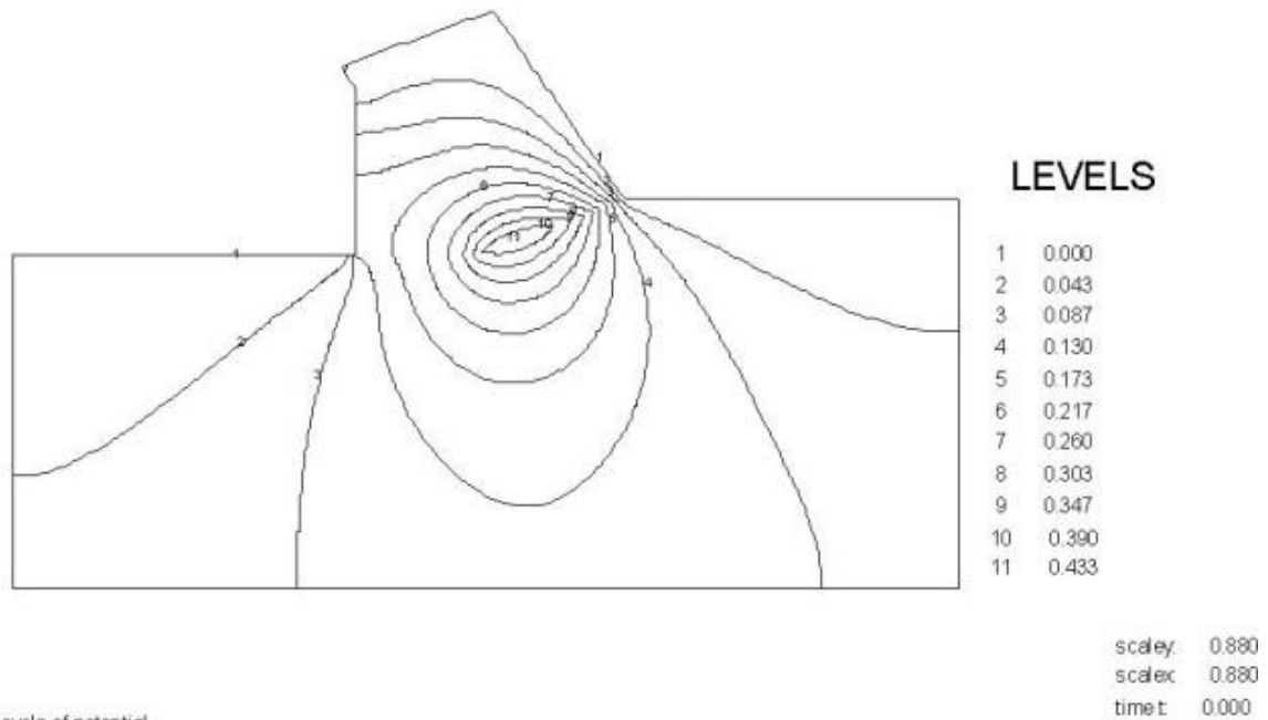
Figure S-13: Equipotential lines of pore pressures.
