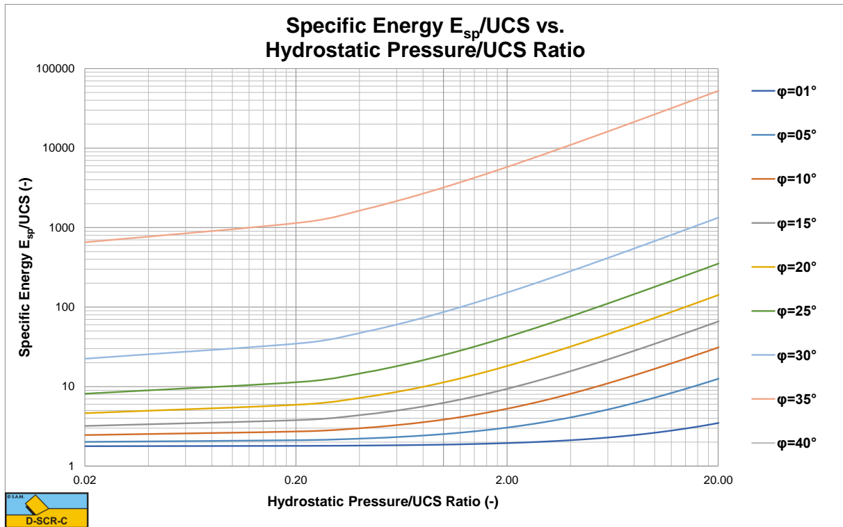
Figure X-35: The specific energy to UCS ratio for a 120 degree blade.
