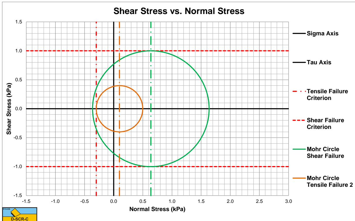
Figure 7-42: The Mohr circles for h_i=0.5 m, only tensile failure possible.
