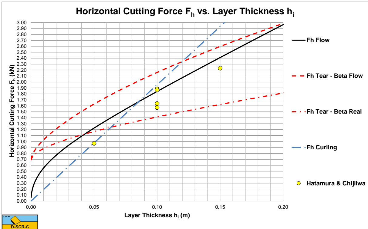
Figure 7-47: The 60 degree experiments.
