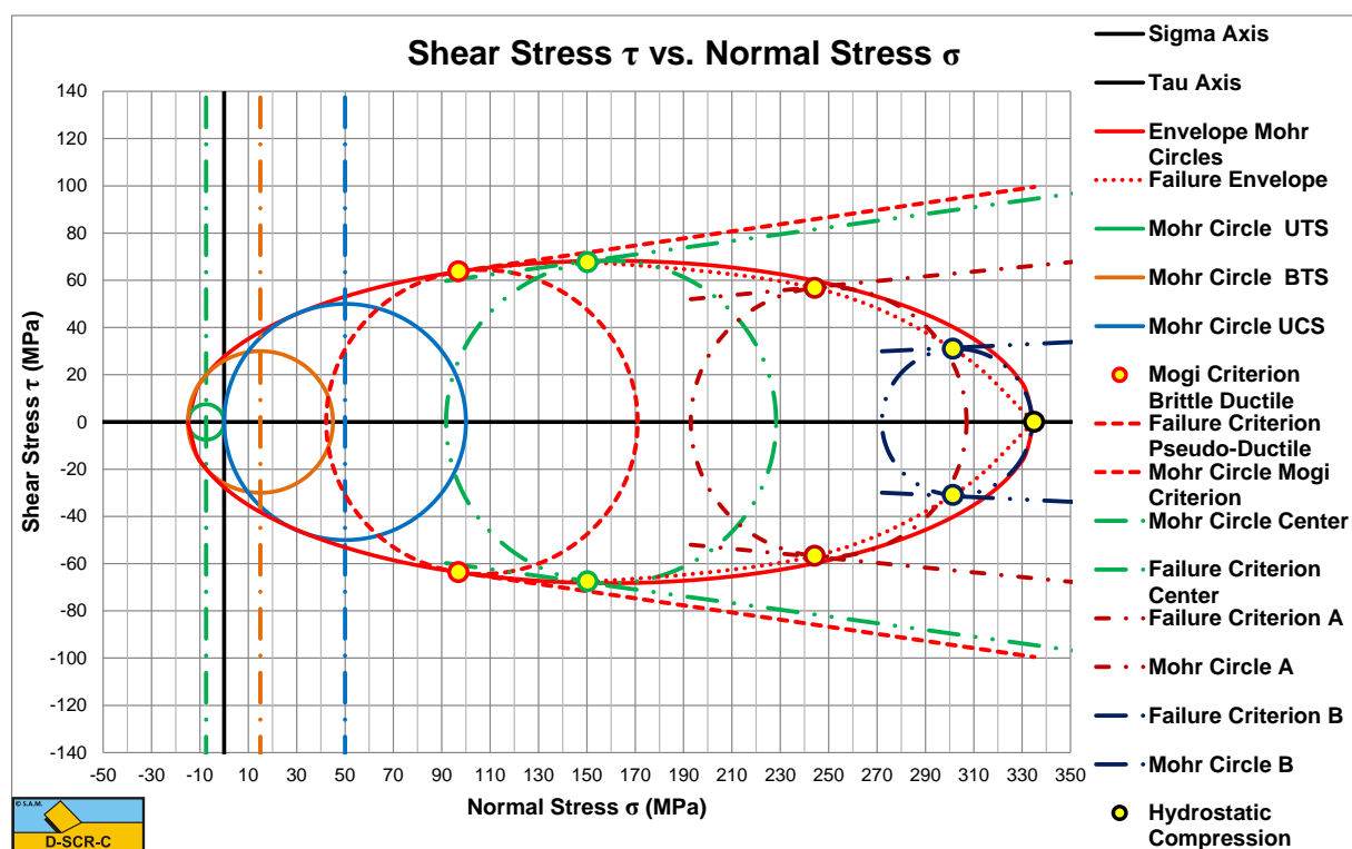
Figure 8-5: Constructing the failure envelope.
