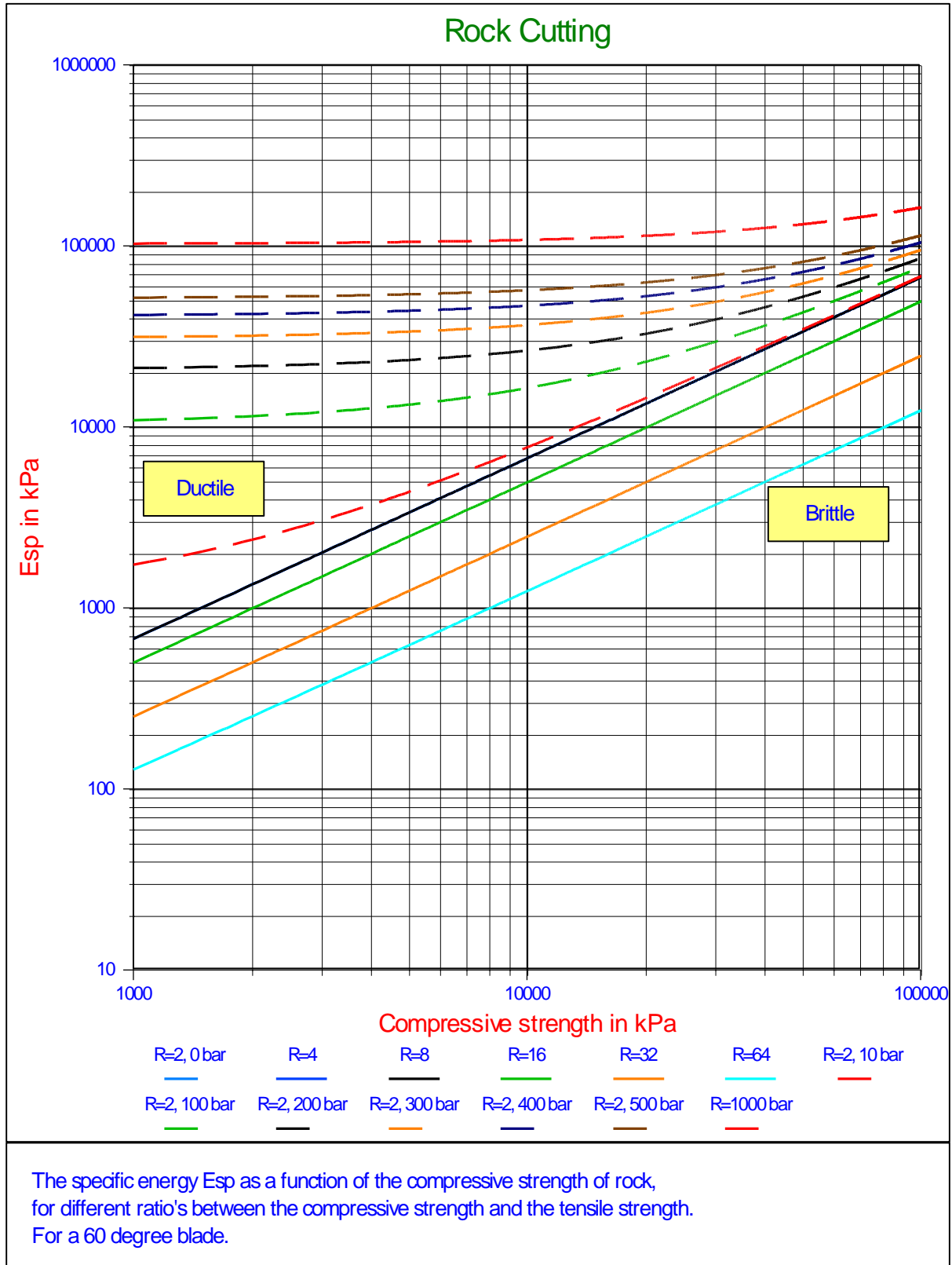
Figure 9-31: The specific energy E_{sp} in rock versus the compressive strength (UCS) for a 60° blade.
