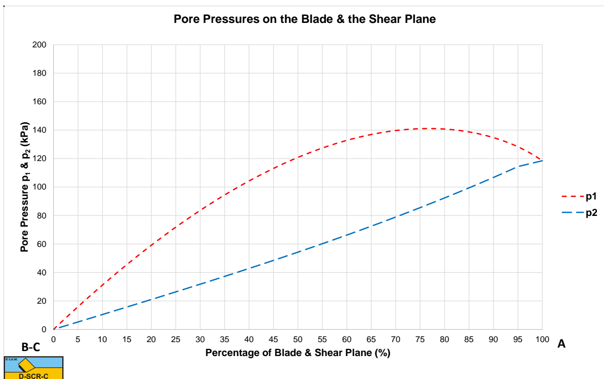
Figure 16-3: The pore pressures on blade and shear plane.
