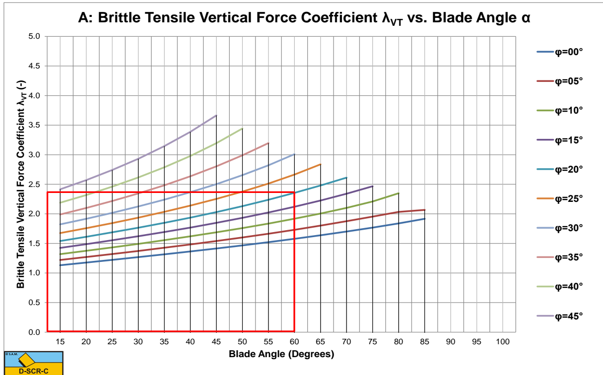
Figure W-32: The brittle (tensile failure) vertical force coefficient \lambda_{VT} .
