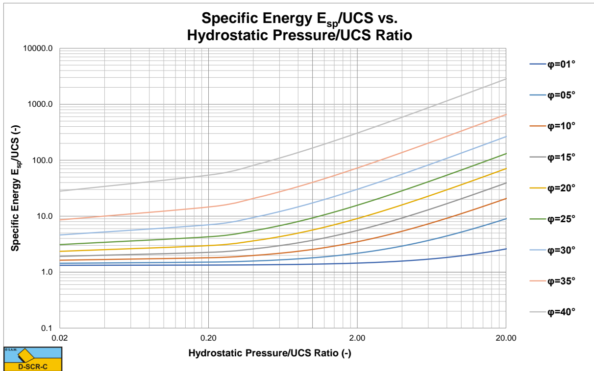
Figure X-30: The specific energy to UCS ratio for a 105 degree blade.
