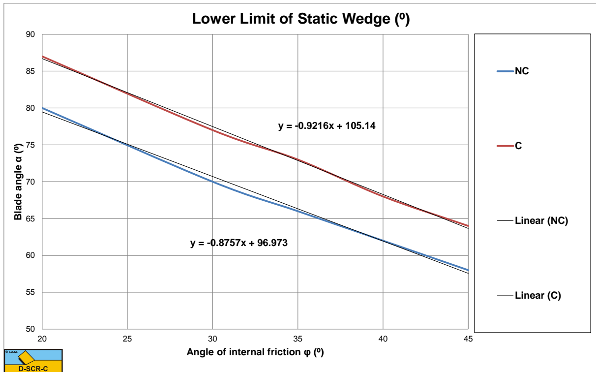
Figure 12-28: The lower limit where the wedge starts to occur.
