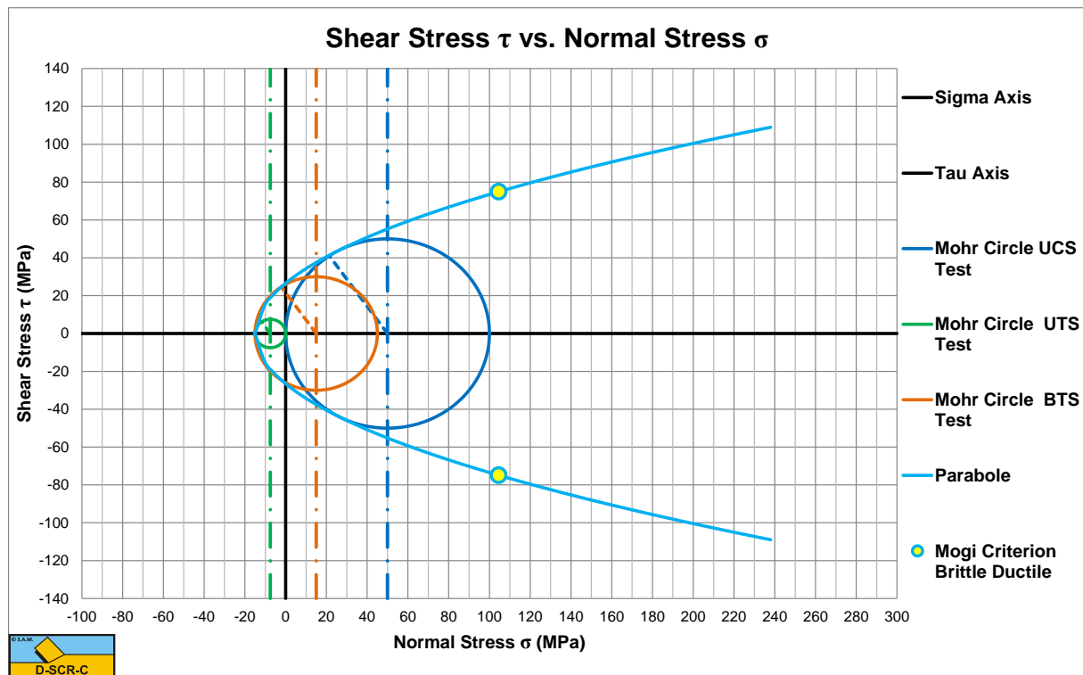
Figure 8-13: The parabolic failure criterion.
