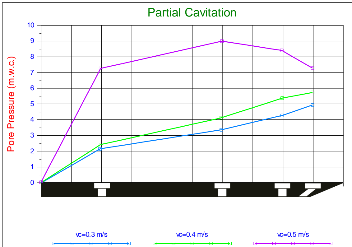
Figure M-2: Measured absolute pore pressures.
