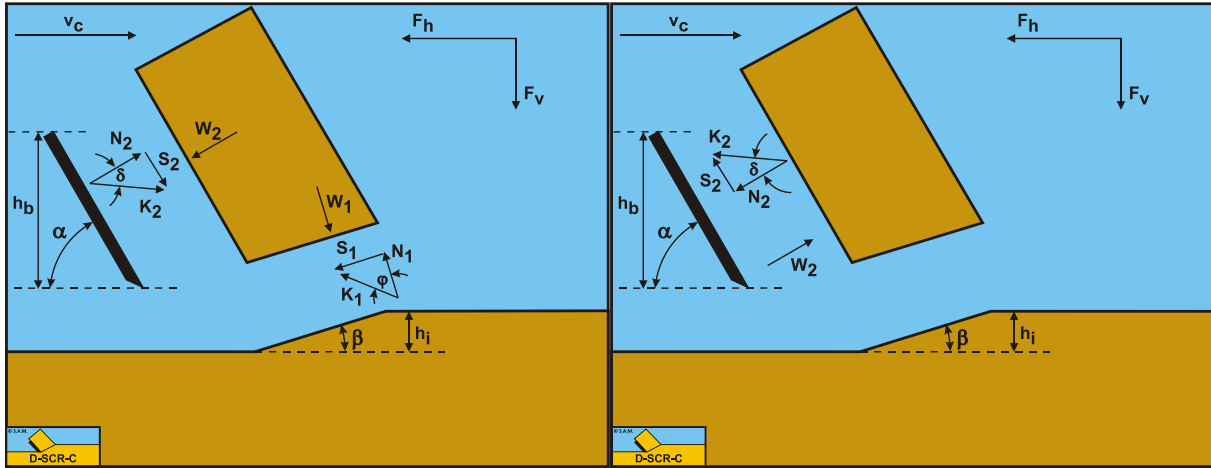
Figure 6-4: The forces on the layer cut in water saturated sand.
