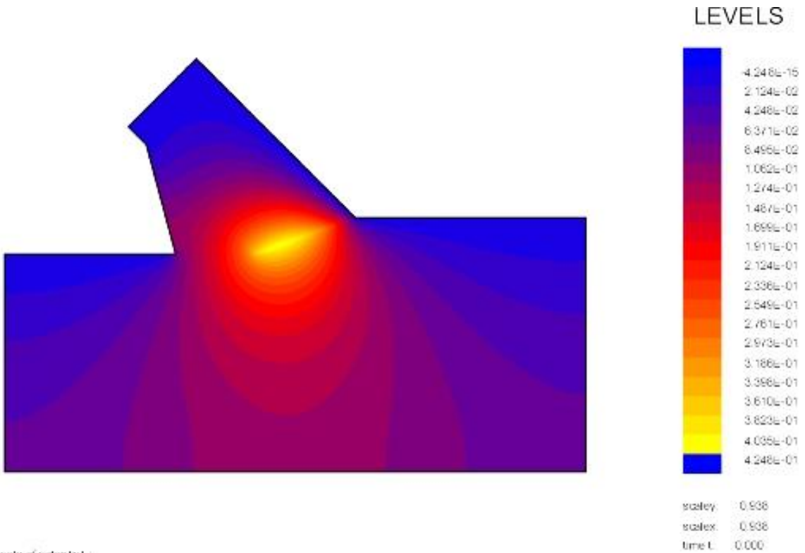
Figure S-11: The equipotential lines in color.
