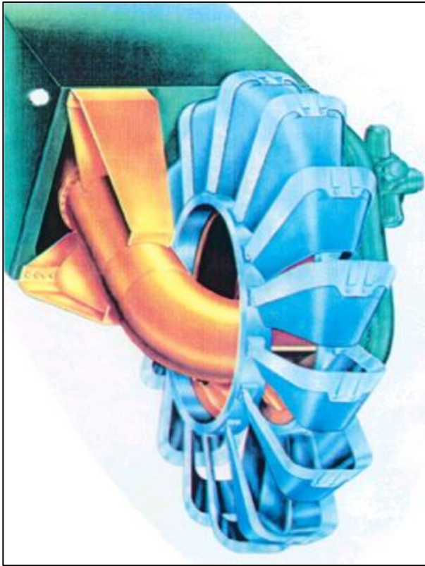
Figure Y-37: A bucket wheel dredge (IHC).
