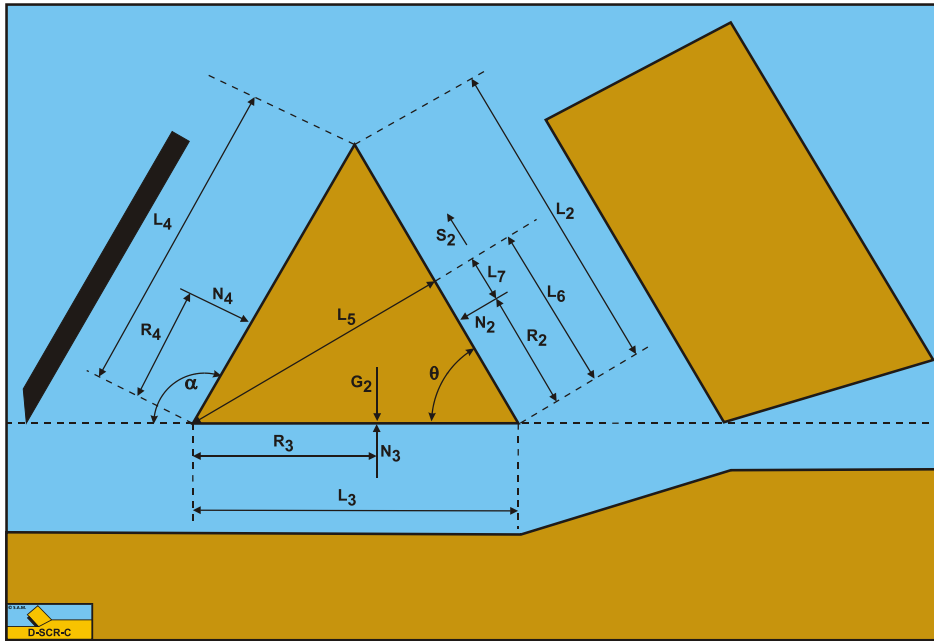
Figure 11-7: The moments on the wedge.
