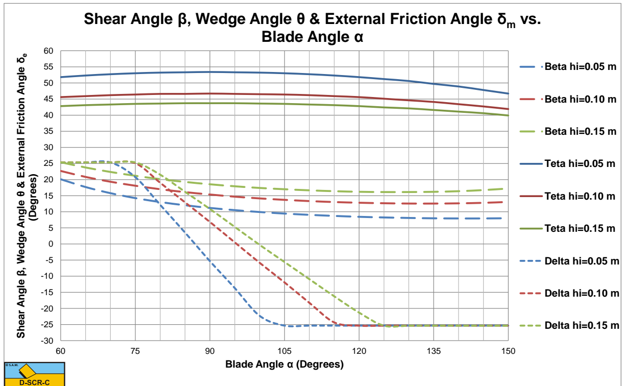
Figure 11-12: The shear angle, wedge angle and mobilized external friction angle calculated with wedge.
