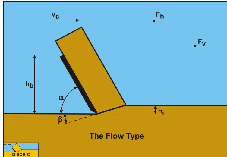
Figure 8-27: The Flow Type cutting mechanism in ductile rock cutting.
