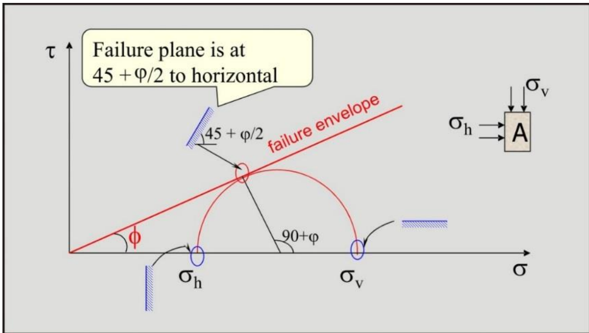
Figure 2-52: The Mohr circle for active soil failure.
