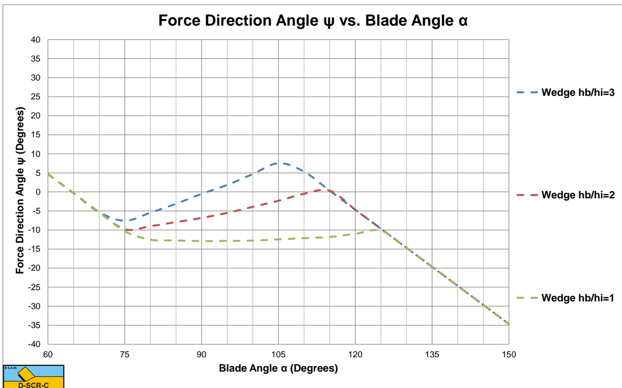
Figure 11-10: The direction of the total cutting force.
