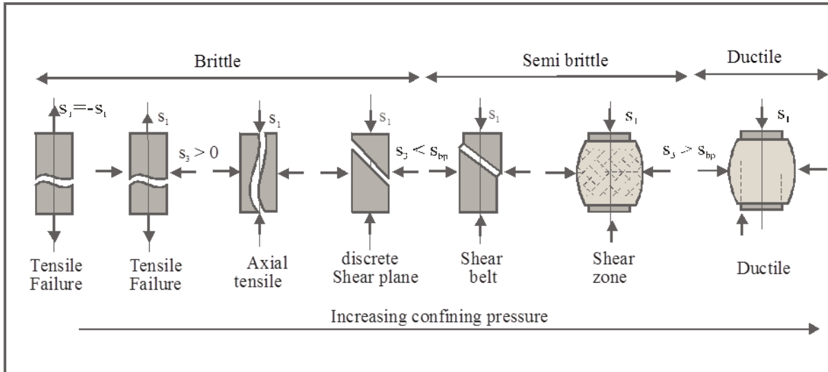
Figure 2-28: Brittle failure types (Vlasblom (2003-2007)).
