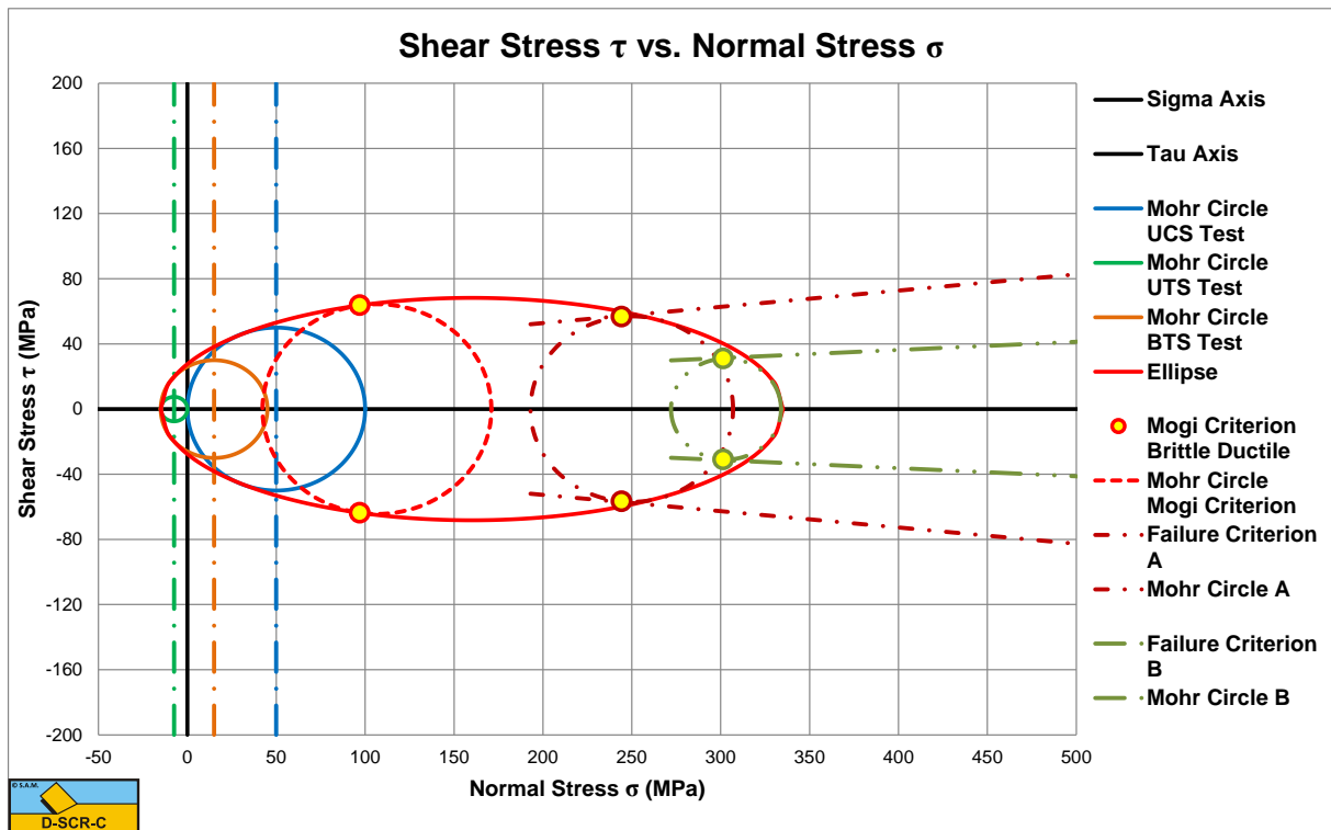
Figure 8-7: Resulting failure curves for Pierre Shale like rocks.
