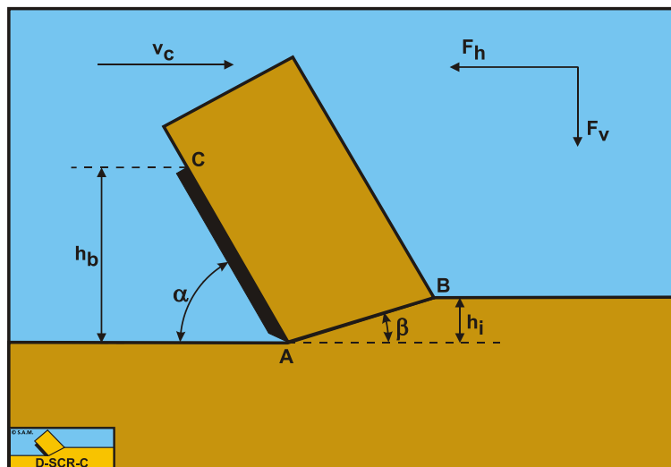
Figure 8-26: The definitions of the cutting process.
