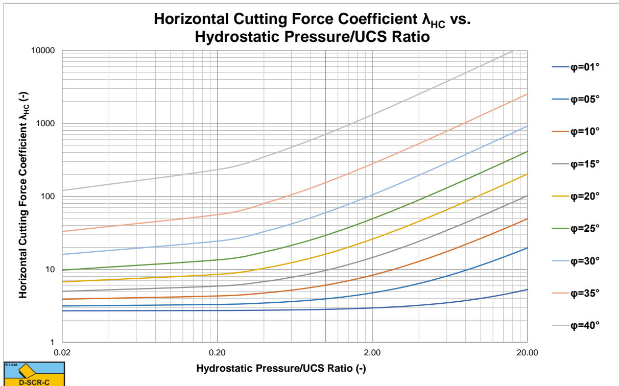
Figure X-28: The horizontal cutting force coefficient \lambda_{HC} for a 105 degree blade.
