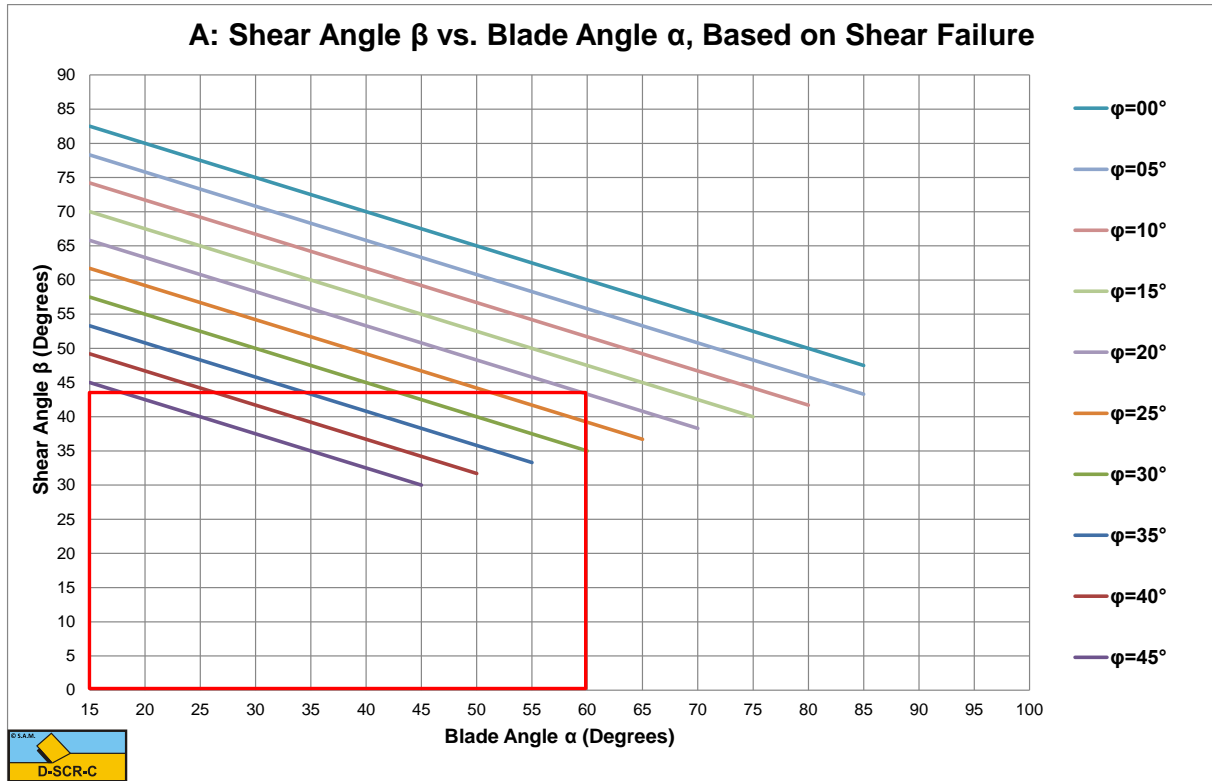
Figure 8-41: The shear angle with limitation.
