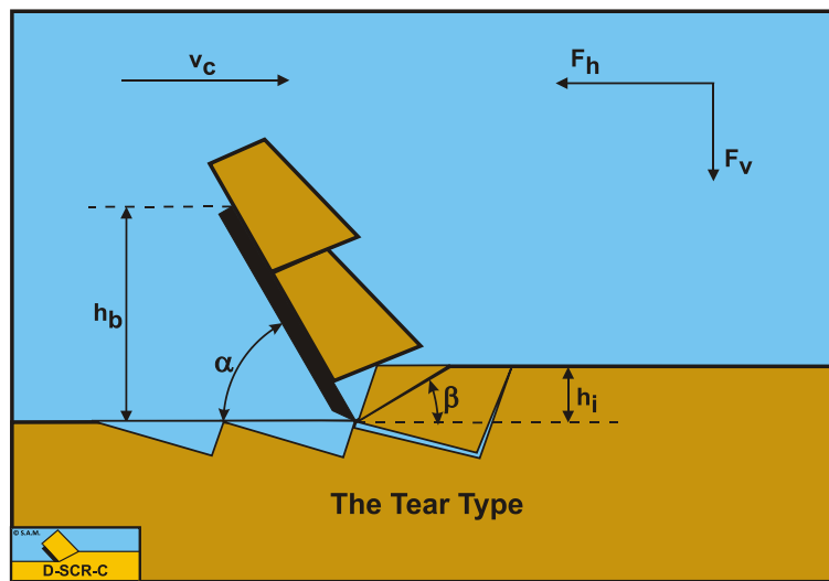
Figure 7-26: The Tear Type cutting mechanism in clay.
