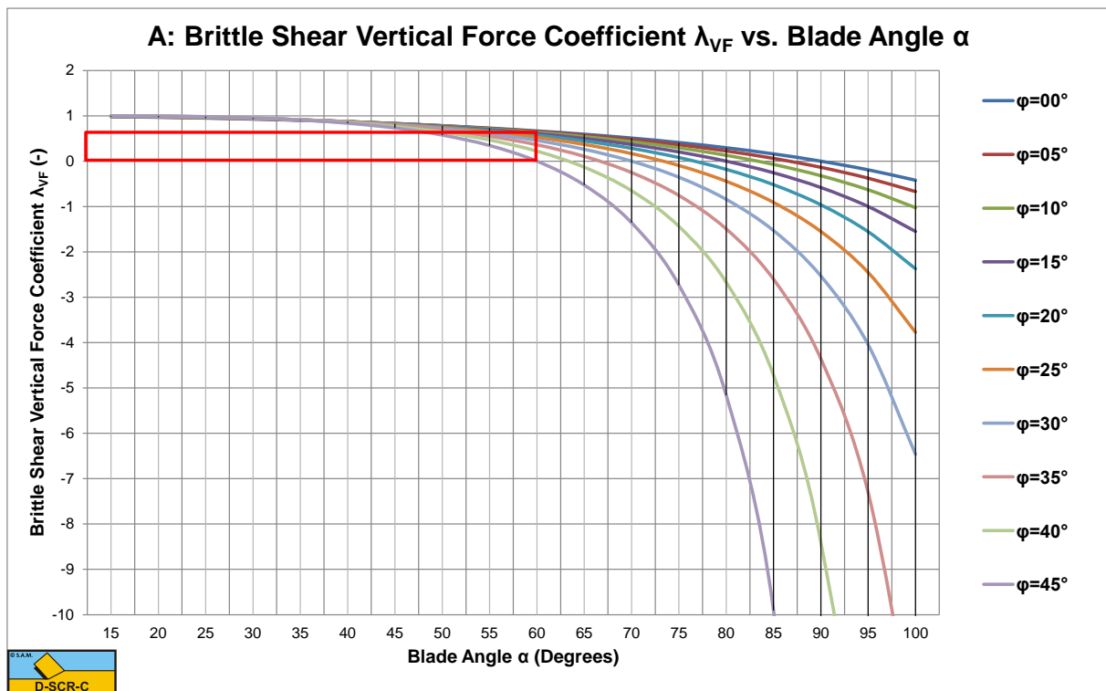
Figure 8-32: The brittle (shear failure) vertical force coefficient \lambda_{VF} .
