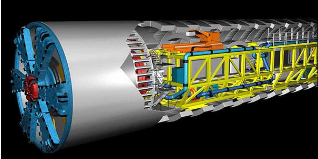
Figure Y-78: The WesterSchelde TBM.
