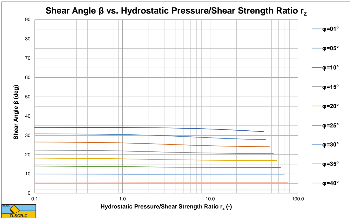
Figure 9-25: The shear angle \beta for a 110 degree blade.
