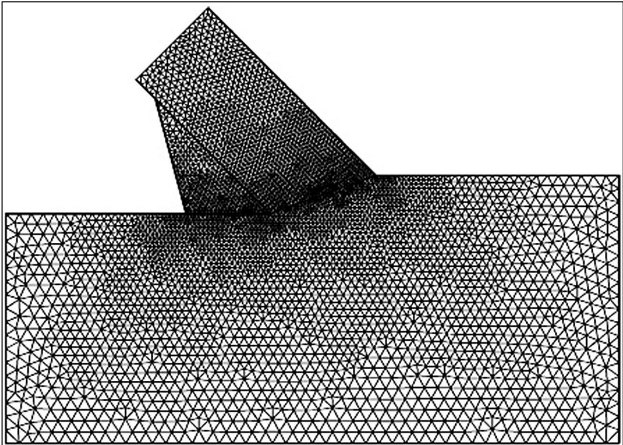
Figure 12-13: The fine mesh.
