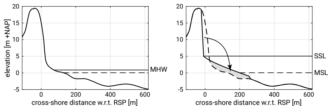
Figure 7.12: Left: profile during a calm period with normal water level and wave conditions (‘summer’ profile, see Fig. 1.13 for details). Right: profile as a result of storm wave height and surge conditions (‘winter profile’). The post-storm profile is computed according to Vellinga, see Fig. 7.18 for further info on the Vellinga profile and the storm conditions considered here.
