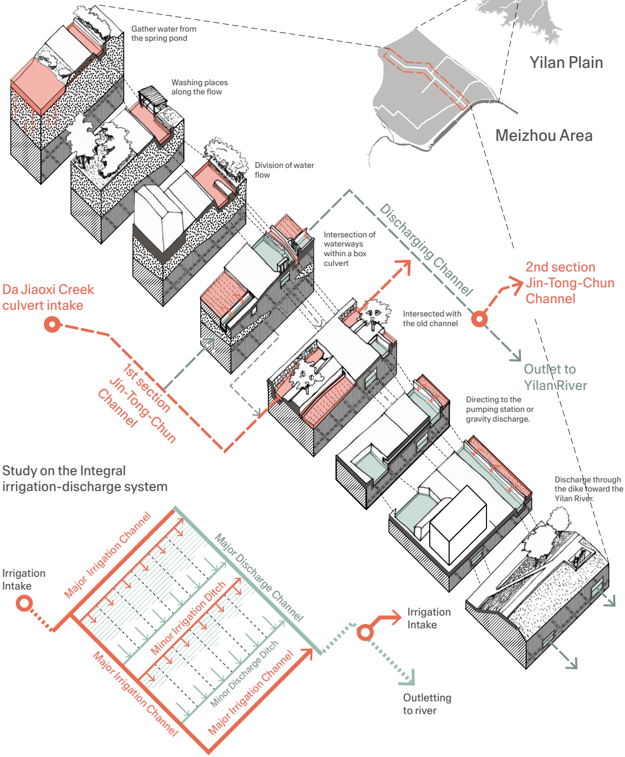
Fig. 17 Study of the Meizhou water system combined with spatial relationship diagrams, illustrating the complex network of pipes and ditches. Using one section of the area as an example, the drawing shows how the function of water channels changes with elevation: some irrigation ditches become drainage channels only a few hundred metres downstream. As the terrain becomes lower, the drainage network grows increasingly complex. The outlet to the main river includes both a gravity discharge and a pumping station designed to manage extreme rainfall events. By the authors.
