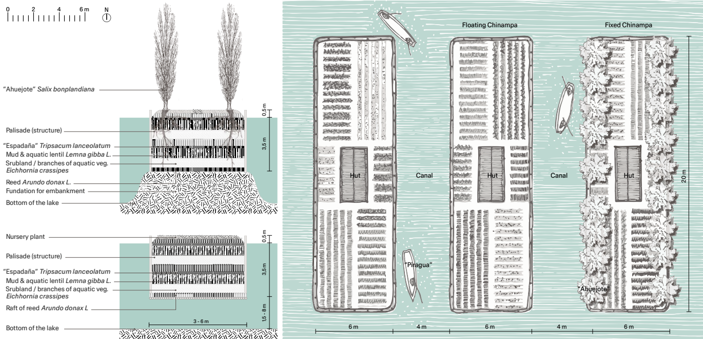
Fig. 2 Detailed plan and section of the Chinampas Farming System in Xochimilco, Mexico City, Mexico. Adapted from Bobbink and Rey-Hernández (2022).
