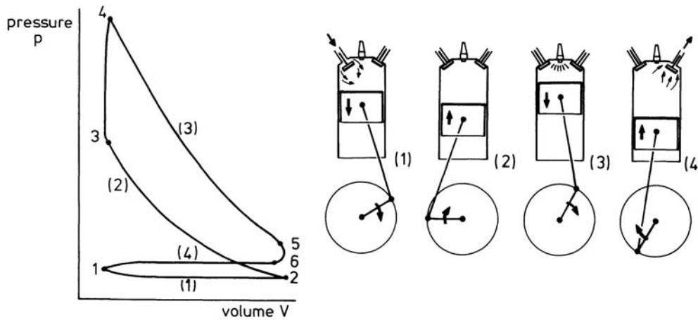
Figure 6.8 Working cycle of the four-stroke piston engine
