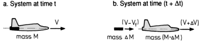
Figure 3.9 Ejection of airplane mass
