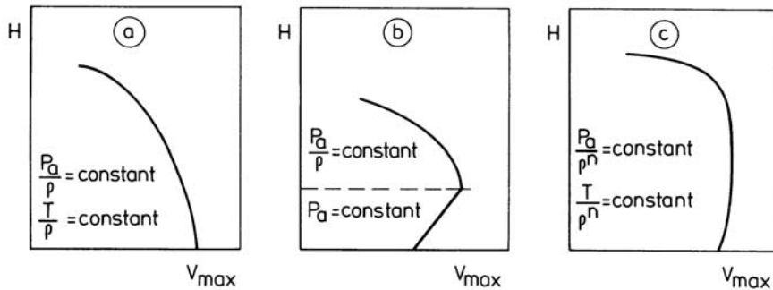
Figure 10.8 Altitude effects on maximum airspeed
