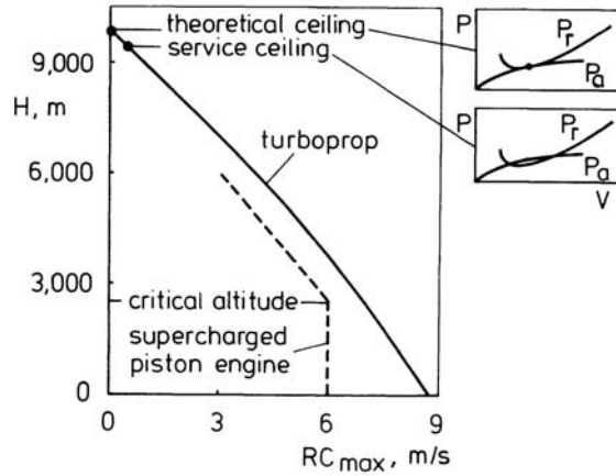
Figure 10.3 Maximum rate of climb versus altitude
