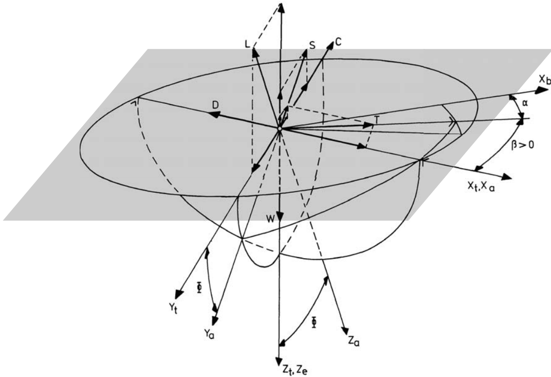
Figure 12.12 Forces in a slipping turn
