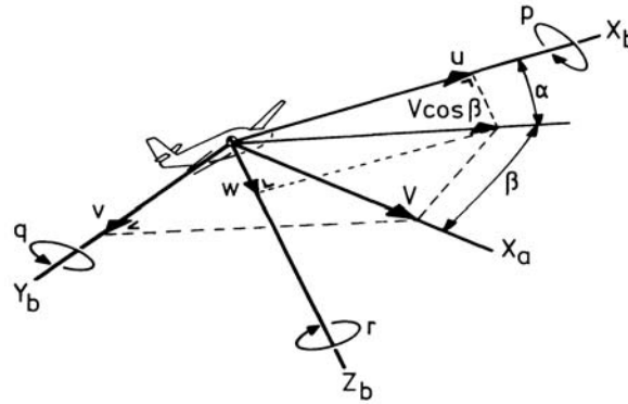
Figure 1.19 Components of airspeed
