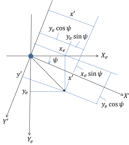
Figure B.1 Yaw rotation of angle \psi about the Z_e axis.
