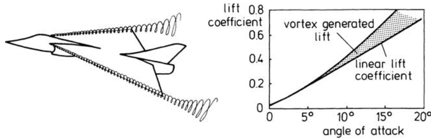
Figure 4.25 Excess lift due to delta-wing vortex flow from leading edges
