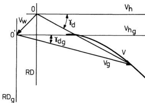
Figure 13.11 Effect of wind in the hodograph diagram
