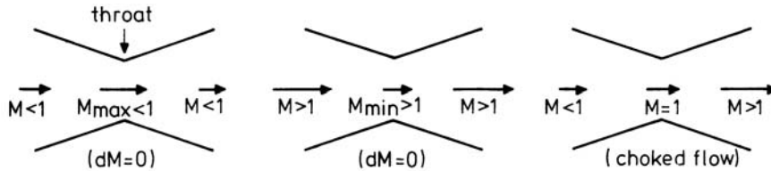
Figure C.9 Isentropic flow through a converging-diverging channel
