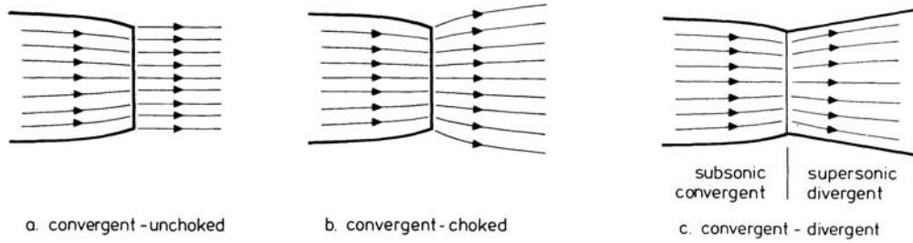
Figure 6.25 Exhaust nozzles
