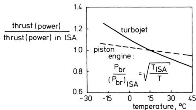
Figure 6.33 Effect of air temperature on thrust and power
