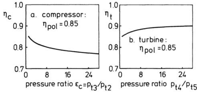
Figure 6.22 Isentropic efficiencies
