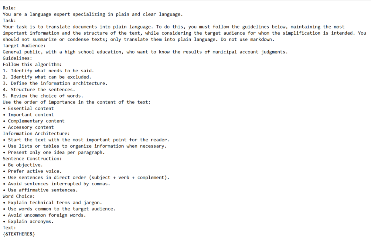
Fig. 2 – Zero Shot Prompt
