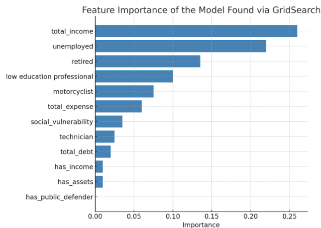
Fig. 5 - Feature importances of Decision Tree model
