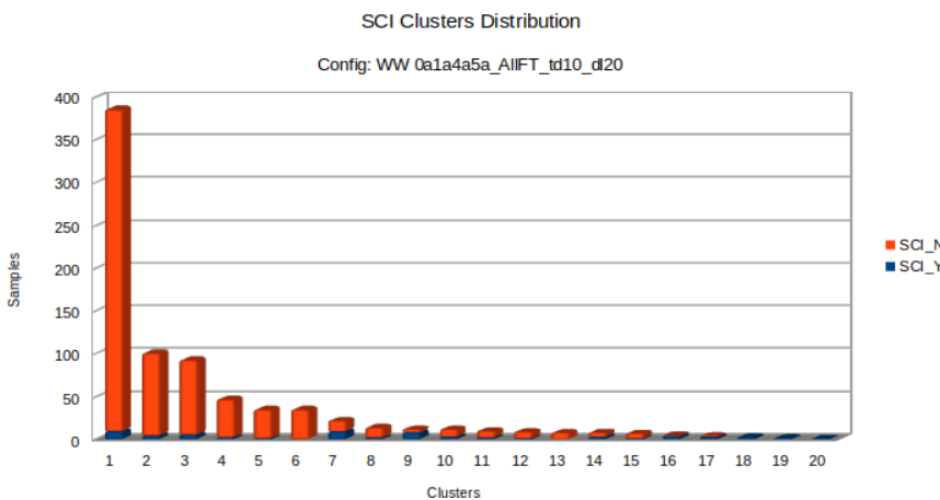
Fig. 3 – SCI clusters distribution using configuration WW_0a1a4a5a_AllFT.
