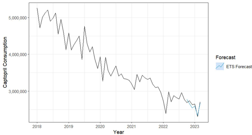
Fig. 9 - Forecast using the ETS model compared to actual consumption data. Source: Original research results.
