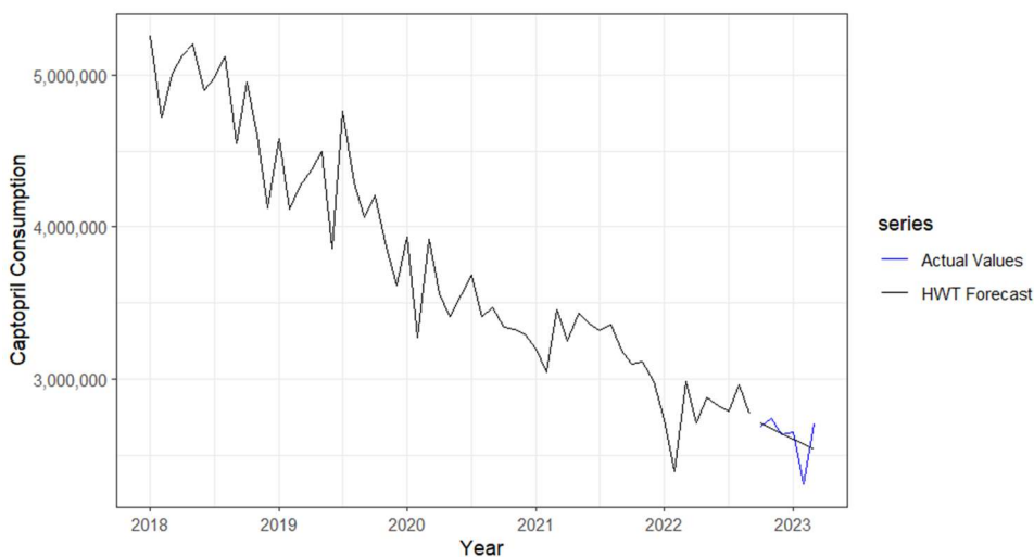
Fig. 6 - Comparison of forecast using the Holt-Winters method with trend and actual values. Source: Original
