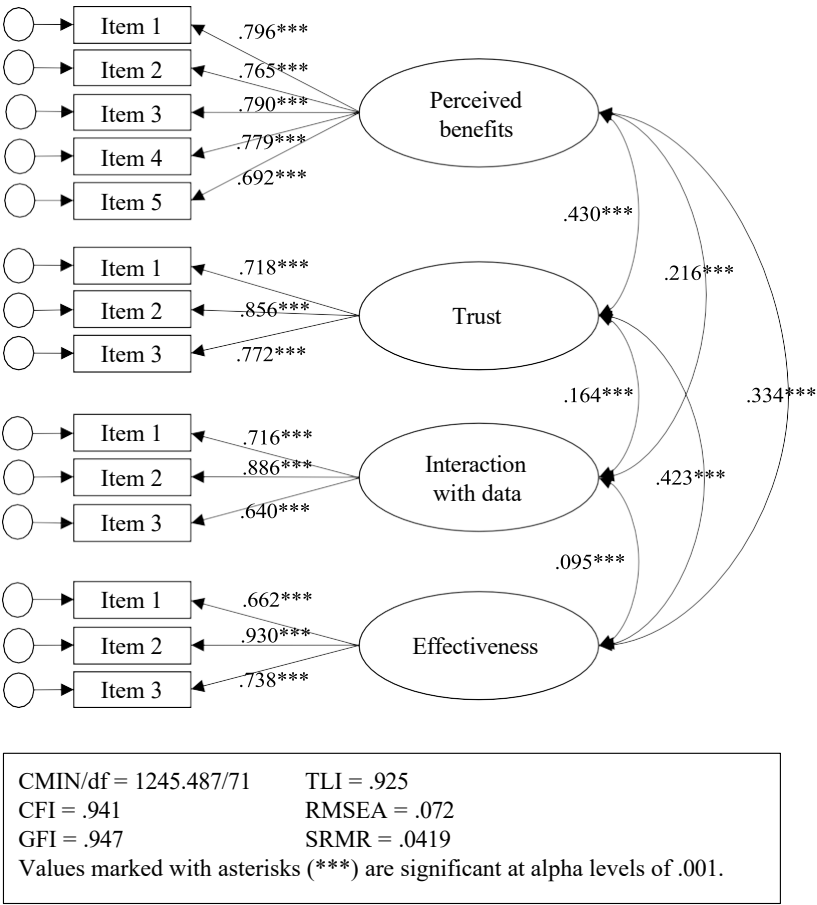
Fig. 1 - The measurement model, including its fit indices
