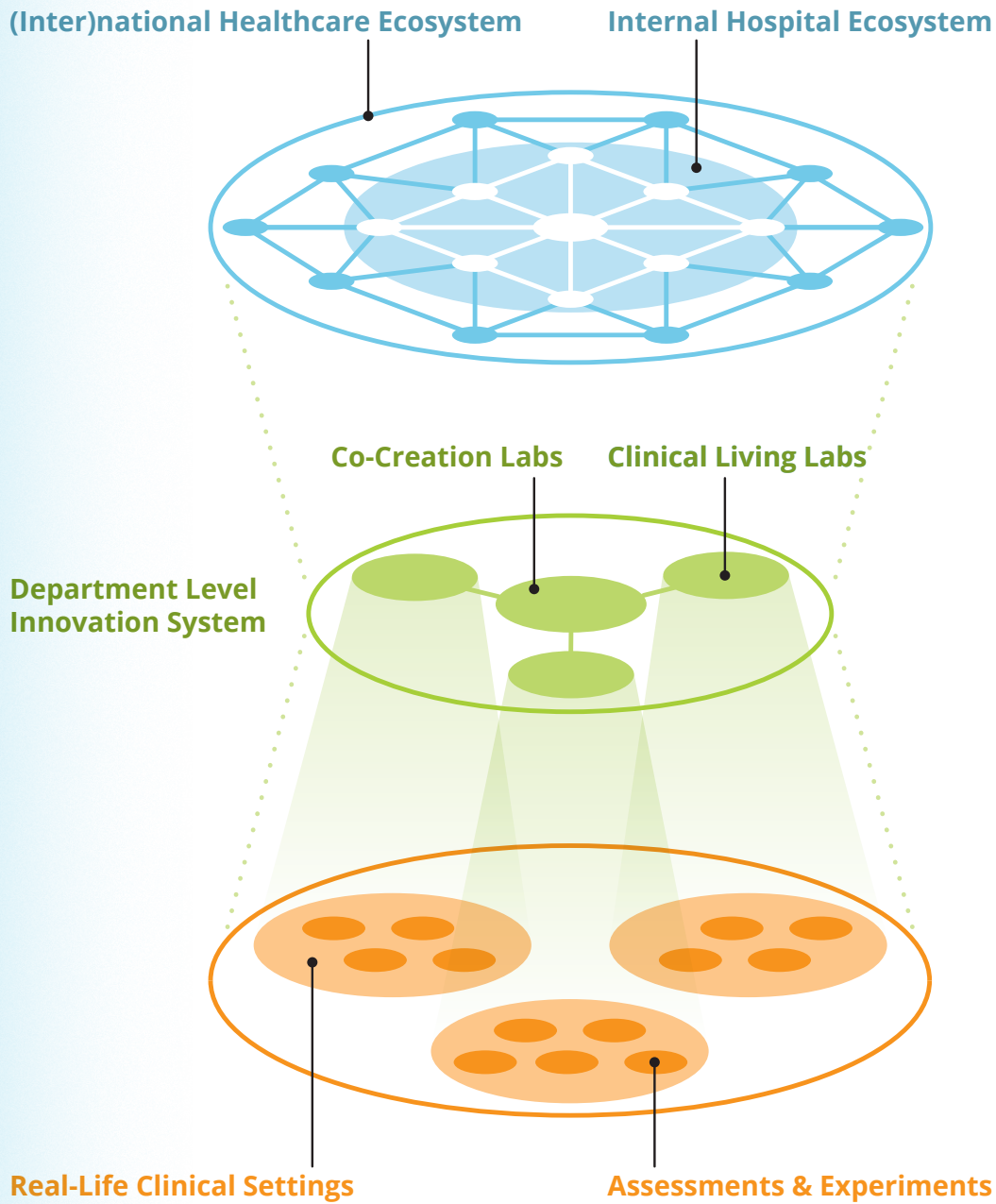
Figure 8: Multilevel Framework
