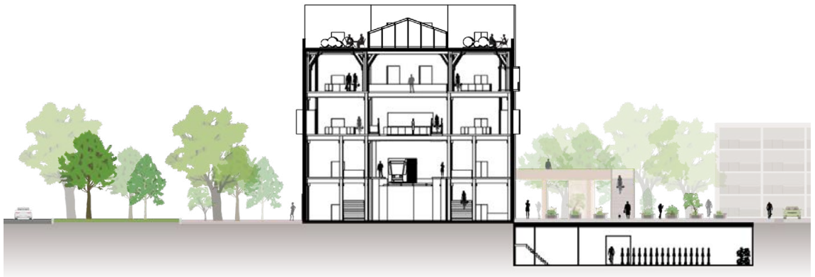
Plan and Section West to East Station and Square
